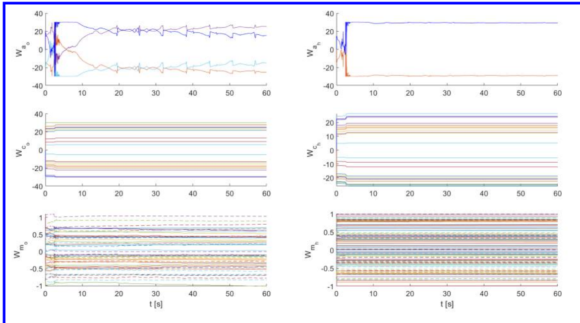
Fig. 13 The weights updates for the critic, actor and model networks (case BC2)
