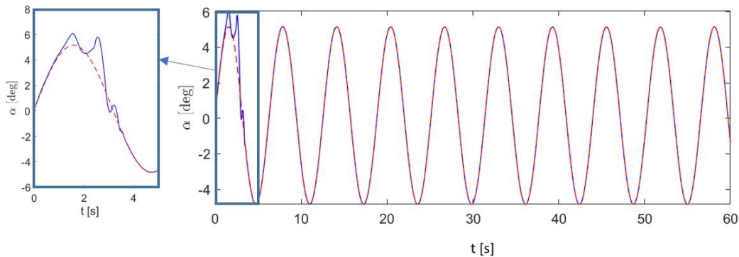
Fig. 10 The time history of the angle of attack response and reference signal with the first 5 seconds zoomed in (case BC2)
