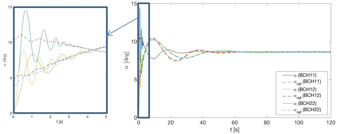
Fig. 16 The angle of attack reference signal and the response of the ICE plant for different benchmarking conditions with the outerloop altitude control
