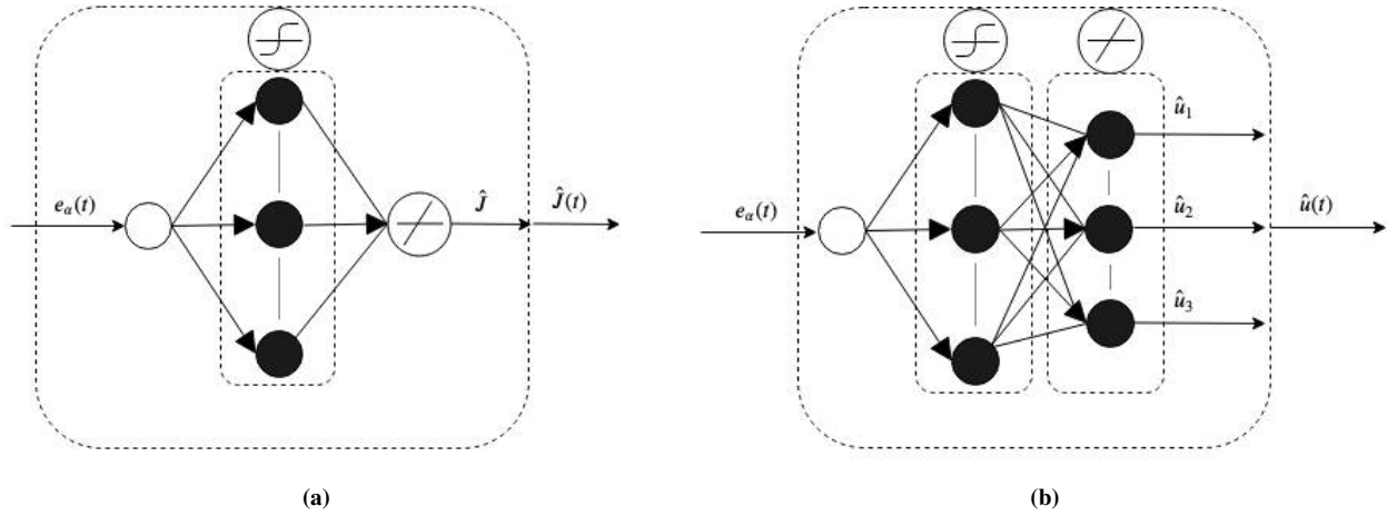
Fig. 6 Schematic of the proposed (a) critic and (b) actor networks
