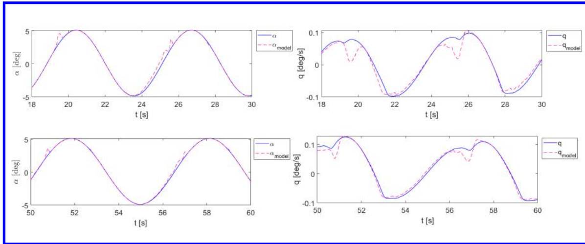
Fig. 12 The zoomed-in (case BC2) plot for model identification for the angle of attack and pitch rate between 18 to 30 seconds (top plots) and 50 to 60 seconds (bottom plots)
