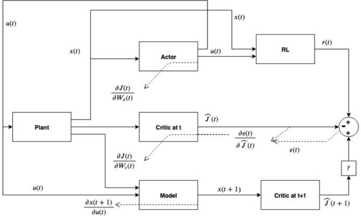
Fig. 3 HDP scheme block diagrams and updates based on [19]
