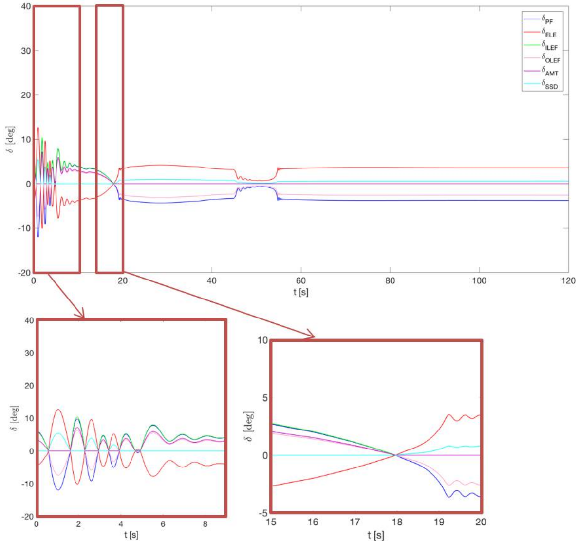
Fig. 20 The effectors responses for BCH22 case
