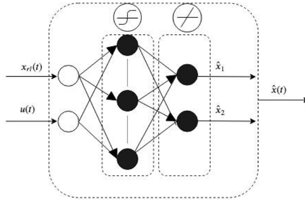
Fig. 7 Schematic of the proposed model network
