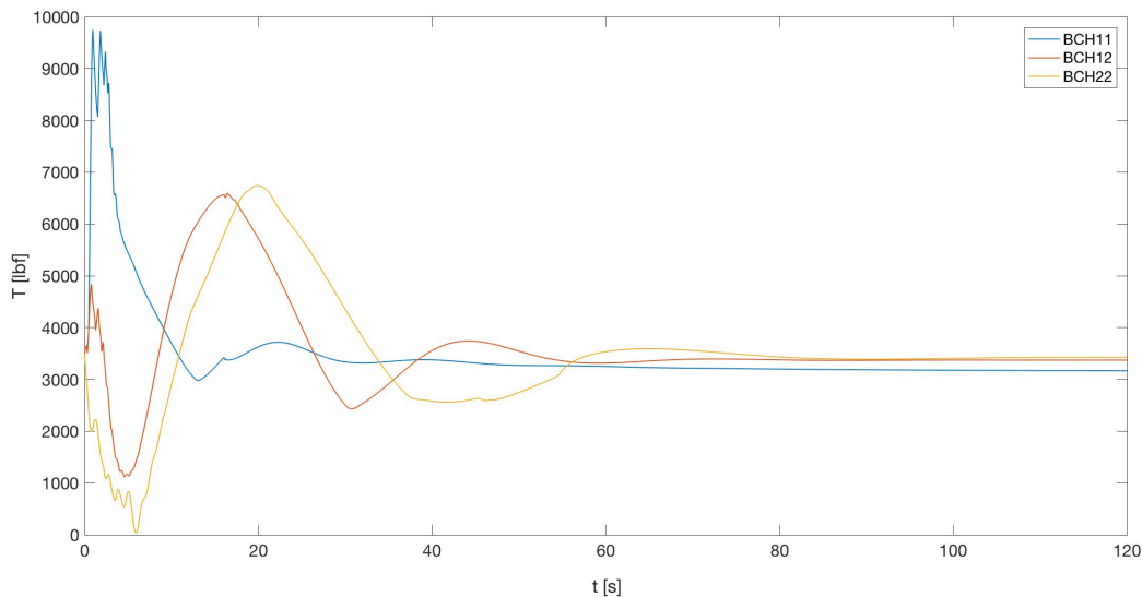
Fig. 17 The thrust values for different benchmarking conditions with the outerloop altitude control
