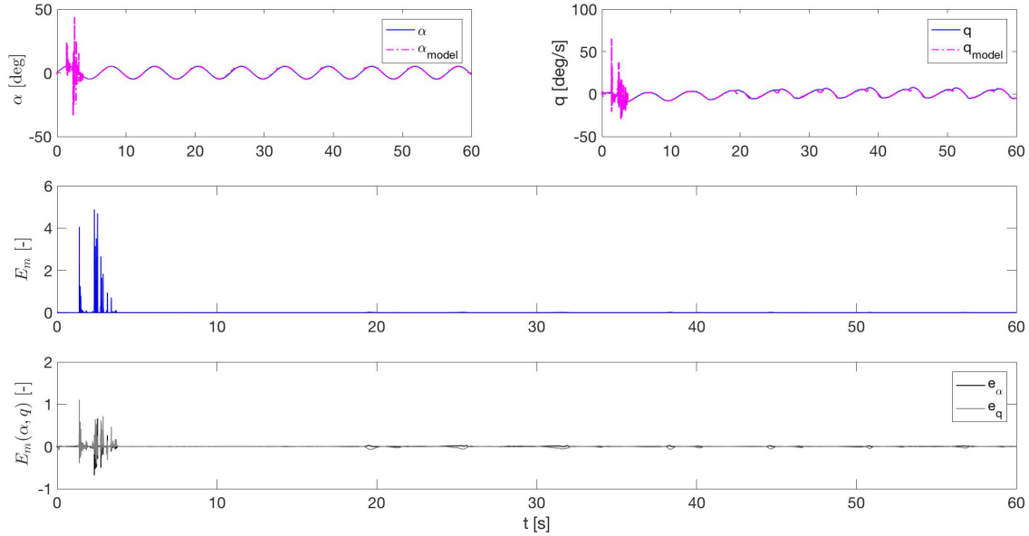
Fig. 11 The online model identification results with the angle of attack and pitch rate plant and model responses on top, the overall model error in middle and the angle of attack and pitch rate errors in the bottom (case BC2)
