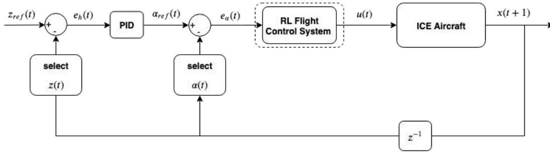
Fig. 8 Layout of the altitude control framework including the RL and the outer loop PID controllers
