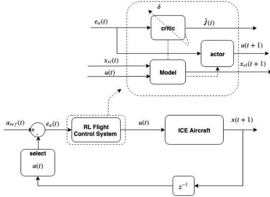
Fig. 5 Layout of the control loop including the reinforcement learning controller for attitude control of the ICE aircraft
