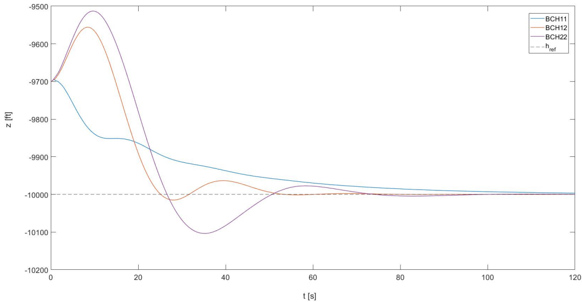
Fig. 15 The altitude tracking results for different benchmarking conditions with 300 ft offset
