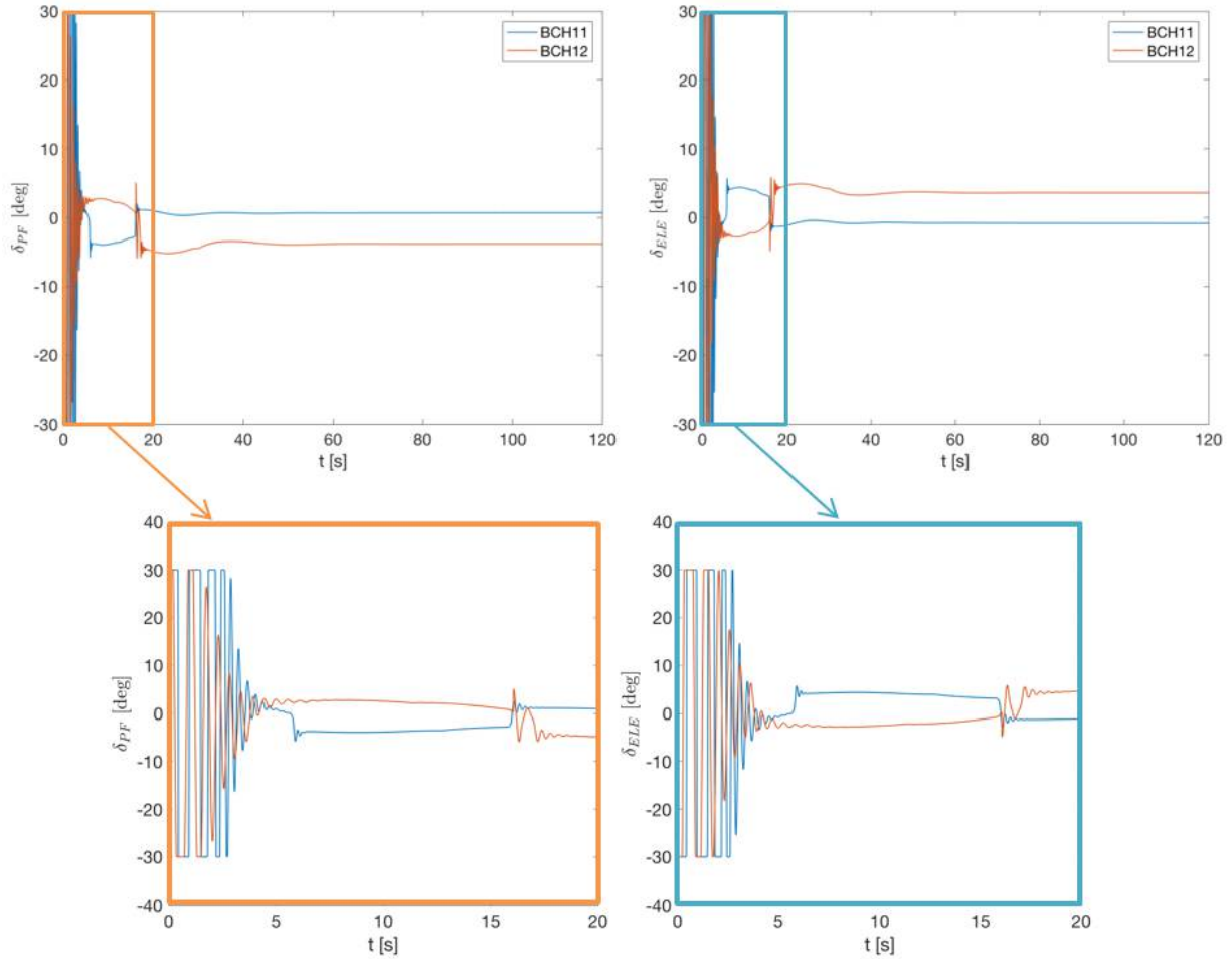
Fig. 19 The pitch flap and elevon responses for BCH11 and BCH12
