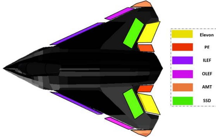
Fig. 4 ICE aircraft control suite
