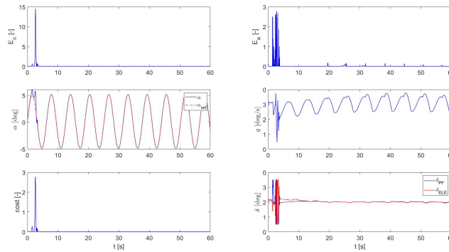
Fig. 9 The attitude control results with the critic network error in top left, the actor network error in the top right, the angle of attack response and the reference angle of attack in the middle left, the pitch rate response in the middle right, the cost value in bottom left, the effectors deflection in the bottom right (case BC2)
