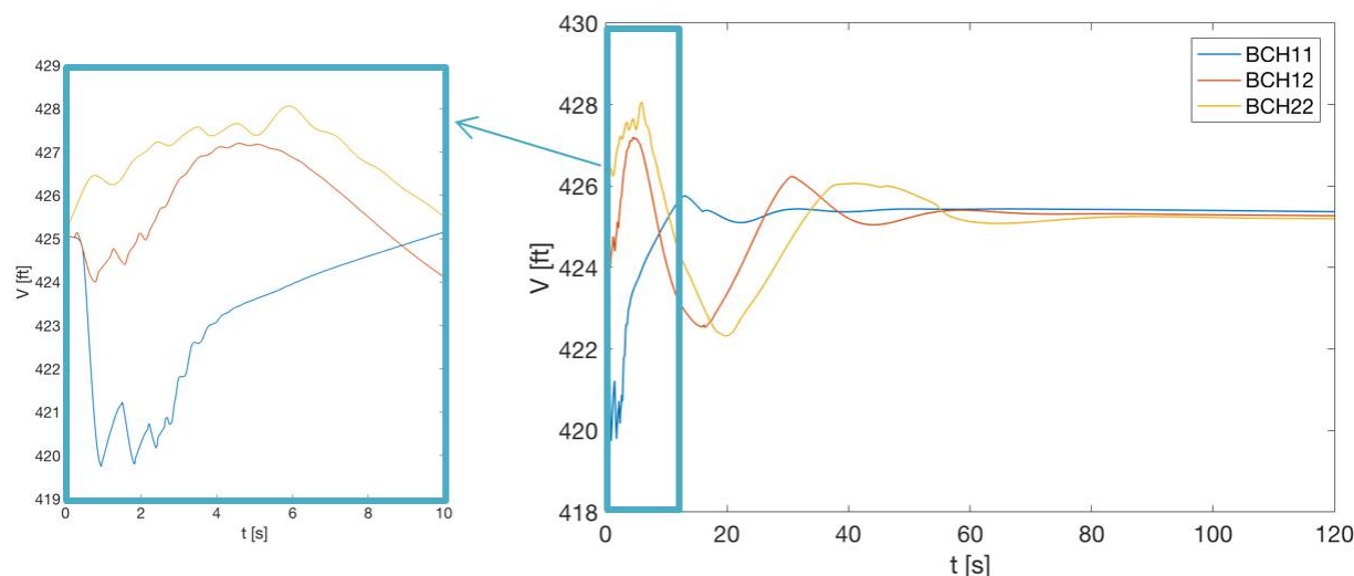
Fig. 18 The airspeeds for different benchmarking conditions with the outerloop altitude control
