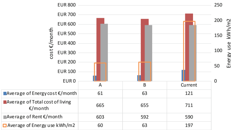
Fig. 26.3 Comparison of the thermal properties upgrade options and the current building, in terms of energy
