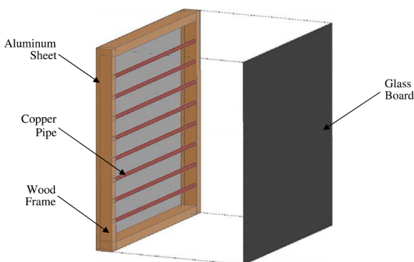
Fig. 10. New PCM-based insulation wall [76].
