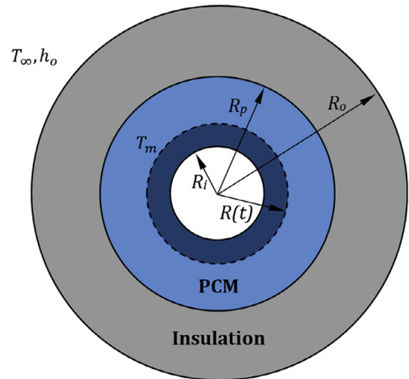
Fig. 26. Analytical model [92].
