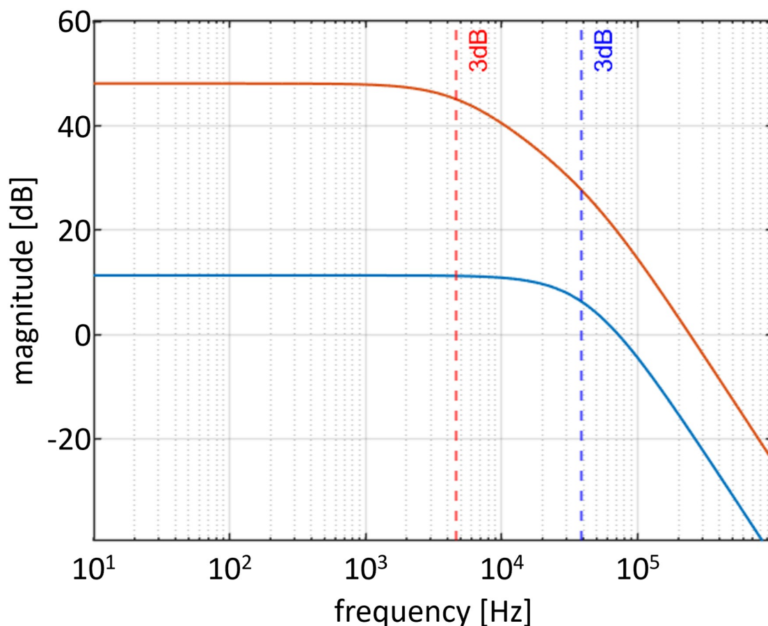
Fig 5. Frequency response simulation of the two-stage, low-noise transimpedance amplifier circuit, indicating a bandwidth of 4.68 kHz for a total gain of 50 MV A -1 (red) and a bandwidth of 39 kHz for a total gain of 6 MV A -1 (blue).
