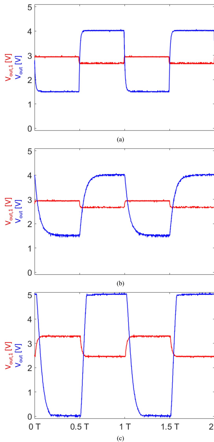
Fig 8. Response of the two-stage, low-noise transimpedance amplifier circuit with 2.8V bias for a square wave signal input with an amplitude of 337 nA, recorded using an oscilloscope. The output voltage after the first stage is illustrated in red; the output voltage after the second stage is illustrated in blue. (a) Input signal frequency of 300 Hz with a 50% duty cycle, G_1 = 440 \text{ kV A}^{-1} . (b) Input signal frequency of 1.5 kHz with a 50% duty cycle, G_1 = 440 \text{ kV A}^{-1} . (c) Input signal frequency of 1.5 kHz with a 50% duty cycle, G_1 \geq 831 \text{ kV A}^{-1} .
