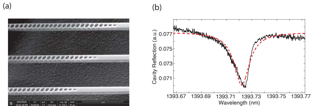
Fig. 2. (a) SEM image of fabricated nanophotonic devices. (b) Reflection spectrum of one of the devices with total Q factor \sim 100,000 .
