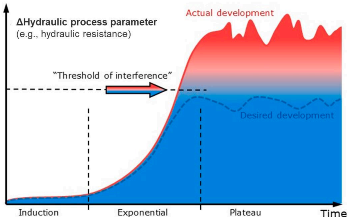
Fig. 1. Development of biofilms and the “Threshold of interference” above which biofouling is reported. The \Delta (Parameter) represents the absolute change in any important hydraulic process parameter (e.g., hydraulic or friction resistance, pressure drop, permeate flux) due to the biofilm formation. While the actual process development exceeds the threshold (red curve), it is desired to keep the biofilm effects below this threshold of interference (adapted after Flemming (2011)).
