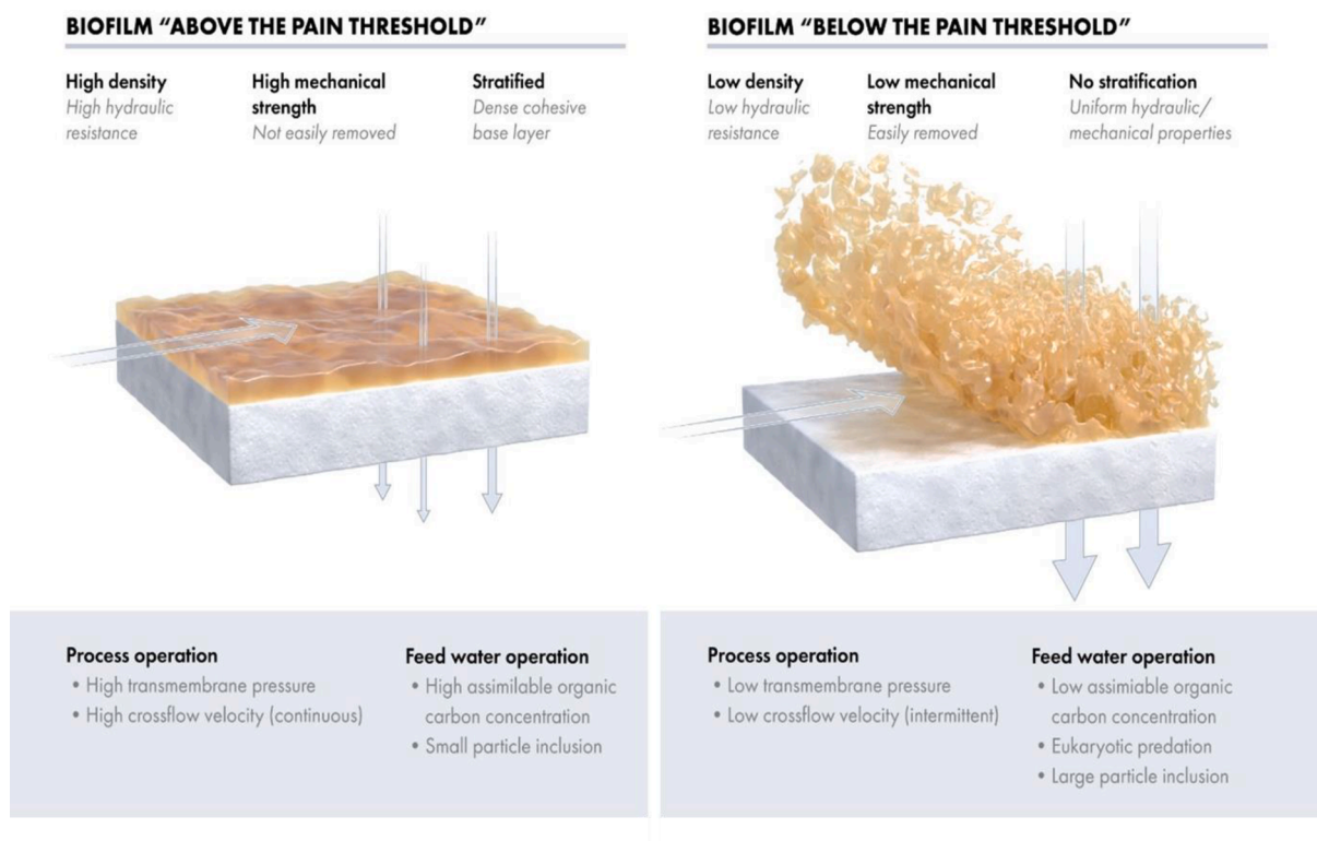
Fig. 8. Physical structure of biofilms above and below the pain-threshold in membrane filtration systems: Process operation and feed water quality can lead to biofilms effective both above and below the pain threshold. Biofilms below the pain threshold (with low density and hydraulic resistance) can be engineered under conditions of low assimilable organic carbon concentration and a process operation defined by a constant TMP/permeate flux. Biofilms above the pain threshold occur under conditions of high AOC concentration and a process operation defined by increasing TMP (leading to biofilm compaction) and with high continuous crossflow velocities (leading to thin and dense biofilms). Image is a graphical representation of reviewed studies in Section 3 which report variation on biofilm physical structure in response to alternation in feedwater quality and/or process operation (Desmond et al., 2018a, Desmond et al. 2021, Desmond et al., 2018c, Jafari et al., 2018, Javier et al., 2020a, Javier et al., 2020b).
