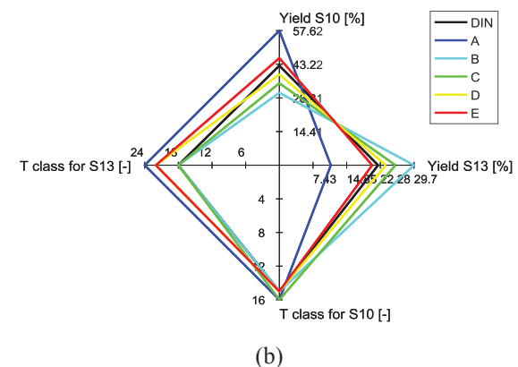
Figure 5: Spider web plot with optimization solutions for optimization of yield and strength to S13 and S10 for Norway spruce selected by: (a) Grade combination T18-T15, (b) same total yield to S13 and S10 compared to DIN 4074 (DIN)
