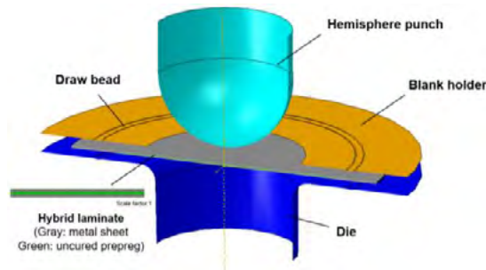
Fig.3: Finite element model of the hot-pressing process for uncured hybrid laminates
