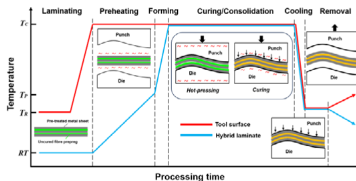
Fig.1: Processing temperature-time profile of the tool surface and hybrid laminates
