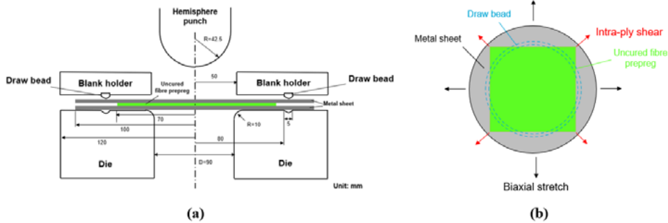
Fig.2: (a) Schematic graph of the double-curved dome forming tool design and dimension; (b) Deformation mechanisms and initial shapes of the individual metal sheet and fibre prepreg
