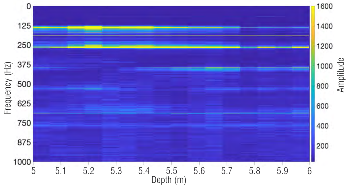
Figure 3 A power spectral density plot of a 10 s recording with a 2 kHz time sampling and a 40-m gauge length. At a depth level of around 5.7 m, there appears to be a transition zone. This can either be a very liquid mud or this is due to the averaging effect of the 40-m gauge length.
