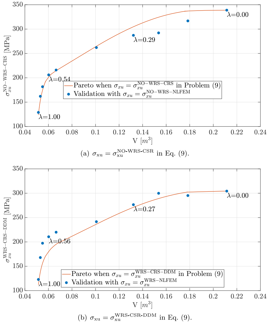
Fig. 5. Optimal V and the optimal \sigma_{xu} varying \lambda in Eq. (9) creating the Pareto fronts when replacing \sigma_{xu} with \sigma_{xu}^{\text{NO-WRS-CSR}} or \sigma_{xu}^{\text{WRS-CSR-DDM}} . For some \lambda s (i.e., the ones that brings a particular optimal volume V \in [0.2114, 0.1322, 0.0602, 0.0515] ) authors reported for verification purposes at the optimal point the \sigma_{xu}^{\text{NO-WRS-NLFEM}} when \sigma_{xu} = \sigma_{xu}^{\text{NO-WRS-CSR}} is exploited in Eq. (9) and \sigma_{xu}^{\text{WRS-NLFEM}} when \sigma_{xu} = \sigma_{xu}^{\text{WRS-CSR-DDM}} is exploited in Eq. (9).
