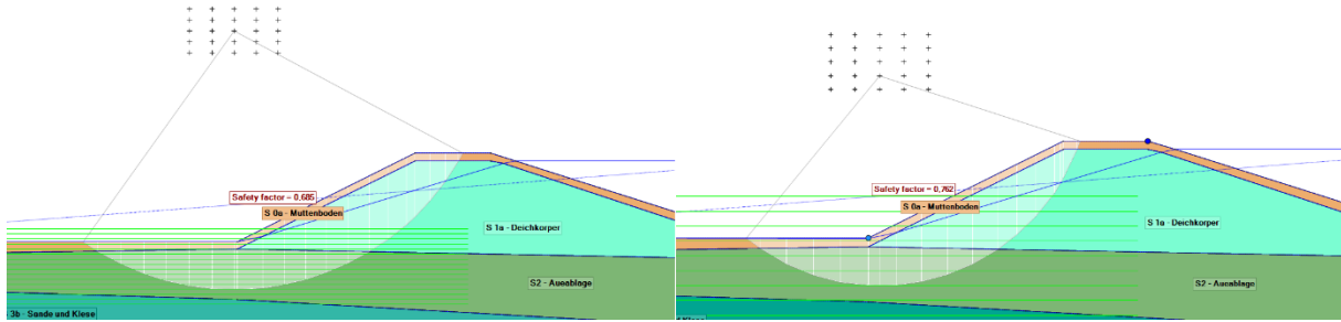
Figure 16 Left: View of scenario A. “Base model” using the Bishop slip circle and low values of POP resulting in FoS=0.69 (undrained soil behavior). Right: Scenario A. “Base model” using the Bishop model and low values of cohesion resulting in FoS=0.76 (drained soil behavior).
