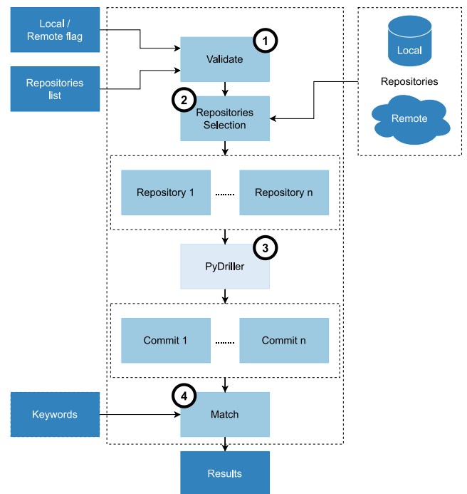
Fig. 2. PyRock Architecture.
