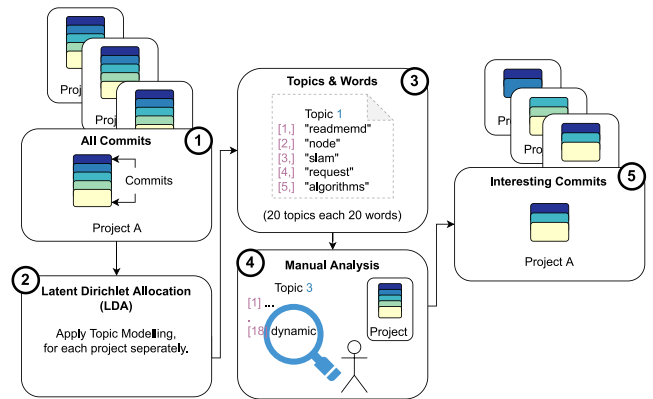
Fig. 1. Topic-Modeling process.
