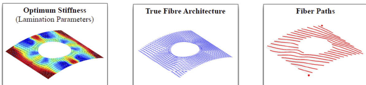
Figure 1. schematic overview of the three-step optimisation approach [64]
