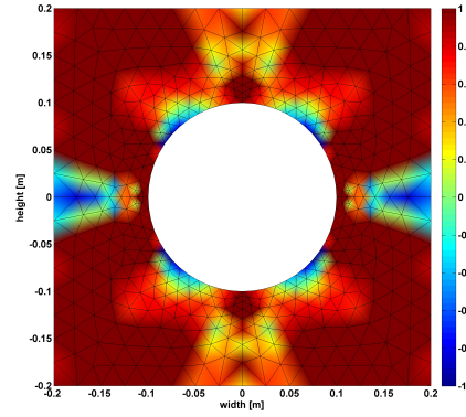
(b) V_3 distribution for optimal stiffness
