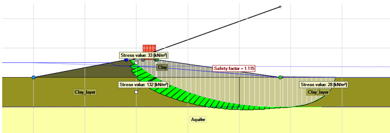
Figure 3. Simple slope geometry with clay dike on clay blanket on top of a sand aquifer.
