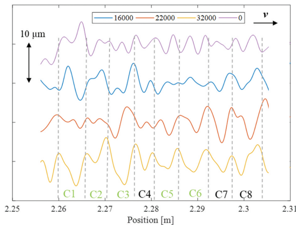
Figure 8. Measured corrugation geometry after the 16,000, 22,000 and 32,000 rotations in the spatial domain from the 3D HandyScan tests. The result at '0' rotation corresponds to the initial rail roughness without wheel passages.
