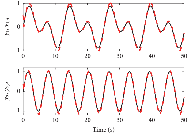
FIGURE 1: Outputs y_1 and y_2 and desired trajectories y_{1,d} and y_{2,d} .
