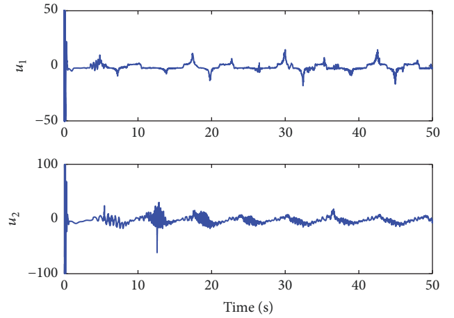
FIGURE 7: Control inputs u_1 and u_2 .
