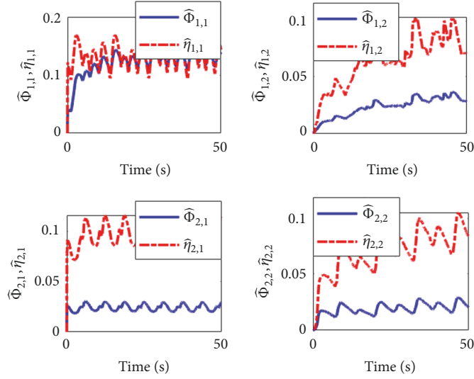
FIGURE 8: Adaptive parameters \hat{\Phi}_{1,1} , \hat{\eta}_{1,1} , \hat{\Phi}_{1,2} , \hat{\eta}_{1,2} , \hat{\Phi}_{2,1} , \hat{\eta}_{2,1} , \hat{\Phi}_{2,2} , and \hat{\eta}_{2,2} .
