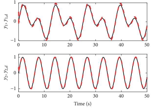
FIGURE 6: Outputs y_1 and y_2 and reference signals y_{1,d} and y_{2,d} .
