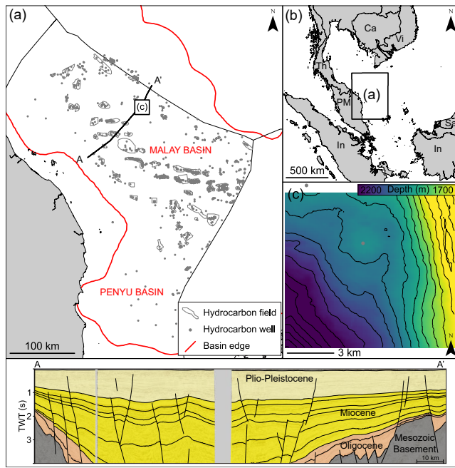
Fig. 1. (a) Map of offshore Peninsular Malaysia showing the outlines of major sedimentary basins, hydrocarbon fields, wells, and the locations of (c) and cross-section A-A', (b) inset map showing (a)'s position in relation to the wider Southeast Asia region and (c) top reservoir surface map in the J Area. A-A': Seismic cross-section showing the main stratigraphic units (after de Jonge-Anderson et al. (2024)). Ca: Cambodia, In: Indonesia, PM: Peninsular Malaysia, Th: Thailand, TWT: two-way-time, Vi: Vietnam.
