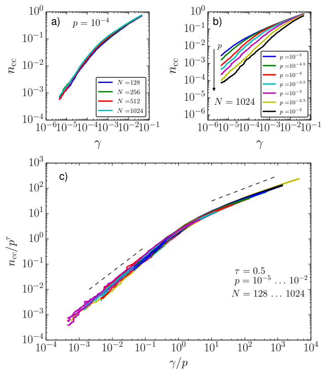
Fig. 7 The contact change density shown for (a) varying system size and (b) varying pressure. (c) Data collapse for pressures p = 10^{-2} \dots 10^{-5} in half decade steps and system sizes N = 128 \dots 1024 in multiples of 2. Dashed lines indicate slopes of 1 and 1/2.
