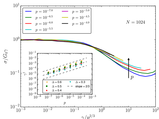
Fig. 6 (main panel) The dimensionless shear modulus of quasistatically sheared Hertzian packings plotted versus the rescaled strain \gamma/p^{2/3} . (inset) Pressure-dependence of the crossover strain \gamma^\dagger .
