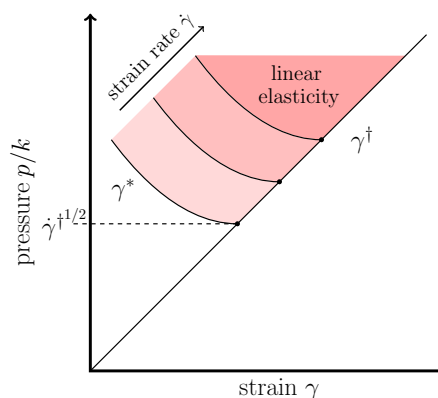
Fig. 9 In a flow start-up test, quasistatic linear response ( G \approx G_0 ) occupies a strain window \gamma^* < \gamma < \gamma^\dagger (shaded regions). For smaller strains the response is rate-dependent, with a crossover strain \gamma^* that depends on both pressure and strain rate. Softening sets in for higher strains, with a crossover \gamma^\dagger that depends only on the pressure. The intersection of the rate-dependent and softening crossovers defines a strain rate \dot{\gamma}^\dagger above which there is no quasistatic linear response, i.e. the shaded region closes.
