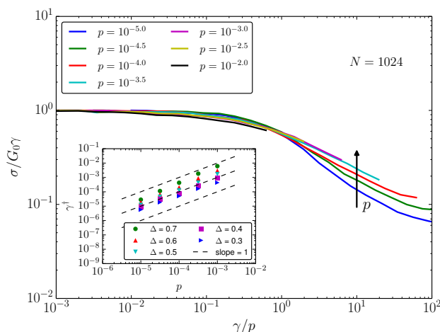
Fig. 5 (main panel) Data from Fig. 4, expressed as a dimensionless effective shear modulus \sigma/G_0\gamma and plotted versus the rescaled strain \gamma/p . (inset) The crossover strain \gamma^\dagger where the effective shear modulus has decayed by an amount \Delta in a system of N = 1024 particles.
