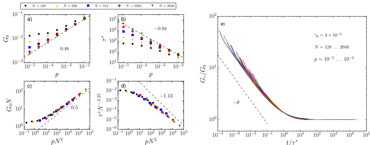
Fig. 3 (a) The linear shear modulus G_0 in harmonic packings for varying pressure p and number of particles N . (b) The relaxation time \tau^* for the same range of p and N as in (a). (c) Finite size scaling collapse of G_0 . (d) Finite size scaling collapse of \tau^* . (e) The relaxation modulus G_r collapses to a master curve when G_r and t are rescaled with G_0 and \tau^* , respectively, as determined in (a) and (b). At short times the master curve decays as a power law with exponent \theta = \mu/\lambda \approx 0.44 (dashed line), using the estimates from (c) and (d).
