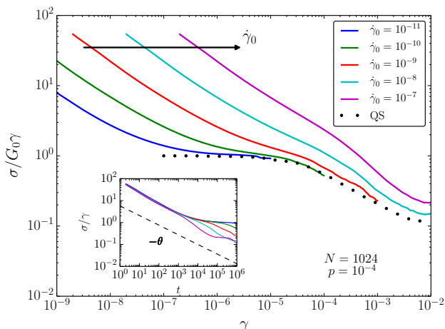
Fig. 8 The effective shear modulus during flow start-up for packings of N = 1024 particles at pressure p = 10^{-4} , plotted versus strain for varying strain rates \dot{\gamma}_0 . (inset) The same data collapses for early times when plotted versus t , decaying as a power law with exponent \theta = \mu/\lambda \approx 0.44 (dashed line).
