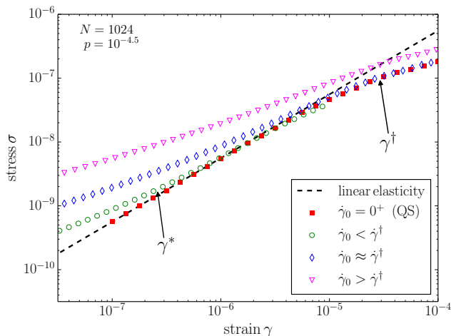
Fig. 1 Ensemble-averaged stress-strain curves of packings sheared at varying strain rate \dot{\gamma}_0 . Close to the jamming point the linear stress-strain curve (dashed line) predicted by Hooke's law holds over a narrow interval at low strain, with deviations due to viscous and plastic dissipation. The crossover strains \gamma^* and \gamma^\dagger are indicated for the data sheared at slow but finite rate 0 < \dot{\gamma}_0 < \dot{\gamma}^\dagger (open circles).
