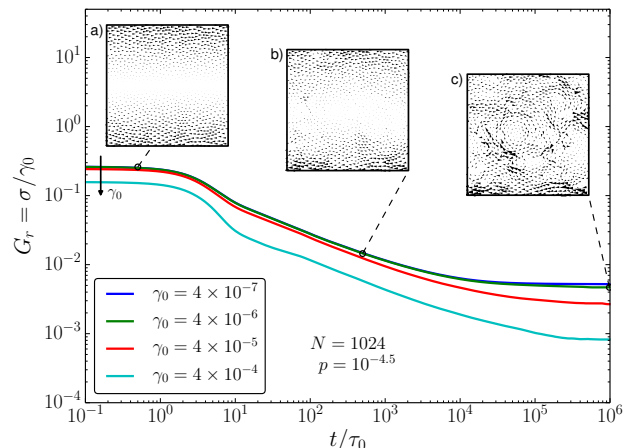
Fig. 2 The ensemble-averaged relaxation modulus G_r at pressure p = 10^{-4.5} for four values of the strain amplitude \gamma_0 . In all four cases, G_r displays an initial plateau corresponding to affine particle motion (inset a), followed by a power law decay as the particle displacements become increasingly non-affine (b). At long times the stress is fully relaxed and the final particle displacements are strongly non-affine (c).
