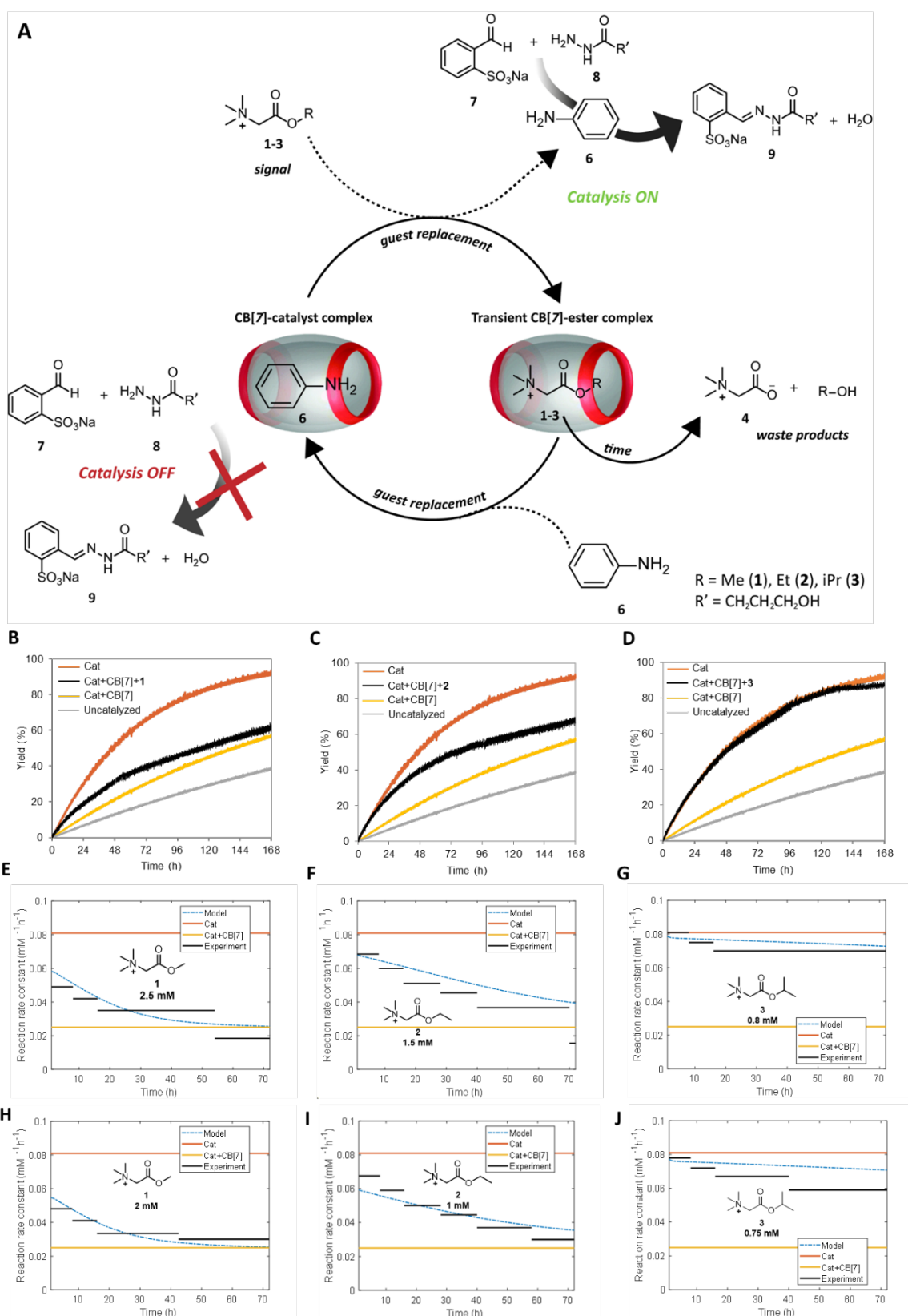
Figure 3: (A) Transient complex formation of hydrolysable ester signals with CB[7] to control the rate of hydrazone formation by aniline catalyst 6 capture and release. Yield (B-D) and rate constant (E-J) for hydrazone formation as a function of time at various catalytic conditions. Values extracted from experimental data with ester signals (black lines) are compared with the model (blue dashed line): (B,E) Methyl ester 1 2.5 mM, (C,F) Ethyl ester 2 1.5 mM, (D,G) Isopropyl ester 3 0.8 mM, (H) Methyl ester 1 2 mM, (I) Ethyl ester 2 1 mM and (J) Isopropyl ester 3 0.75 mM. Conditions: pH 7.5, 100 mM phosphate buffer; 0.2 mM aldehyde 7 , 0.02 mM hydrazide 8 , 0.2 mM catalyst 6 and 0.6 mM CB[7].
