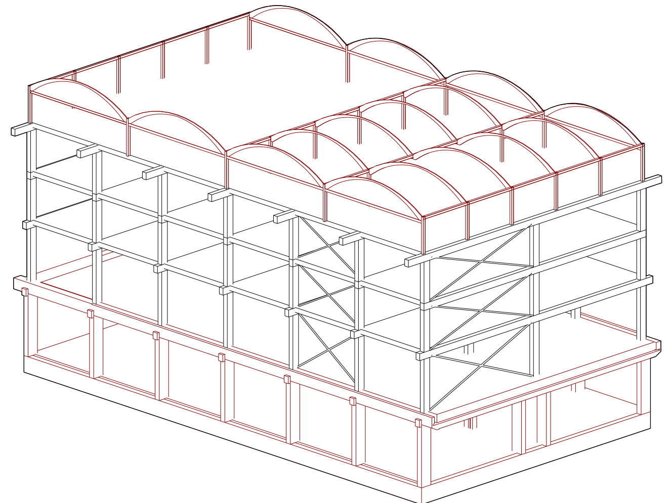
proposed structure design
