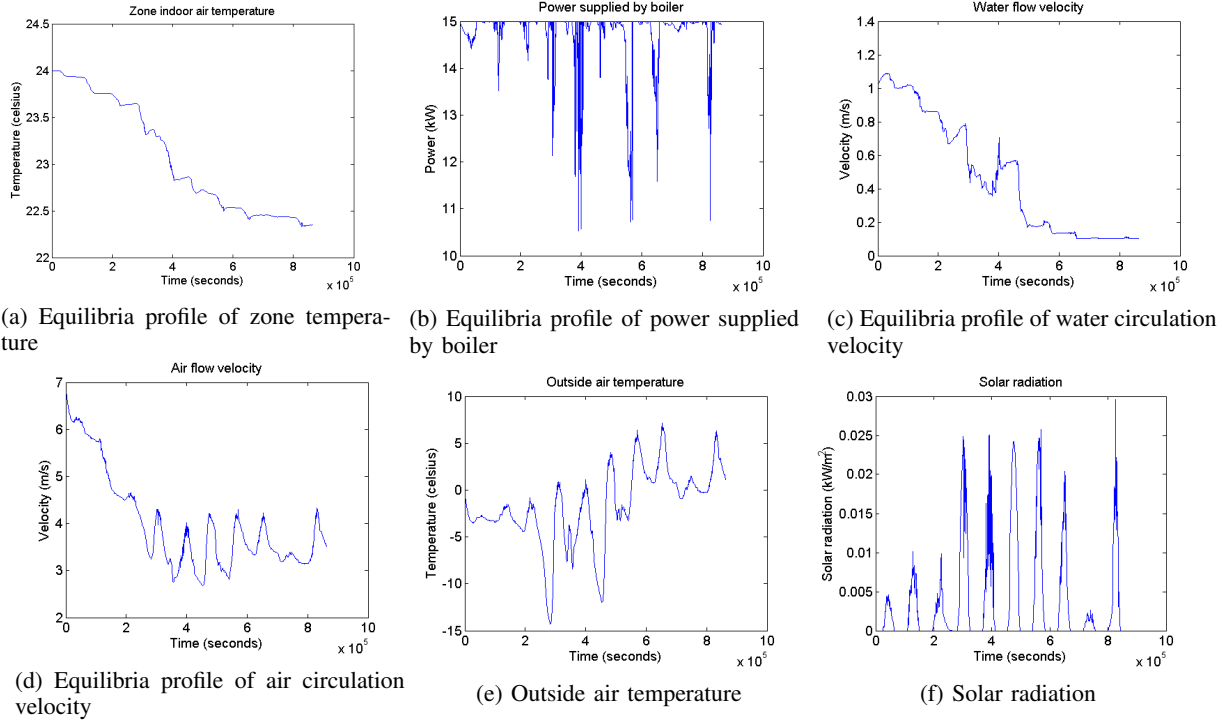
Fig. 2: (a)-(b)-(c)-(d): Equilibria profile of selected states and inputs. Fig. 2: (e)-(f): Few disturbances acting on the system
