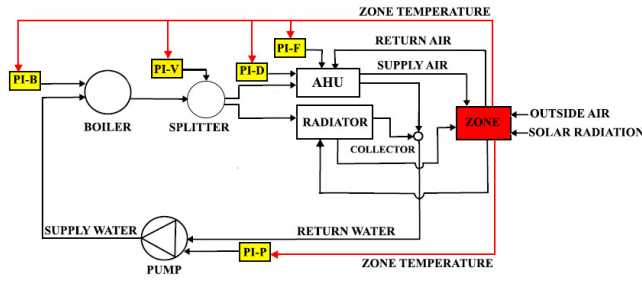
Fig. 1: HVAC system and control architecture
