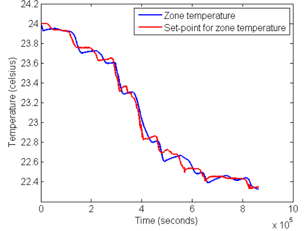
Fig. 3: Zone temperature using optimal PI
