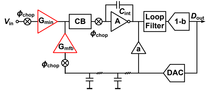
Fig. 7. Closed-loop CFIA-like BDC: Gm-C CTΔΣM BDC.
