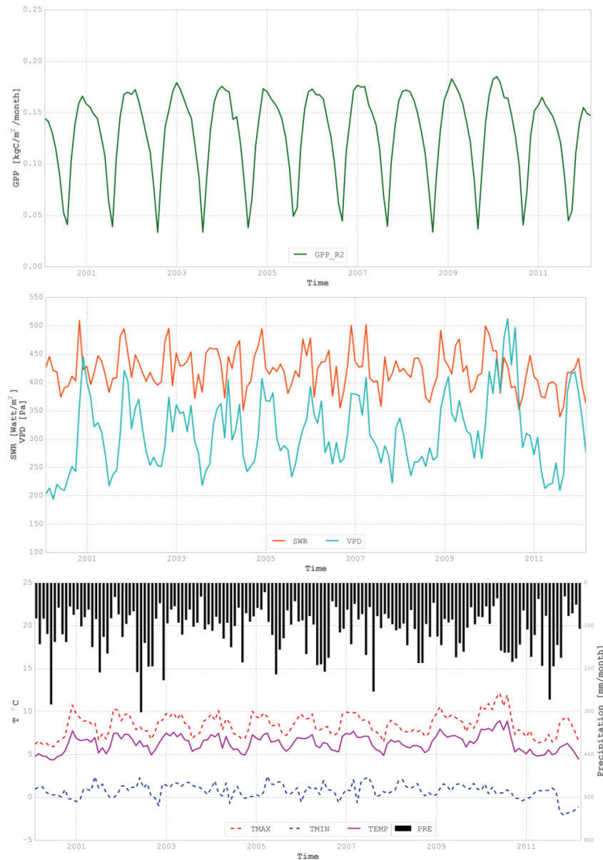
Figure 5-2 Monthly time-series data of GPP and meteorological variables for 12 years (2000 - 2011) at altitudinal range R2 (4200-4400 m a.s.l.)
