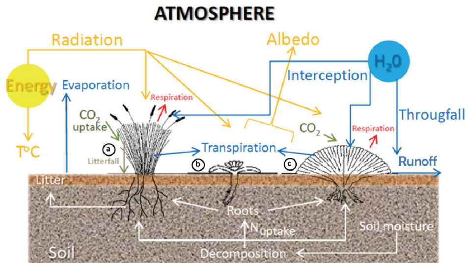
Figure 4-5 BIOME-BGC detailed model flow chart for a) Tussocks, b) Acaulescent Rosettes, and c) cushions.
