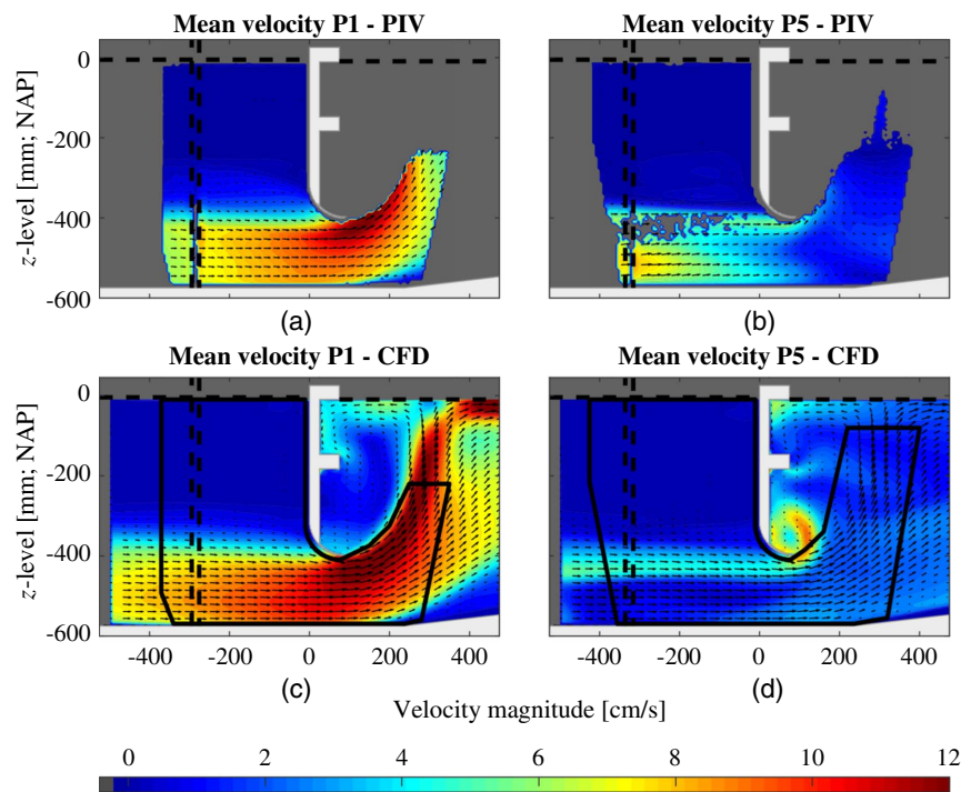
Fig. 10. Flow patterns for test 300F as measured by (a and b) PIV and (c and d) simulated for the plane at the northside of the screen (P1–a and c) and for the plane at the southside of the screen (P5–b and d). In the mixing zone, no measurements could be obtained with PIV. The dashed lines represent the water surface and the extend of the curved northern and southern sidewalls. The solid line (c and d) show the outline of the PIV measurements.
