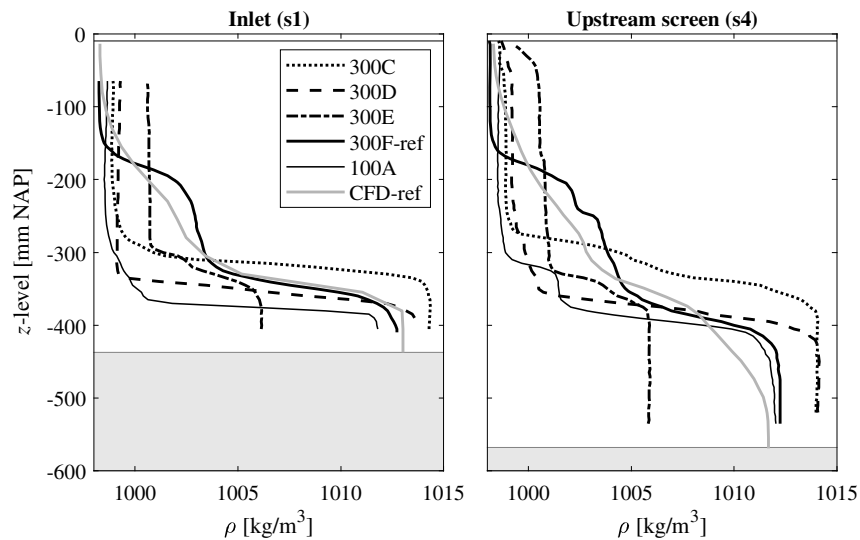
Fig. 12. Stationary vertical density profiles at the inlet (s1) and at the screen (s4) for each test condition. CFD-ref corresponds to test 300F-ref.
