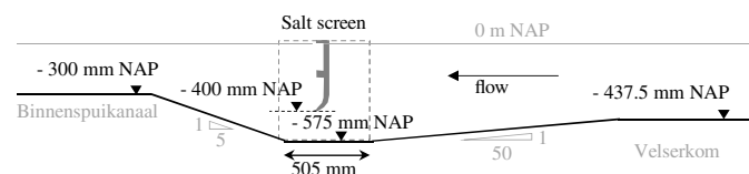
Fig. 4. Schematic representation of the floor levels along the axis of the salt screen; screen represented by solid shape and pillars by dashed rectangle.
