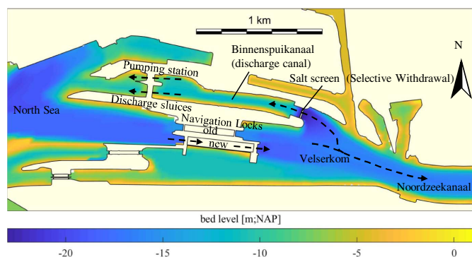
Fig. 1. Map of the IJmuiden Locks and Discharge Complex with the location of the salt screen. The salt water from the North Sea enters the Velserkom through the locks. By means of selective withdrawal, the additional salt in the Velserkom will be discharged back to the North Sea through the discharge canal, sluices, and pumping station north of the locks. The dashed lines show the transit of the saltwater.
