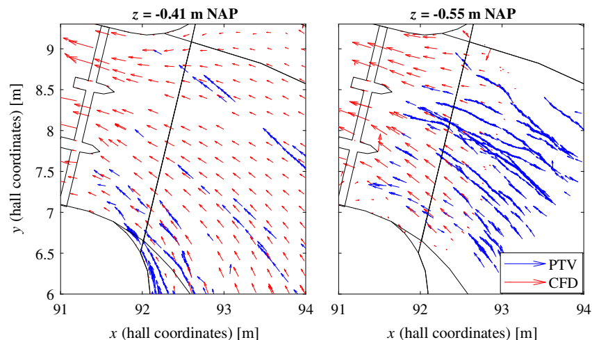
Fig. 11. Flow patterns for test 300F as measured by 3D-PTV and simulated for a horizontal plane immediately below the screen ( -0.41 m NAP) and just above the bottom ( -0.55 m NAP).
