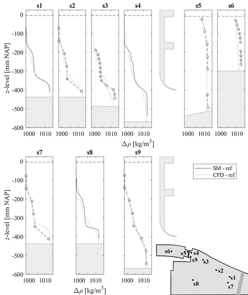
Fig. 13. Measured and modeled density profiles in the model. The dotted lines with markers indicate the fixed measurement points and the solid lines represent densities obtained from the moving conductivity gauges in test 300F.
