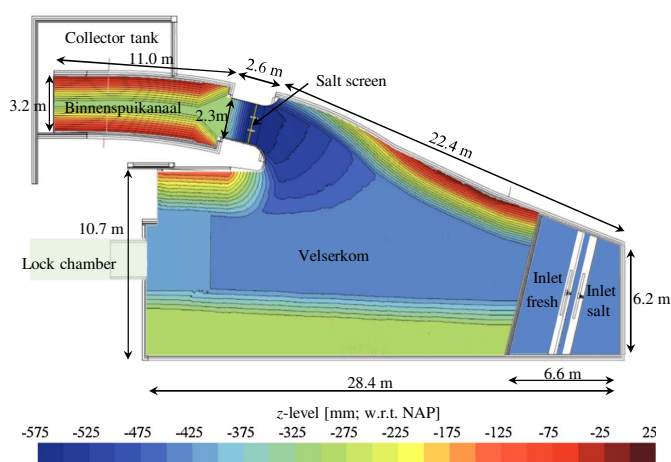
Fig. 3. Overview of the physical scale model with main dimensions including bathymetry in model scale (relative to Amsterdam Ordnance Datum–NAP on model scale).
