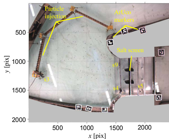
Fig. 7. Image of camera 1 used for 3D-PTV measurement. The tracer particles and the 8 ArUco markers are visible at the white floor of the scale model. The three particle dispensers are located in the upper left corner of the photo. The measurement stations s3–s5 and s9 are visible in the photo (see Fig. 5).
