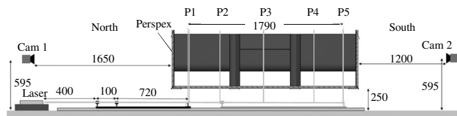
Fig. 6. Schematic sideview of the PIV setup with the measurement planes P1 to P5. The laser is positioned at the hall floor below the Perspex box with the salt screen. The laser beam is directed by means of lenses and mirrors to the correct measurement plane. Camera 1 captures the measurement planes P1 to P3 and Camera 2 captures the measurement planes P4 and P5. All dimensions are in mm.
