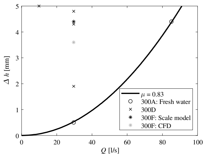
Fig. 14. Measured and modeled head differences at the salt screen for all test conditions. The solid line represents only freshwater tests (both tests gave a discharge coefficient of 0.83). The remaining dots depend on the density profiles as shown in Fig. 12.
