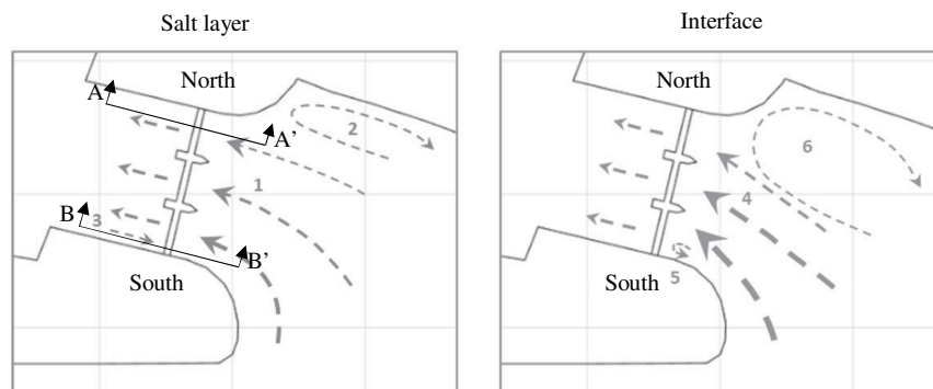
Fig. 8. Schematized flow patterns in the salt layer and at the interface, measured by means of PTV and dye injection.
