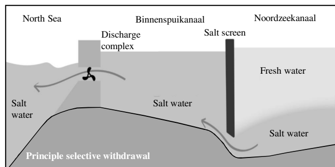
Fig. 2. Schematic representation of the salt screen at the entrance of the Binnenspuikanaal, allowing mainly salt water to flow to the discharge sluices and pumping station. (Reprinted with permission from Rijkswaterstaat.)
