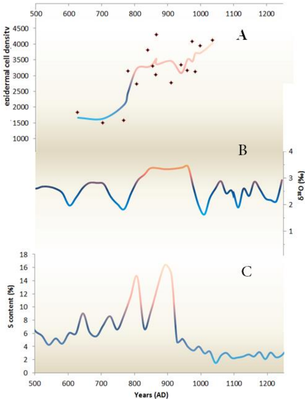
Fig. 9 : (A) Epidermal Cell Density record at the Maya Lowlands (Tabasco, Mexico), 3 pt run. Avg., showing a rapid increase at ~750 AD, indicating the start of a dryer period. Small interval occurs at around 920 AD, possibly showing variations in local precipitation and humidity levels at that time. (B) \delta^{18}\text{O} concentration from Lake Chichancanab (Yucatan, Mexico), 3 pt run. avg., indicating a drought episode between 800 and 900 AD. (C) Sulphur content in percentages from Lake Chichancanab, indicating drought between 750 and 925 AD, with a sudden decreasing episode at 830 AD.
