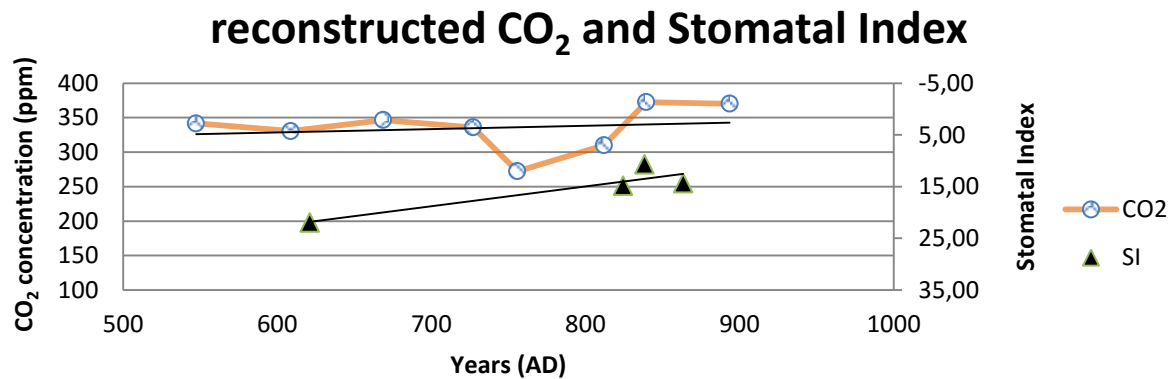
Fig. 7: Comparison of CO 2 reconstruction by Rundgren and Beerling (1999) based on Salix herbacea , with the mean stomatal index of Type 3 species from the Maya Lowlands. Age model is based on radiocarbon dating at both sites and OSL dating at the Maya Lowlands. Note that there is a negative correlation between CO 2 concentrations and SI, therefore the SI axis is reversed.
