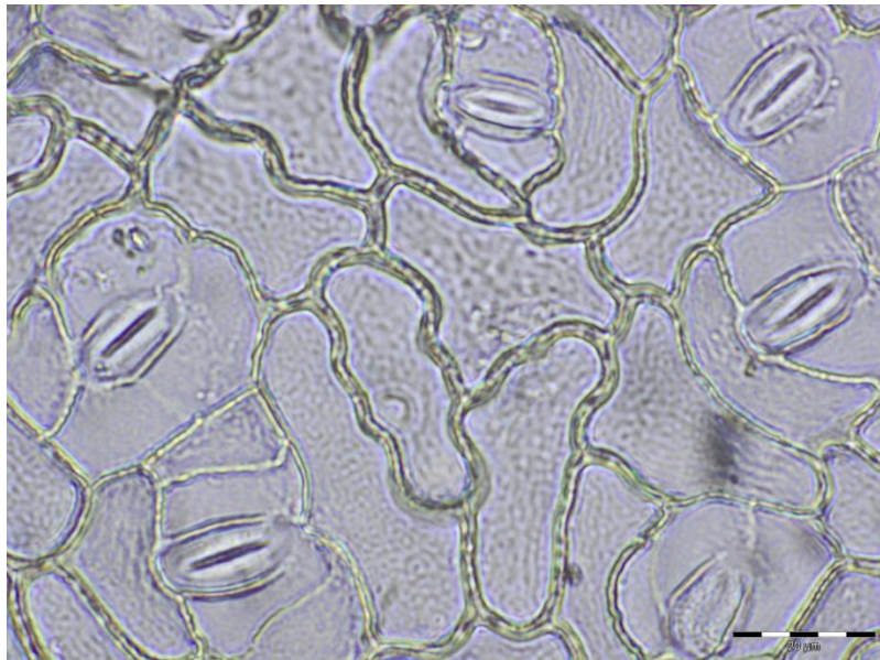
Fig. : Sample 193 171 SP 7 A, (age 767 AD) Type 2, indet. Possibly Fabaceae. Scale bar represents 20 \mu\text{m} .
