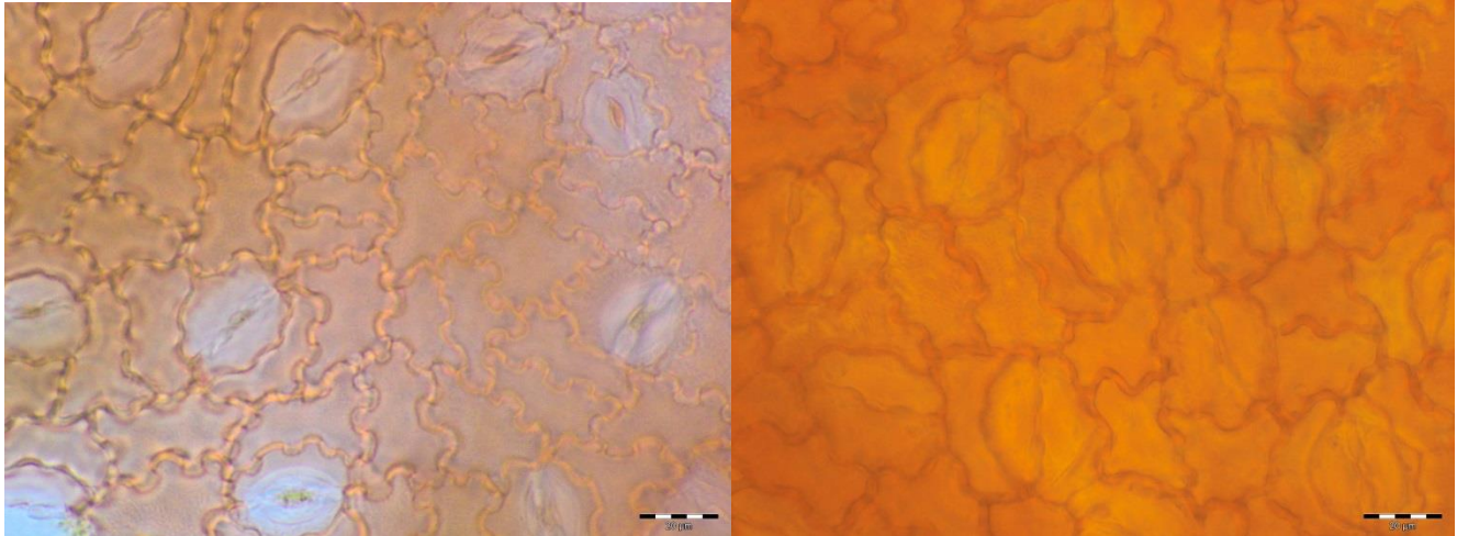
Fig. : (Left) Sample 426 255 I, (age 621 AD) Type 3. (Right) Sample 181 225 II, (age 864 AD) Type 3. Scale bar represents 20 \mu\text{m} .
