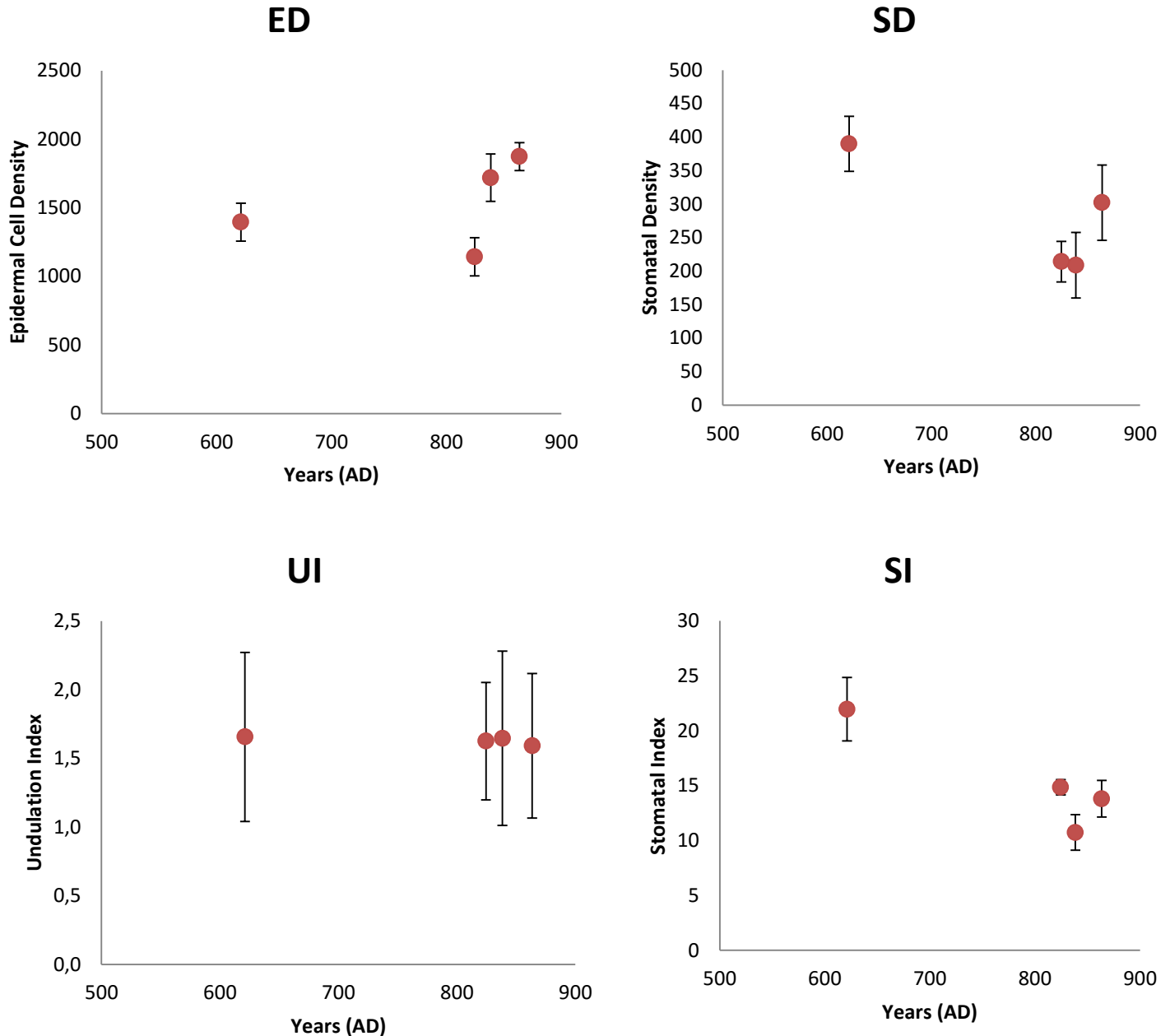
Fig. 5 : All results are plotted over time, using radiocarbon and OSL derived dates. (Upper left corner) Mean Epidermal Cell Density of Type 3. (Upper right corner) Mean Stomatal Cell Density of Type 3. (Lower left corner) Undulation Index of Type 3. (Lower right corner) Mean Stomatal Index of Type 3.
