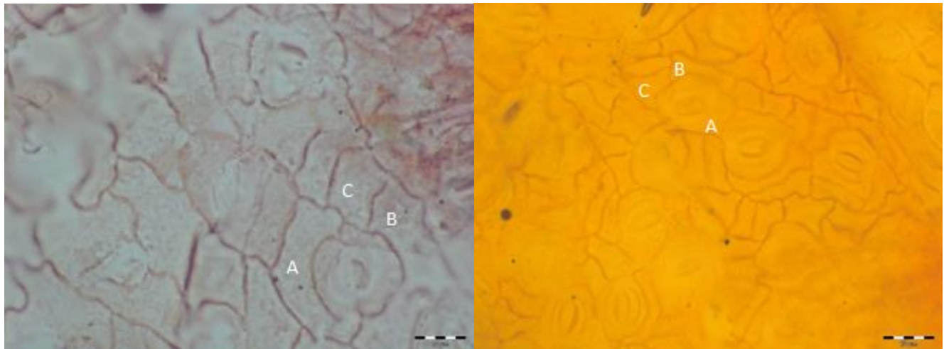
Fig. 4 : (Left) Sample 397 160 + 180 I, (age 694 AD) Type 1, Fabaceae, (Right) Sample 380- 155 I, (age 850 AD) Type 1, Fabaceae. Scale bar represents 20 \mu m.
