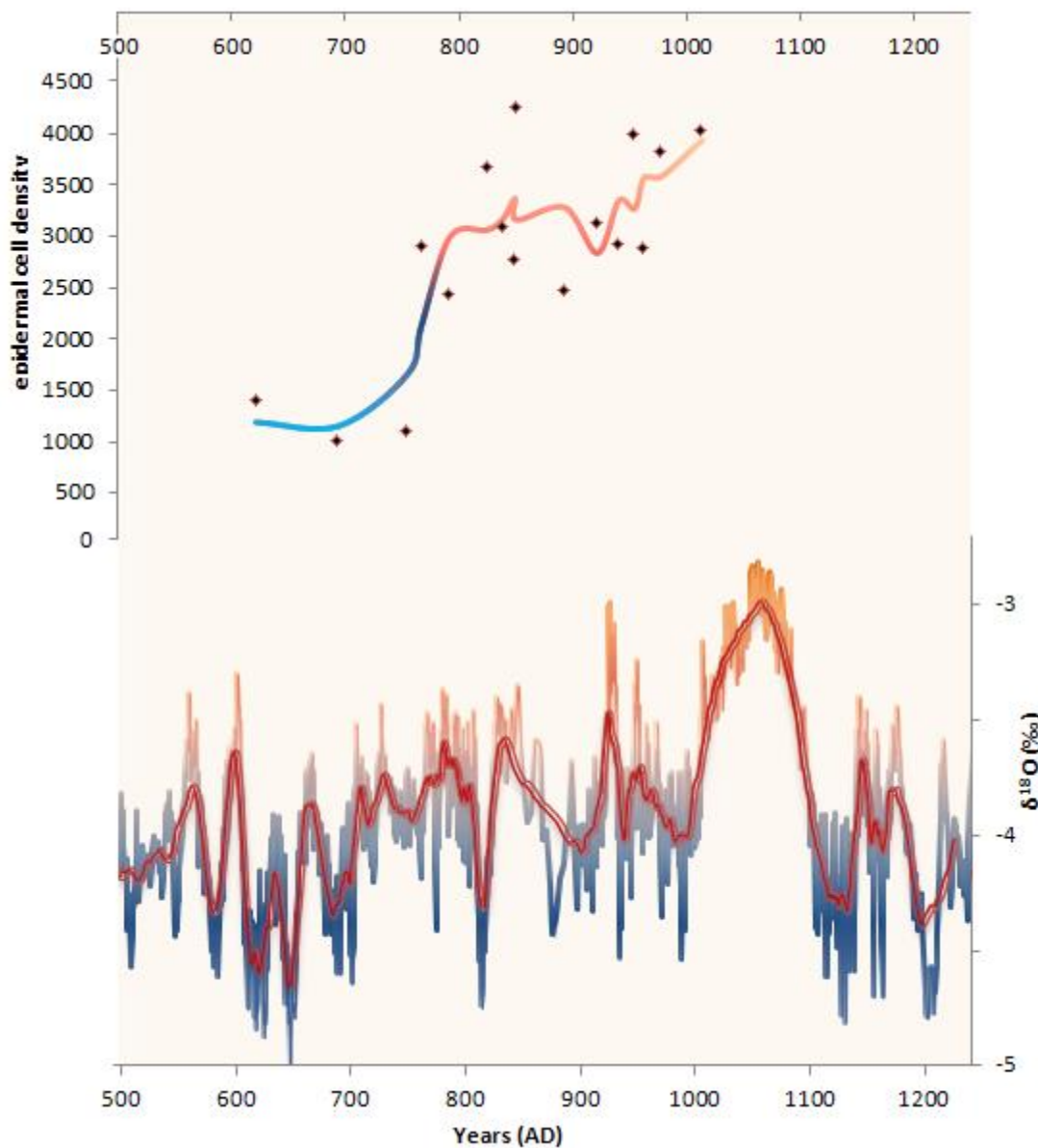
Fig. 8 : (Top) Epidermal Cell Density record at the Maya Lowlands (Tabasco, Mexico). 3 pt run. Avg., results show fluctuation in precipitation after the start of the drought episode. (Bottom) Speleothem \delta^{18}\text{O} records from Yok Ballum Cave (Belize), 31 pt run. Avg., indicating multiple drought episodes during the TCP.
