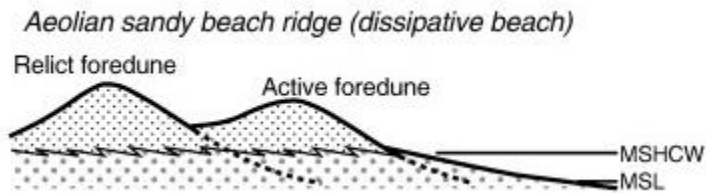
Fig. 2 : Schematic illustration showing the proposed formation of an aeolian sandy beach ridge. When coring in the ridges, samples from an older ridge can be obtained in the core due to the deposition of the younger ridge (Tamura T., 2012).
