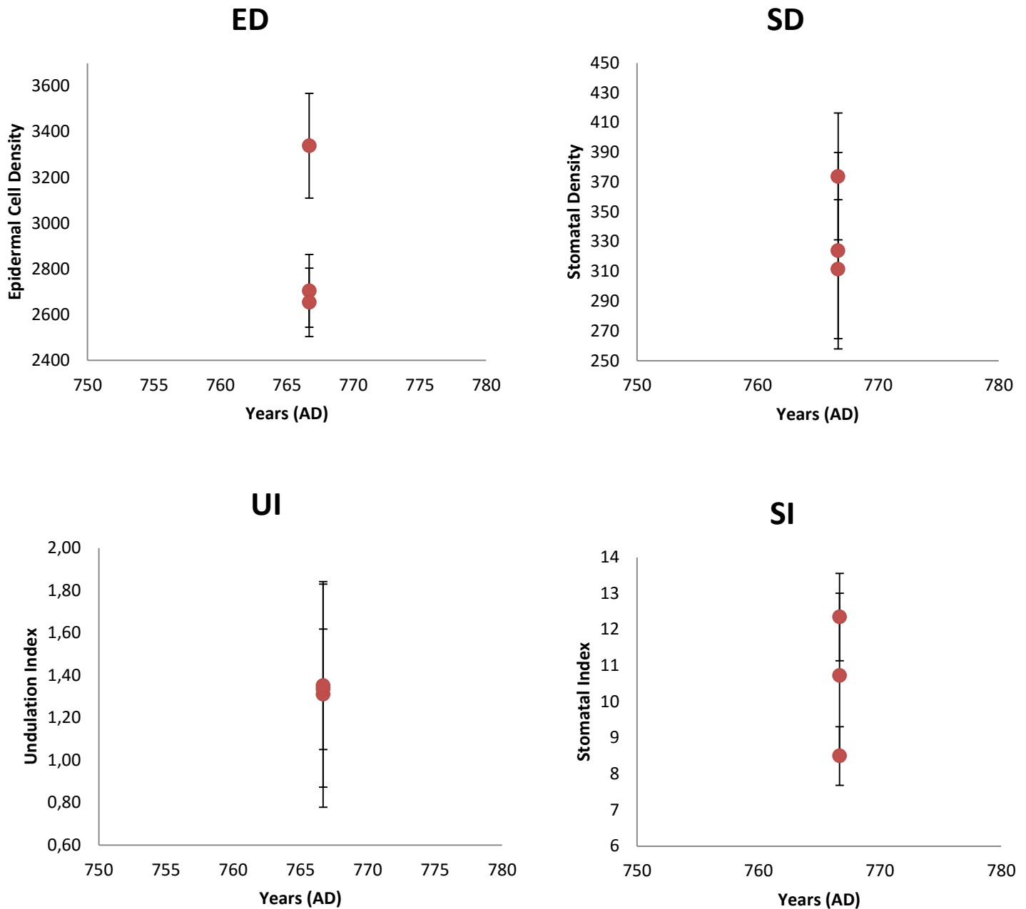
Fig. 5 : All results are plotted over time, using radiocarbon and OSL derived dates. (Upper left corner) Mean Epidermal Cell Density of Type 2. (Upper right corner) Mean Stomatal Cell Density of Type 2. (Lower left corner) Undulation Index of Type 2. (Lower right corner) Mean Stomatal Index of Type 2.
