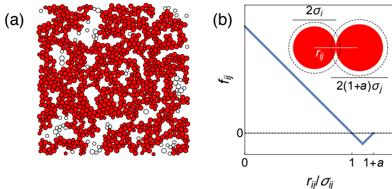
Figure 3.1: (left) A periodic packing of sticky disks at \phi \approx \phi_c . Red disks participate in the spanning rigid cluster. (right) Their force law. The dimensionless parameter a sets the range and strength of the attractive interaction; a = 0.1 at left.
