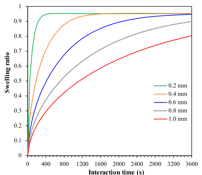
Figure 13. Swelling ratios of rubber particles of different sizes over the course of time.
