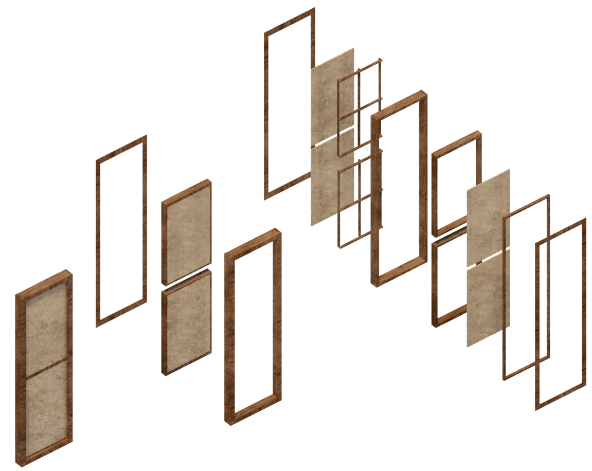
FACADE ELEMENT
