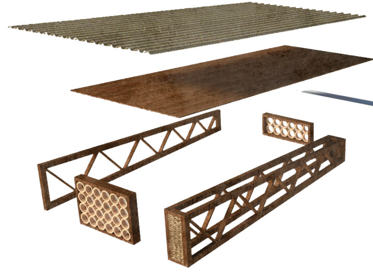
ROOF ELEMENT
