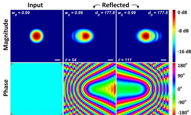
Figure A19. Magnitude and phase at the detector plane. (Left column) an ideal TEM 0,0 Gaussian beam waist is placed at the input plane. (Middle) the reflected beam magnitude and phase sampled at the input plane after routing through OAP mirrors A and B, reflection from the spherical target and then back through OAP A and B. The scan mirror directs the beam centroid at an angle of \theta = 54^\circ w.r.t. the z-axis and the OAP mirror tip separation is d_0 = 177.8 mm. (Right) same as middle except \theta = 111^\circ .
