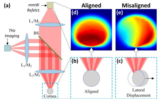
Figure 1. Alignment concept. (a) A quasi-optical diplexer (e.g. wire grid polarizer) multiplexes the THz and mmW beams on a common optical axis. When the cornea is positioned correctly with respect to the aperture in (b) the THz image shows the contrast in (d). When the cornea is misaligned (c) there is a significant change in imaging contrast (e) arising from the rapid degradation in coupling.
