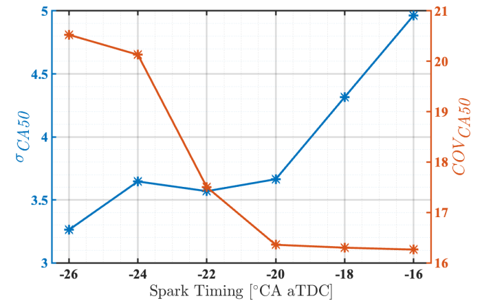
FIGURE 15: IMPACT OF ST DELAY ON COV AND \sigma OF CA50
