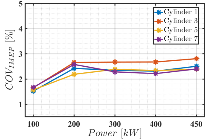
FIGURE 5: COV IMEP FOR ACROSS ALL LOAD POINTS AND CYLINDERS
