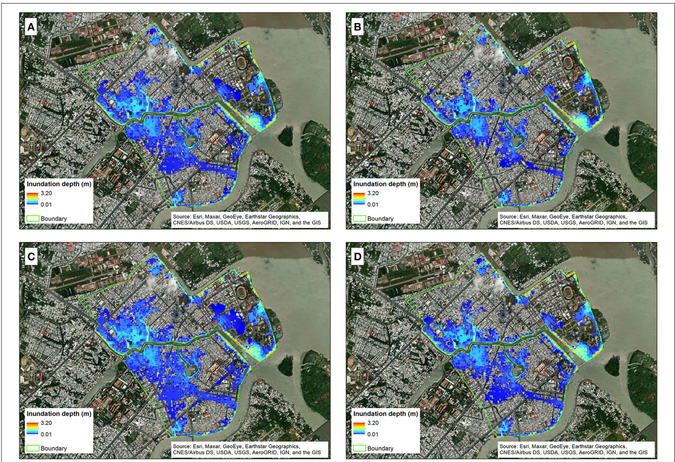
FIGURE 10 | Flood hazard maps (i.e., maximum flood depths) for the 100-year return period of water level for hydrograph shape Pattern 1 (left) and Pattern 2 (right) under RCP 4.5 (A,B) and RCP 8.5 (C,D) (without land subsidence). The inundated area (for cells with maximum inundation depths \geq 0.02 m) for RCP 4.5 and RCP 8.5 corresponding to Pattern 1 are 1.96 and 2.30 km 2 , respectively, while for Pattern 2 are 1.41 and 1.81 km 2 , respectively.
