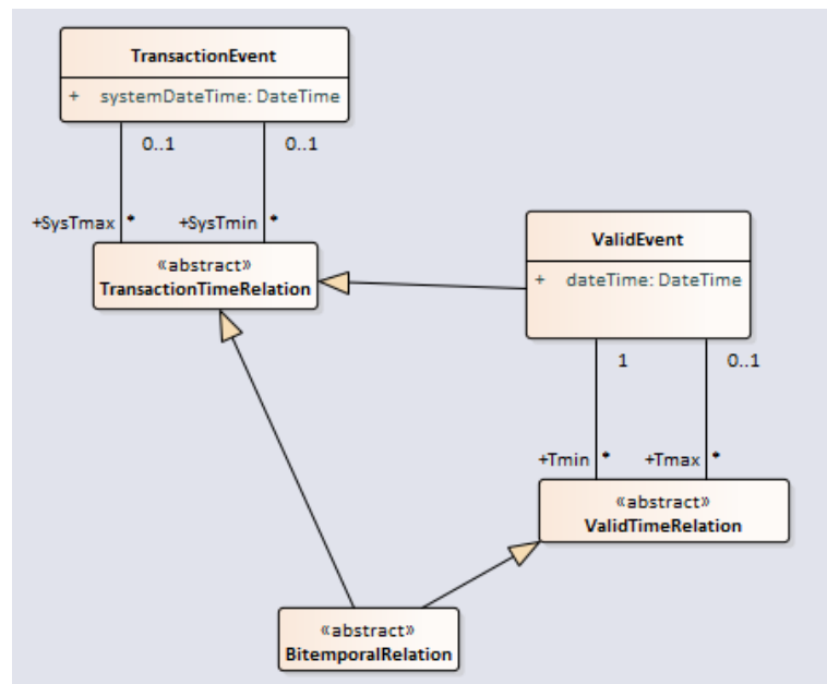
Figure 5 Bi-Temporal concepts.
