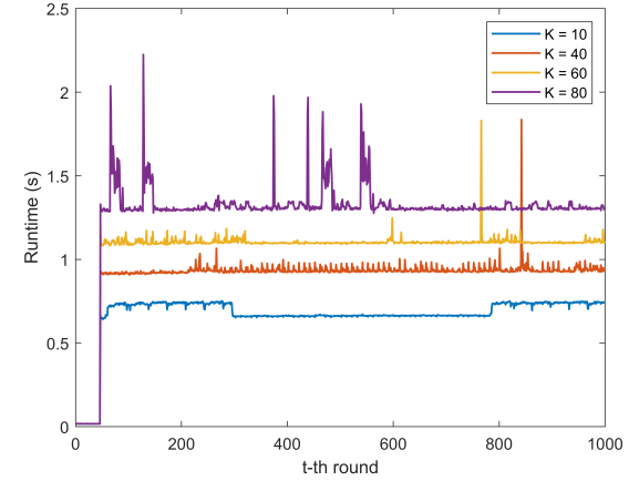
Fig. 11: Runtime with t -th round
