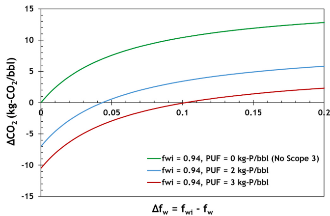
Fig. 6. Impact of polymer utilization factor on extent of CO 2 intensity reduction.
