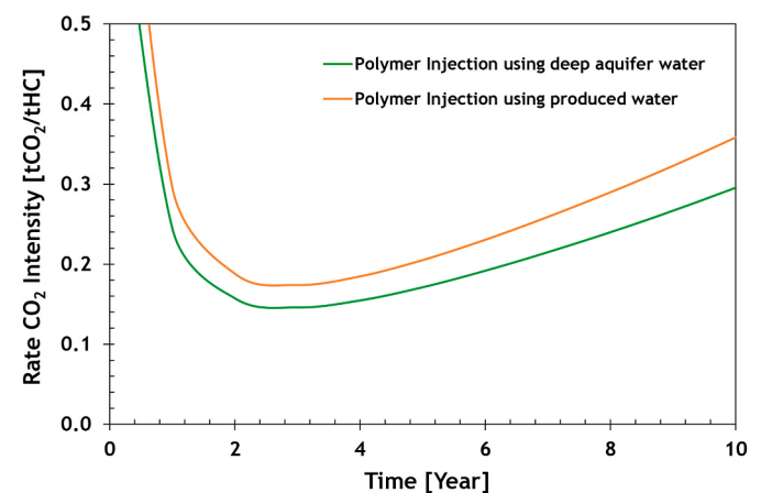
Fig. 11. Comparison of CO 2 intensity for polymer flooding using two sources of water: deep aquifer and produced water.
