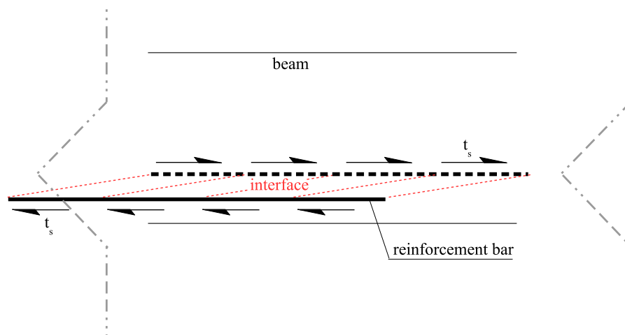
Fig. 23 illustration of the use of truss element to model reinforcement bar
