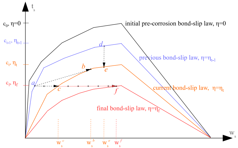
Fig. 3 Transition between bond-slip laws with increasing corrosion: a \rightarrow b increase of both load and corrosion, a \rightarrow c and a \rightarrow f increasing corrosion under constant load, d \rightarrow e increasing corrosion under constant slip displacement
