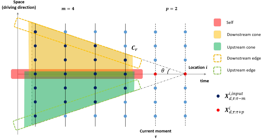
Figure 3.1: Illustration of localized spatial correlation: an example of input-output pairs. The dash-dot line triangle is the spreading cone; Sub-areas are marked by different colors.
