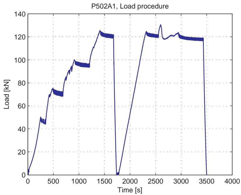
Fig. 5.80.4. Load-Time curve
