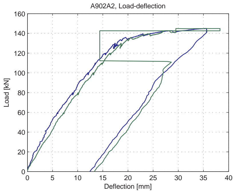
Fig. 5.18.4. Load-deflection curve
