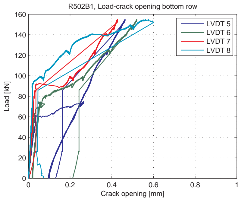
Fig. 5.99.8. Load-Crack opening for LVDT's 5-8 (bottom row)
