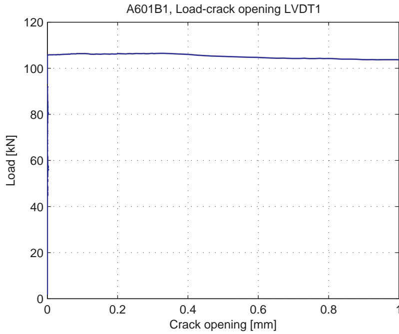
Fig. 5.33.5. Load-Crack opening for LVDT1
