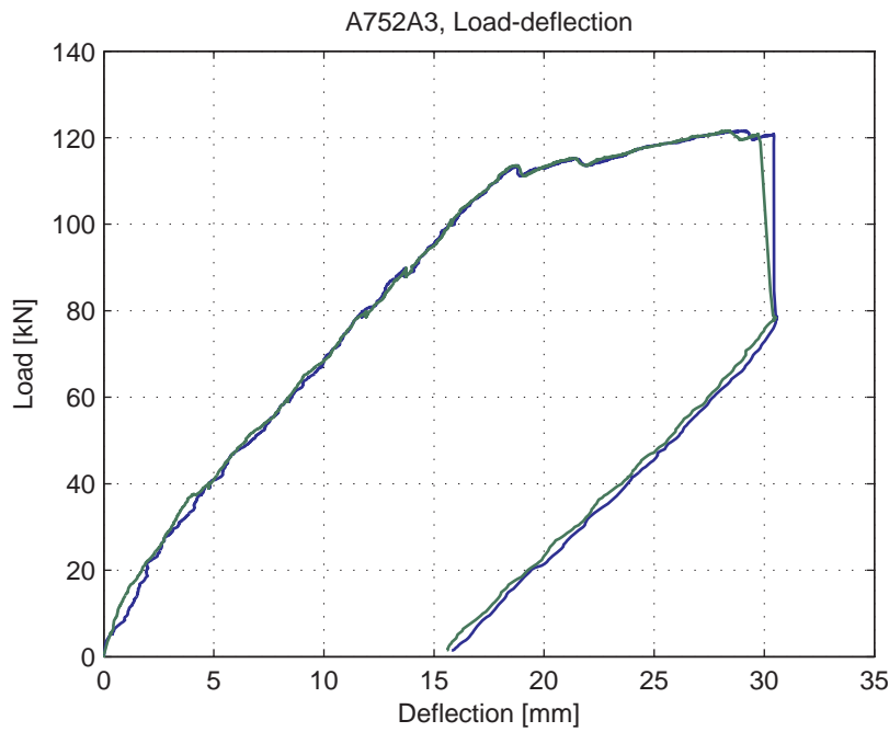
Fig. 5.28.4. Load-deflection curve
