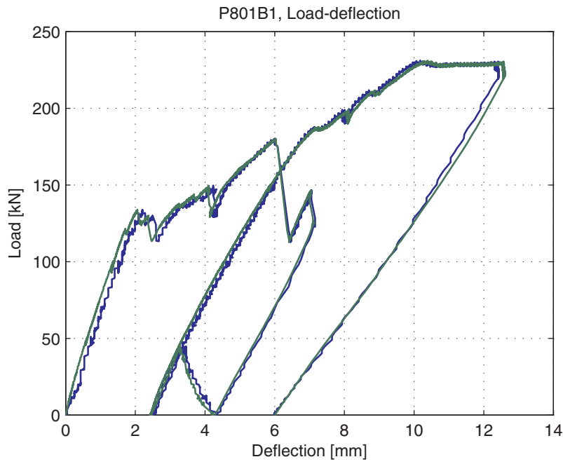
Fig. 5.86.6. Load-deflection curve
