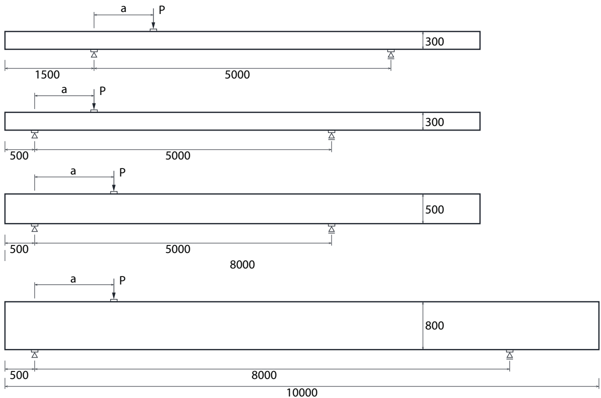
Fig. 3.1.1. Configurations of the boundary conditions of the tests.
