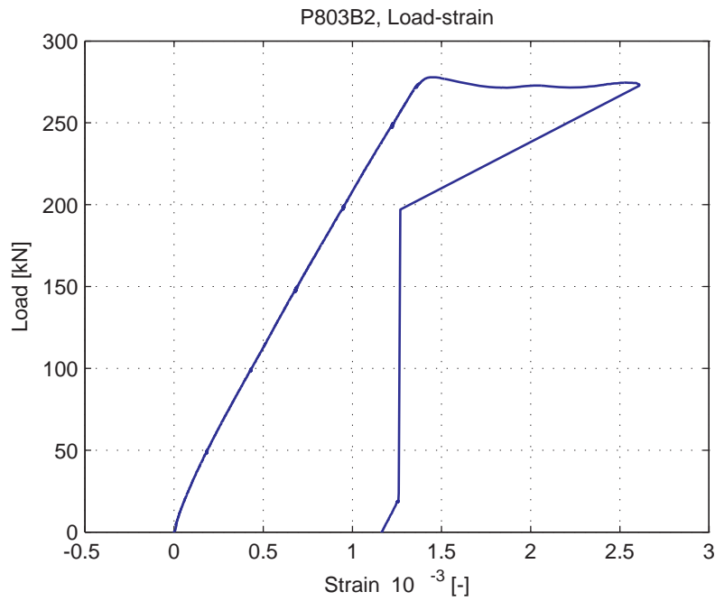
Fig. 5.91.11. Average strain over 1m length, measured at bottom of specimen (LVDT 14)
