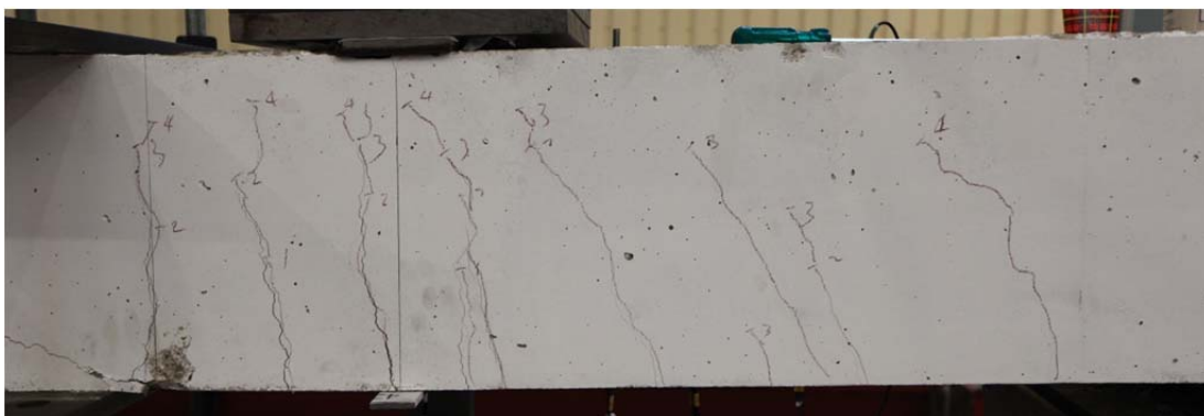
Fig. 5.69.2. Crack pattern after failure south side
