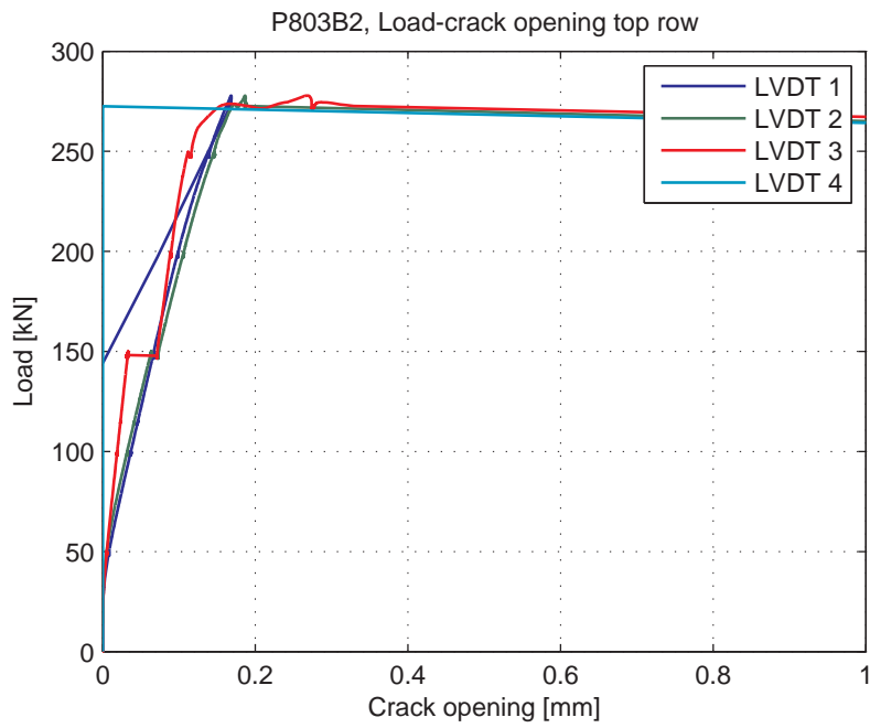
Fig. 5.91.6. Load-Crack opening for LVDT's 1-4 (top row)
