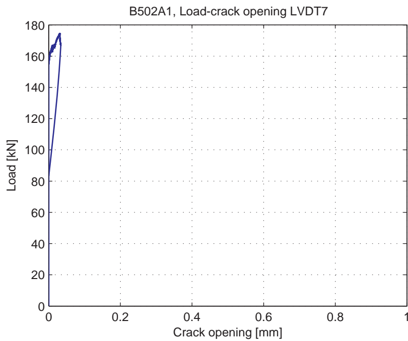
Fig. 5.50.8. Load-Crack opening for LVDT7
