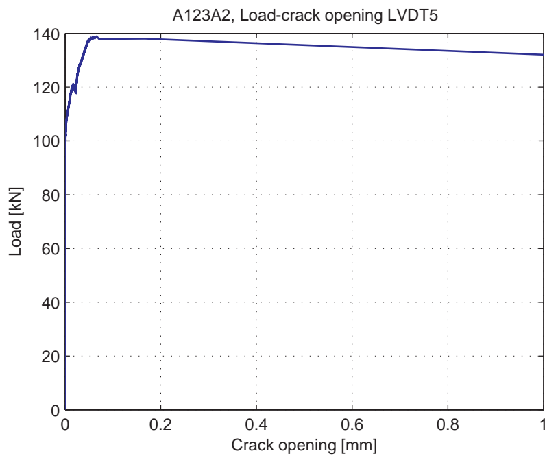
Fig. 5.9.6. Load-Crack opening for LVDT5
