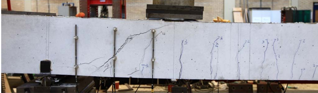
Fig. 5.39.1. Crack pattern after failure north side
