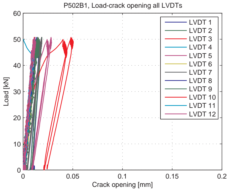
Fig. 5.82.10. Load-Crack opening first part of test for all LVDT's
