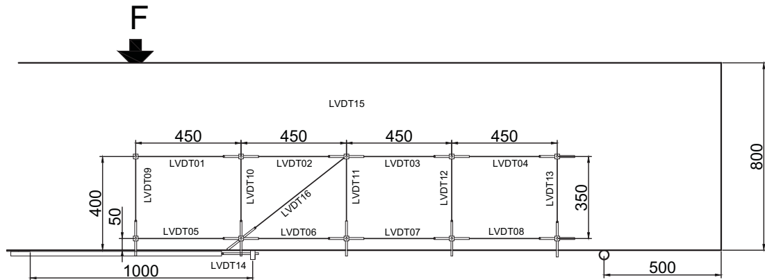
Fig. 5.90.3. LVDT layout and numbering for 800 mm deep beams
