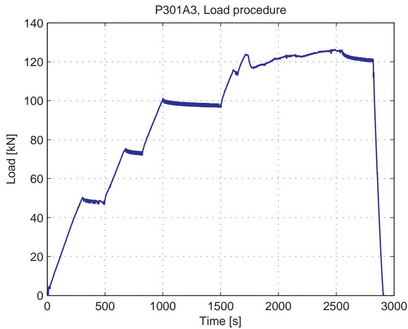
Fig. 5.73.4. Load-Time curve
