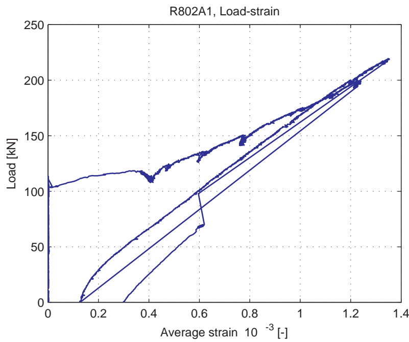
Fig. 5.102.10. Average strain over 1m length, measured at bottom of specimen (LVDT 14)
