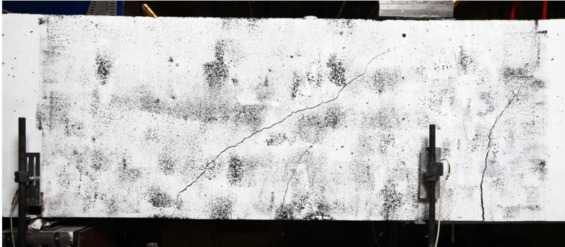
Fig. 5.85.1. Crack pattern after failure north side
