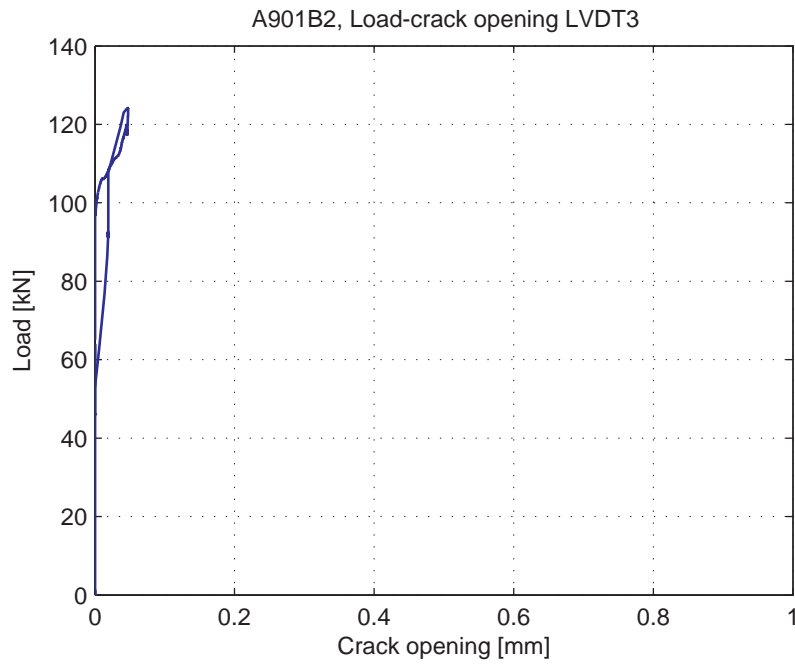
Fig. 5.16.7. Load-Crack opening for LVDT3
