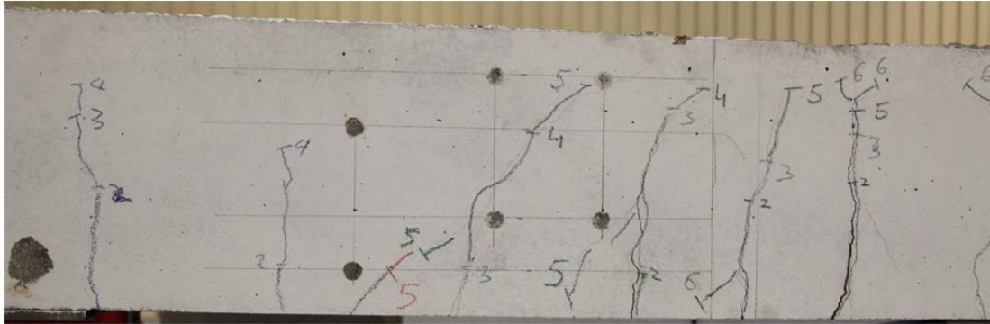
Fig. 5.36.1. Crack pattern after failure north side. (Picture taken after test A602A3.)
