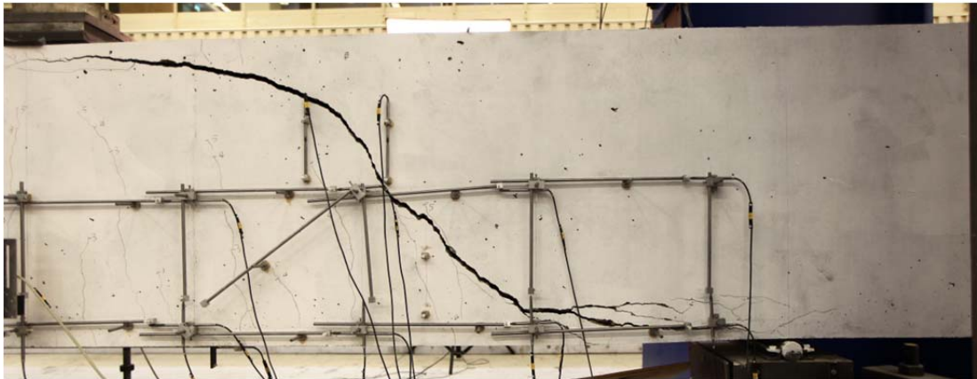
Fig. 5.89.2. Crack pattern after failure south side
