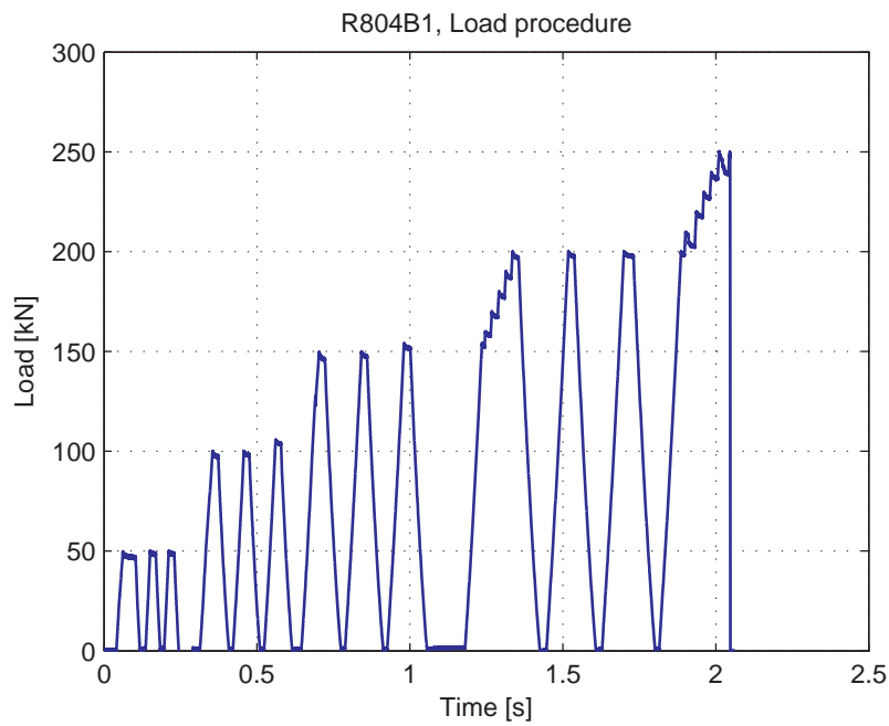
Fig. 5.107.4. Load-Time curve
