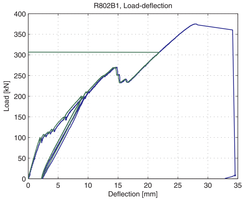
Fig. 5.103.5. Load-deflection curve
