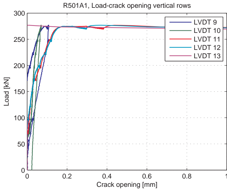
Fig. 5.95.7. Load-Crack opening for LVDT's 9-13 (vertical LVDT's)
