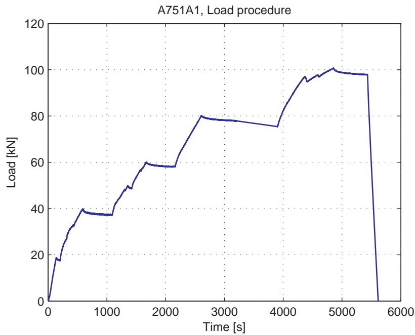
Fig. 5.22.3. Load-Time curve
