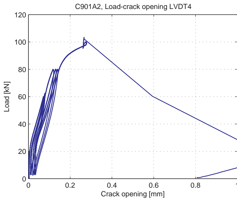
Fig. 5.55.5. Load-Crack opening for LVDT4
