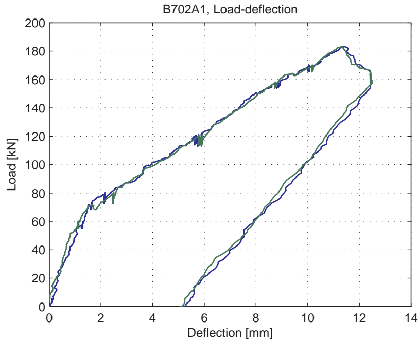
Fig. 5.45.4. Load-deflection curve
