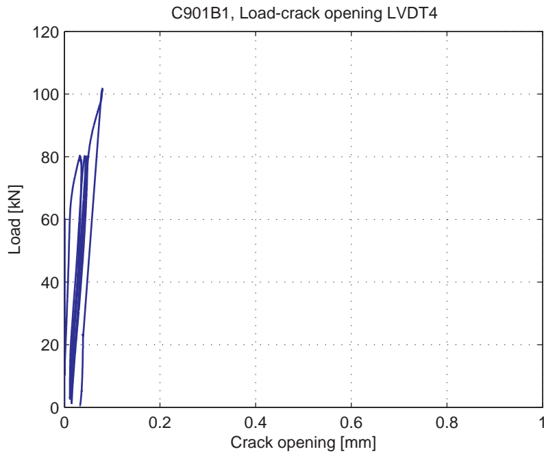
Fig. 5.57.7. Load-Crack opening for LVDT4
