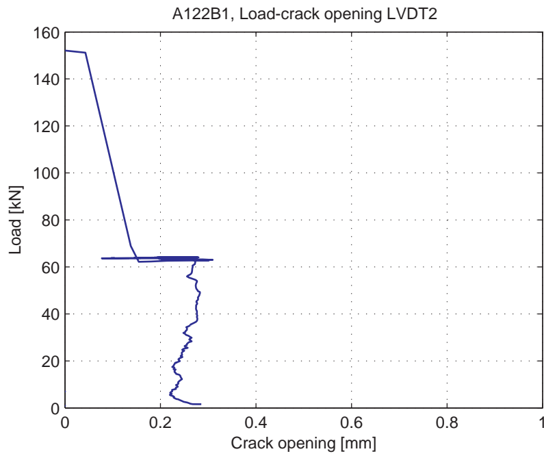
Fig. 5.6.6. Load-Crack opening for LVDT2
