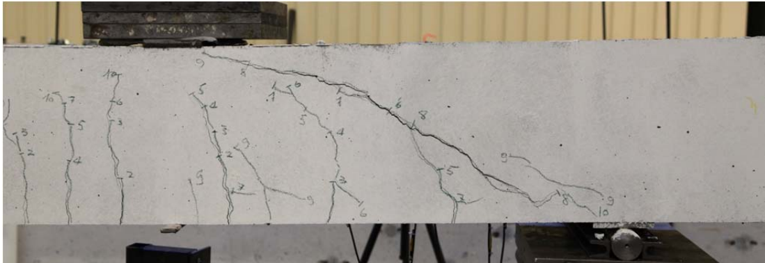
Fig. 5.5.2. Crack pattern after failure south side
