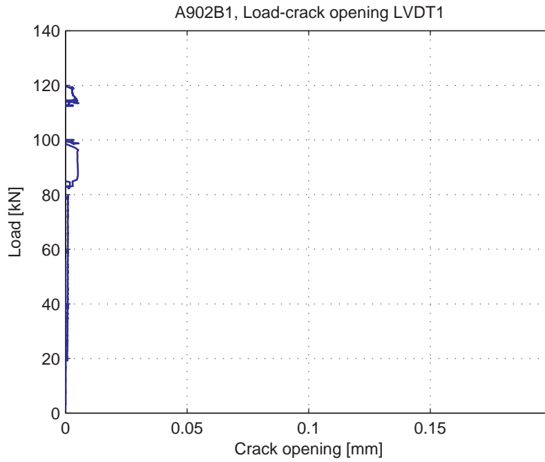
Fig. 5.20.5. Load-Crack opening for LVDT1
