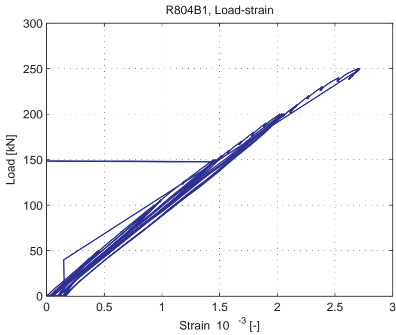
Fig. 5.107.9. Average strain over 1m length, measured at bottom of specimen (LVDT 14)
