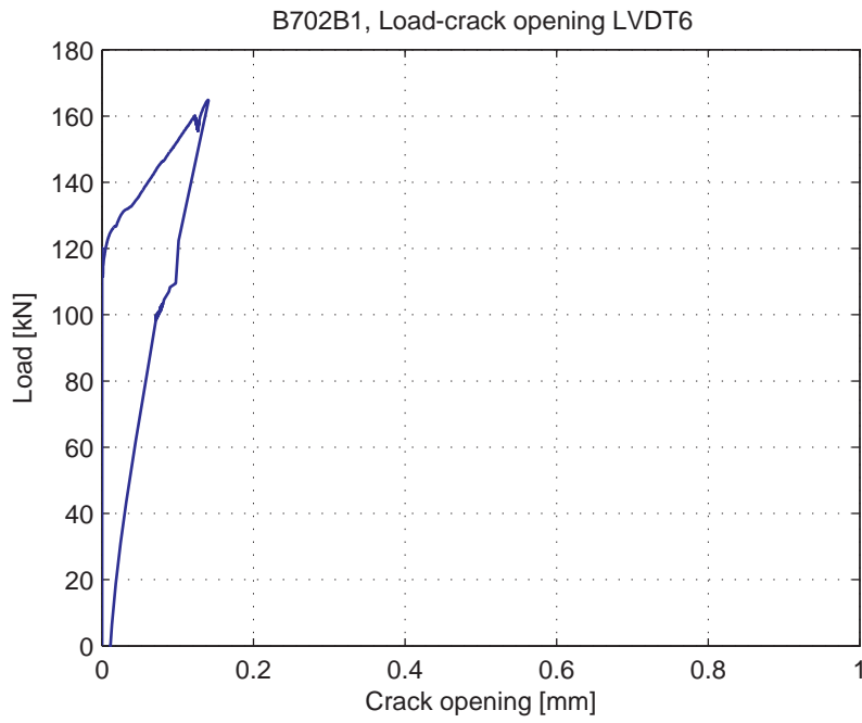
Fig. 5.46.7. Load-Crack opening for LVDT6
