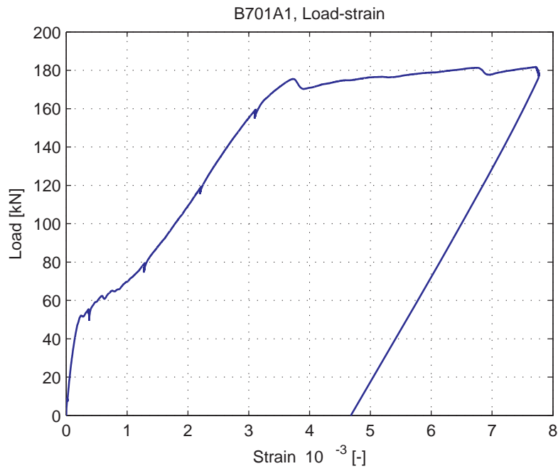
Fig. 5.40.5. Average strain over 1m length, measured at bottom of specimen (LVDT 3)
