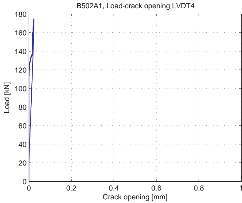
Fig. 5.50.5. Load-Crack opening for LVDT4
