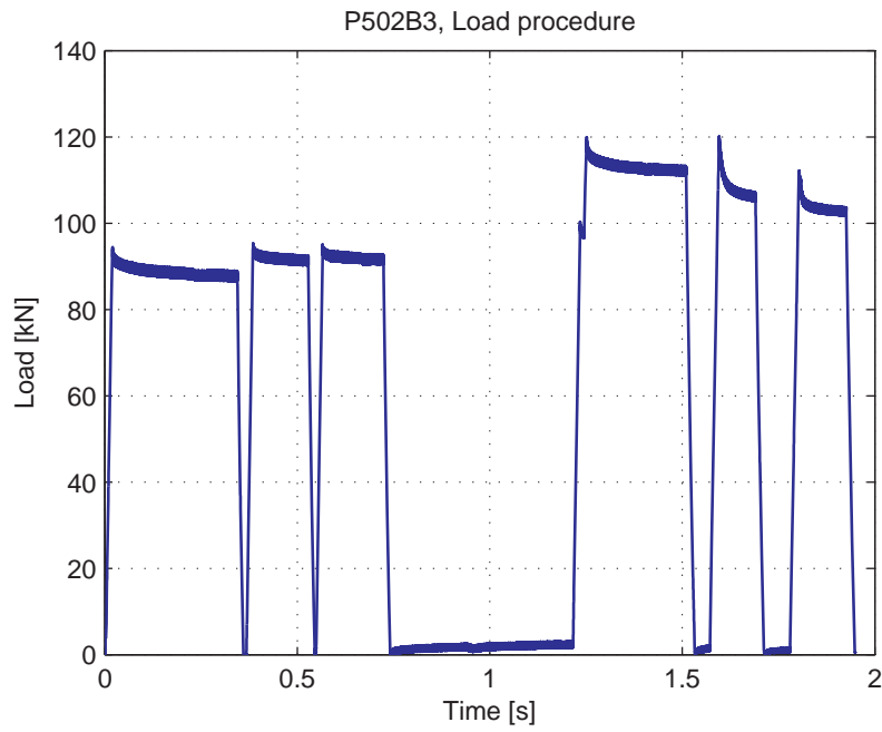
Fig. 5.82.6. Load-Time curve for third part of test
