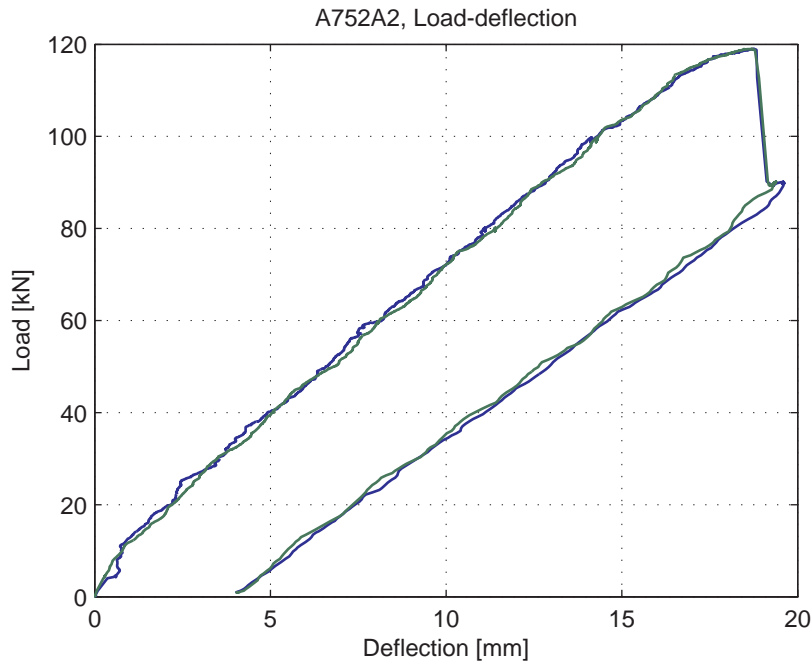
Fig. 5.27.4. Load-deflection curve
