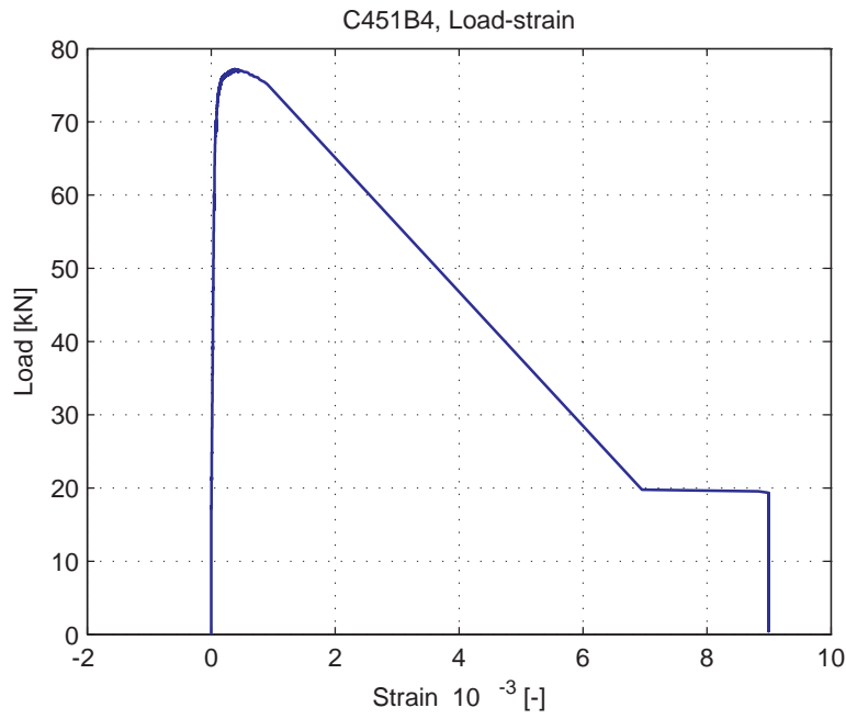
Fig. 5.70.9. Average strain over 1m length, measured at bottom of specimen (LVDT 3)
