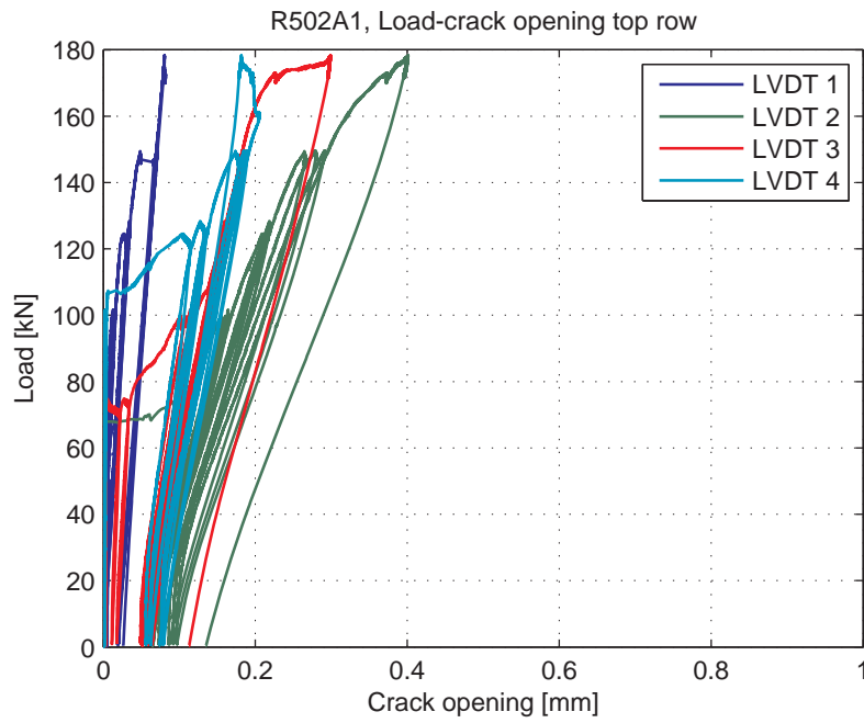
Fig. 5.97.6. Load-Crack opening for LVDT's 1-4 (top row)
