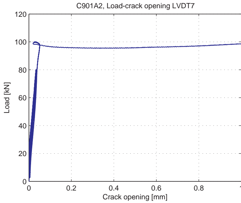
Fig. 5.55.8. Load-Crack opening for LVDT7
