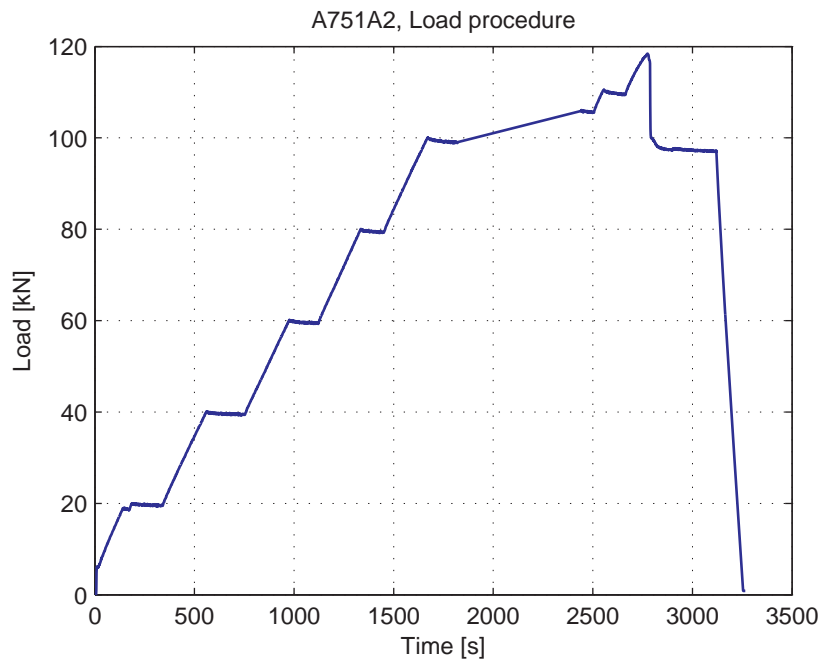
Fig. 5.23.3. Load-Time curve
