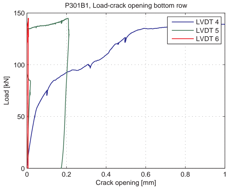
Fig. 5.75.8. Load-Crack opening for LVDT's 4-6 (bottom row)
