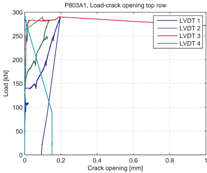
Fig. 5.89.6. Load-Crack opening for LVDT's 1-4 (top row)
