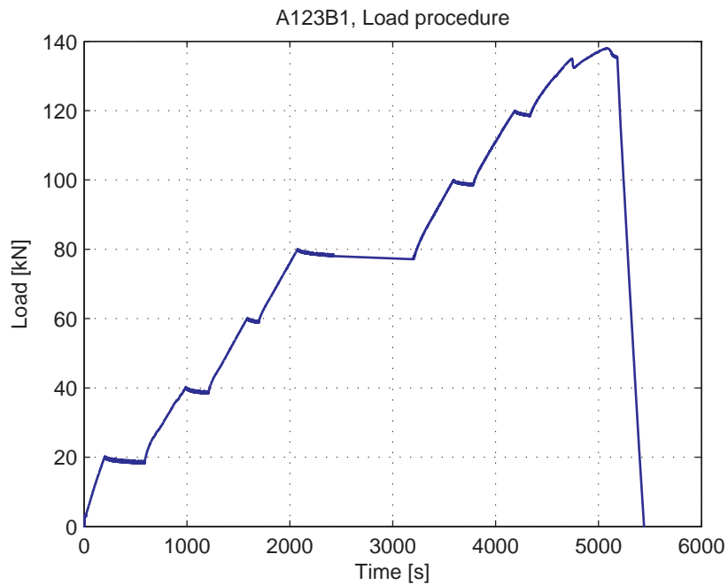
Fig. 5.10.3. Load-Time curve
