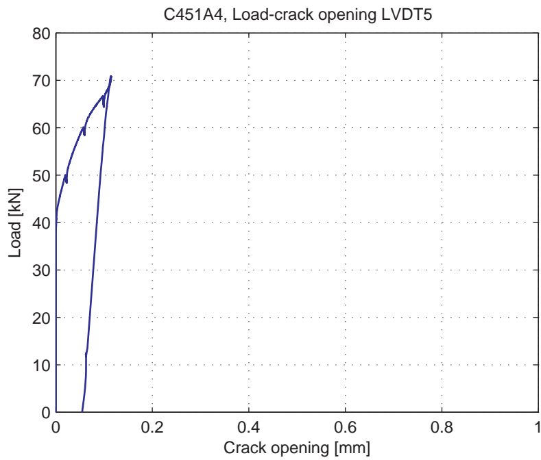
Fig. 5.65.6. Load-Crack opening for LVDT5
