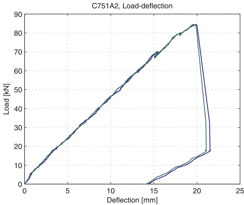
Fig. 5.59.4. Load-deflection curve
