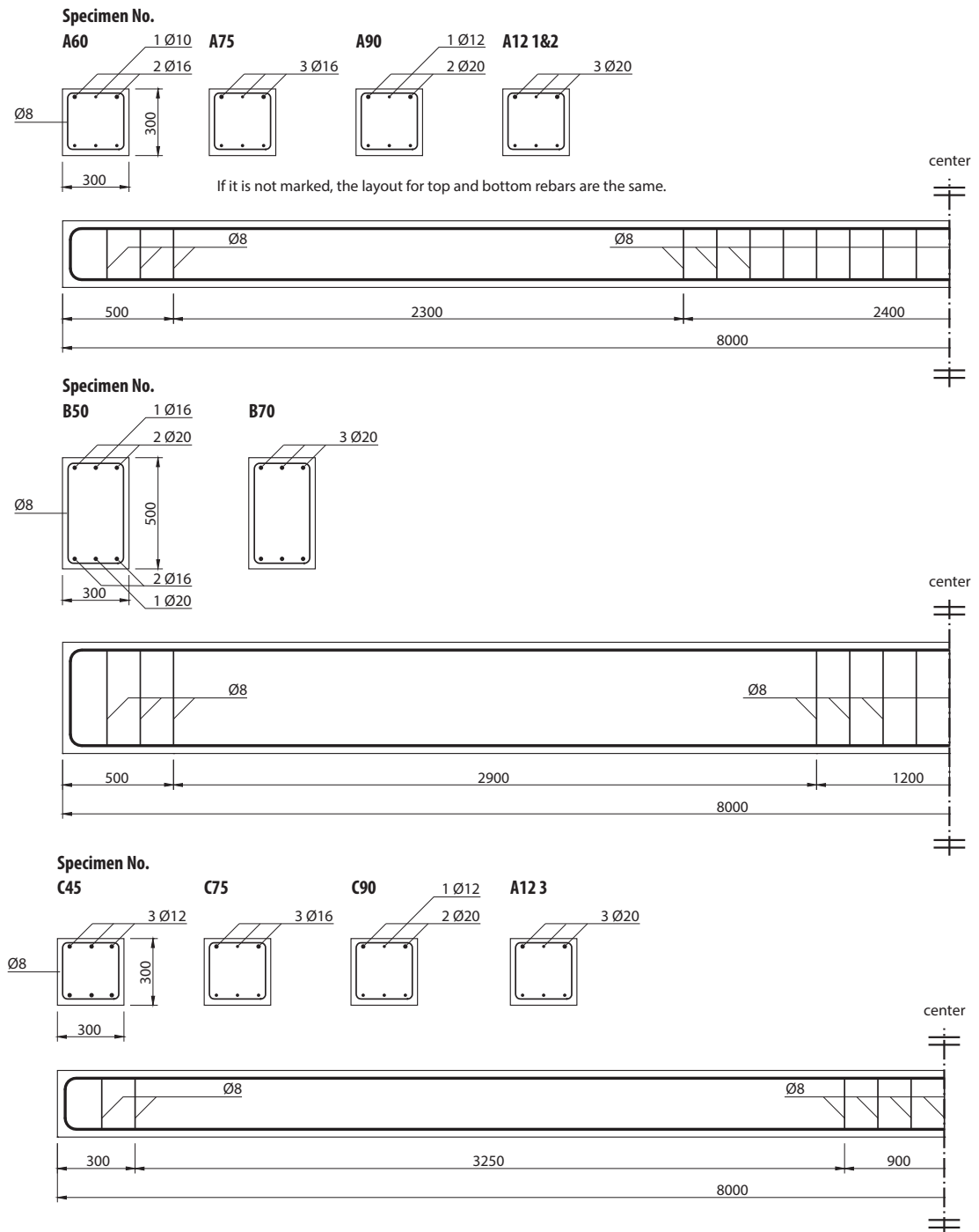
Fig. 2.3.1. Reinforcement layout for tested specimens in A, B and C series.
