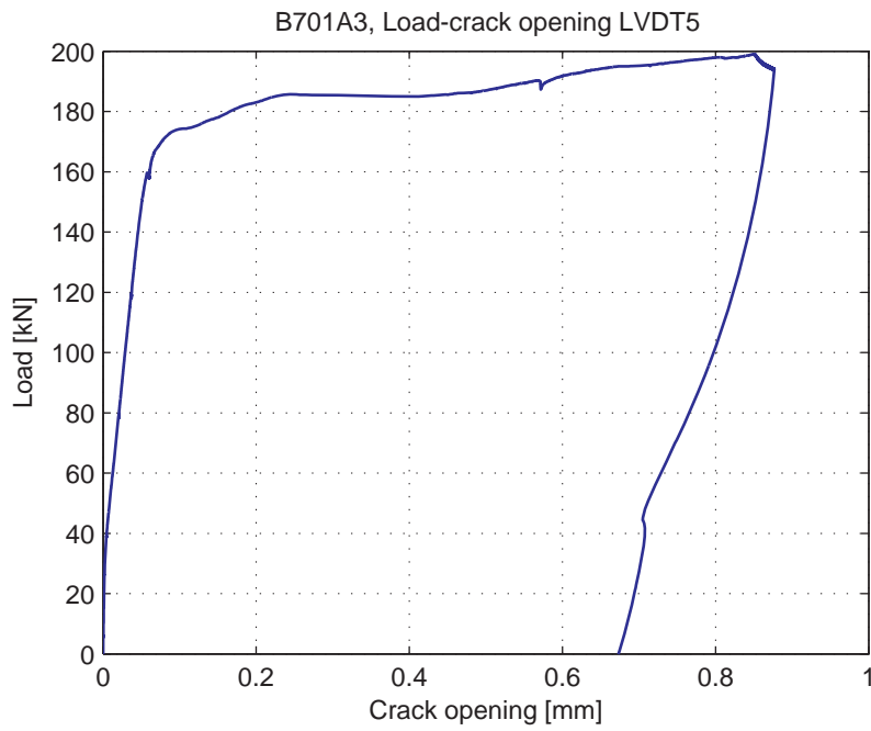
Fig. 5.42.6. Load-Crack opening for LVDT5
