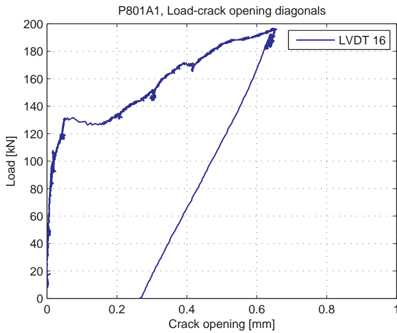
Fig. 5.83.8. Load-Crack opening for LVDT 16 (diagonal)
