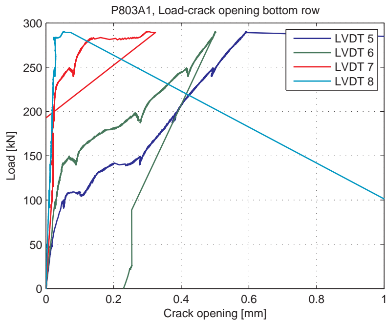
Fig. 5.89.8. Load-Crack opening for LVDT's 5-8 (bottom row)
