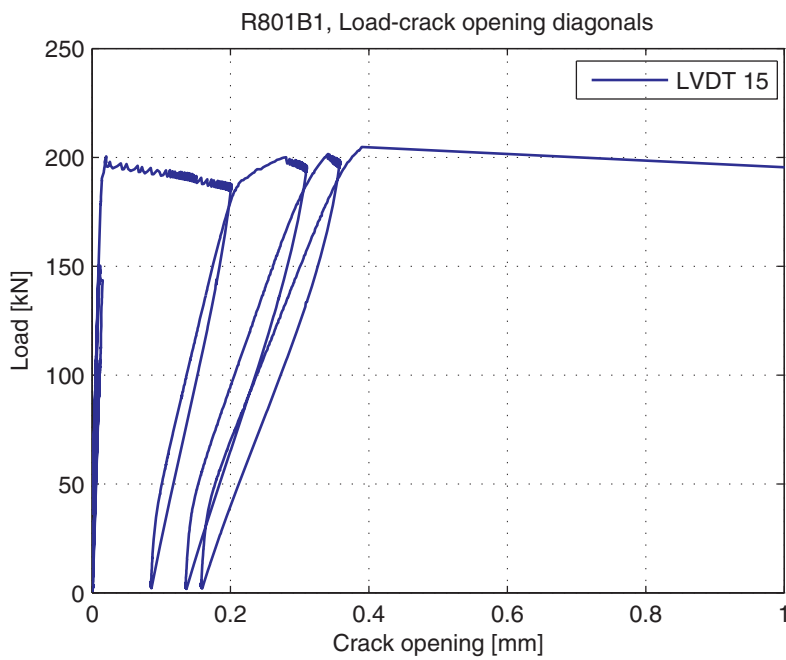
Fig. 5.101.9. Load-Crack opening for LVDT 16 (diagonal)
