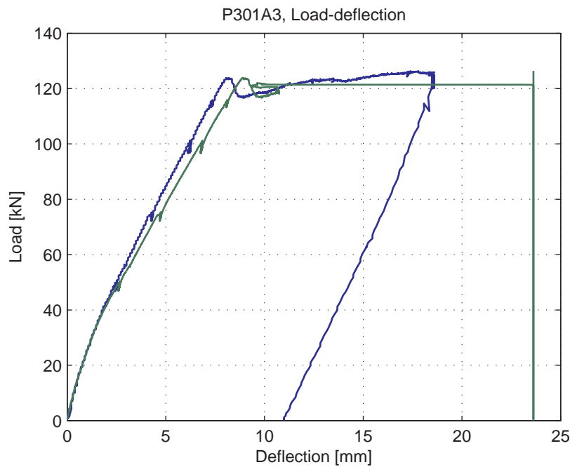
Fig. 5.73.5. Load-deflection curve
