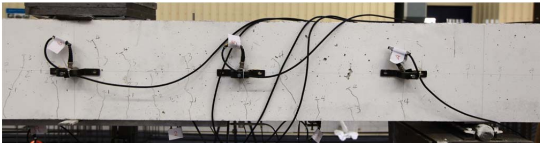
Fig. 5.57.3. Sensors used for Acoustic Emission measurements at side beam
