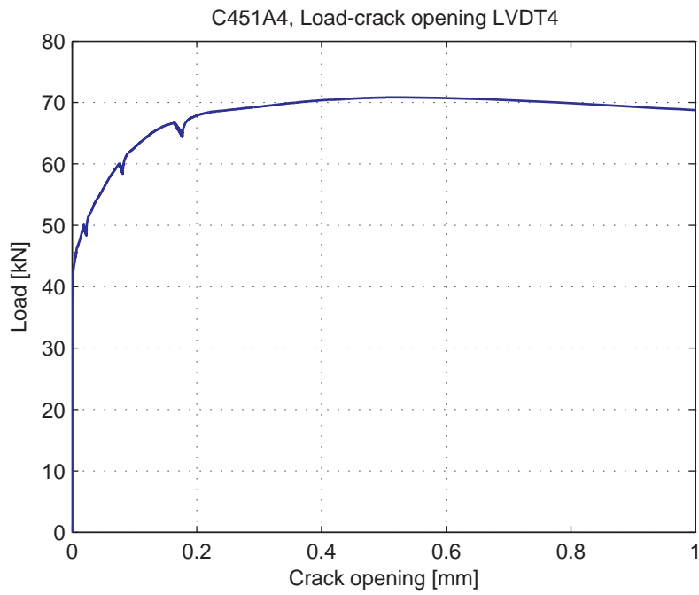
Fig. 5.65.5. Load-Crack opening for LVDT4
