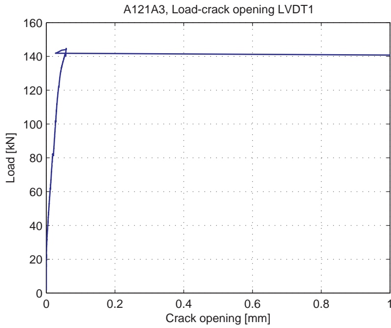
Fig. 5.3.5. Load-Crack opening for LVDT1
