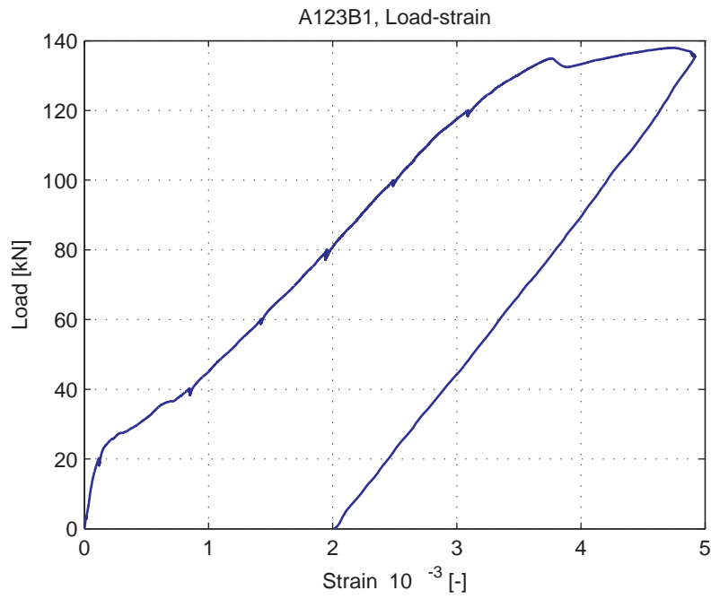
Fig. 5.10.8. Average strain over 1m length, measured at bottom of specimen (LVDT 3)
