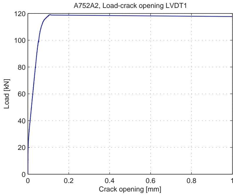
Fig. 5.27.5. Load-Crack opening for LVDT1
