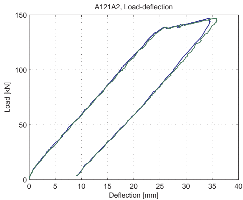
Fig. 5.2.4. Load-deflection curve
