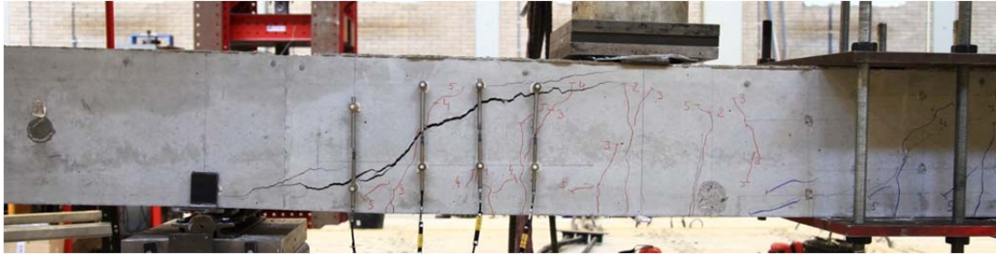
Fig. 5.25.1. Crack pattern after failure north side
