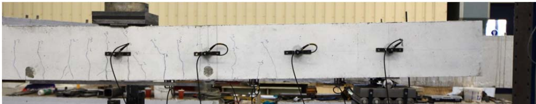
Fig. 5.38.3. Sensors used for Acoustic Emission measurements
