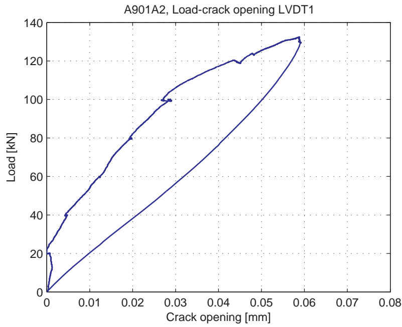
Fig. 5.13.5. Load-Crack opening for LVDT1
