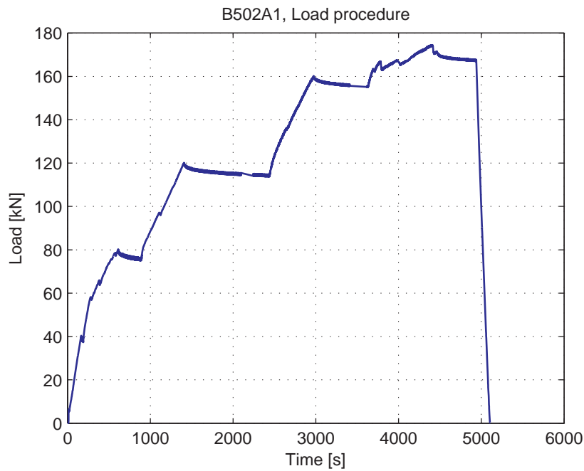
Fig. 5.50.3. Load-Time curve
