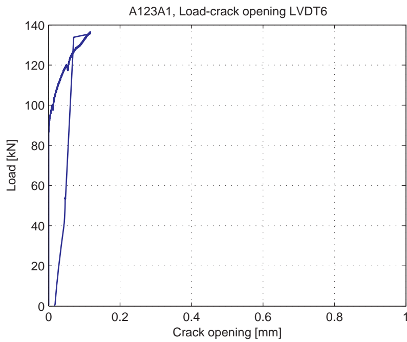
Fig. 5.8.7. Load-Crack opening for LVDT6
