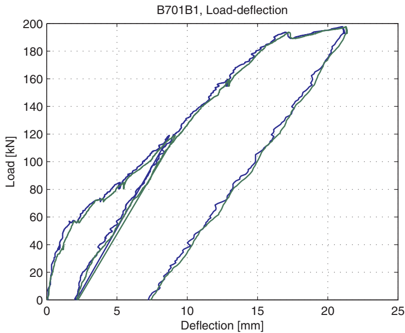
Fig. 5.43.4. Load-deflection curve
