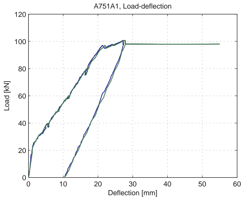
Fig. 5.22.4. Load-deflection curve
