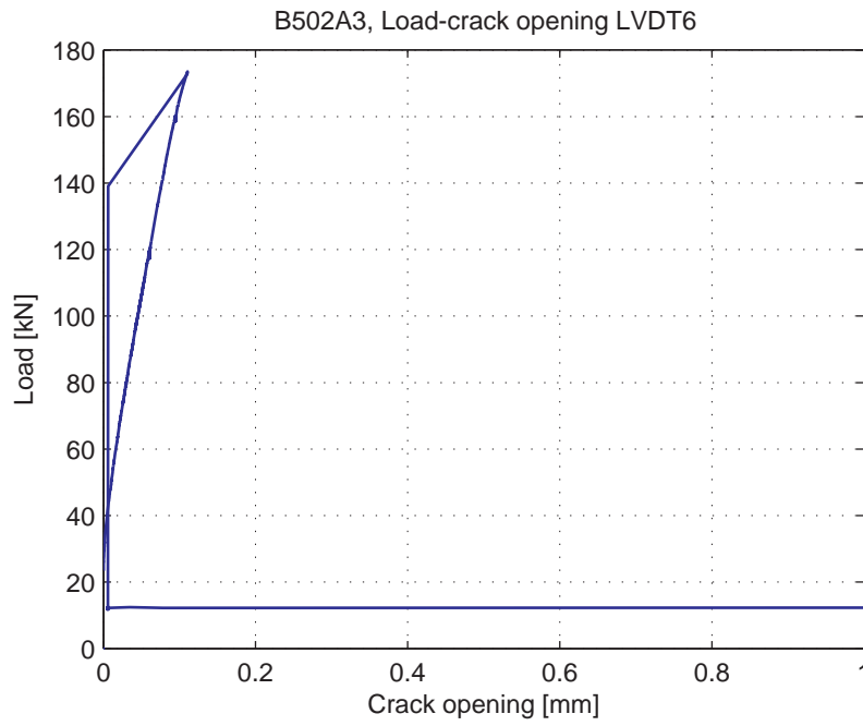
Fig. 5.52.7. Load-Crack opening for LVDT6
