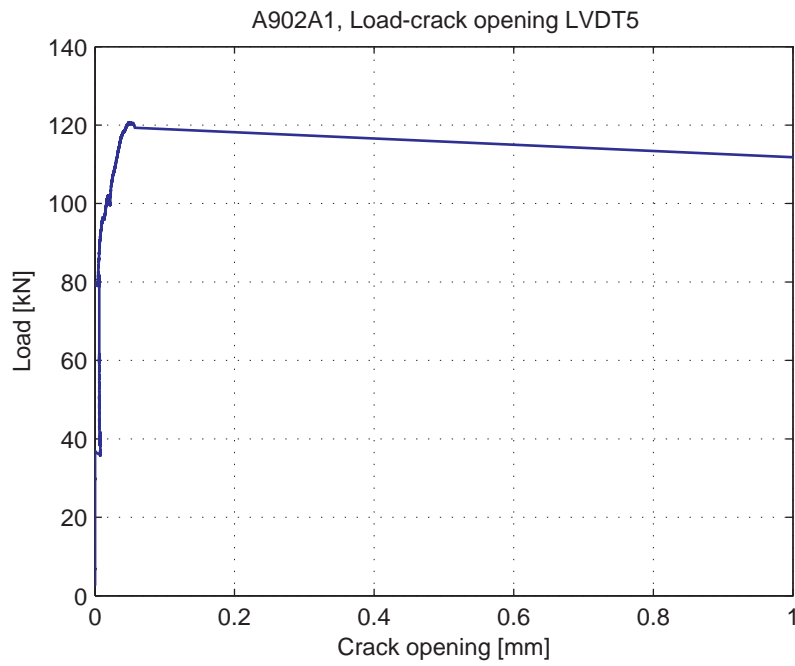
Fig. 5.17.8. Load-Crack opening for LVDT5
