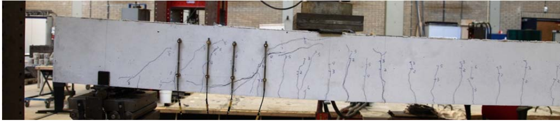
Fig. 5.4.1. Crack pattern after failure north side
