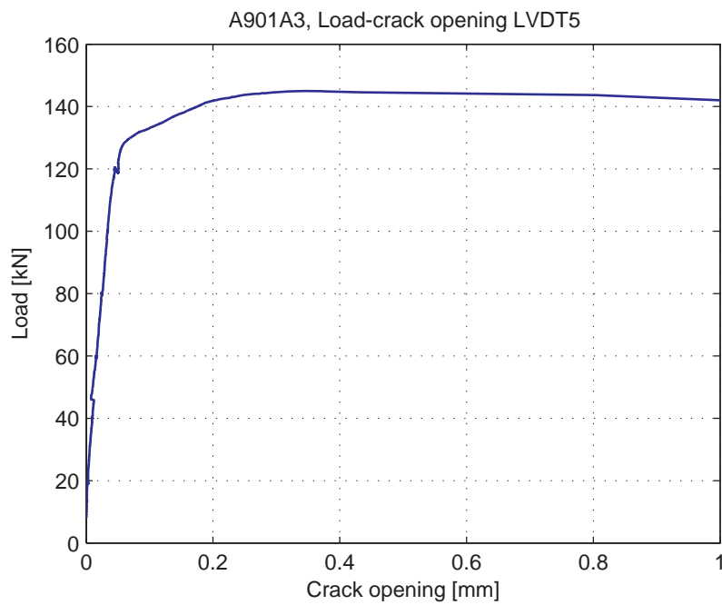
Fig. 5.14.8. Load-Crack opening for LVDT5
