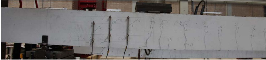
Fig. 5.26.1. Crack pattern after failure north side
