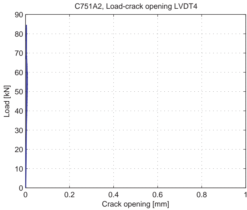
Fig. 5.59.5. Load-Crack opening for LVDT4
