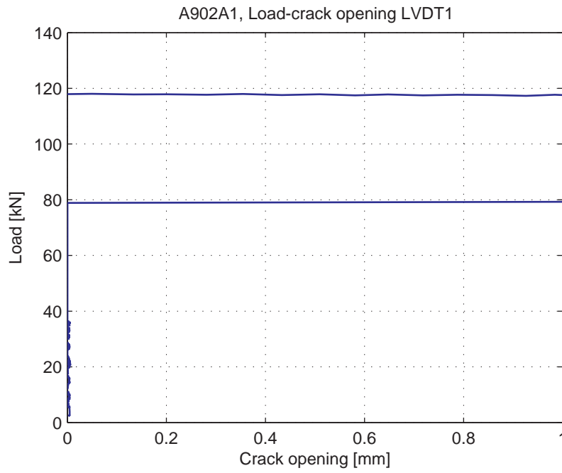
Fig. 5.17.5. Load-Crack opening for LVDT1
