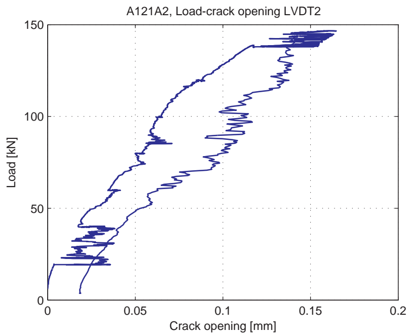
Fig. 5.2.6. Load-Crack opening for LVDT2
