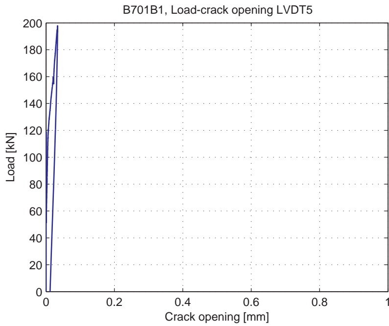
Fig. 5.43.6. Load-Crack opening for LVDT5
