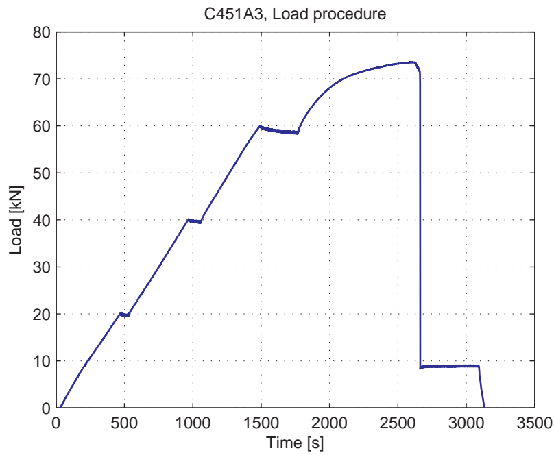
Fig. 5.64.3. Load-Time curve
