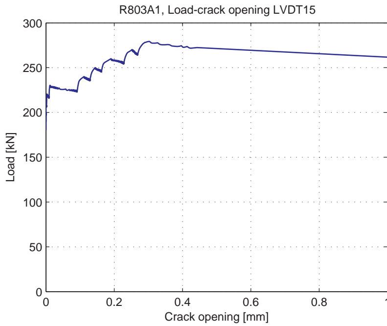
Fig. 5.104.9. Load-Crack opening for LVDT 15
