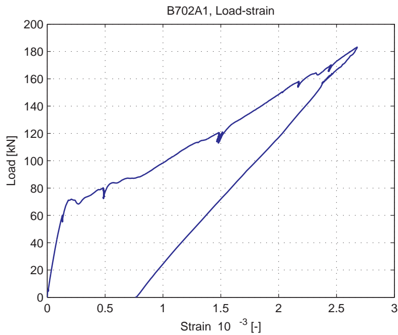
Fig. 5.45.8. Average strain over 1m length, measured at bottom of specimen (LVDT 3)
