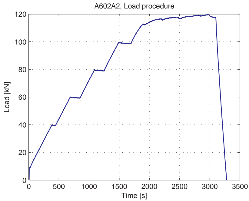
Fig. 5.36.3. Load-Time curve
