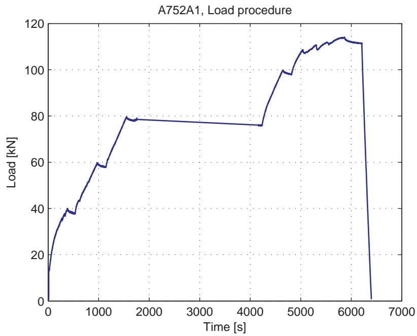
Fig. 5.26.3. Load-Time curve
