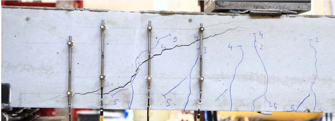
Fig. 5.24.1. Crack pattern after failure north side
