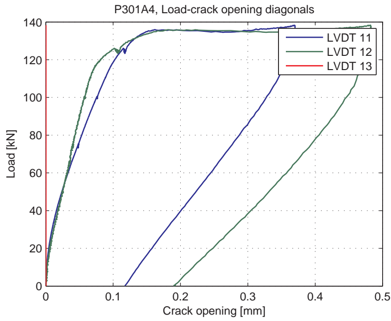
Fig. 5.74.9. Load-Crack opening for LVDT's 11-13 (diagonal)
