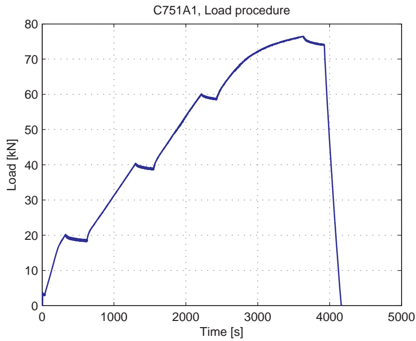
Fig. 5.58.3. Load-Time curve
