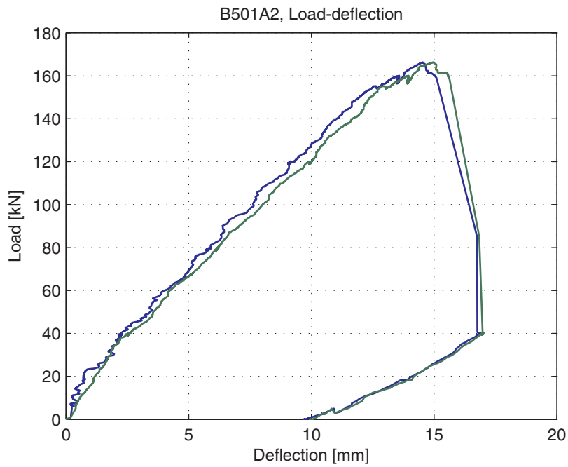
Fig. 5.48.4. Load-deflection curve
