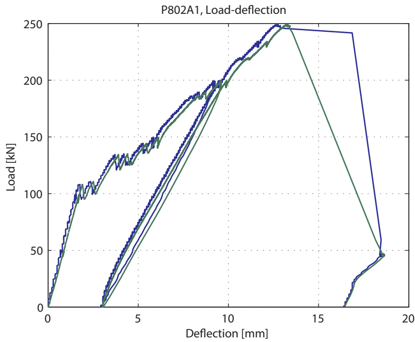
Fig. 5.87.5. Load-deflection curve
