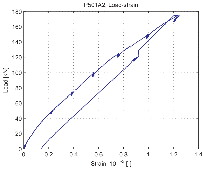
Fig. 5.77.9. Average strain over 1m length, measured at bottom of specimen (LVDT 14)
