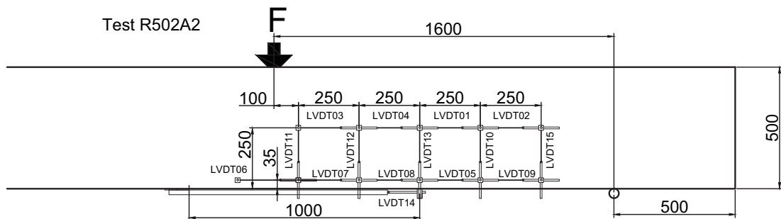
Fig. 5.98.2. LVDT layout and numbering for 500 mm deep beams for test R502A2
