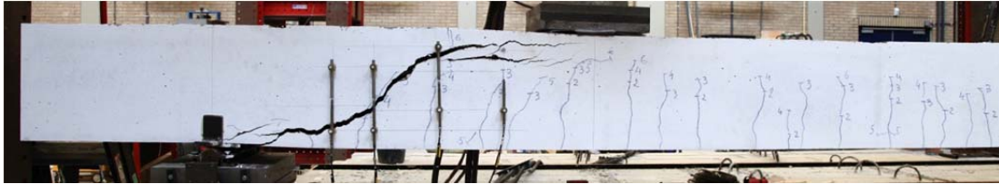
Fig. 5.17.1. Crack pattern after failure north side
