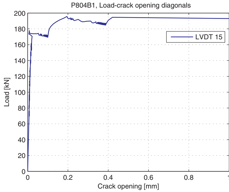
Fig. 5.94.9. Load-Crack opening for LVDT 15 (diagonal)
