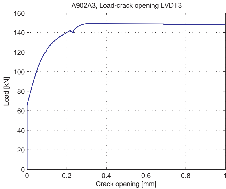
Fig. 5.19.7. Load-Crack opening for LVDT3
