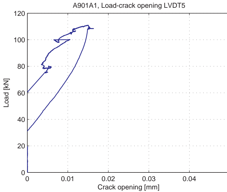
Fig. 5.12.8. Load-Crack opening for LVDT5
