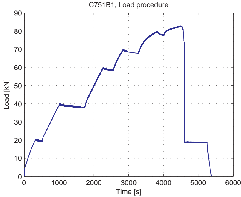
Fig. 5.61.3. Load-Time curve
