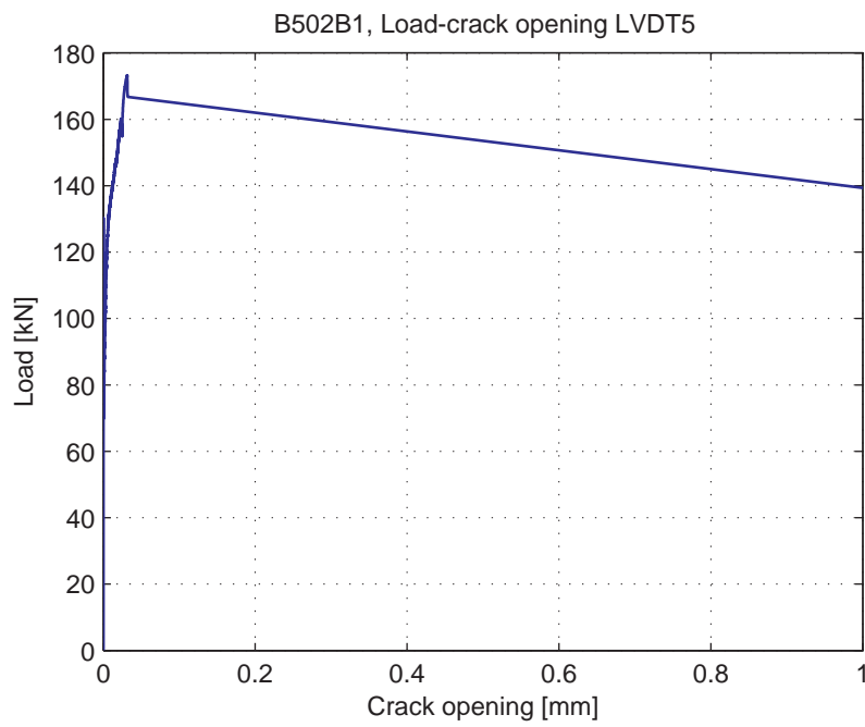
Fig. 5.53.6. Load-Crack opening for LVDT5
