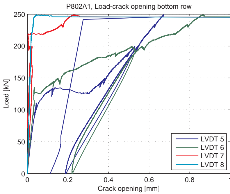
Fig. 5.87.8. Load-Crack opening for LVDT's 5-8 (bottom row)
