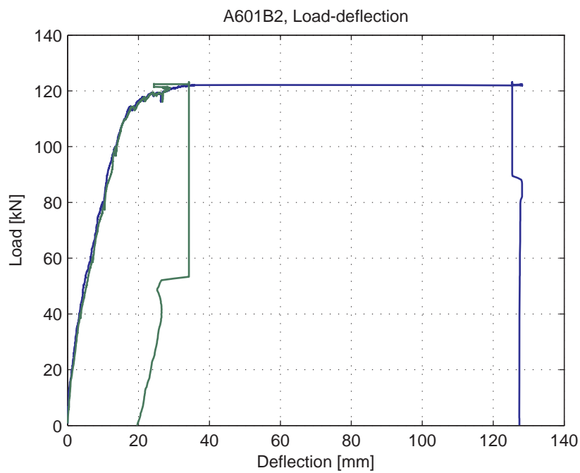
Fig. 5.34.4. Load-deflection curve
