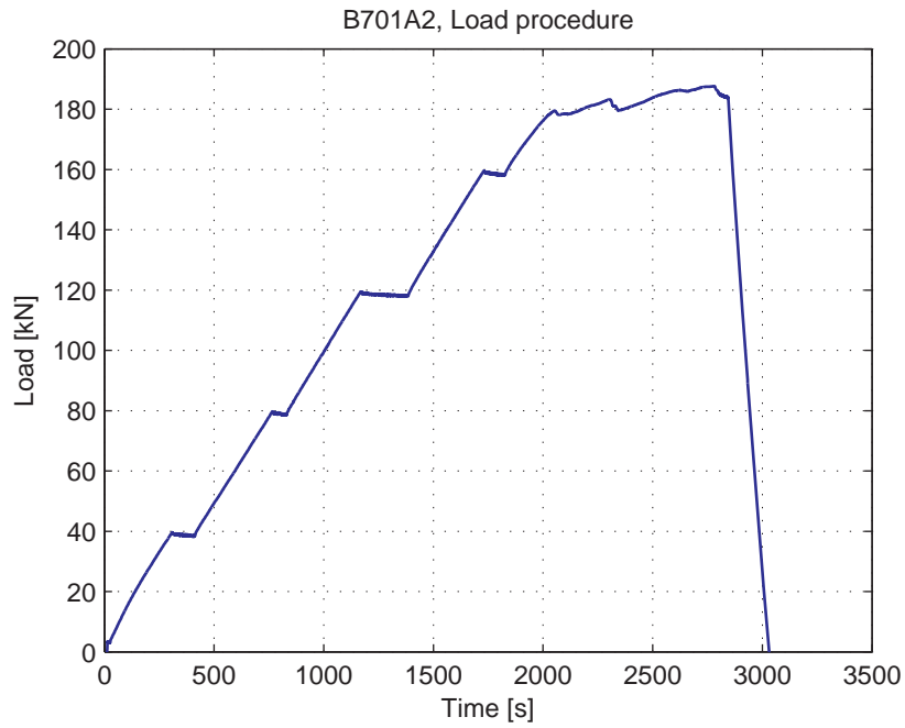
Fig. 5.41.3. Load-Time curve
