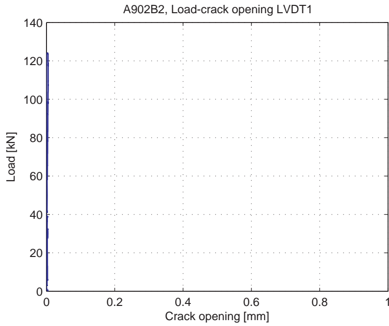
Fig. 5.21.5. Load-Crack opening for LVDT1
