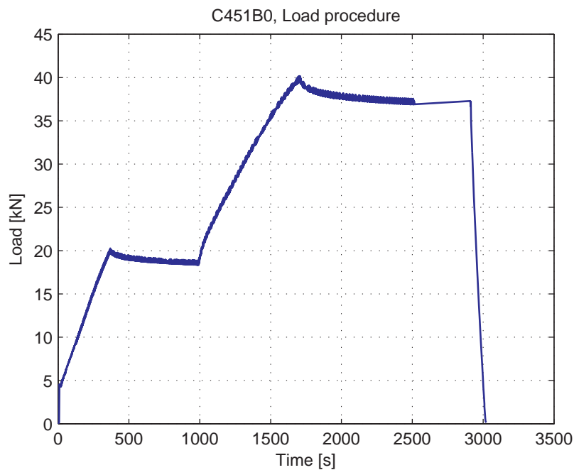
Fig. 5.66.1. Load-Time curve
