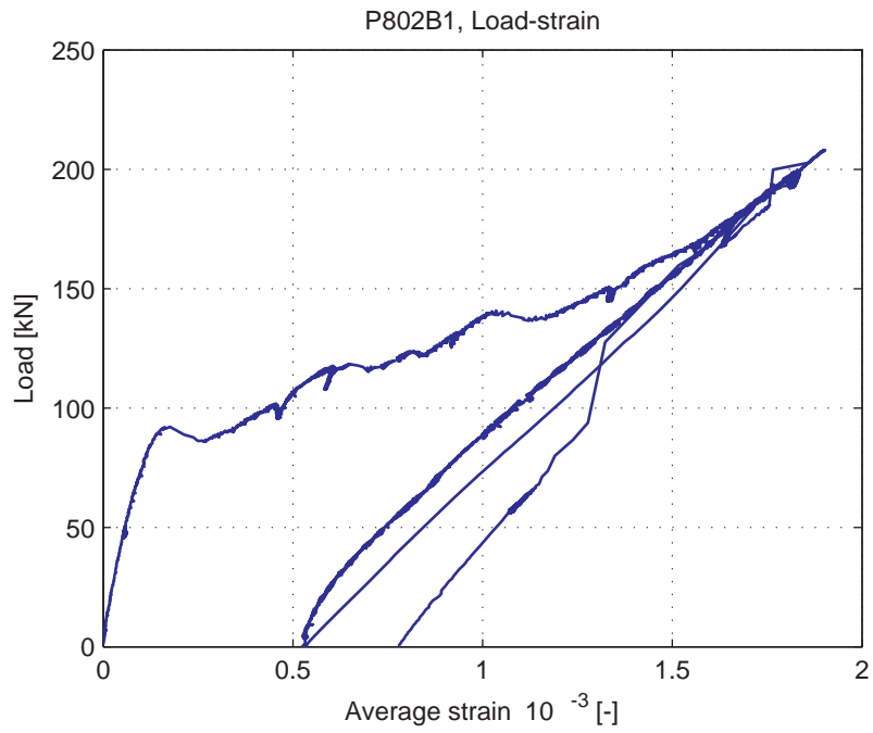
Fig. 5.88.11. Average strain over 1m length, measured at bottom of specimen (LVDT 14)
