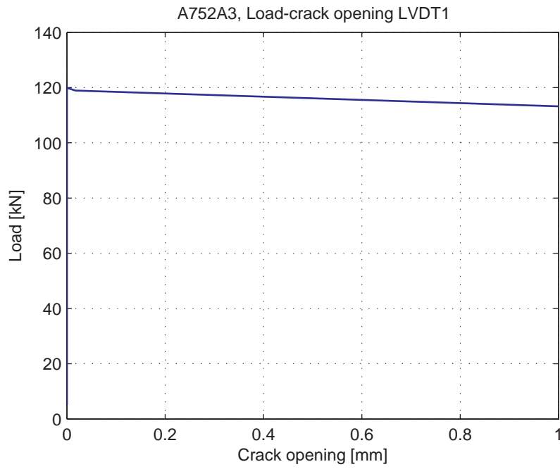
Fig. 5.28.5. Load-Crack opening for LVDT1
