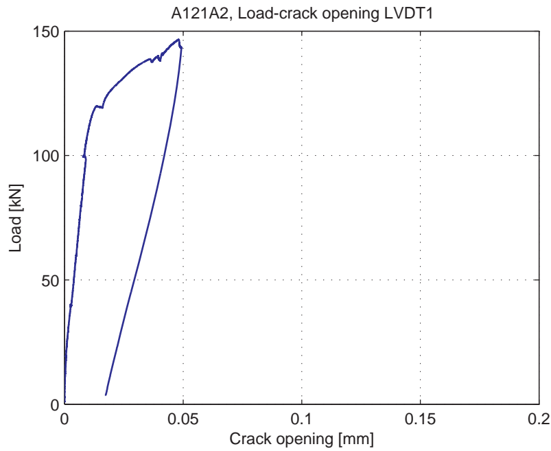
Fig. 5.2.5. Load-Crack opening for LVDT1
