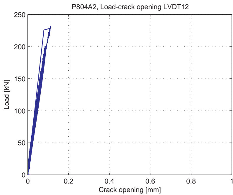
Fig. 5.93.8. Load-Crack opening for LVDT 12
