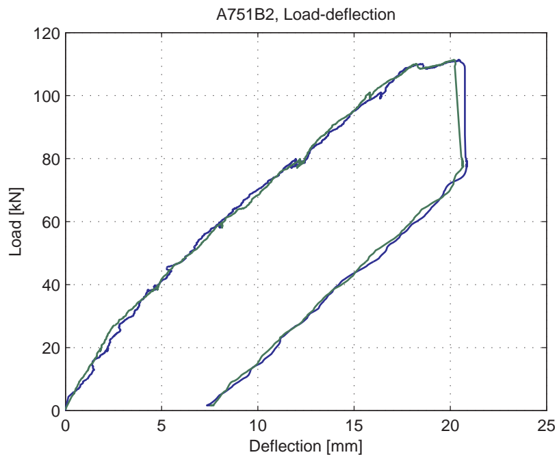
Fig. 5.25.4. Load-deflection curve
