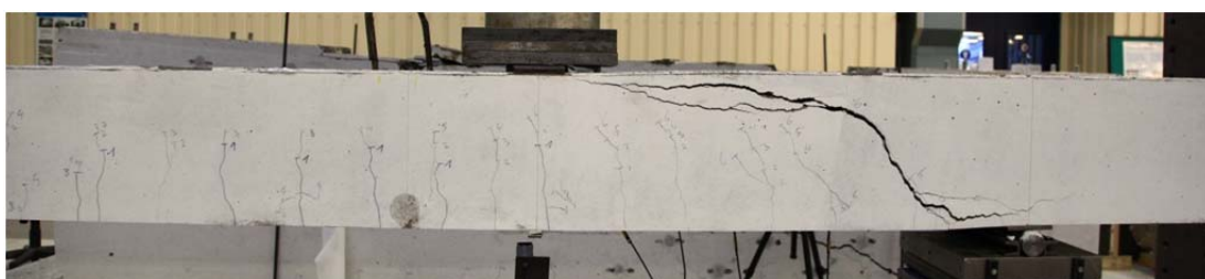
Fig. 5.6.2. Crack pattern after failure south side
