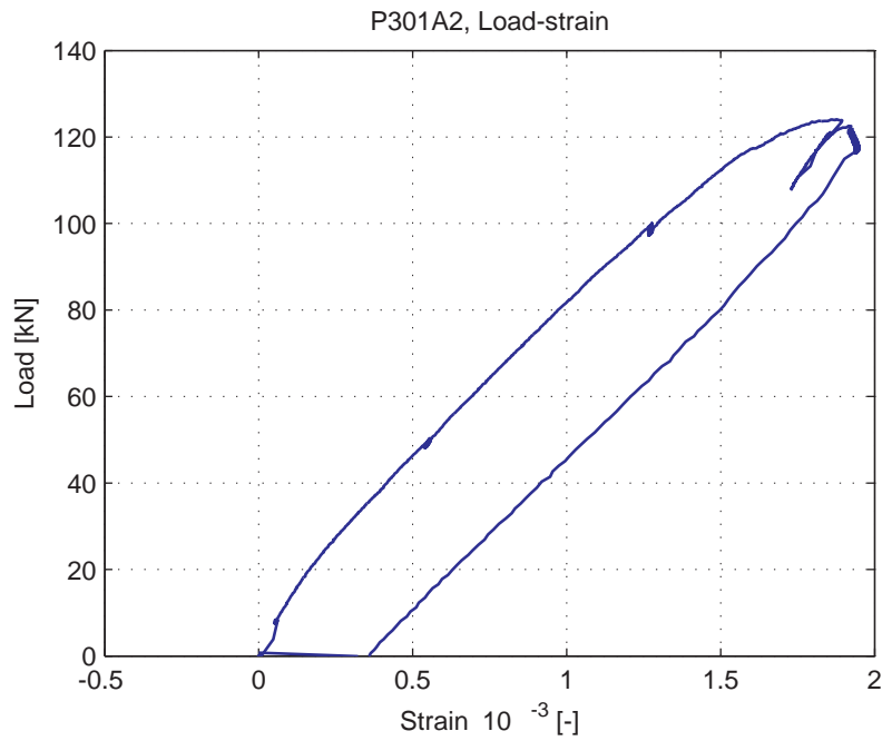
Fig. 5.72.10. Average strain over 1m length, measured at bottom of specimen (LVDT 14)
