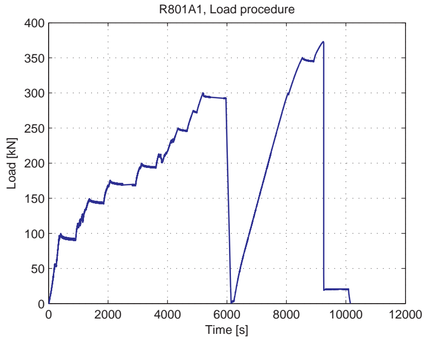
Fig. 5.100.4. Load-Time curve
