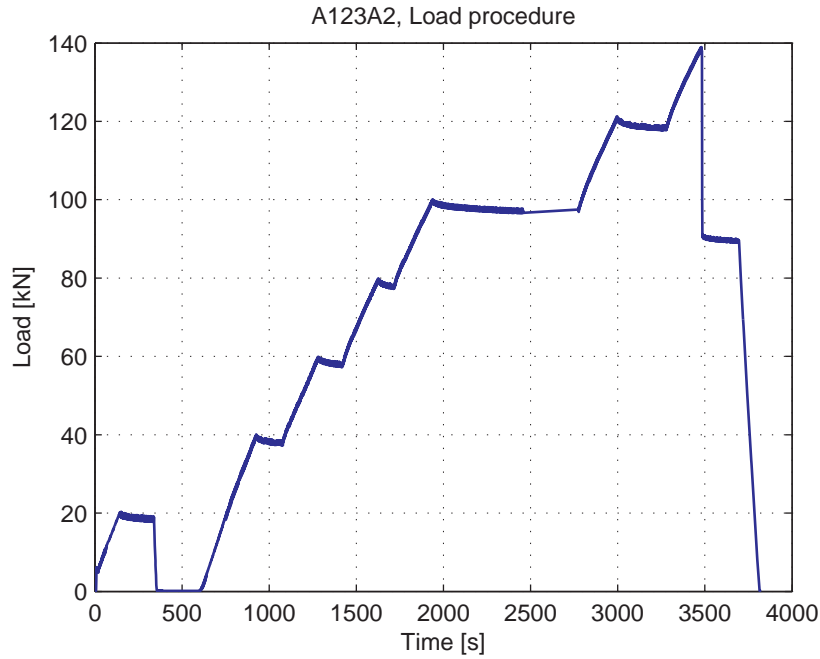
Fig. 5.9.3. Load-Time curve
