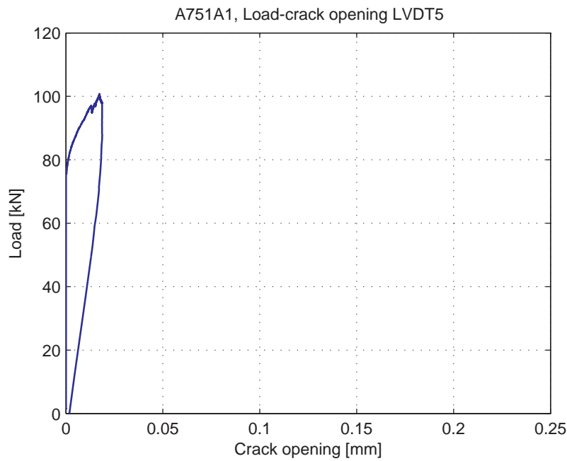
Fig. 5.22.8. Load-Crack opening for LVDT5
