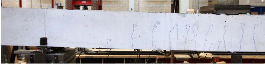
Fig. 5.38.1. Crack pattern after failure north side
