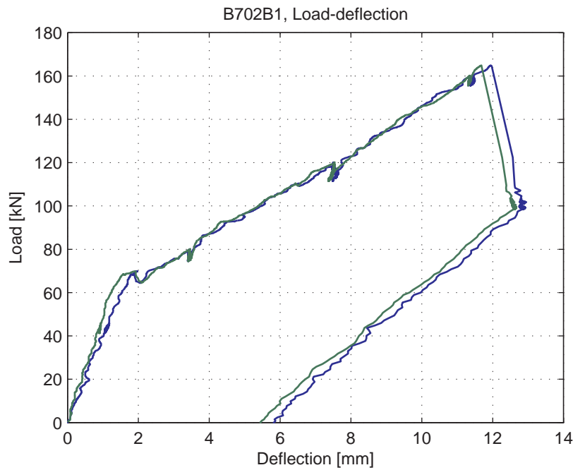
Fig. 5.46.4. Load-deflection curve
