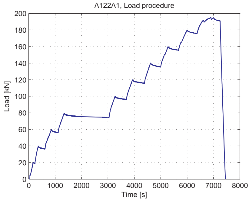
Fig. 5.5.3. Load-Time curve
