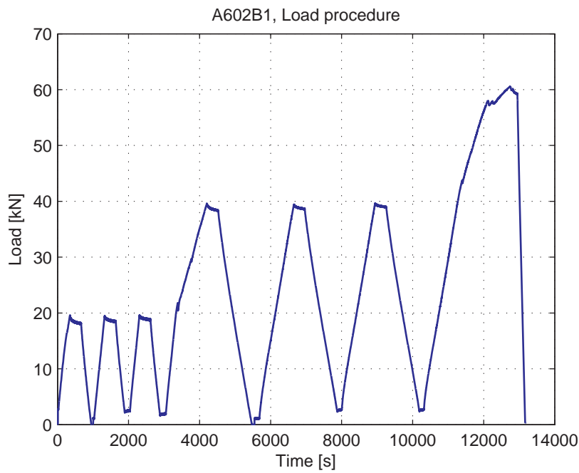
Fig. 5.38.4. Load-Time curve
