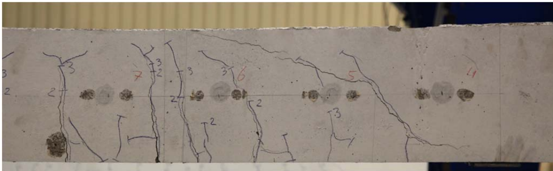
Fig. 5.30.2. Crack pattern after failure south side
