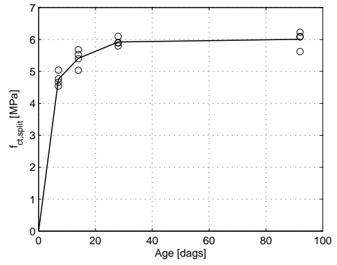
Fig. 2.2.10. F_{ct,split} development for cast 6
