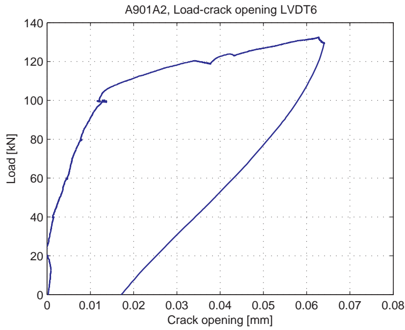
Fig. 5.13.9. Load-Crack opening for LVDT6
