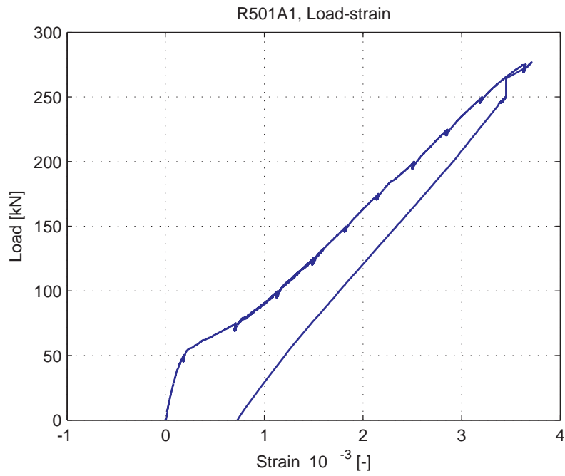
Fig. 5.95.9. Average strain over 1m length, measured at bottom of specimen (LVDT 14)
