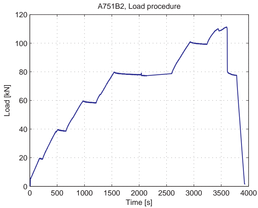
Fig. 5.25.3. Load-Time curve
