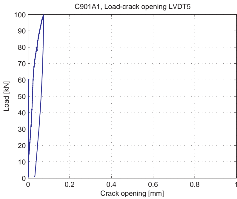
Fig. 5.54.4. Load-Crack opening for LVDT5
