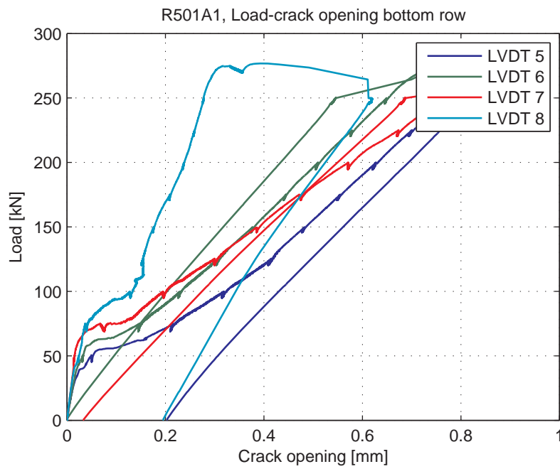
Fig. 5.95.8. Load-Crack opening for LVDT's 5-8 (bottom row)
