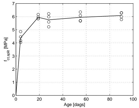
Fig. 2.2.14. F_{ct,split} development for cast 8
