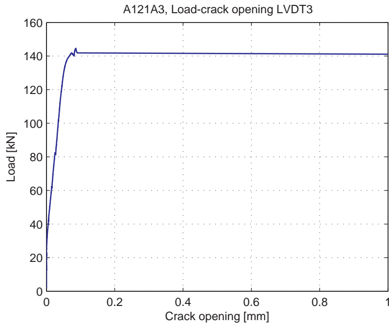
Fig. 5.3.7. Load-Crack opening for LVDT3
