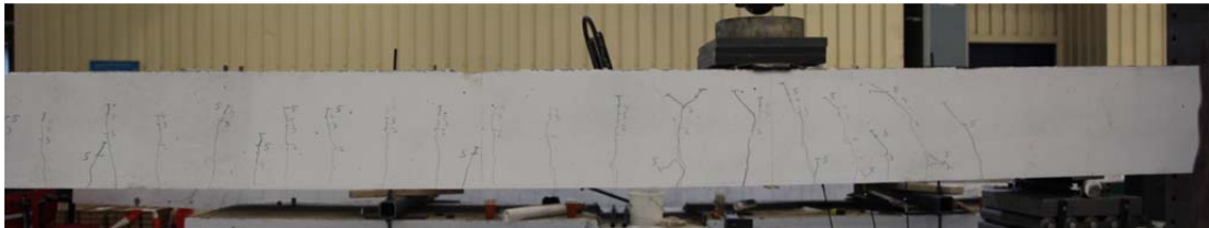
Fig. 5.26.2. Crack pattern after failure south side
