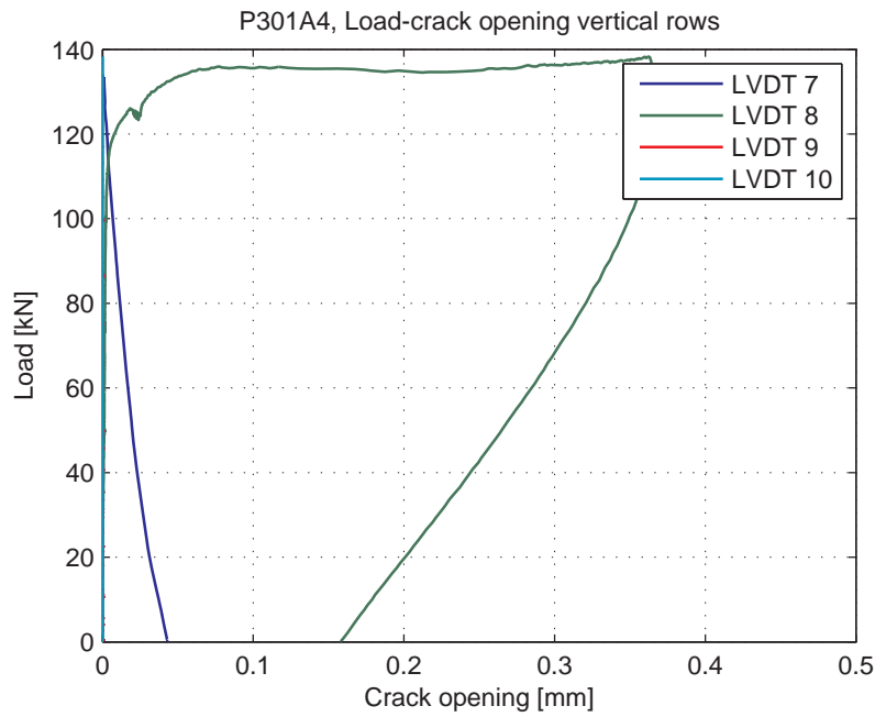
Fig. 5.74.7. Load-Crack opening for LVDT's 7-10 (vertical LVDT's)
