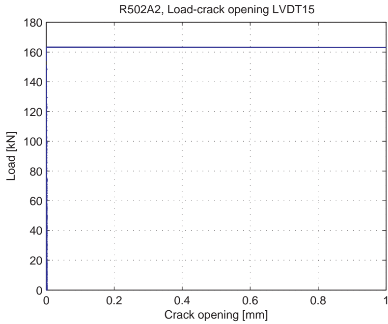
Fig. 5.98.9. Load-Crack opening for LVDT 15
