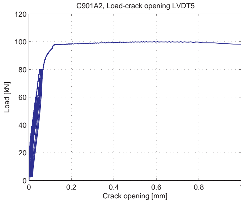
Fig. 5.55.6. Load-Crack opening for LVDT5
