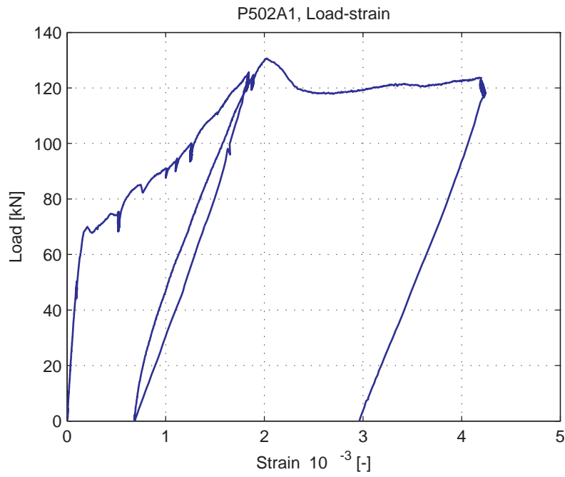
Fig. 5.80.9. Average strain over 1m length, measured at bottom of specimen (LVDT 14)
