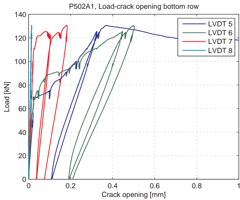
Fig. 5.80.8. Load-Crack opening for LVDT's 5-8 (bottom row)
