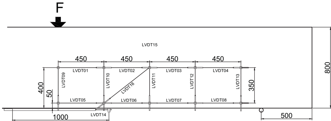
Fig. 5.84.2. LVDT layout and numbering for 800 mm deep beams
