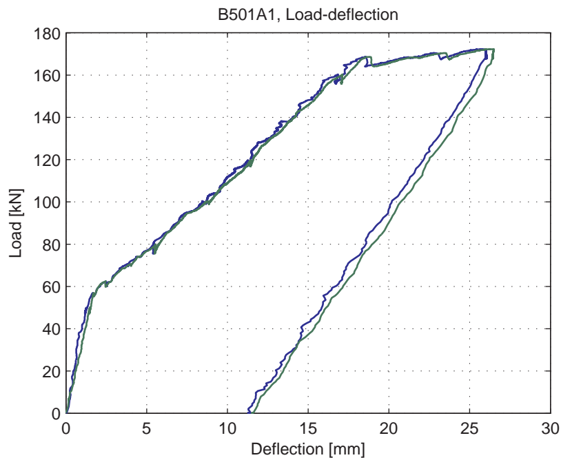
Fig. 5.47.4. Load-deflection curve
