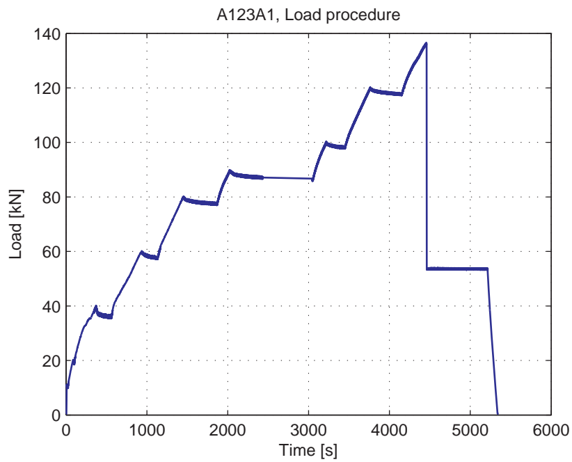
Fig. 5.8.3. Load-Time curve
