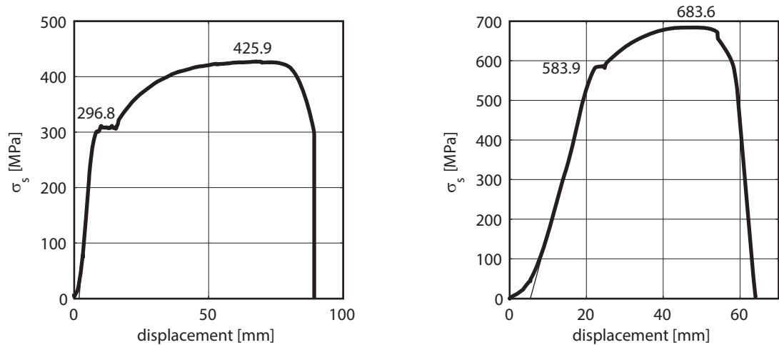
Fig. 2.2.17. Comparison of typical stress-displacement curve of plain bar(left) and ribbed bar(right).
