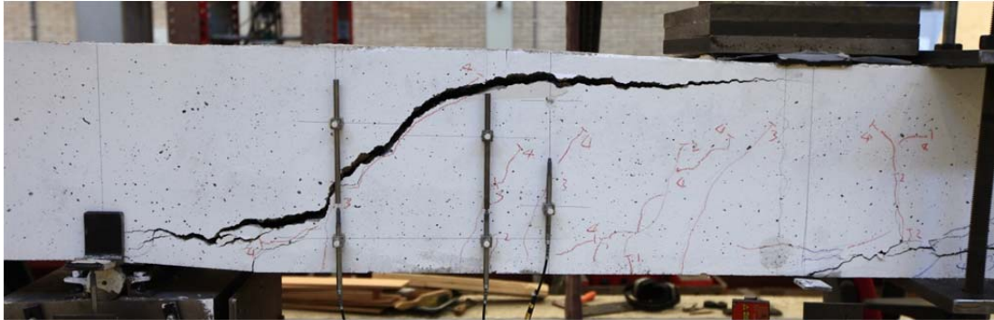
Fig. 5.60.1. Crack pattern after failure north side
