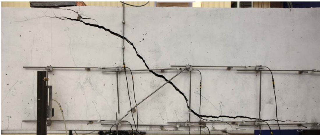
Fig. 5.88.2. Crack pattern after failure and LVDT layout at south side of beam
