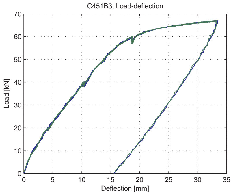
Fig. 5.69.4. Load-deflection curve
