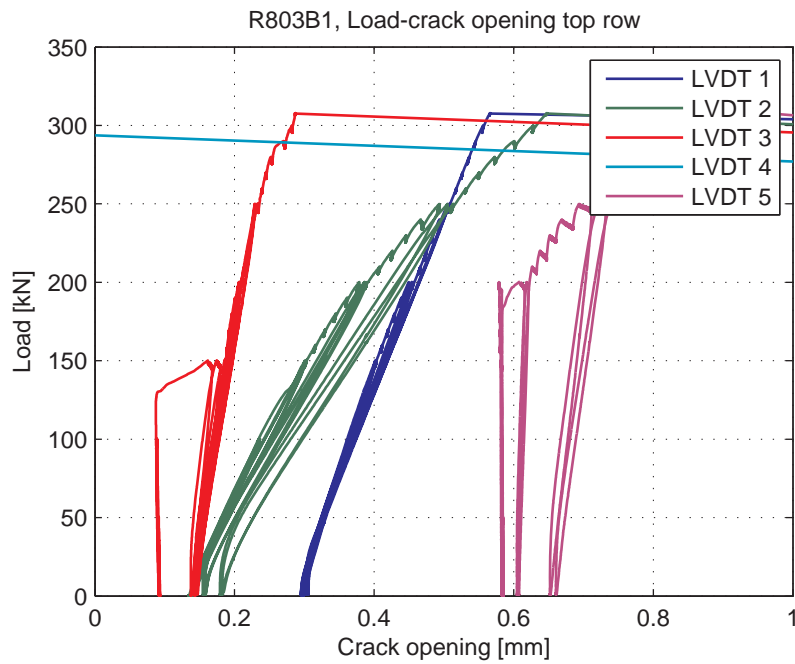
Fig. 5.105.6. Load-Crack opening for LVDT's 1-4 (top row)
