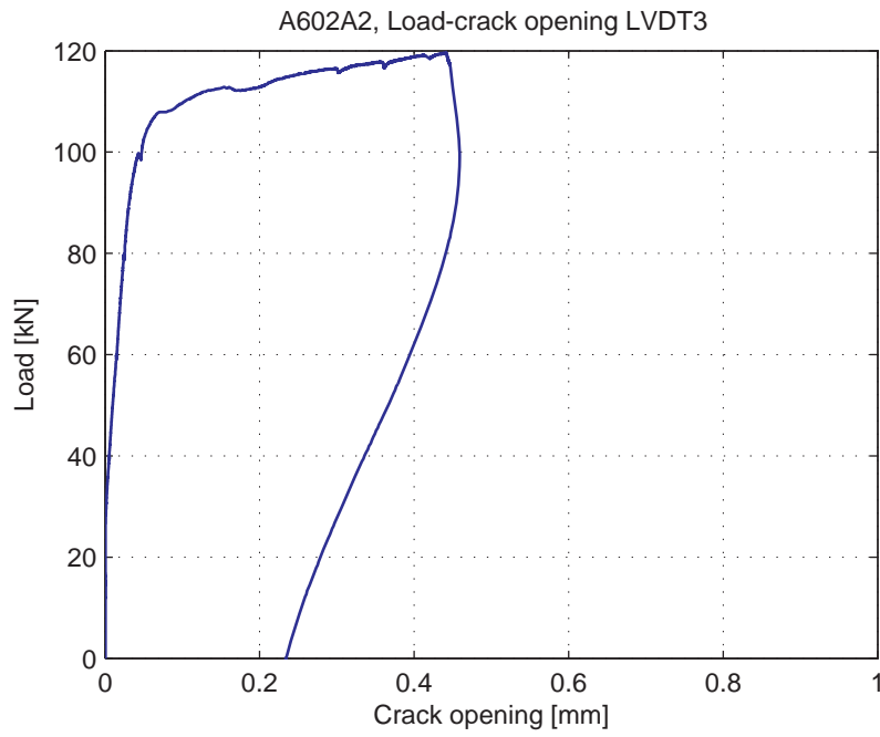
Fig. 5.36.7. Load-Crack opening for LVDT3
