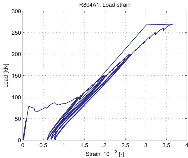
Fig. 5.106.10. Average strain over 1m length, measured at bottom of specimen (LVDT 14)
