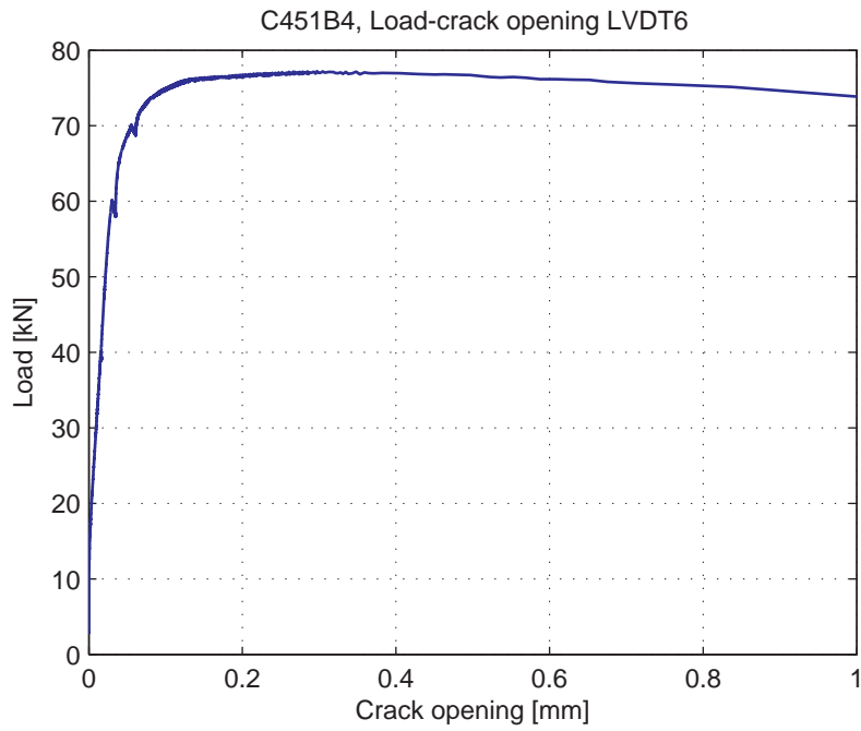
Fig. 5.70.8. Load-Crack opening for LVDT6
