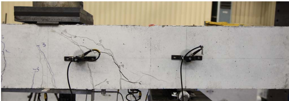
Fig. 5.39.2. Crack pattern after failure south side
