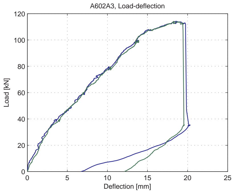
Fig. 5.37.4. Load-deflection curve
