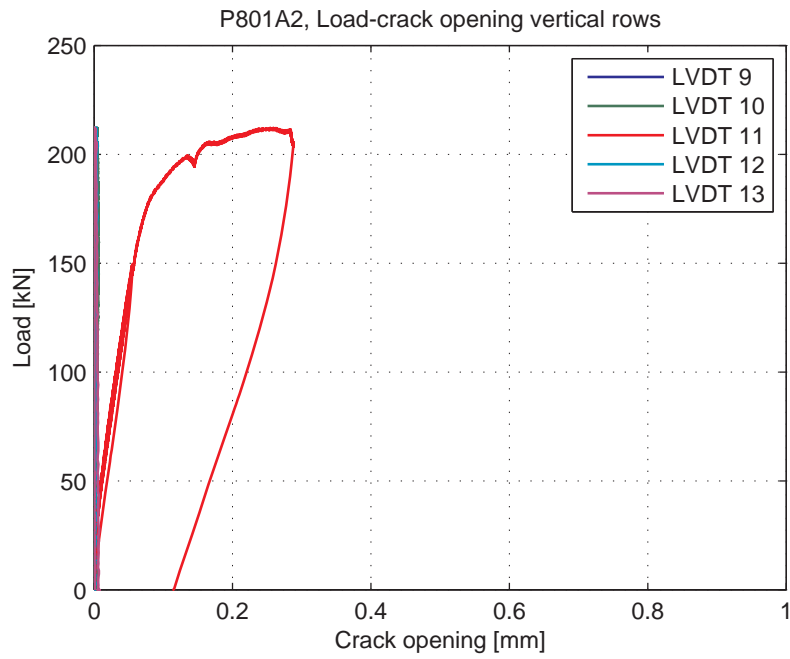
Fig. 5.84.6. Load-Crack opening for LVDT's 9-13 (vertical LVDT's)
