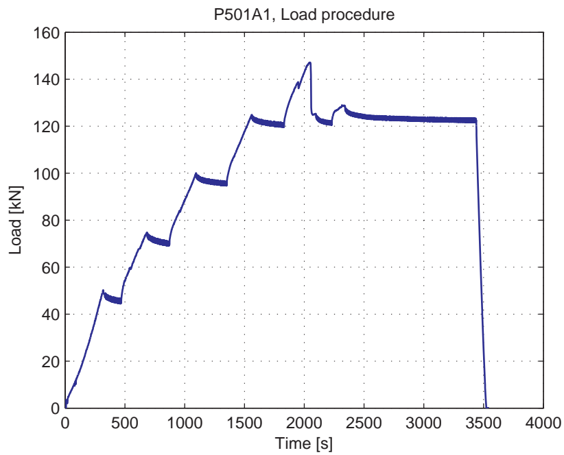
Fig. 5.76.4. Load-Time curve
