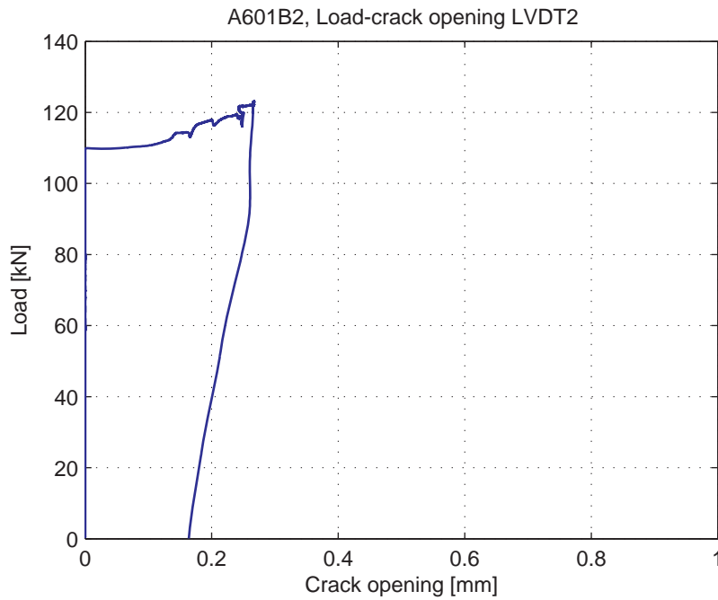
Fig. 5.34.6. Load-Crack opening for LVDT2
