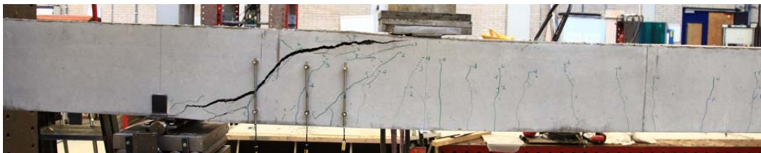
Fig. 5.15.1. Crack pattern after failure north side
