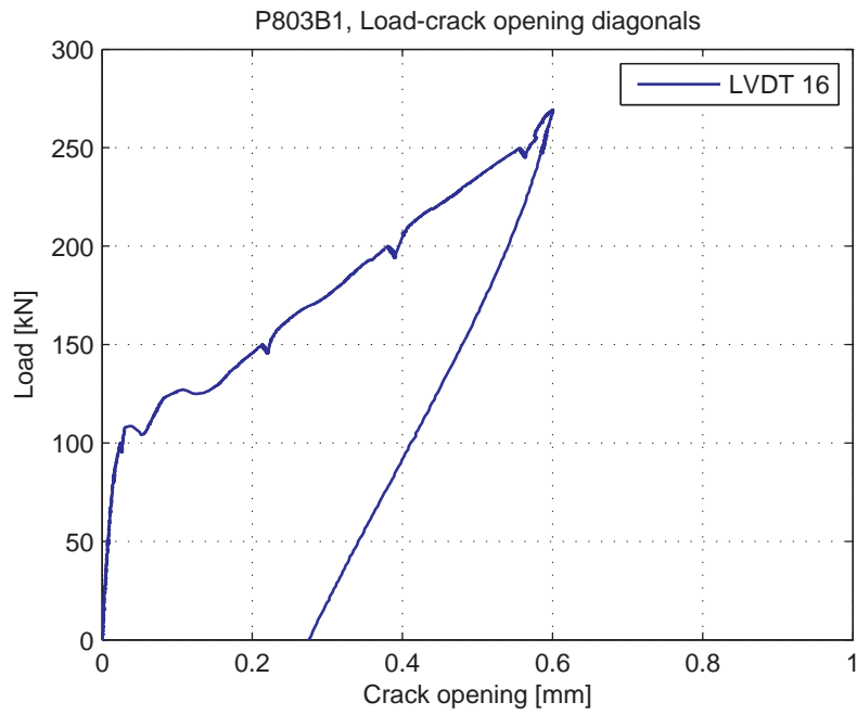
Fig. 5.90.9. Load-Crack opening for LVDT 16 (diagonal)
