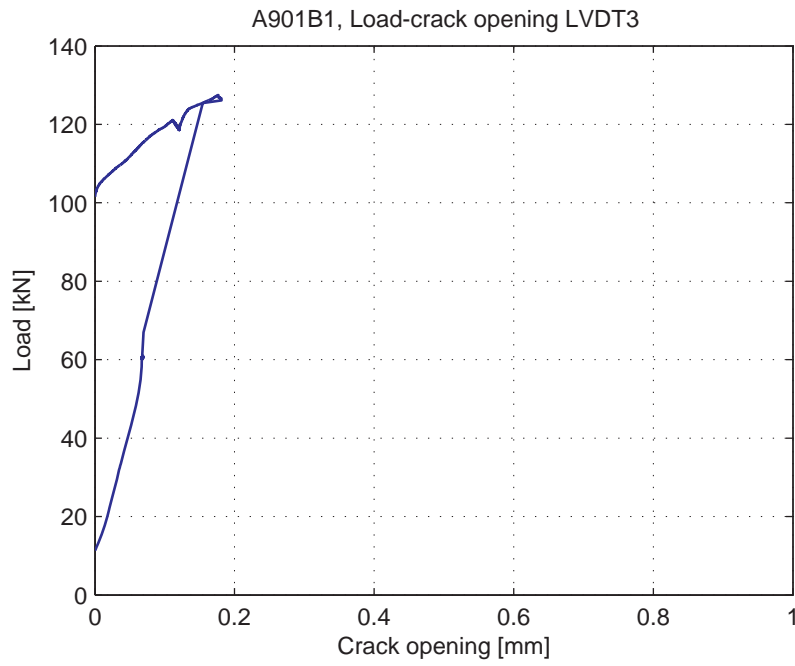
Fig. 5.15.7. Load-Crack opening for LVDT3
