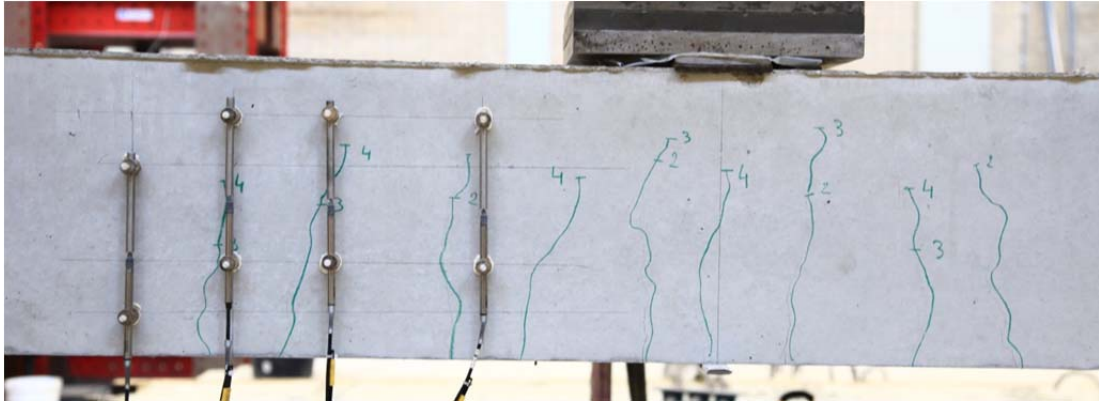
Fig. 5.22.1. Crack pattern after failure north side
