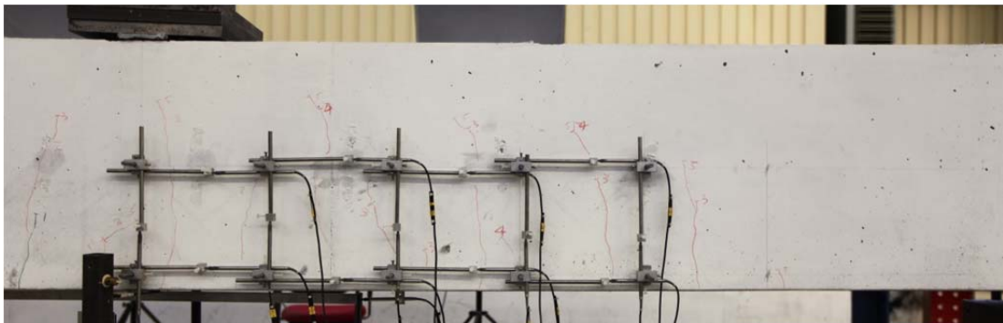
Fig. 5.76.2. Crack pattern after failure back side
