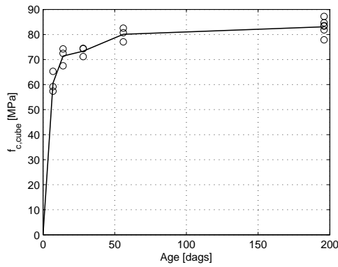
Fig. 2.2.3. F_{c,cube} development for cast 2
