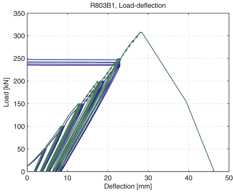
Fig. 5.105.5. Load-deflection curve
