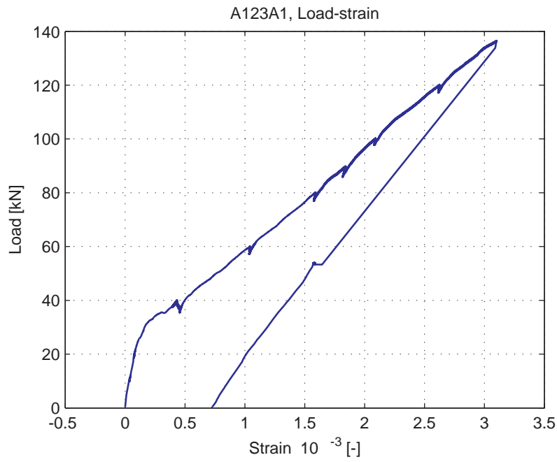
Fig. 5.8.8. Average strain over 1m length, measured at bottom of specimen (LVDT 3)
