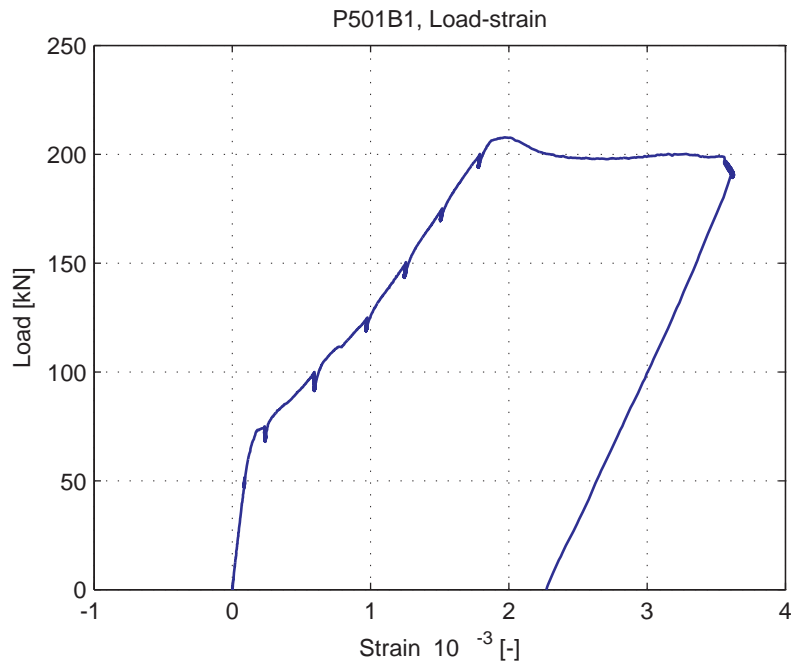
Fig. 5.78.9. Average strain over 1m length, measured at bottom of specimen (LVDT 14)
