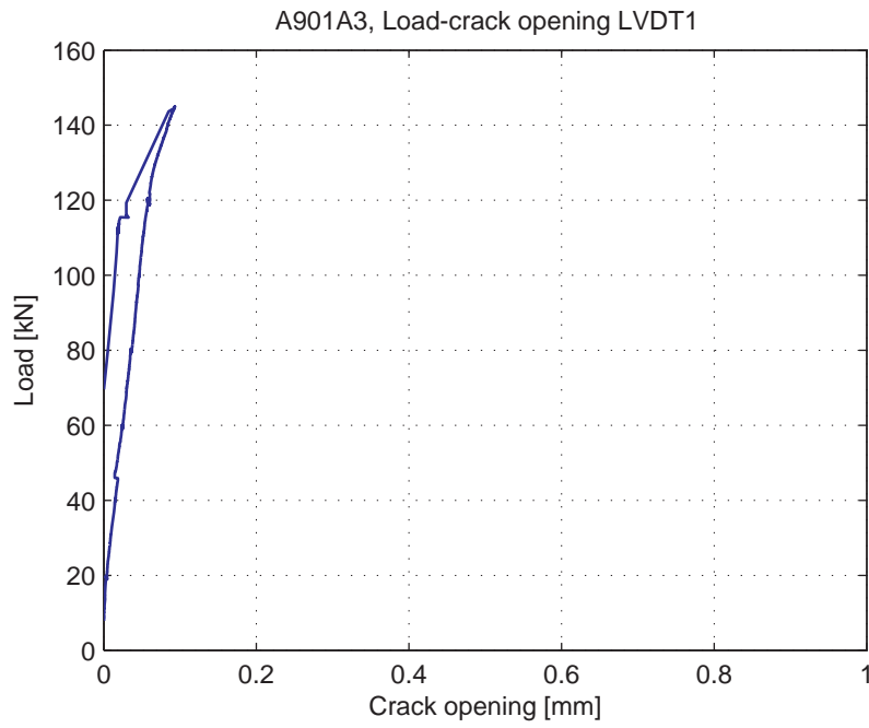
Fig. 5.14.5. Load-Crack opening for LVDT1
