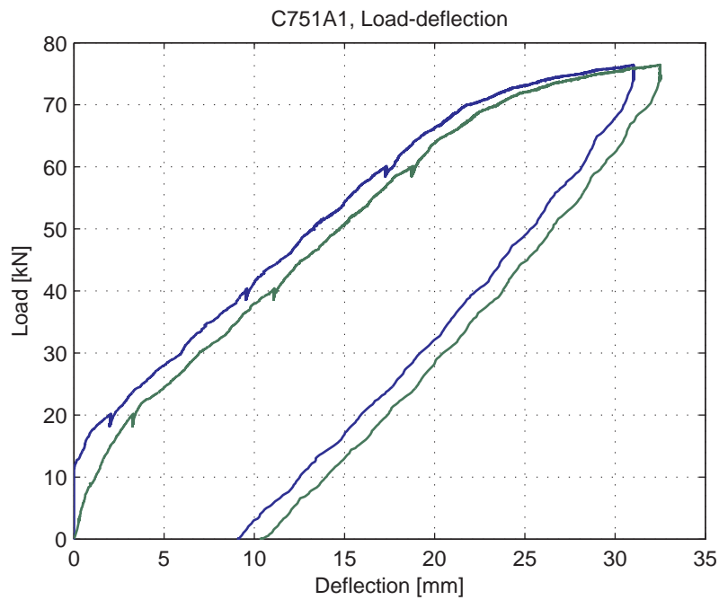
Fig. 5.58.4. Load-deflection curve
