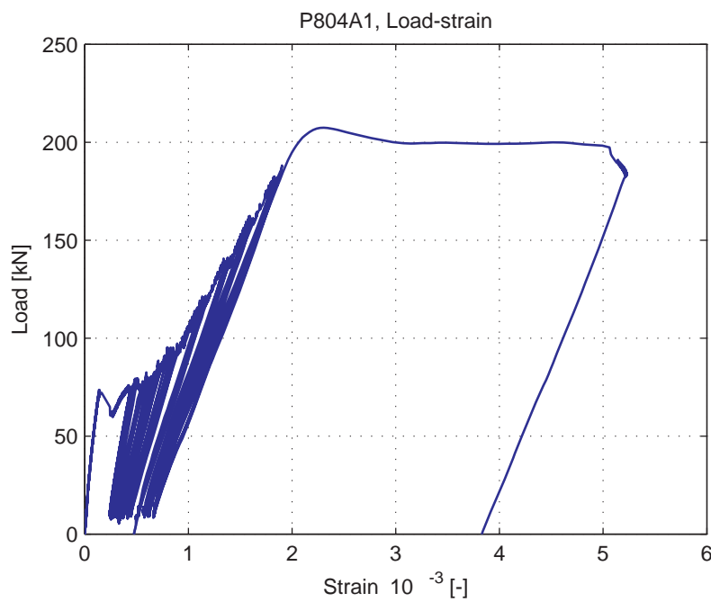
Fig. 5.92.13. Average strain over 1m length, measured at bottom of specimen (LVDT 14)
