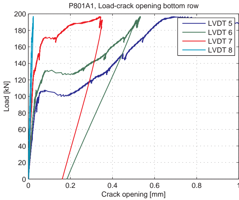
Fig. 5.83.7. Load-Crack opening for LVDT's 5-8 (bottom row)
