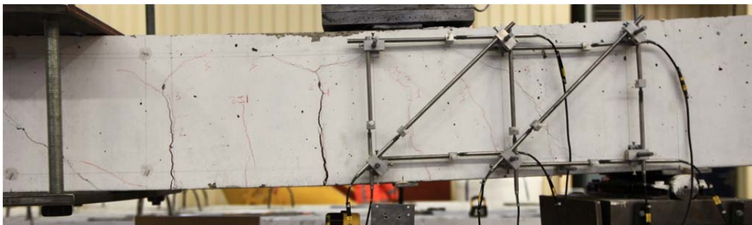
Fig. 5.74.2. Crack pattern after failure back side
