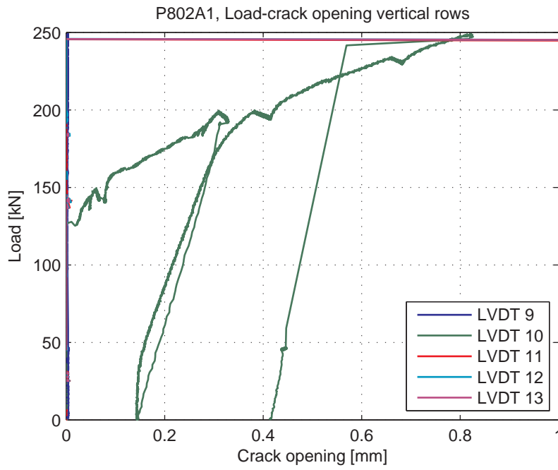
Fig. 5.87.7. Load-Crack opening for LVDT's 9-13 (vertical LVDT's)
