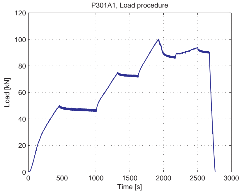
Fig. 5.71.3. Load-Time curve
