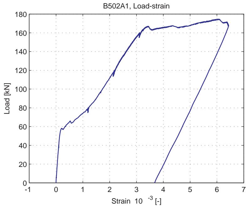
Fig. 5.50.9. Average strain over 1m length, measured at bottom of specimen (LVDT 3)
