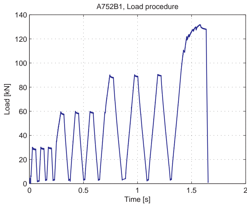
Fig. 5.29.4. Load-Time curve
