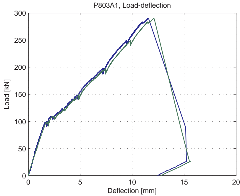
Fig. 5.89.5. Load-deflection curve
