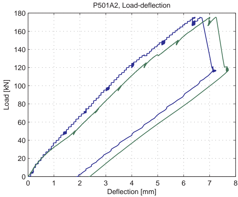
Fig. 5.77.5. Load-deflection curve
