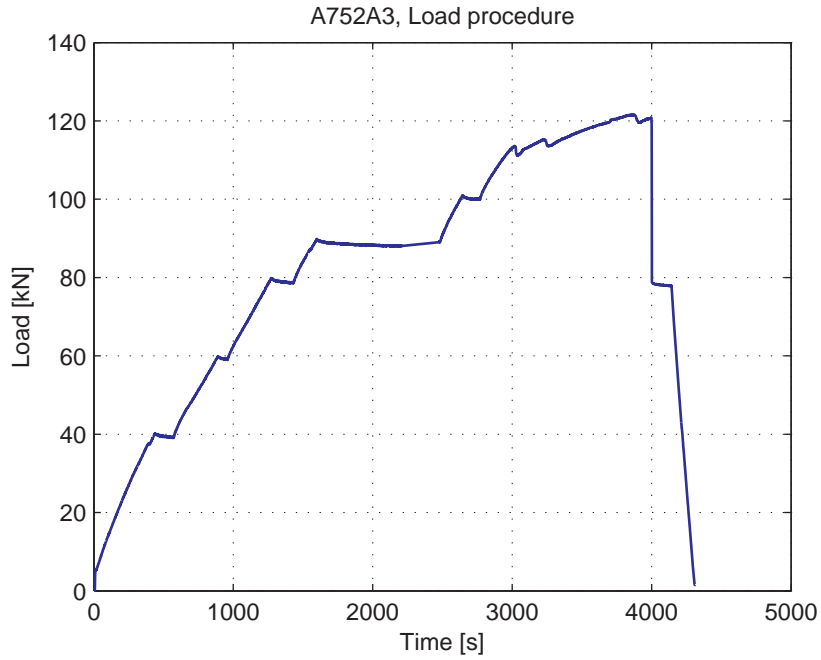
Fig. 5.28.3. Load-Time curve
