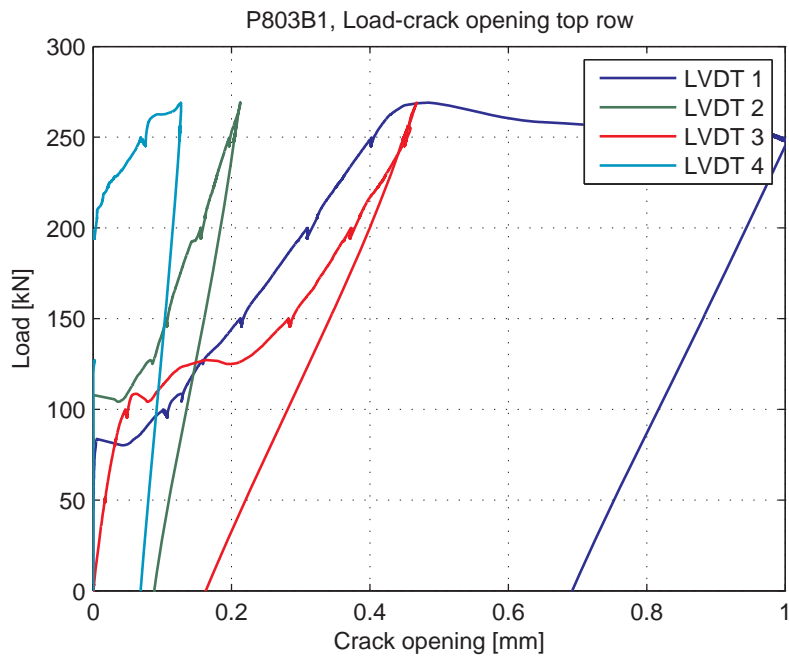
Fig. 5.90.6. Load-Crack opening for LVDT's 1-4 (top row)
