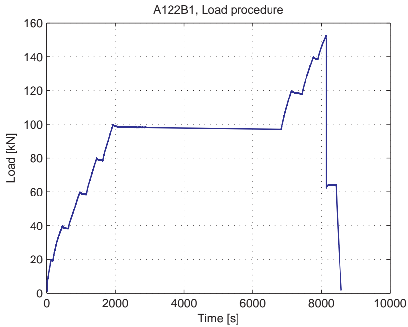
Fig. 5.6.3. Load-Time curve
