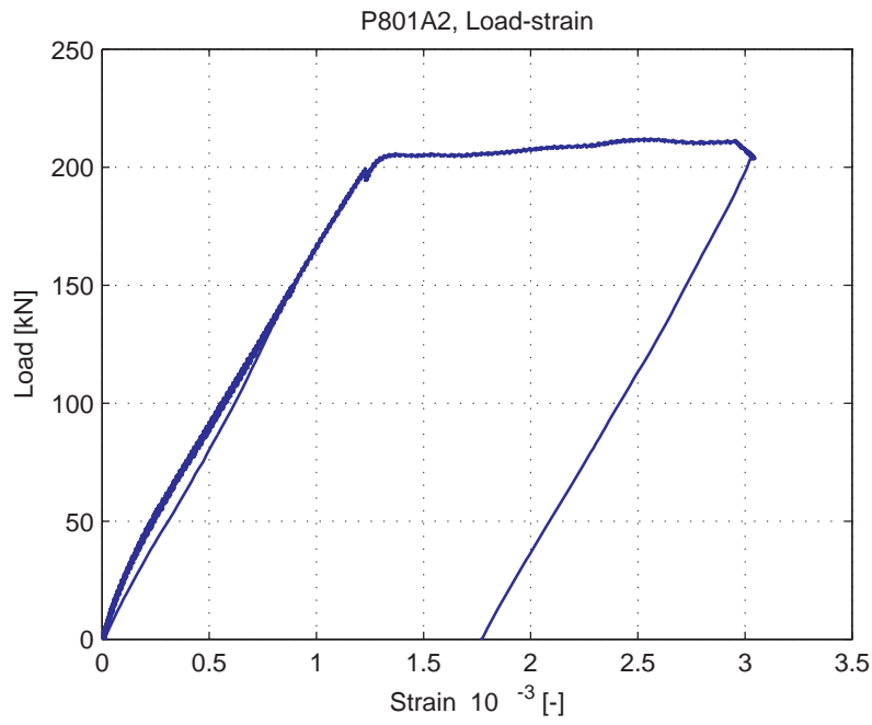
Fig. 5.84.10. Average strain over 1m length, measured at bottom of specimen (LVDT 14)
