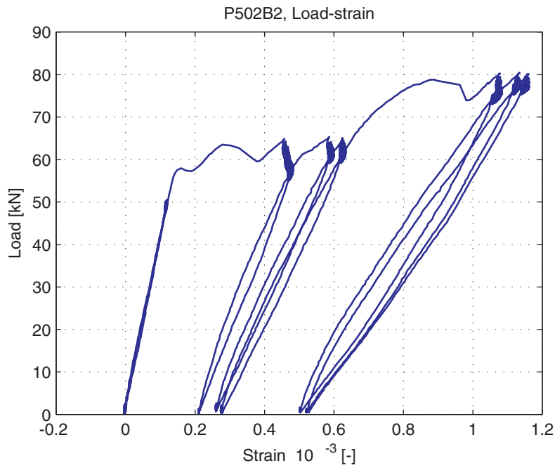
Fig. 5.82.14. Average strain over 1m length for second part of test, measured at bottom of specimen (LVDT 13)
