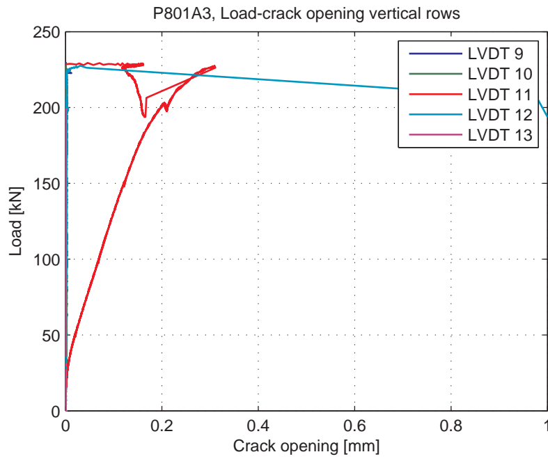
Fig. 5.85.7. Load-Crack opening for LVDT's 9-13 (vertical LVDT's)
