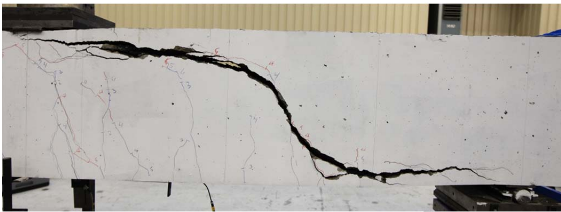
Fig. 5.52.2. Crack pattern after failure south side
