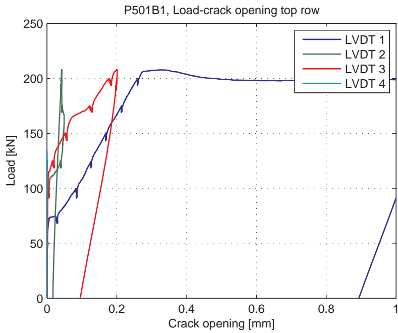
Fig. 5.78.6. Load-Crack opening for LVDT's 1-4 (top row)
