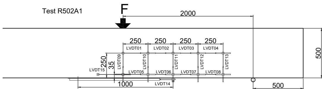
Fig. 5.97.3. LVDT layout and numbering for 500 mm deep beams for test R502A1
