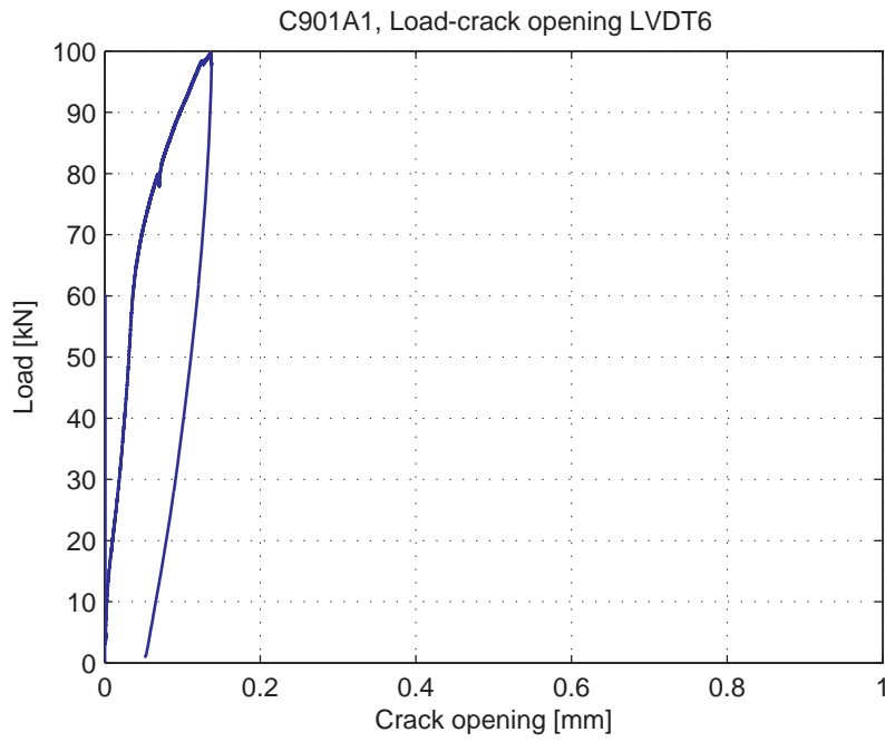
Fig. 5.54.5. Load-Crack opening for LVDT6
