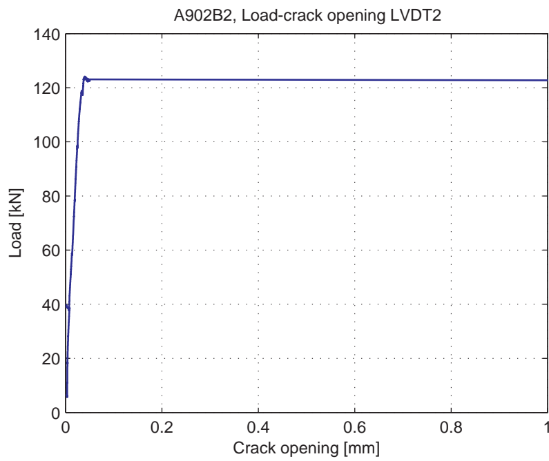
Fig. 5.21.6. Load-Crack opening for LVDT2
