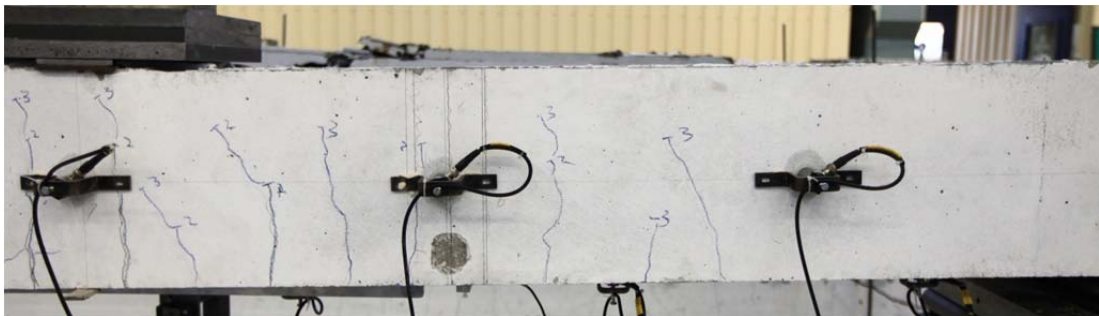
Fig. 5.38.2. Crack pattern after failure south side
