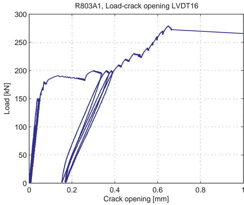
Fig. 5.104.10. Load-Crack opening for LVDT 16
