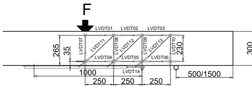
Fig. 5.72.3. LVDT layout and numbering for 300 mm deep beams
