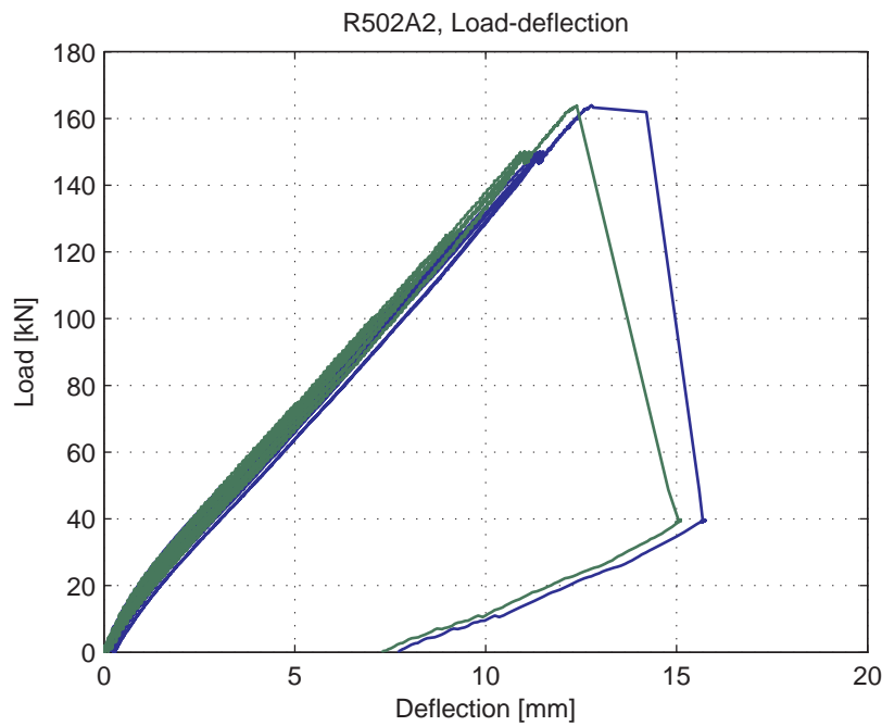
Fig. 5.98.4. Load-deflection curve
