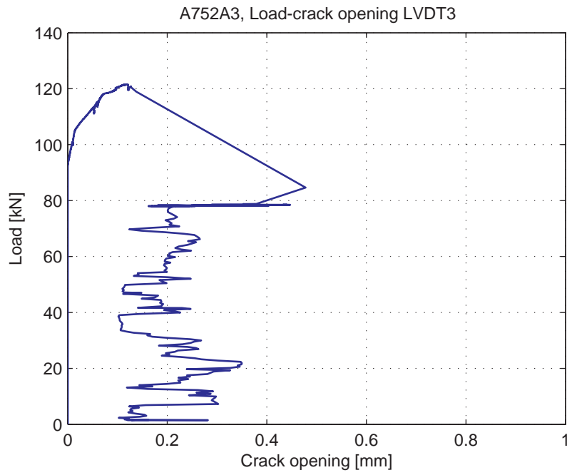
Fig. 5.28.7. Load-Crack opening for LVDT3
