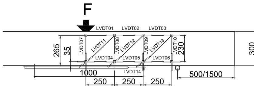
Fig. 5.71.2. LVDT layout and numbering for 300 mm deep beams
