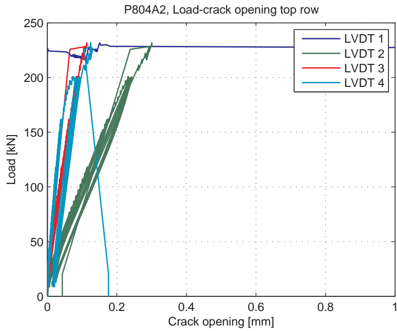
Fig. 5.93.5. Load-Crack opening for LVDT's 1-4 (top row)
