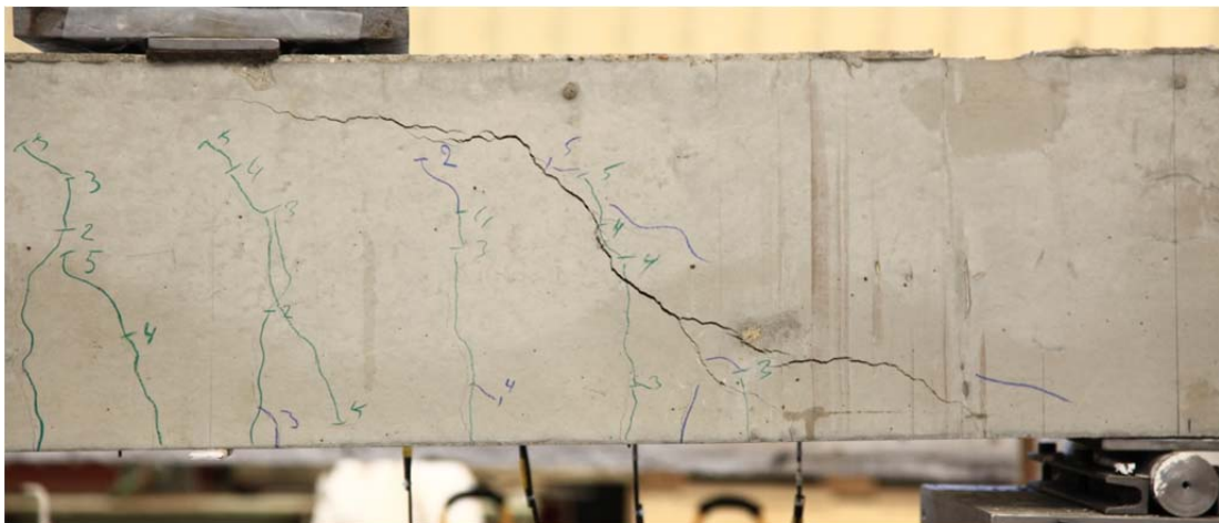
Fig. 5.23.2. Crack pattern after failure south side
