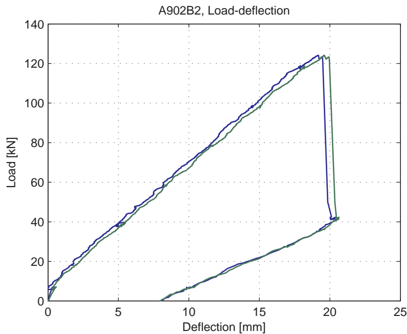
Fig. 5.21.4. Load-deflection curve
