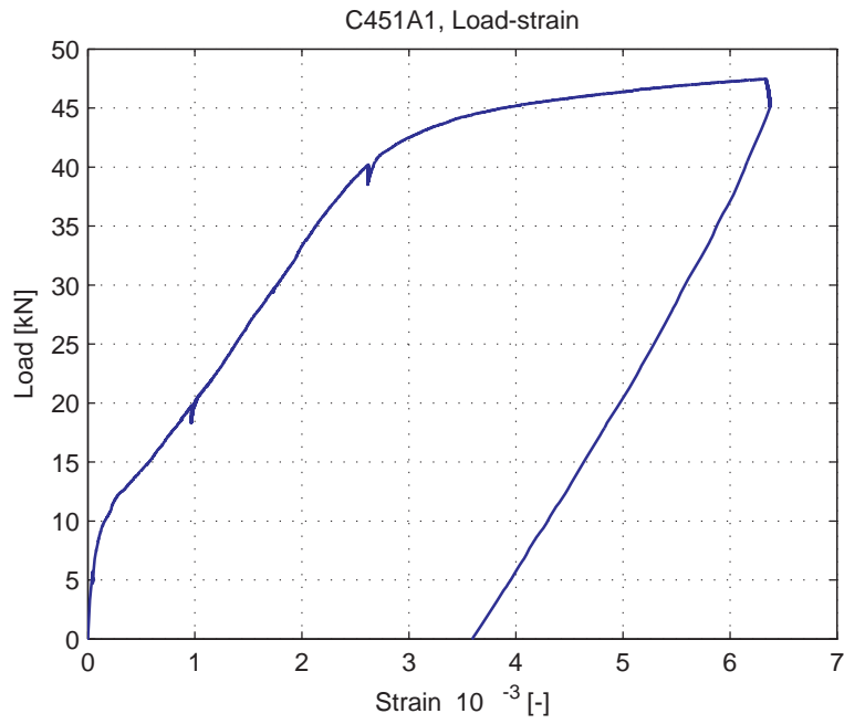
Fig. 5.62.5. Average strain over 1m length, measured at bottom of specimen (LVDT 3)
