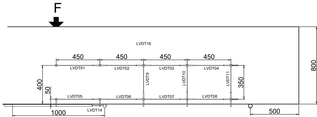
Fig. 5.92.3. LVDT layout and numbering for P804A1 beam
