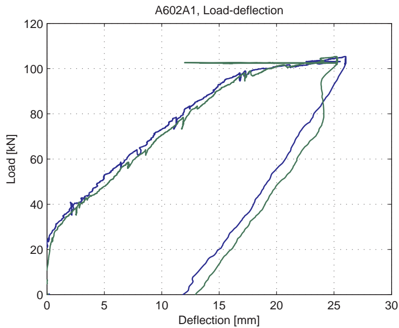
Fig. 5.35.4. Load-deflection curve
