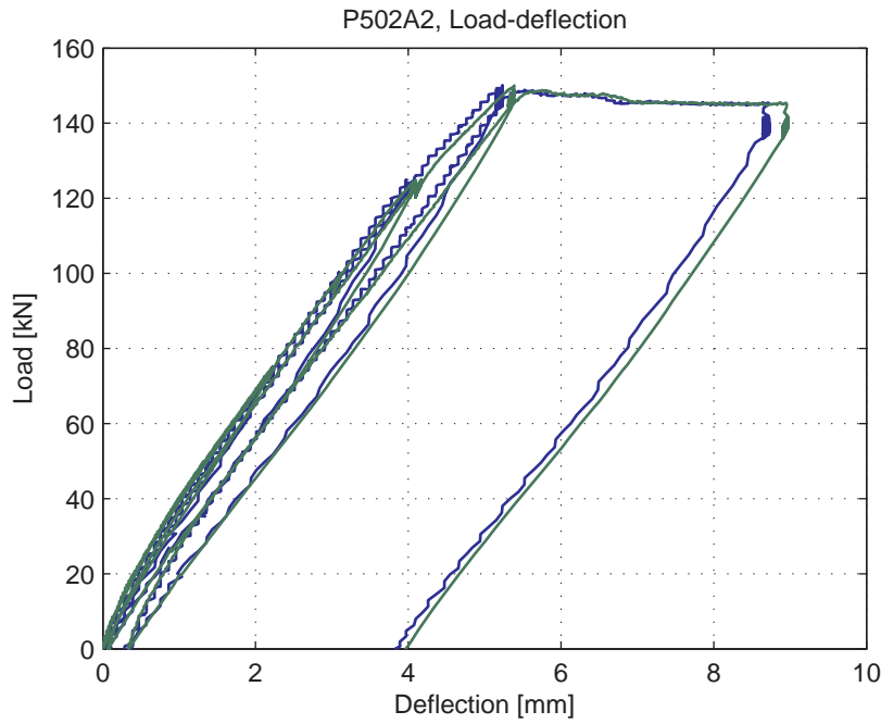
Fig. 5.81.5. Load-deflection curve
