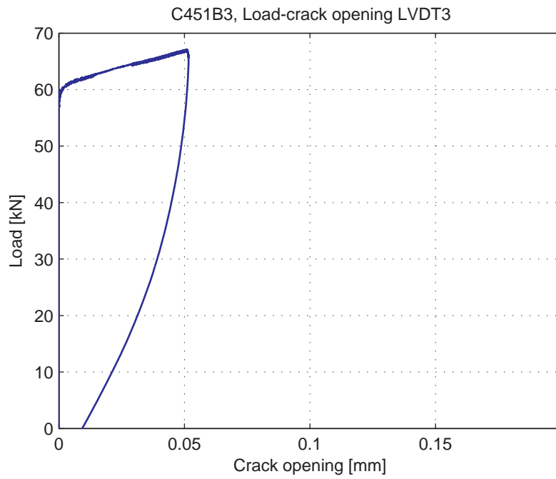
Fig. 5.69.5. Load-Crack opening for LVDT3
