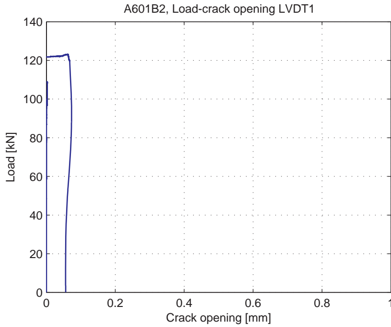
Fig. 5.34.5. Load-Crack opening for LVDT1
