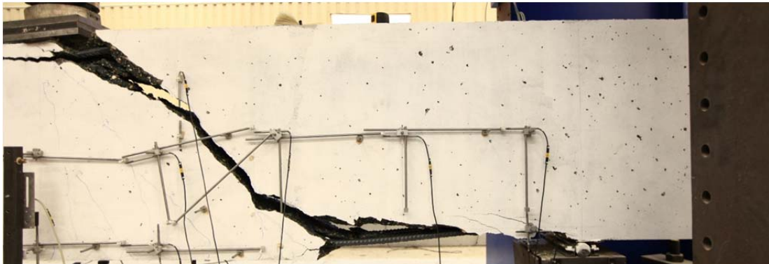
Fig. 5.100.2. Crack pattern after failure south side
