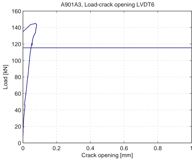
Fig. 5.14.9. Load-Crack opening for LVDT6
