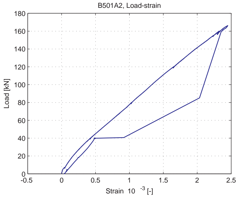
Fig. 5.48.5. Average strain over 1m length, measured at bottom of specimen (LVDT 3)
