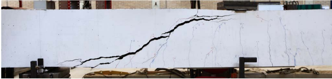
Fig. 5.48.1. Crack pattern after failure north side
