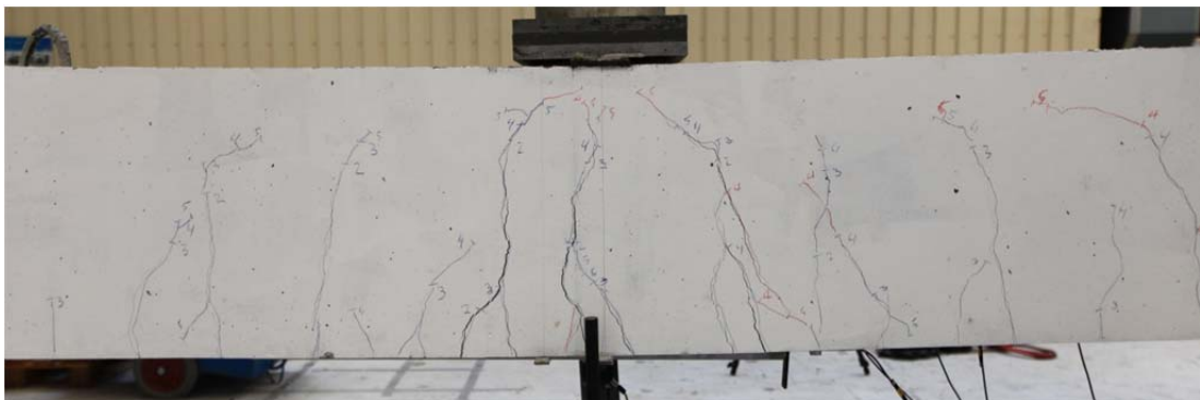
Fig. 5.51.2. Crack pattern after failure south side
