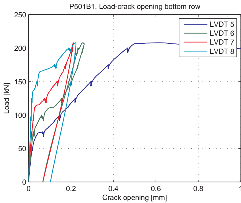
Fig. 5.78.8. Load-Crack opening for LVDT's 5-8 (bottom row)
