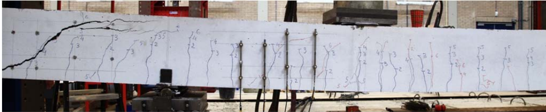
Fig. 5.18.1. Crack pattern after failure north side
