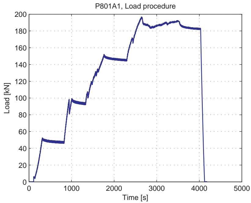
Fig. 5.83.3. Load-Time curve
