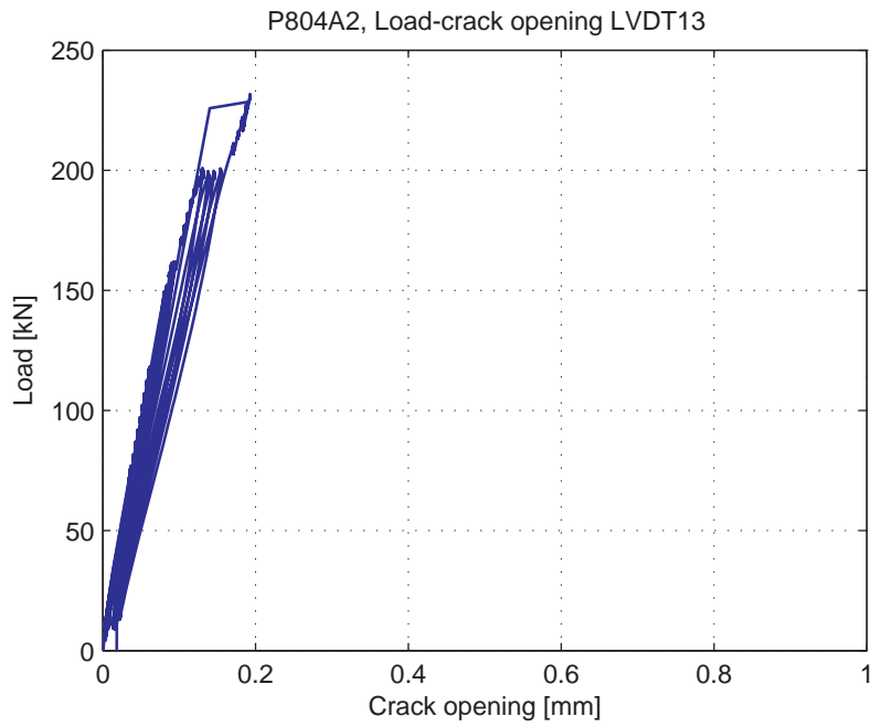
Fig. 5.93.9. Load-Crack opening for LVDT 13
