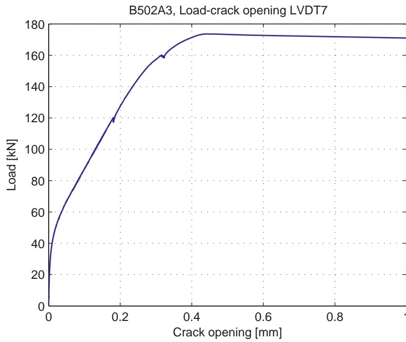
Fig. 5.52.8. Load-Crack opening for LVDT7
