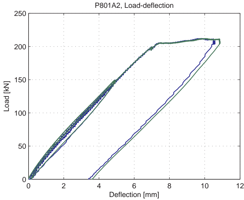
Fig. 5.84.4. Load-deflection curve
