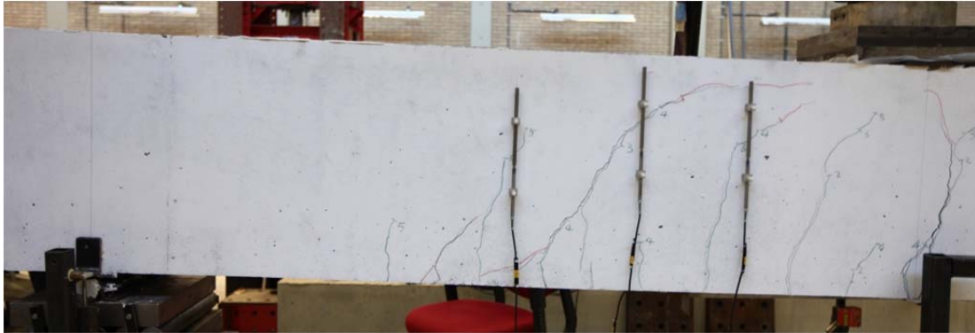
Fig. 5.42.1. Crack pattern after failure north side
