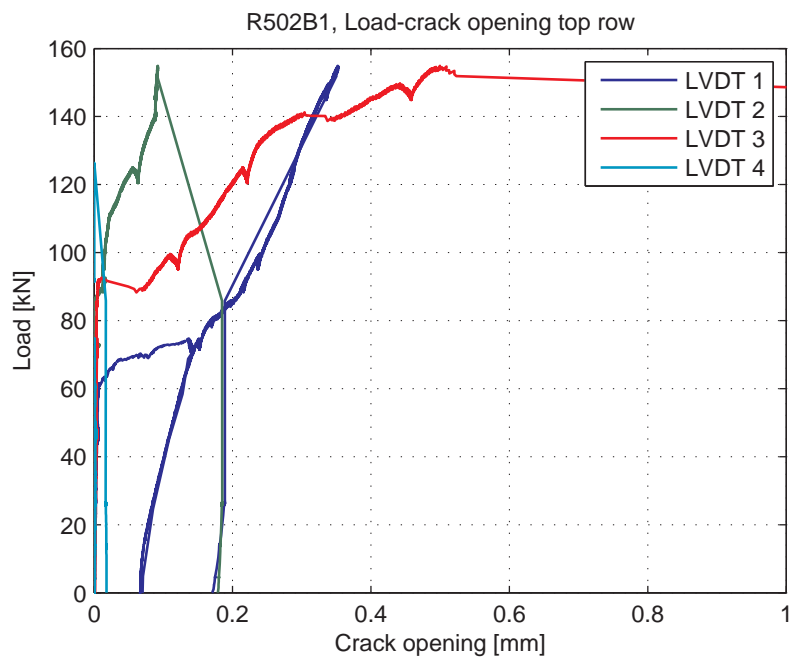
Fig. 5.99.6. Load-Crack opening for LVDT's 1-4 (top row)
