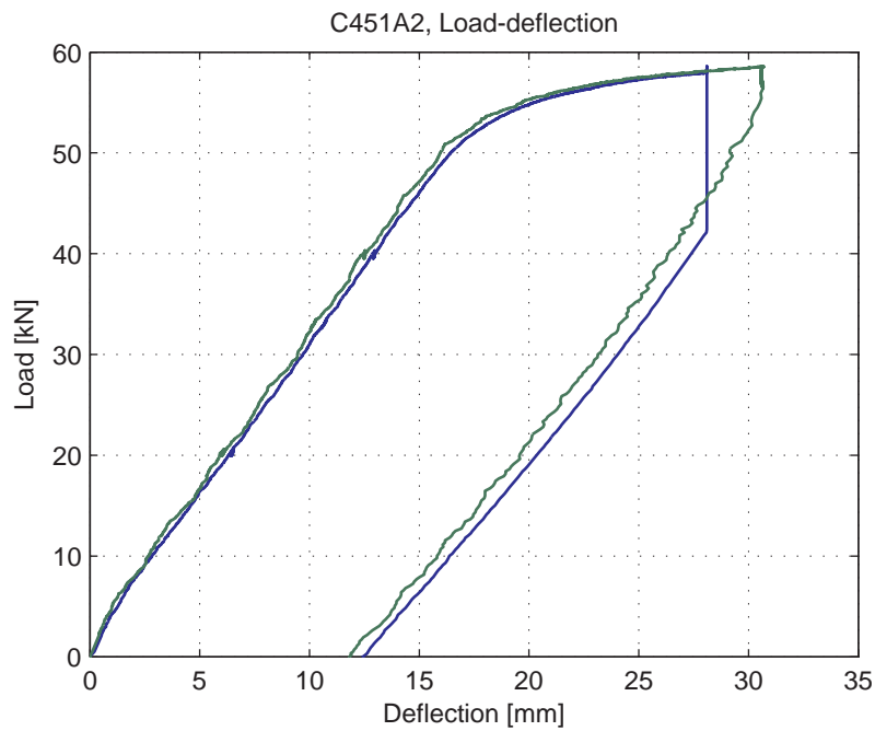
Fig. 5.63.4. Load-deflection curve
