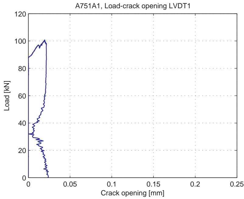
Fig. 5.22.5. Load-Crack opening for LVDT1
