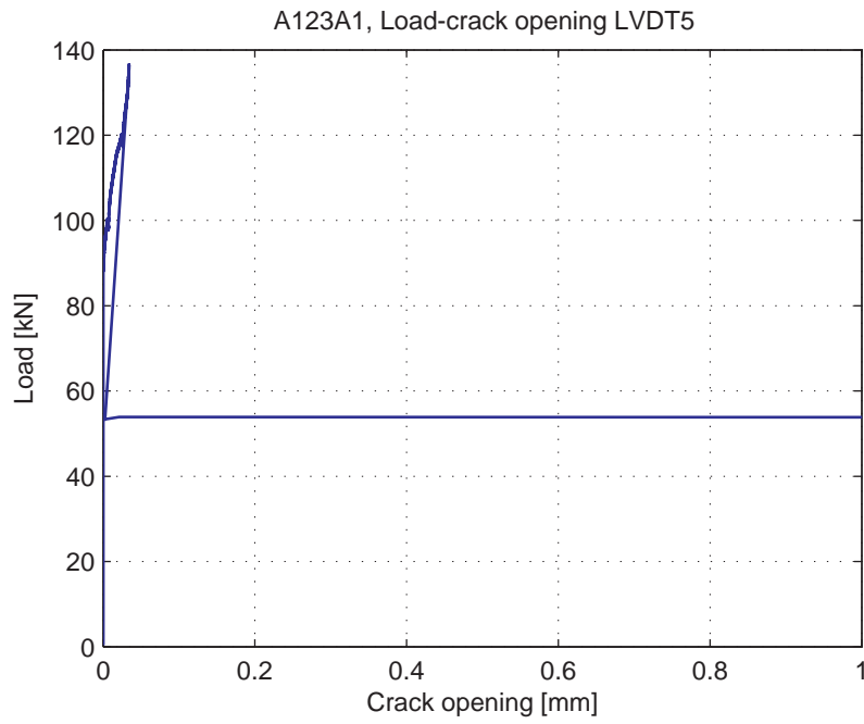
Fig. 5.8.6. Load-Crack opening for LVDT5
