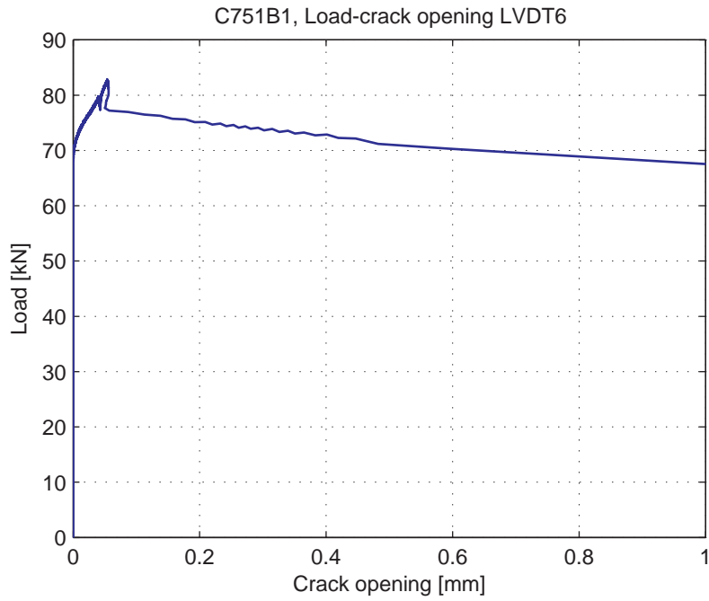
Fig. 5.61.7. Load-Crack opening for LVDT6
