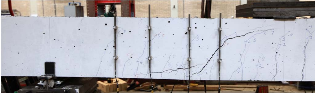
Fig. 5.11.1. Crack pattern after failure north side
