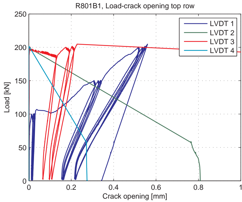
Fig. 5.101.6. Load-Crack opening for LVDT's 1-4 (top row)
