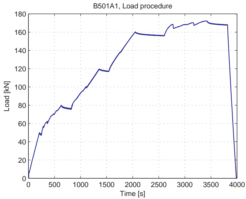
Fig. 5.47.3. Load-Time curve
