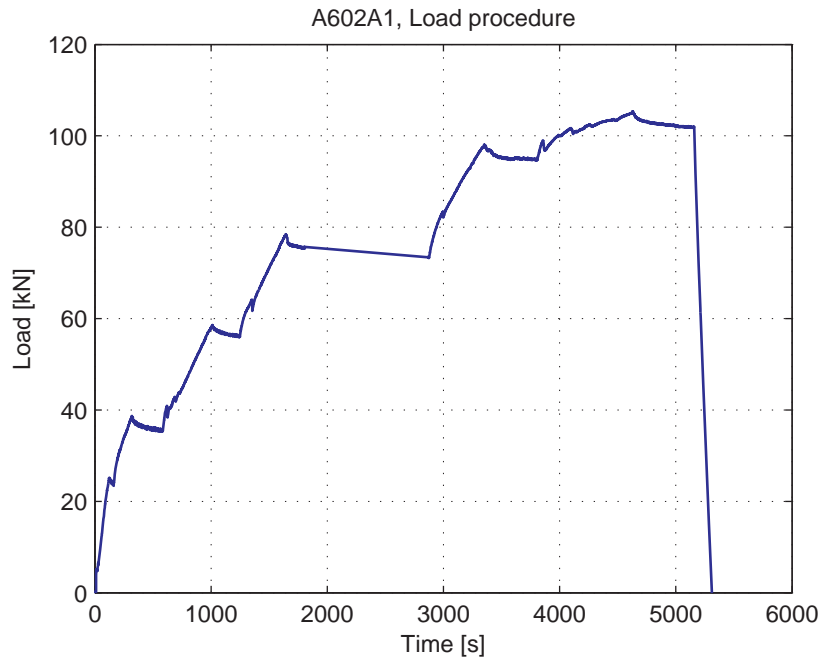
Fig. 5.35.3. Load-Time curve
