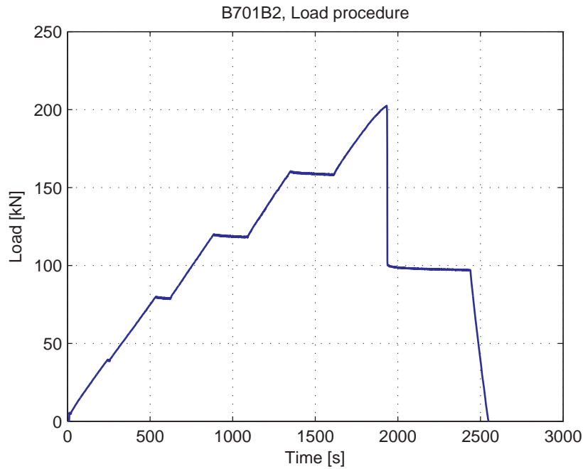
Fig. 5.44.3. Load-Time curve
