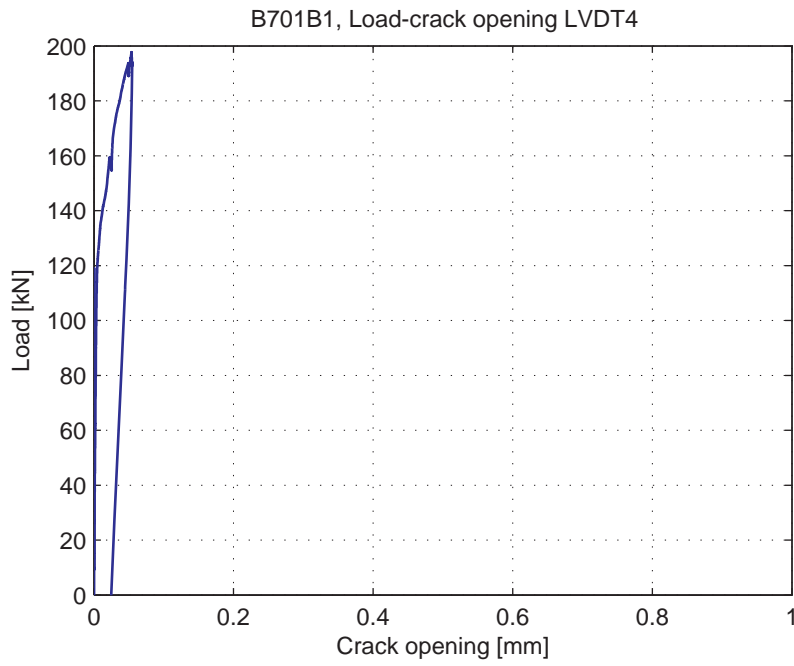
Fig. 5.43.5. Load-Crack opening for LVDT4
