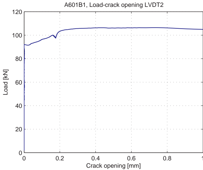
Fig. 5.33.6. Load-Crack opening for LVDT2
