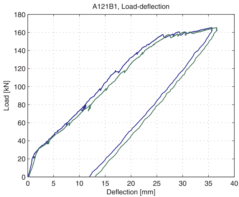
Fig. 5.4.4. Load-deflection curve
