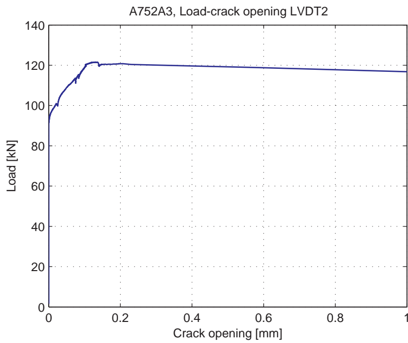
Fig. 5.28.6. Load-Crack opening for LVDT2
