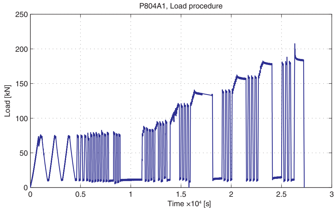
Fig. 5.92.4. Load-Time curve
