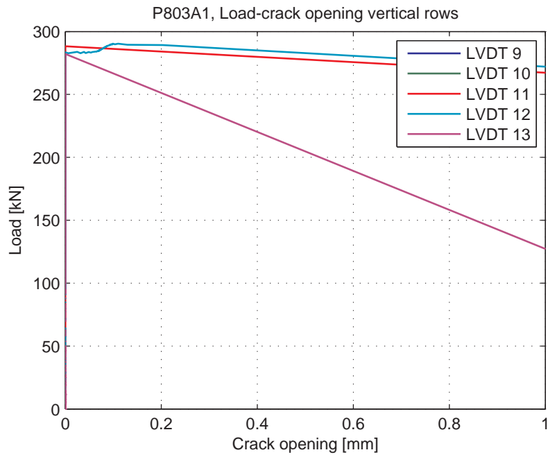
Fig. 5.89.7. Load-Crack opening for LVDT's 9-13 (vertical LVDT's)
