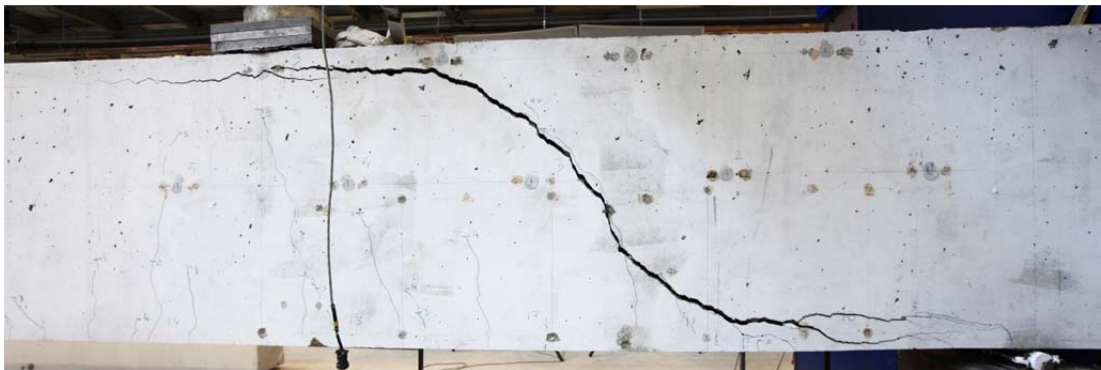
Fig. 5.101.2. Crack pattern after failure west side
