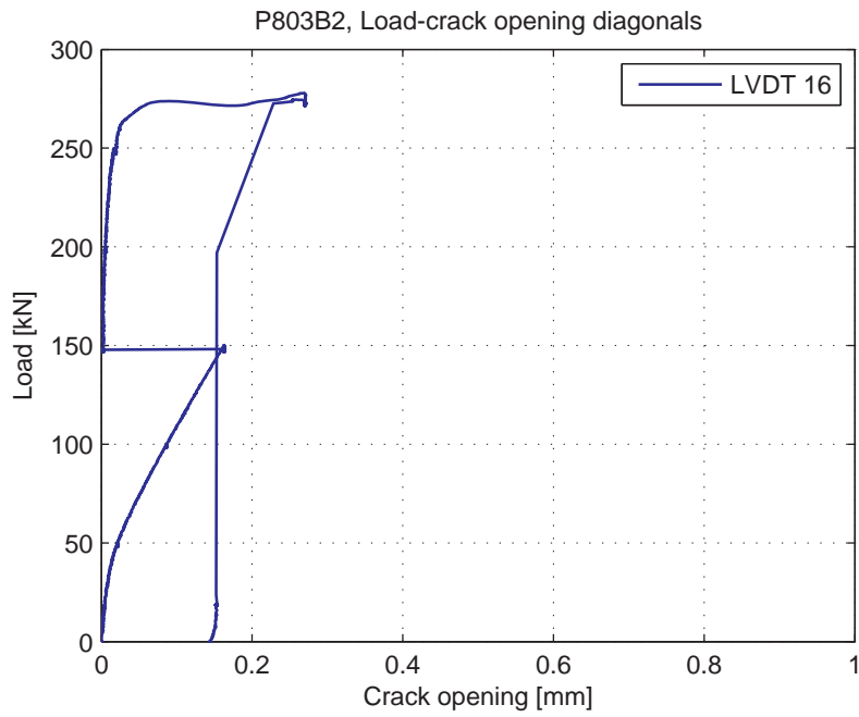
Fig. 5.91.9. Load-Crack opening for LVDT 16 (diagonal)
