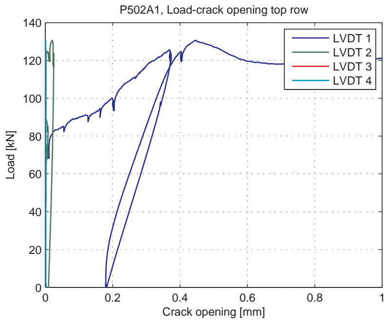
Fig. 5.80.6. Load-Crack opening for LVDT's 1-4 (top row)
