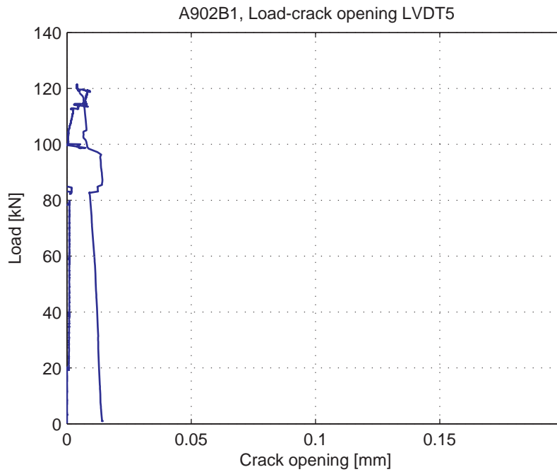
Fig. 5.20.8. Load-Crack opening for LVDT5
