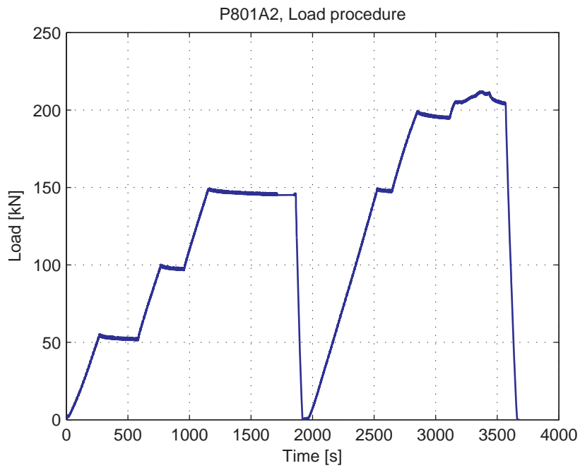
Fig. 5.84.3. Load-Time curve
