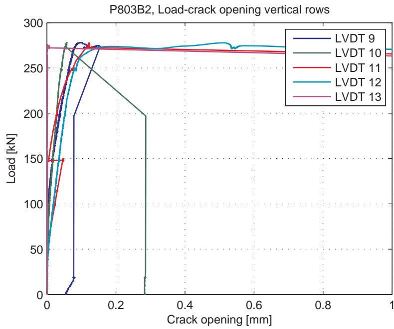
Fig. 5.91.7. Load-Crack opening for LVDT's 9-13 (vertical LVDT's)
