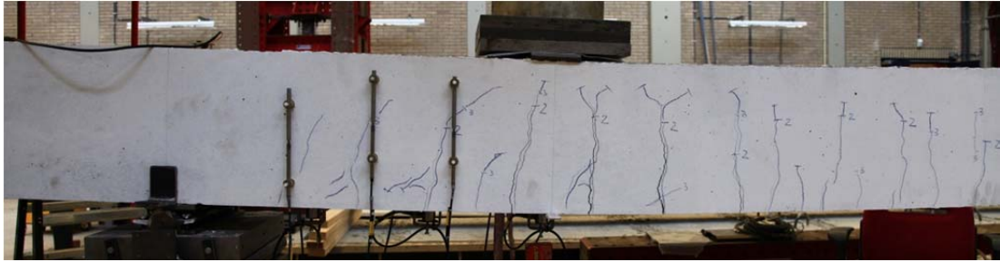
Fig. 5.29.1. Crack pattern after failure north side
