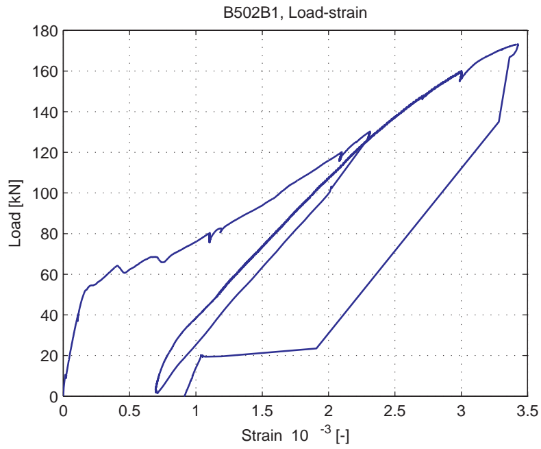
Fig. 5.53.9. Average strain over 1m length, measured at bottom of specimen (LVDT 3)
