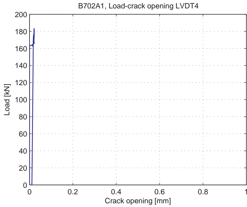
Fig. 5.45.5. Load-Crack opening for LVDT4
