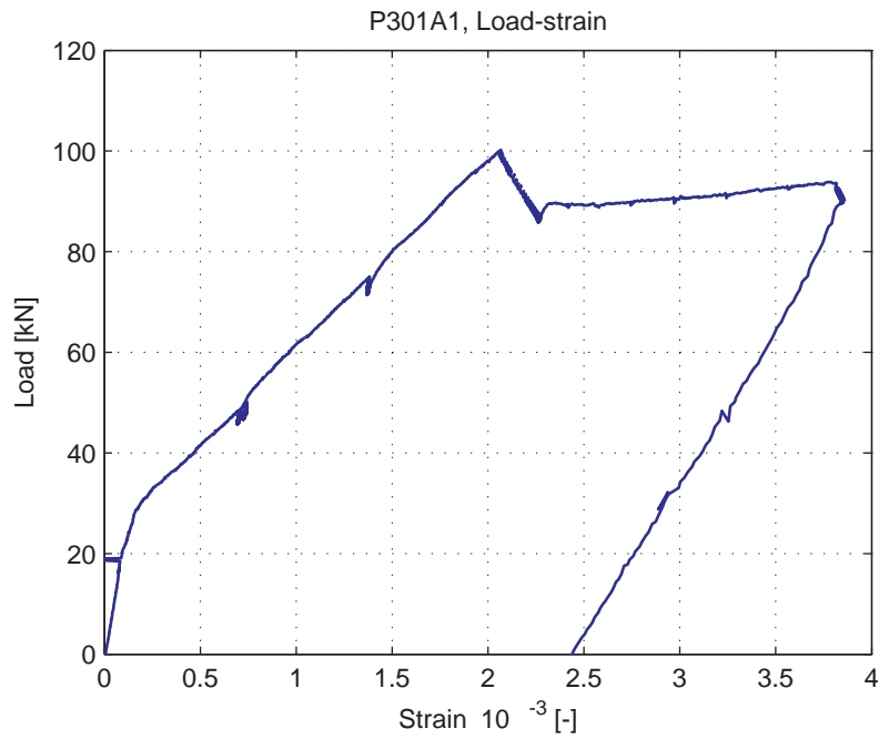
Fig. 5.71.9. Average strain over 1m length, measured at bottom of specimen (LVDT 14)
