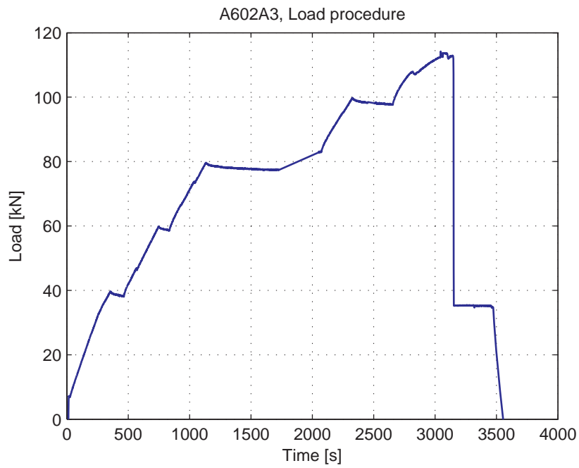
Fig. 5.37.3. Load-Time curve
