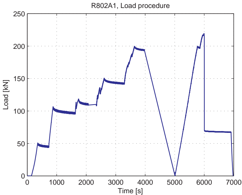
Fig. 5.102.4. Load-Time curve
