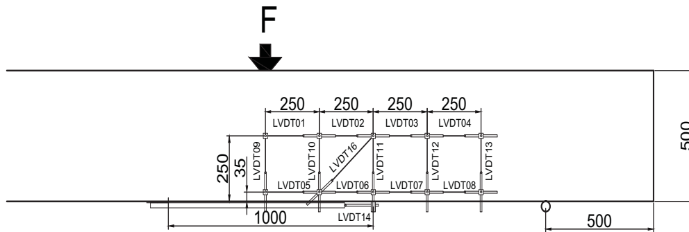
Fig. 5.99.3. LVDT layout and numbering for 500 mm deep beams
