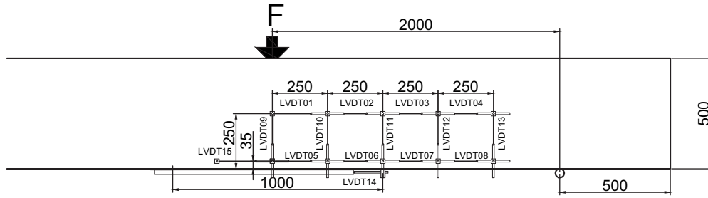
Fig. 5.79.3. LVDT layout and numbering for 500 mm deep beams (
