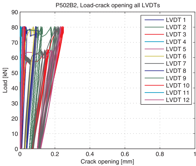
Fig. 5.82.11. Load-Crack opening second part of test for all LVDT's
