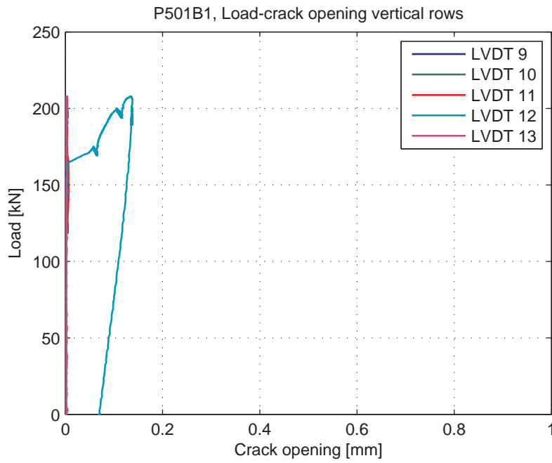
Fig. 5.78.7. Load-Crack opening for LVDT's 9-13 (vertical LVDT's)
