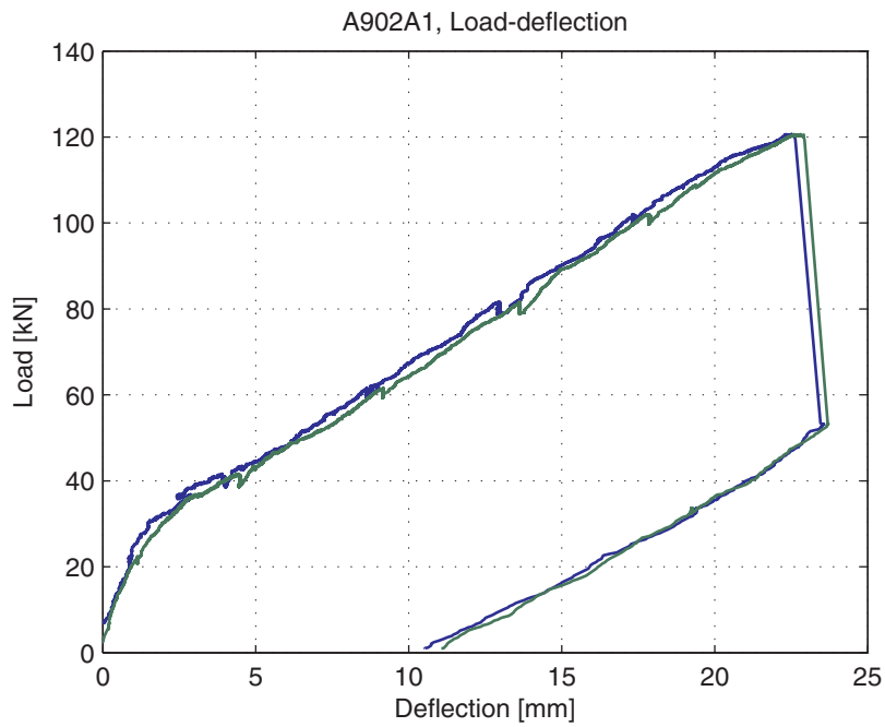
Fig. 5.17.4. Load-deflection curve
