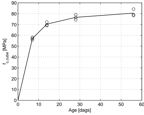
Fig. 2.2.11. F_{c,cube} development for cast 7
