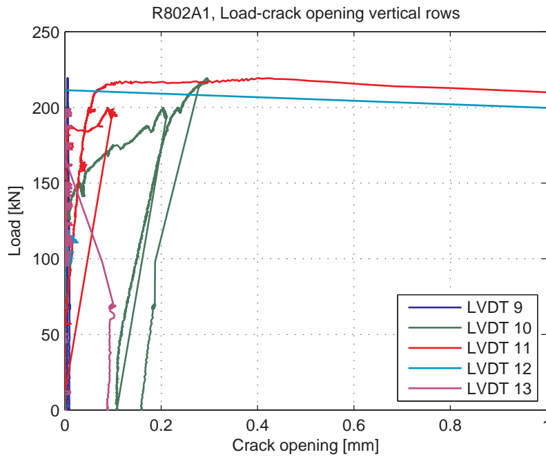
Fig. 5.102.7. Load-Crack opening for LVDT's 9-13 (vertical LVDT's)
