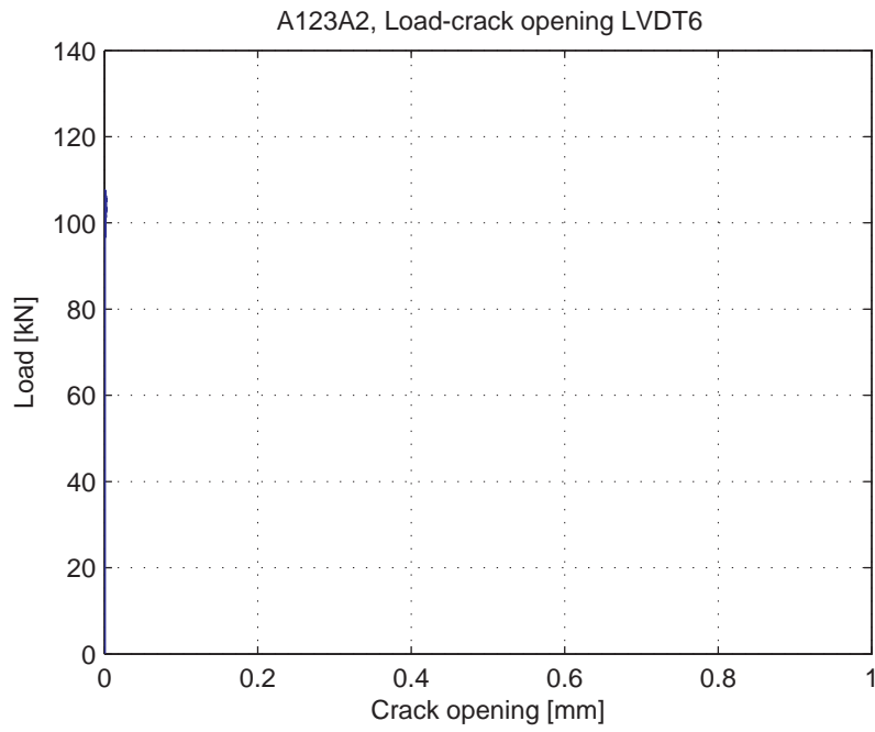
Fig. 5.9.7. Load-Crack opening for LVDT6
