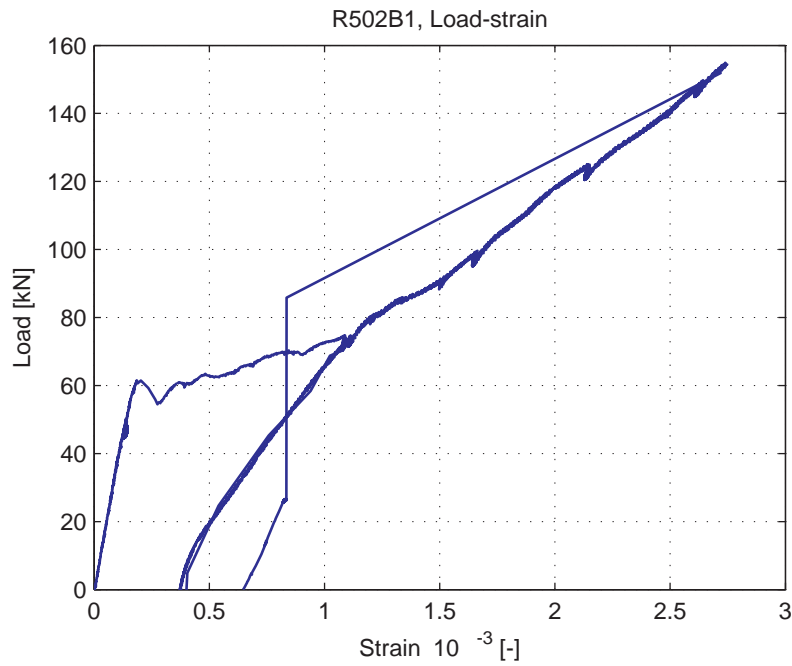
Fig. 5.99.11. Average strain over 1m length, measured at bottom of specimen (LVDT 14)
