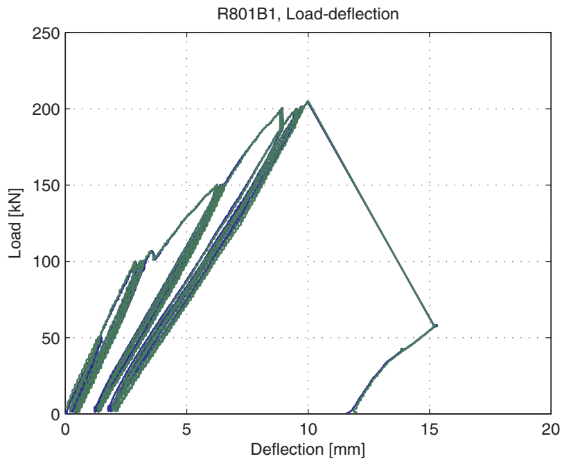
Fig. 5.101.5. Load-deflection curve
