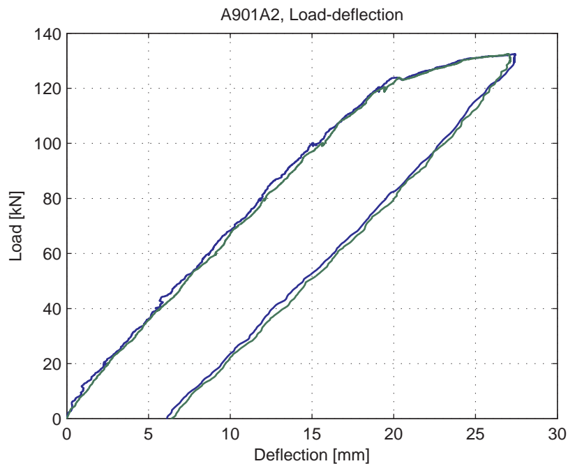
Fig. 5.13.4. Load-deflection curve
