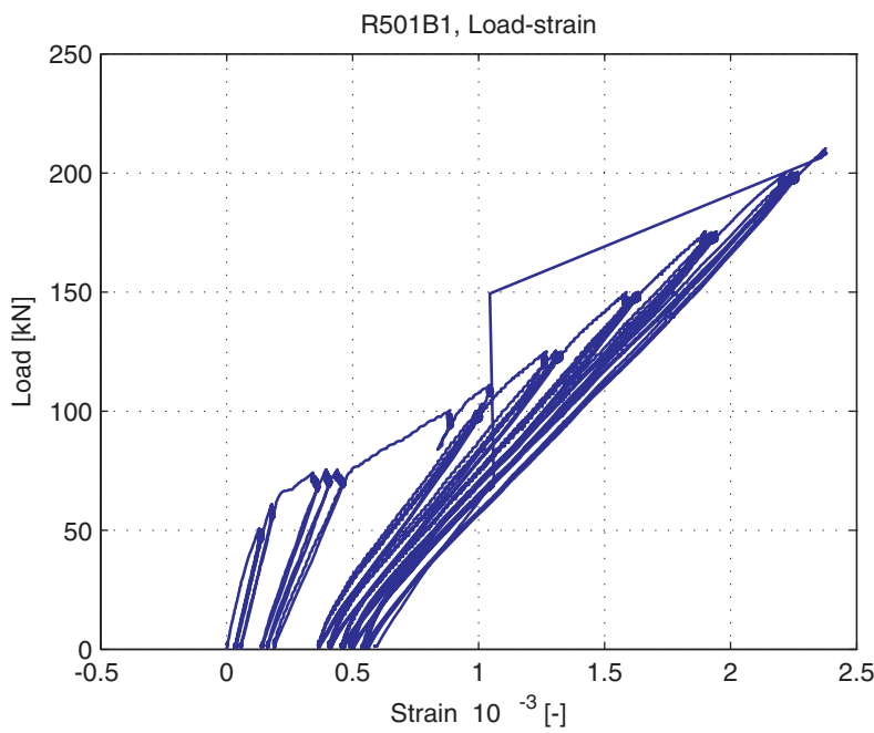
Fig. 5.96.7. Average strain over 1m length, measured at bottom of specimen (LVDT 10)
