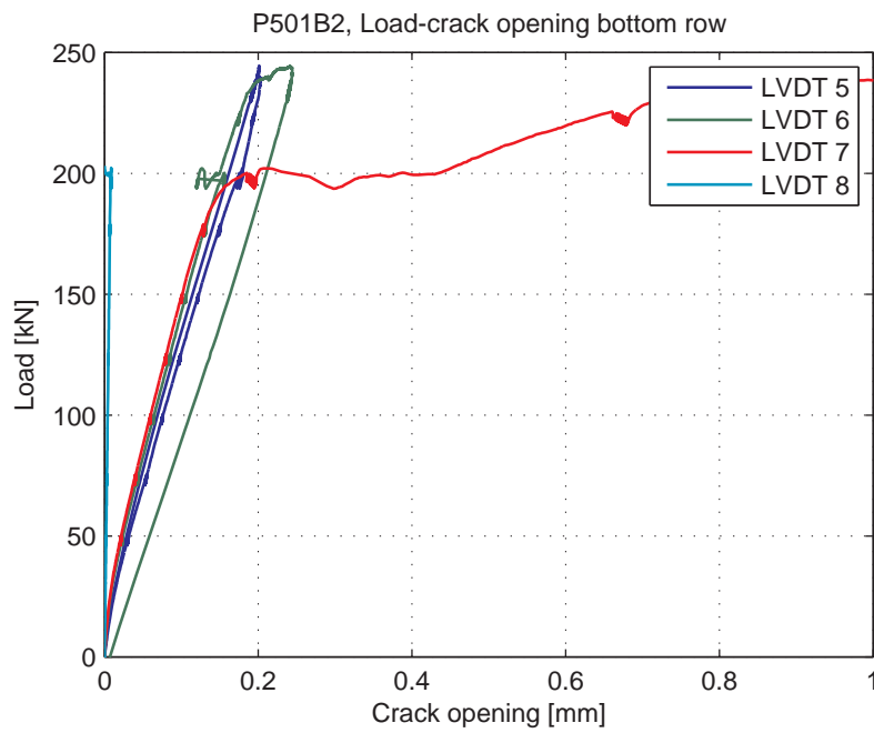
Fig. 5.79.8. Load-Crack opening for LVDT's 5-8 (bottom row)
