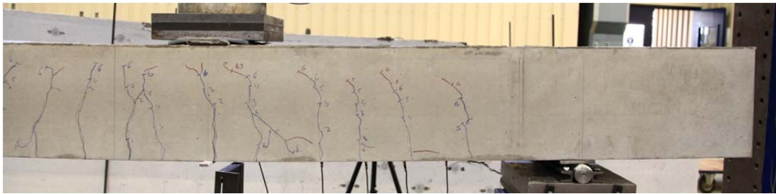
Fig. 5.13.2. Crack pattern after failure south side
