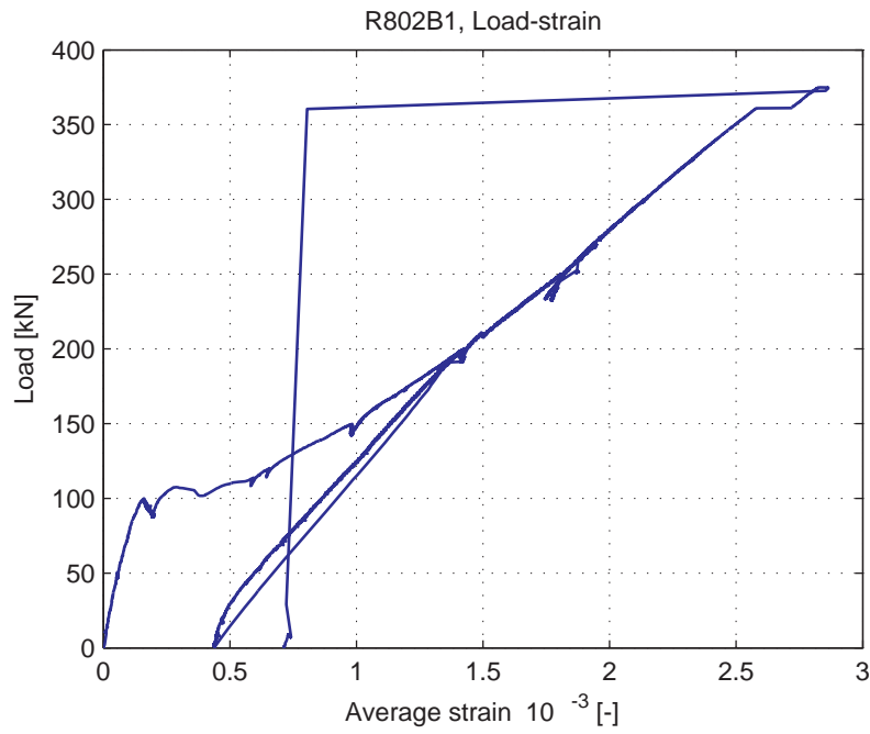
Fig. 5.103.11. Average strain over 1m length, measured at bottom of specimen (LVDT 14)
