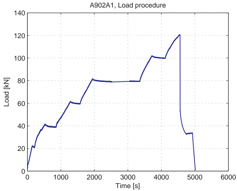
Fig. 5.17.3. Load-Time curve
