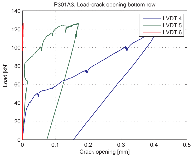
Fig. 5.73.8. Load-Crack opening for LVDT's 4-6 (bottom row)
