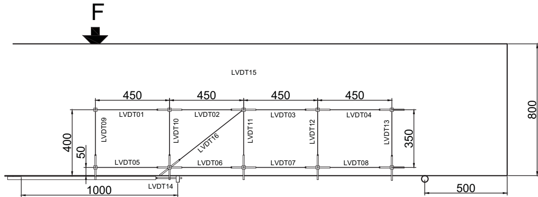
Fig. 5.89.3. LVDT layout and numbering for 800 mm deep beams
