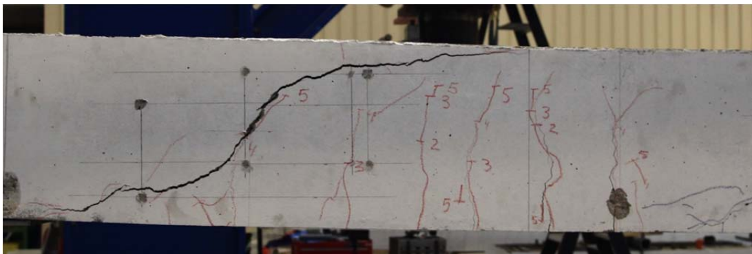
Fig. 5.28.1. Crack pattern after failure north side
