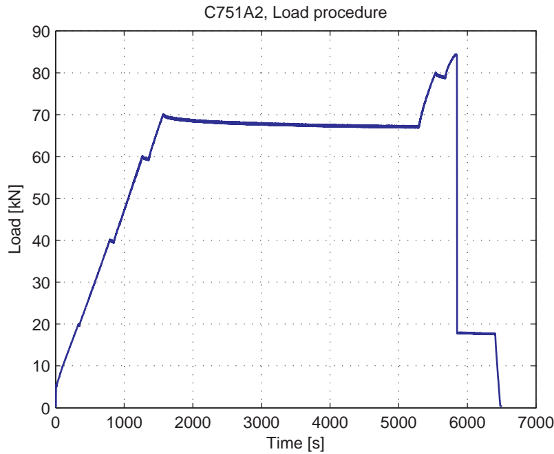
Fig. 5.59.3. Load-Time curve
