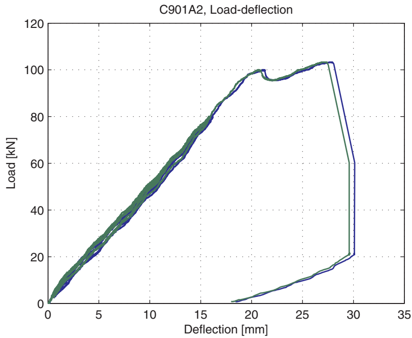
Fig. 5.55.4. Load-deflection curve
