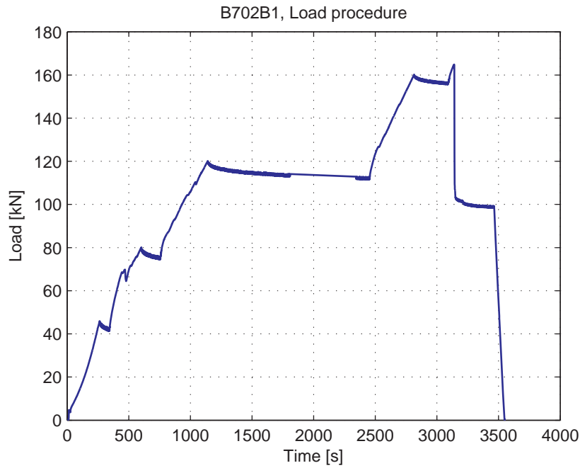
Fig. 5.46.3. Load-Time curve
