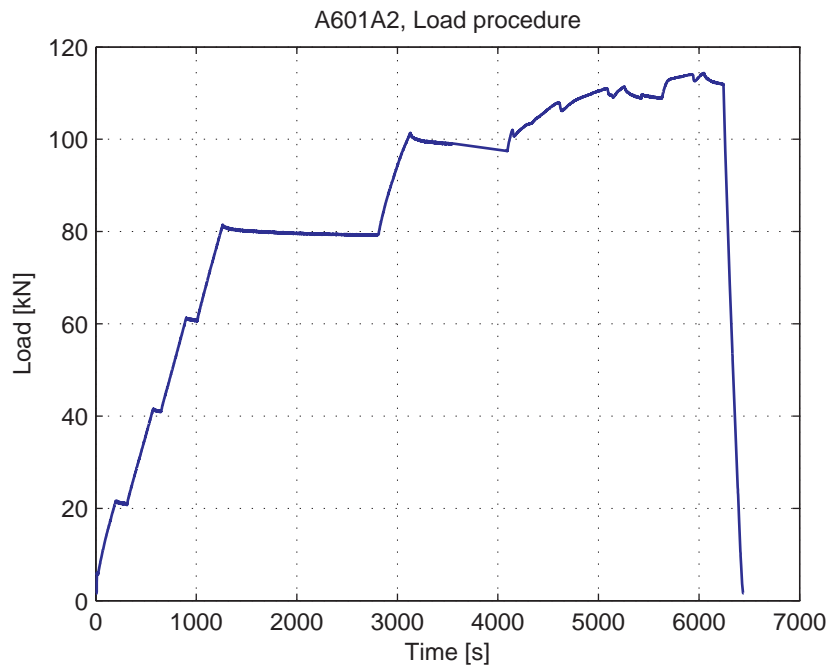
Fig. 5.32.3. Load-Time curve
