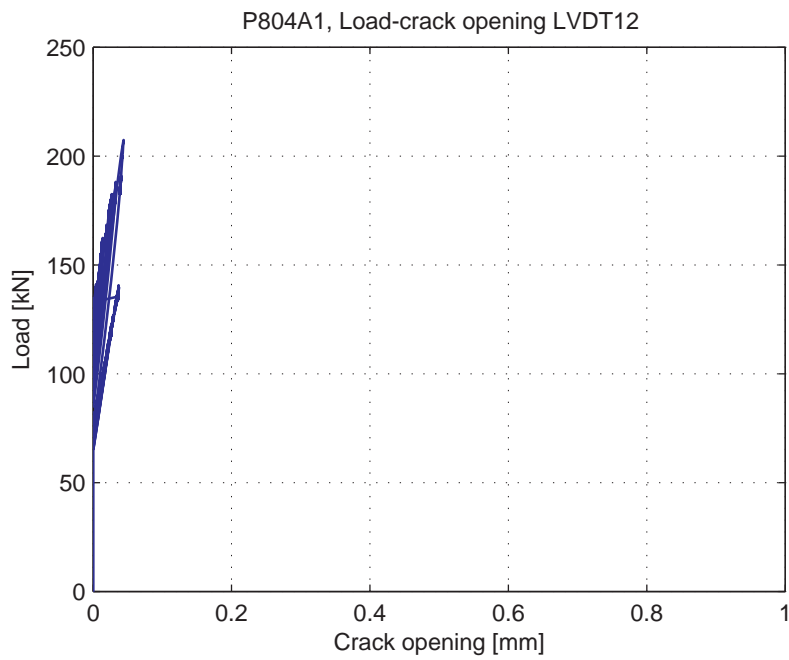
Fig. 5.92.9. Load-Crack opening for LVDT 12
