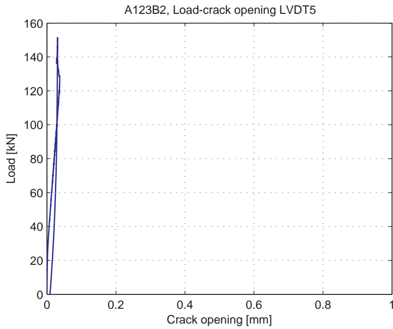
Fig. 5.11.6. Load-Crack opening for LVDT5
