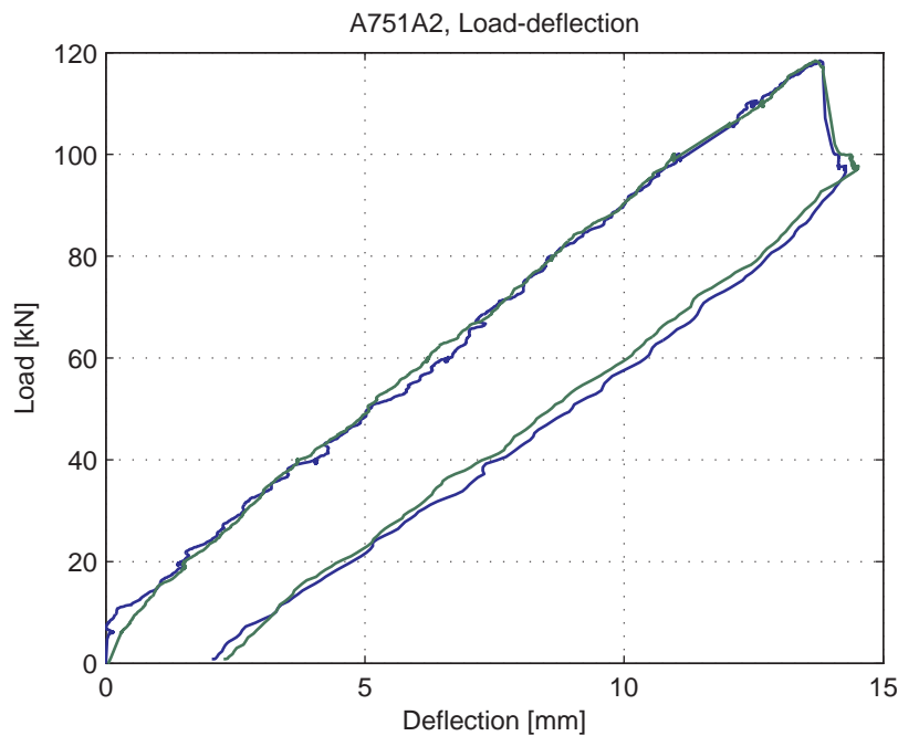
Fig. 5.23.4. Load-deflection curve
