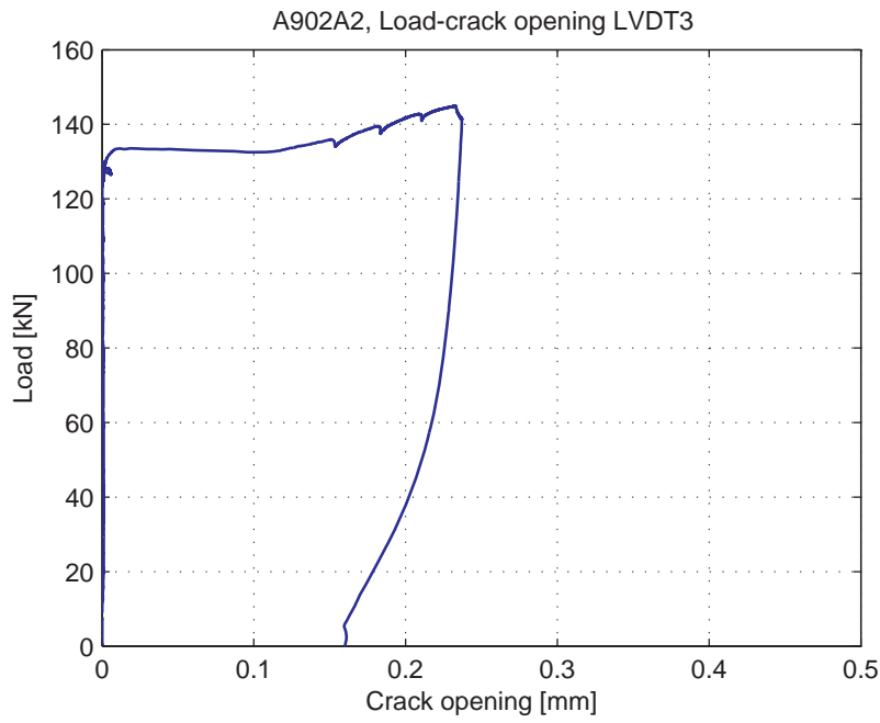
Fig. 5.18.7. Load-Crack opening for LVDT3
