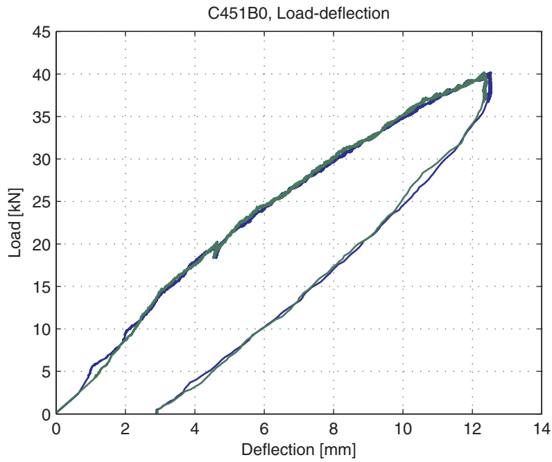
Fig. 5.66.2. Load-deflection curve
