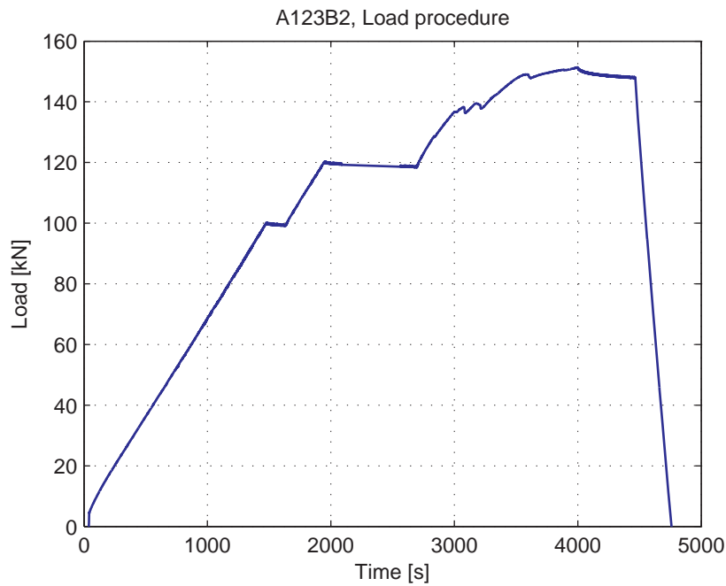
Fig. 5.11.3. Load-Time curve
