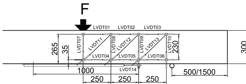
Fig. 5.75.3. LVDT layout and numbering for 300 mm deep beams
