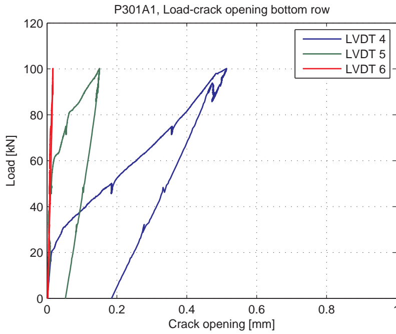
Fig. 5.71.7. Load-Crack opening for LVDT's 4-6 (bottom row)
