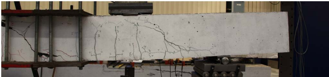
Fig. 5.34.2. Crack pattern after failure south side
