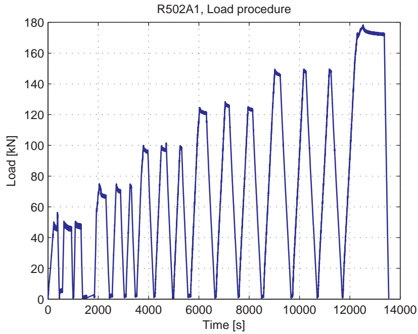
Fig. 5.97.4. Load-Time curve
