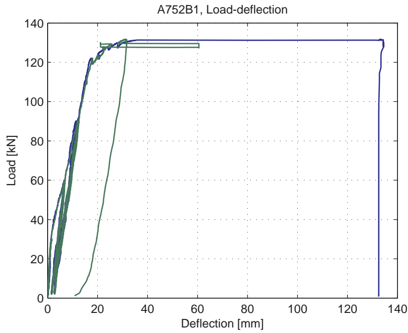
Fig. 5.29.5. Load-deflection curve
