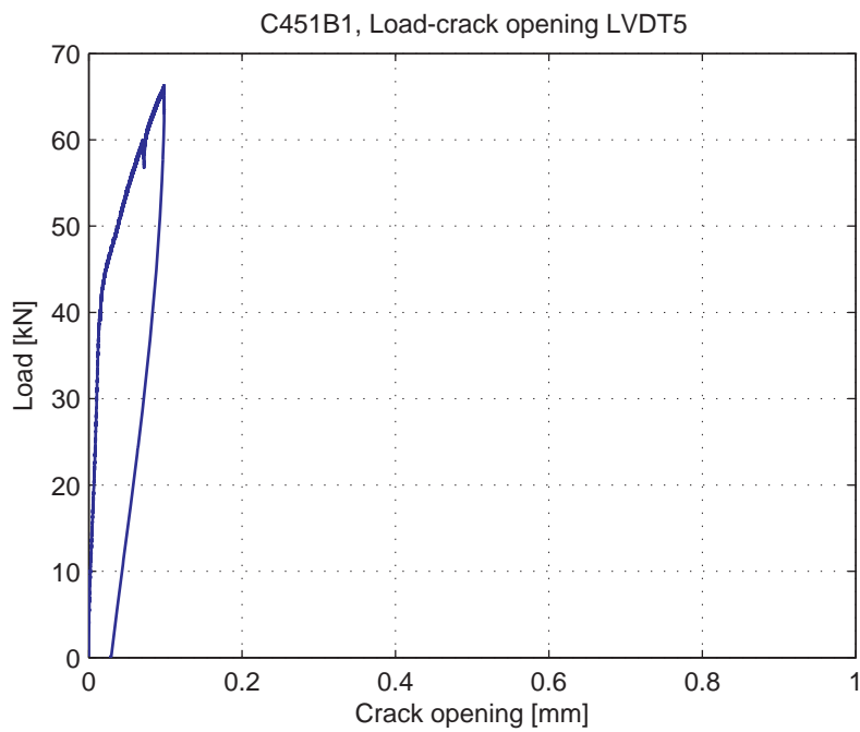
Fig. 5.67.6. Load-Crack opening for LVDT5
