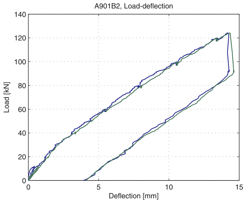
Fig. 5.16.4. Load-deflection curve
