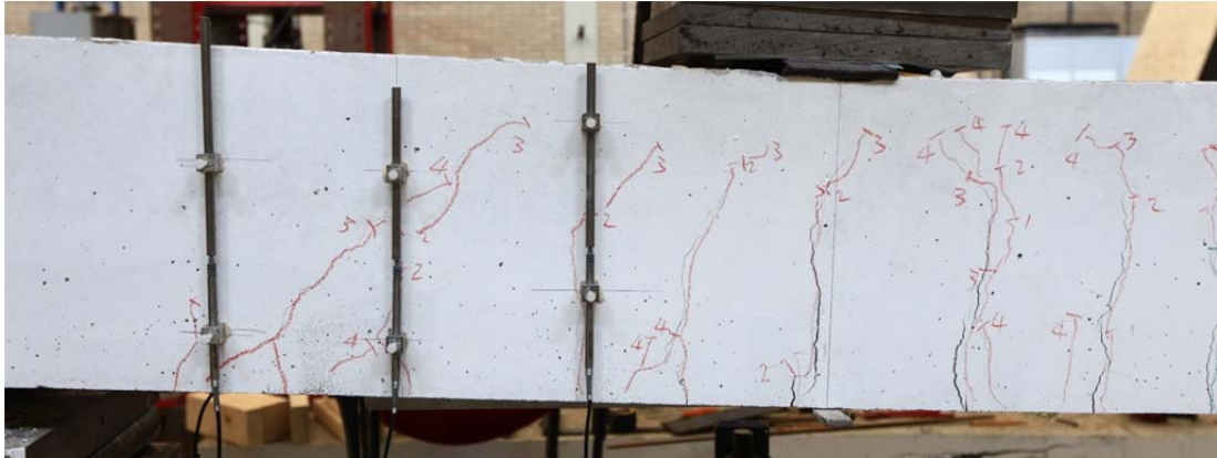
Fig. 5.67.1. Crack pattern after failure north side
