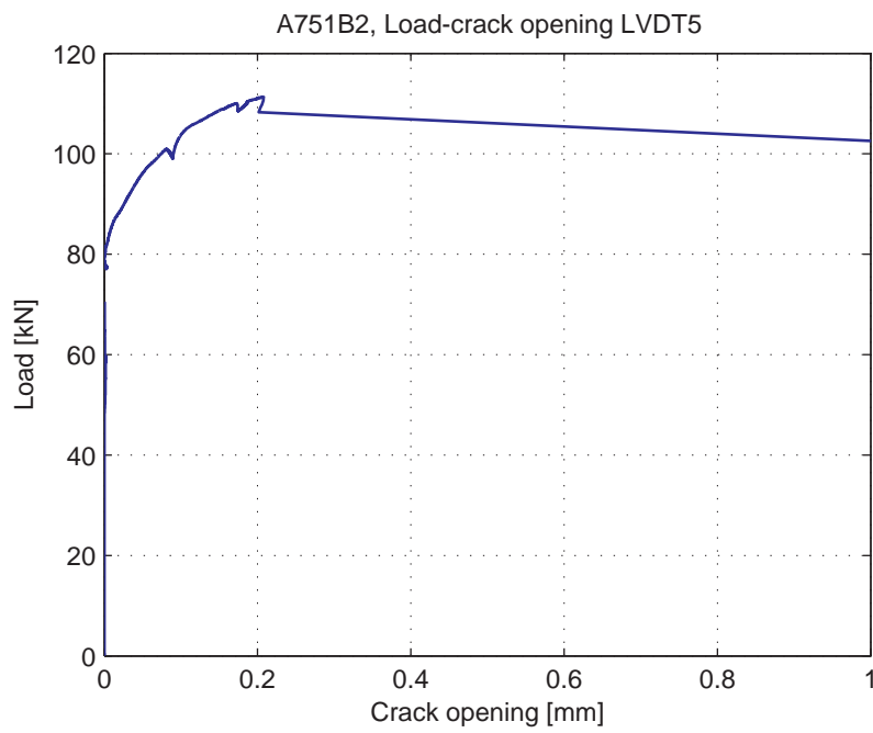
Fig. 5.25.8. Load-Crack opening for LVDT5
