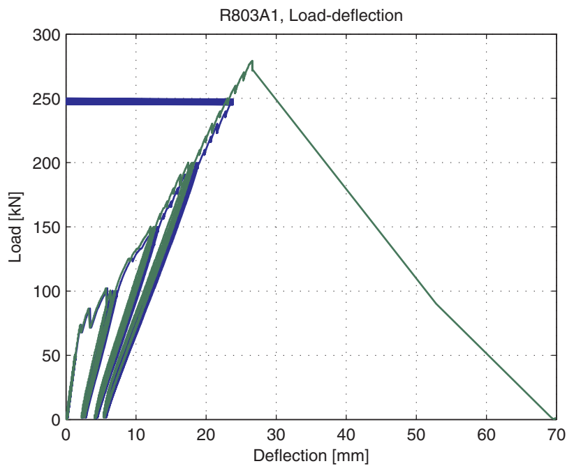
Fig. 5.104.5. Load-deflection curve
