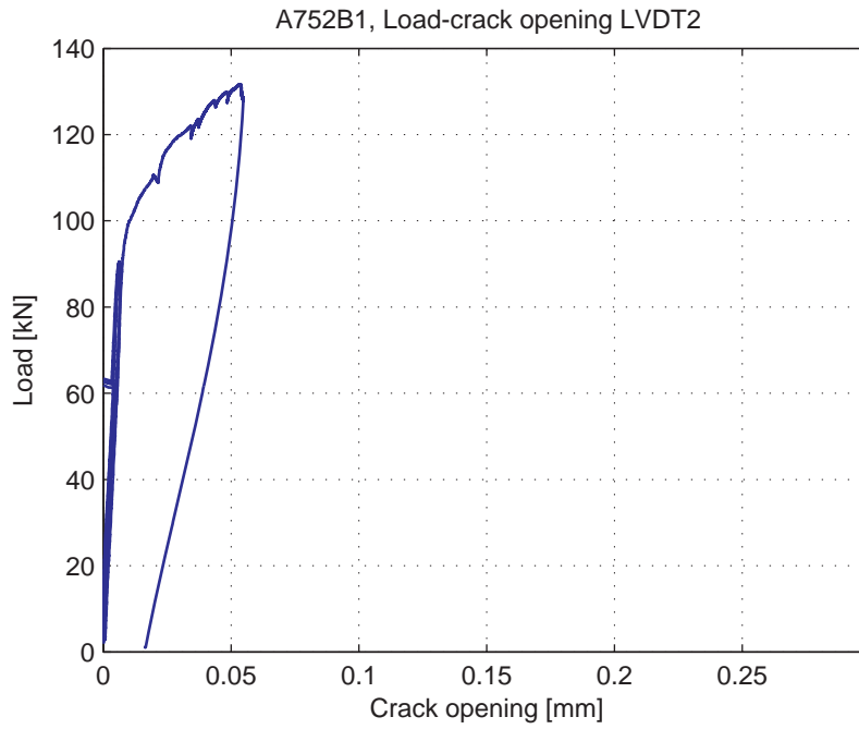
Fig. 5.29.7. Load-Crack opening for LVDT2
