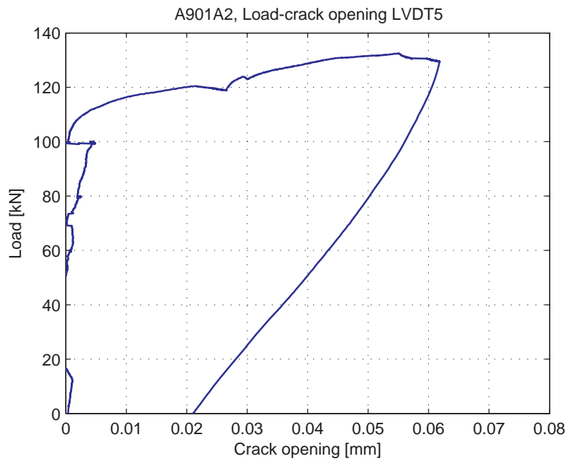
Fig. 5.13.8. Load-Crack opening for LVDT5
