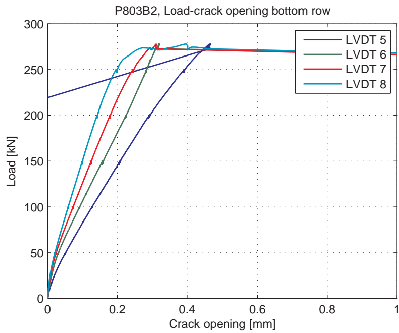
Fig. 5.91.8. Load-Crack opening for LVDT's 5-8 (bottom row)
