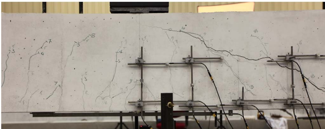
Fig. 5.95.2. Crack pattern after failure south side
