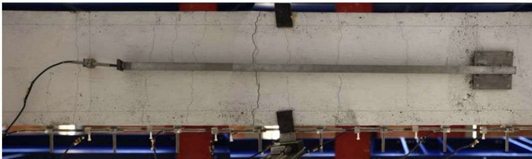
Fig. 3.2.2. Elongation measurement of bottom fibre of specimen using 1m steel rod and LVDT
