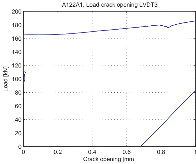
Fig. 5.5.7. Load-Crack opening for LVDT3
