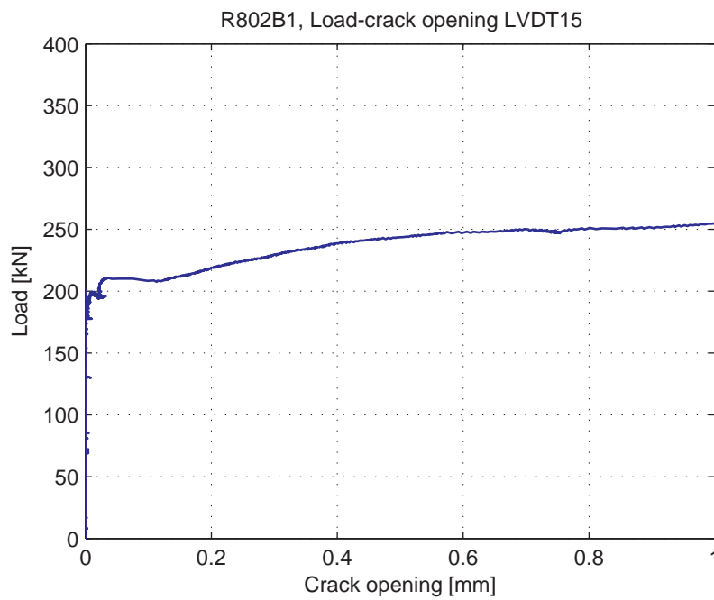
Fig. 5.103.10. Load-Crack opening for LVDT 15
