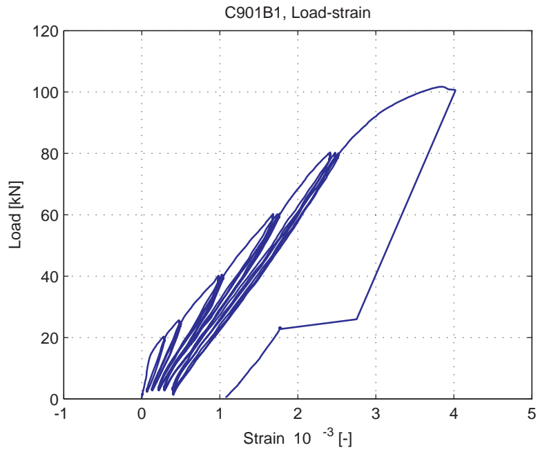
Fig. 5.57.11. Average strain over 1m length, measured at bottom of specimen (LVDT 3)
