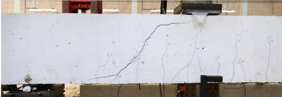
Fig. 5.45.1. Crack pattern after failure north side
