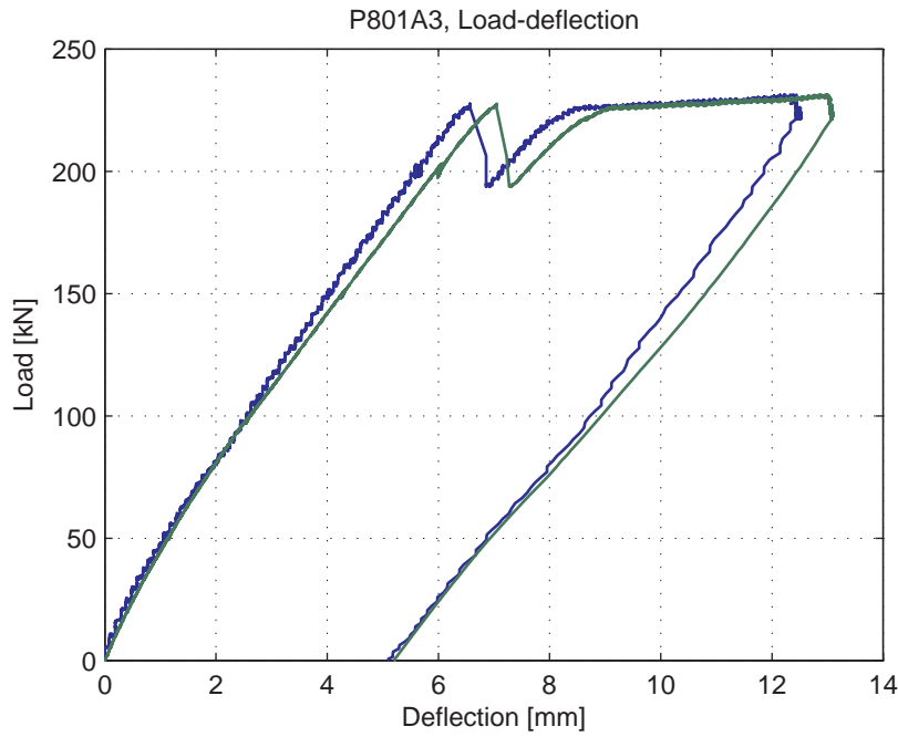
Fig. 5.85.5. Load-deflection curve
