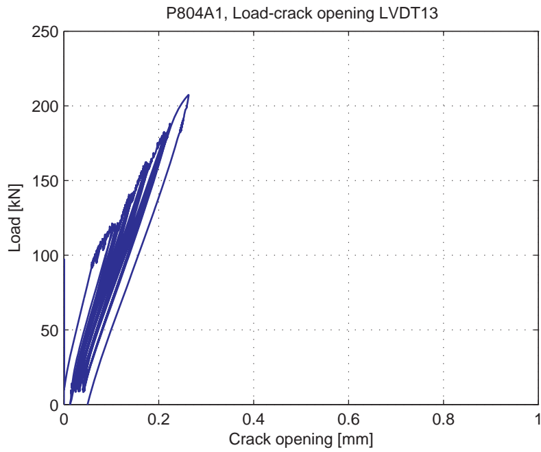
Fig. 5.92.10. Load-Crack opening for LVDT 13
