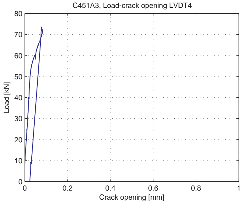
Fig. 5.64.5. Load-Crack opening for LVDT4
