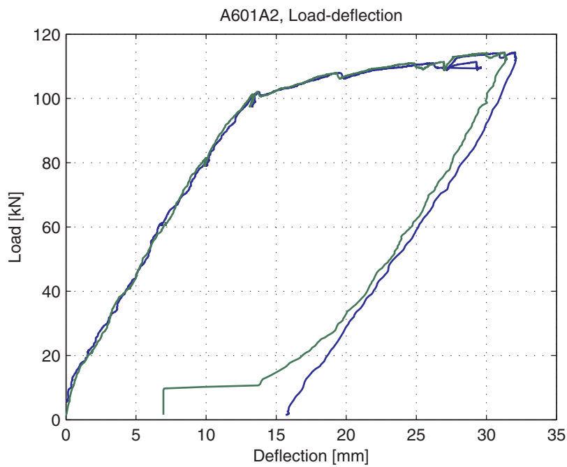
Fig. 5.32.4. Load-deflection curve
