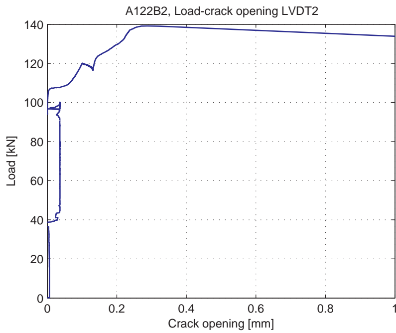
Fig. 5.7.6. Load-Crack opening for LVDT2
