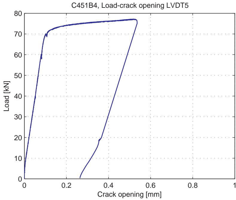
Fig. 5.70.7. Load-Crack opening for LVDT5
