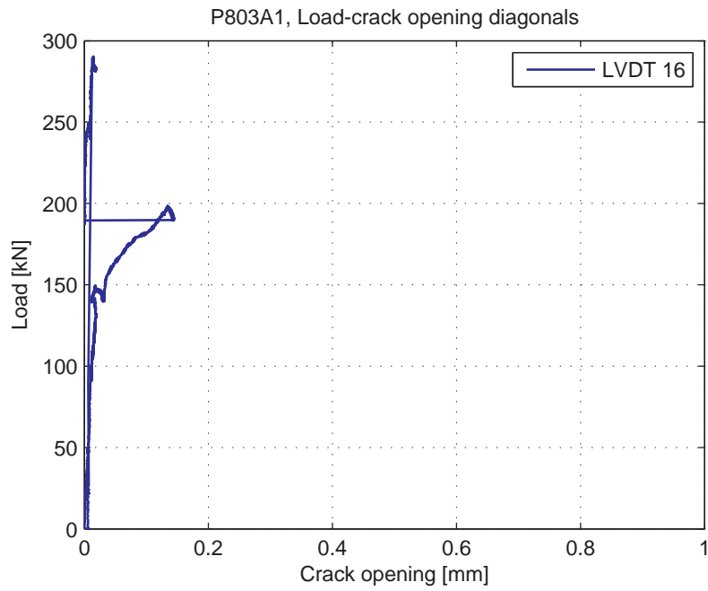
Fig. 5.89.9. Load-Crack opening for LVDT 16 (diagonal)
