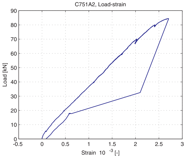
Fig. 5.59.8. Average strain over 1m length, measured at bottom of specimen (LVDT 3)
