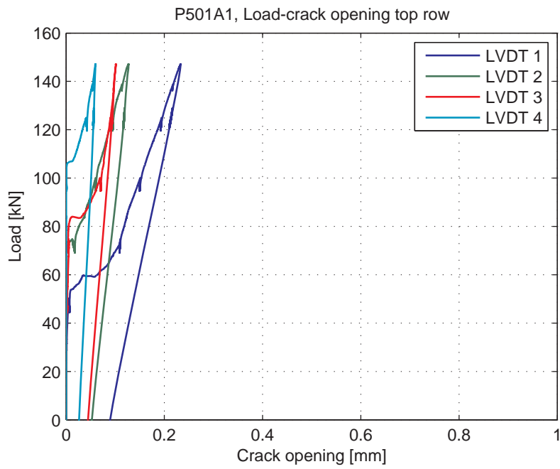
Fig. 5.76.6. Load-Crack opening for LVDT's 1-4 (top row)
