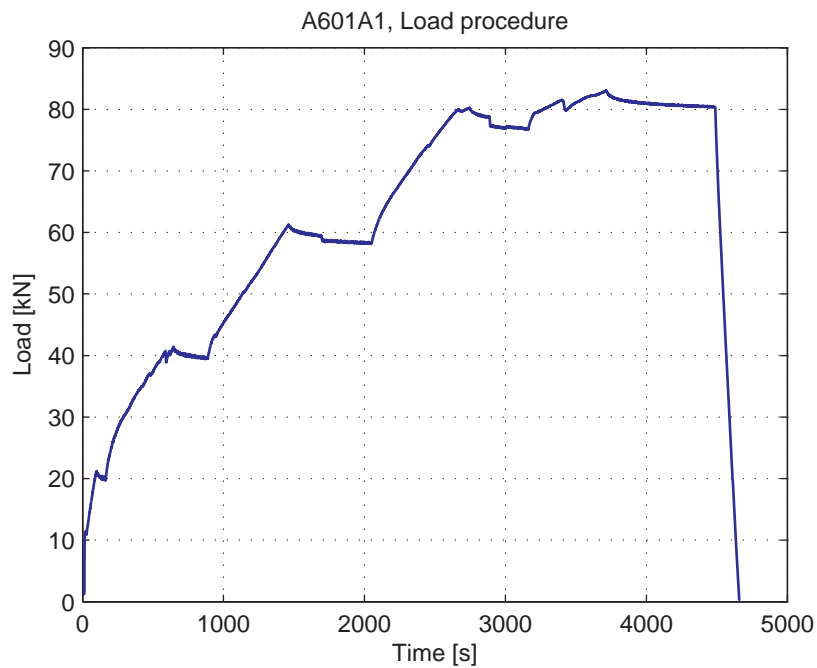
Fig. 5.31.1. Load-Time curve
