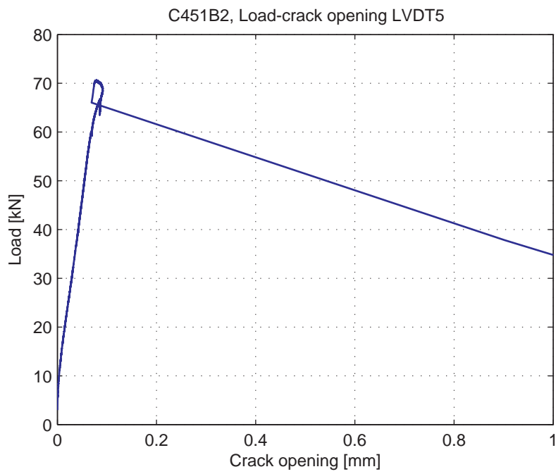
Fig. 5.68.6. Load-Crack opening for LVDT5
