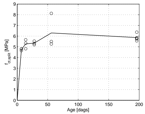
Fig. 2.2.4. F_{ct,split} development for cast 2
