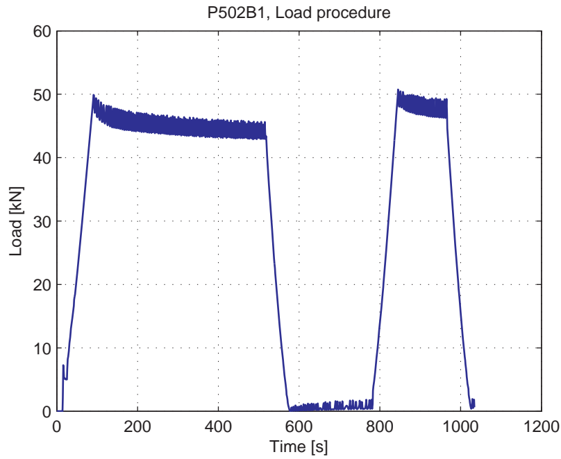
Fig. 5.82.4. Load-Time curve for first part of test
