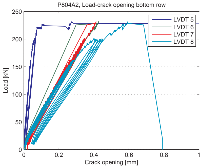
Fig. 5.93.7. Load-Crack opening for LVDT's 5-8 (bottom row)
