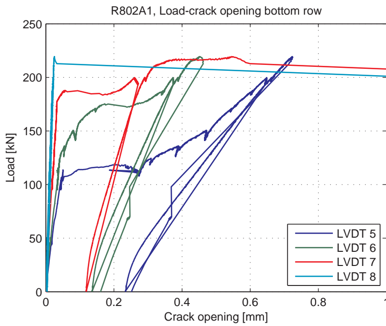
Fig. 5.102.8. Load-Crack opening for LVDT's 5-8 (bottom row)
