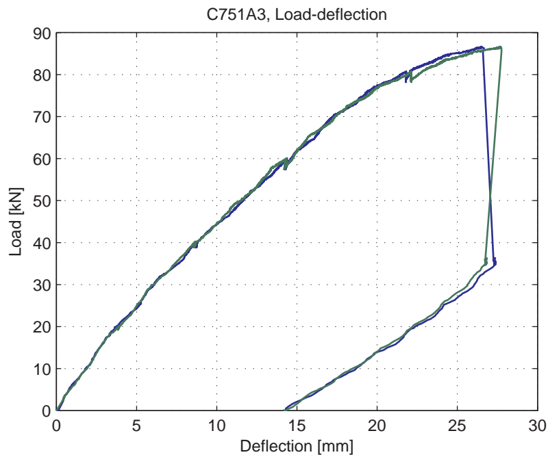
Fig. 5.60.4. Load-deflection curve
