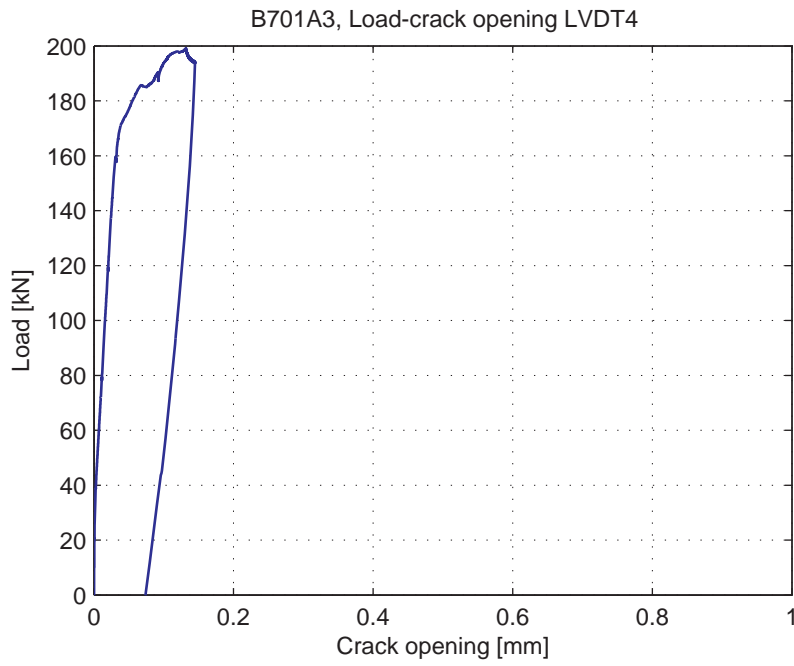
Fig. 5.42.5. Load-Crack opening for LVDT4
