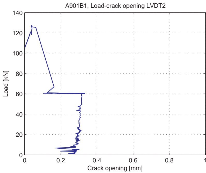
Fig. 5.15.6. Load-Crack opening for LVDT2
