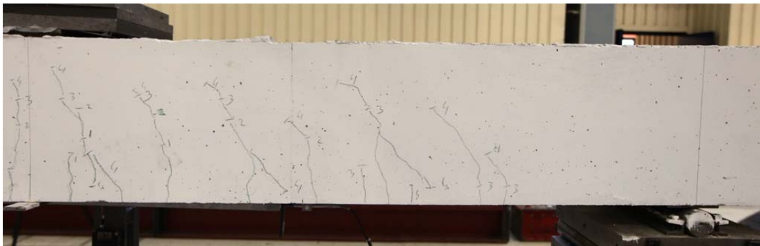
Fig. 5.58.2. Crack pattern after failure south side
