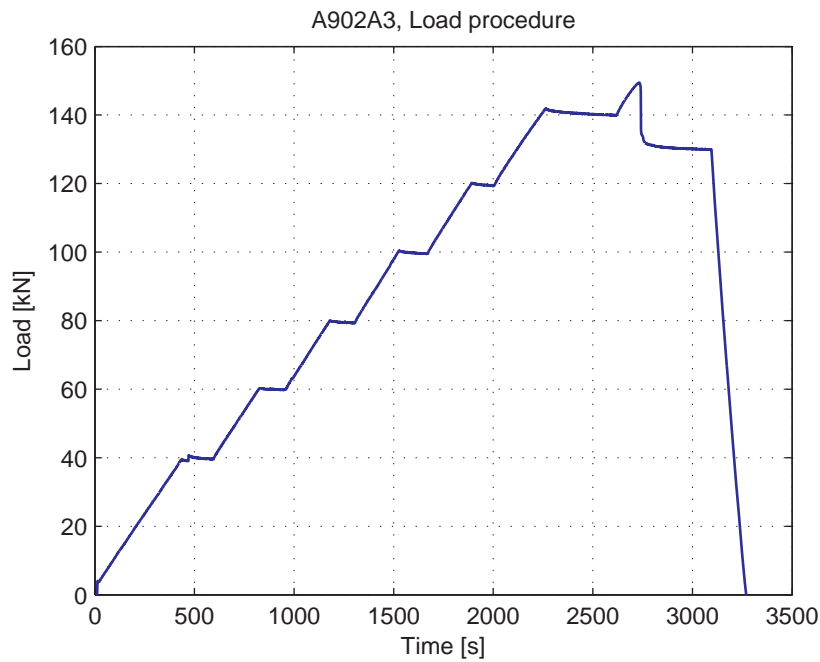
Fig. 5.19.3. Load-Time curve
