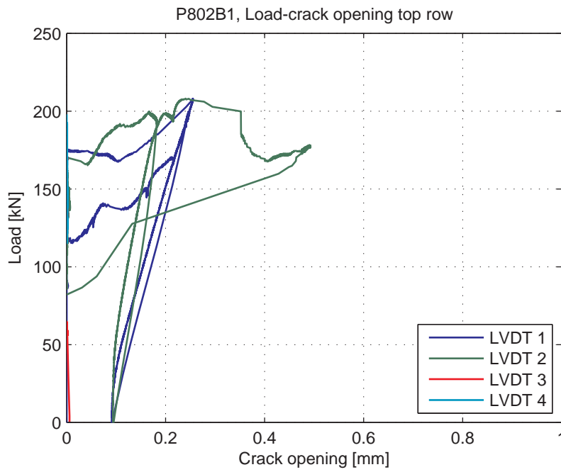
Fig. 5.88.6. Load-Crack opening for LVDT's 1-4 (top row)
