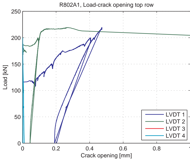
Fig. 5.102.6. Load-Crack opening for LVDT's 1-4 (top row)
