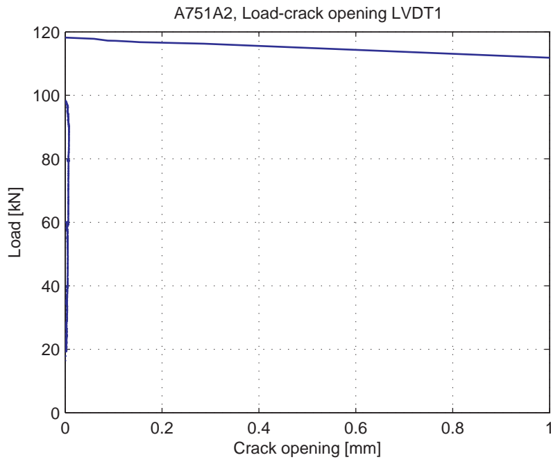
Fig. 5.23.5. Load-Crack opening for LVDT1
