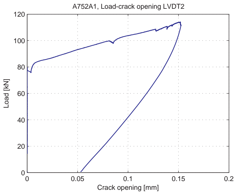
Fig. 5.26.6. Load-Crack opening for LVDT2
