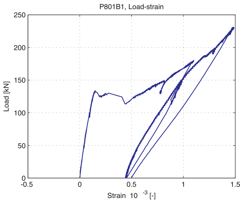
Fig. 5.86.11. Average strain over 1m length, measured at bottom of specimen (LVDT 14)
