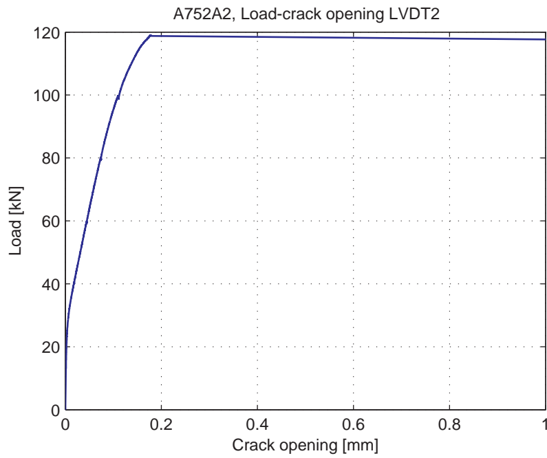
Fig. 5.27.6. Load-Crack opening for LVDT2
