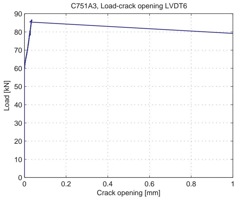
Fig. 5.60.7. Load-Crack opening for LVDT6
