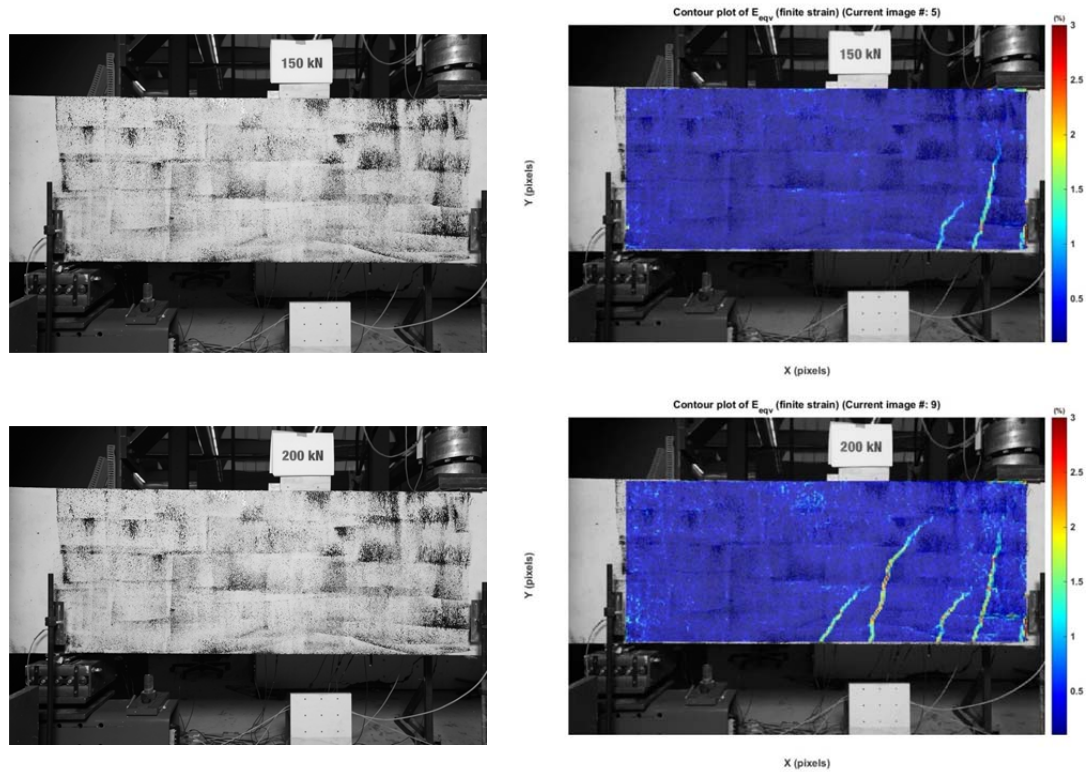
Fig. 3.2.3. DIC input pictures and results of 3 load steps
