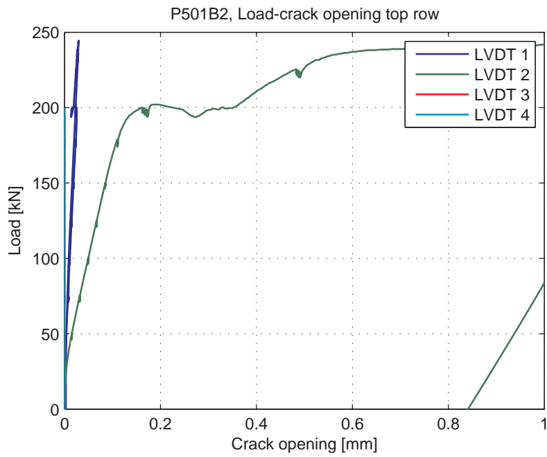
Fig. 5.79.6. Load-Crack opening for LVDT's 1-4 (top row)
