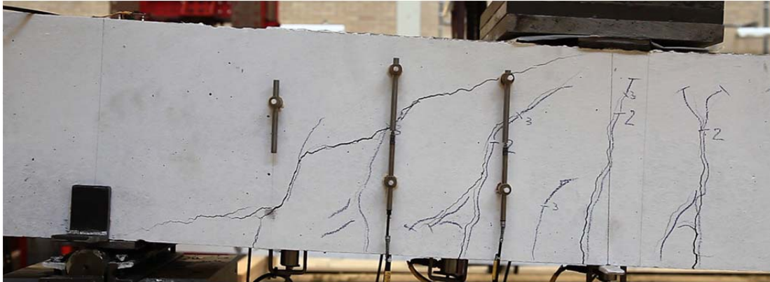
Fig. 5.30.1. Crack pattern after failure north side
