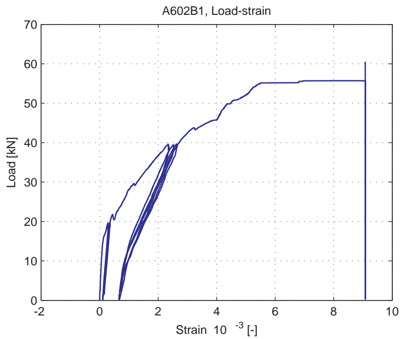
Fig. 5.38.6. Average strain over 1m length, measured at bottom of specimen (LVDT 3)
