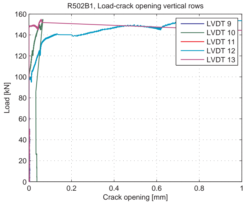
Fig. 5.99.7. Load-Crack opening for LVDT's 9-13 (vertical LVDT's)
