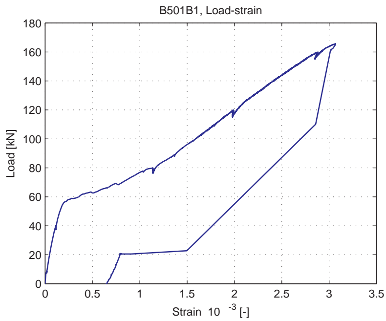
Fig. 5.49.8. Average strain over 1m length, measured at bottom of specimen (LVDT 3)
