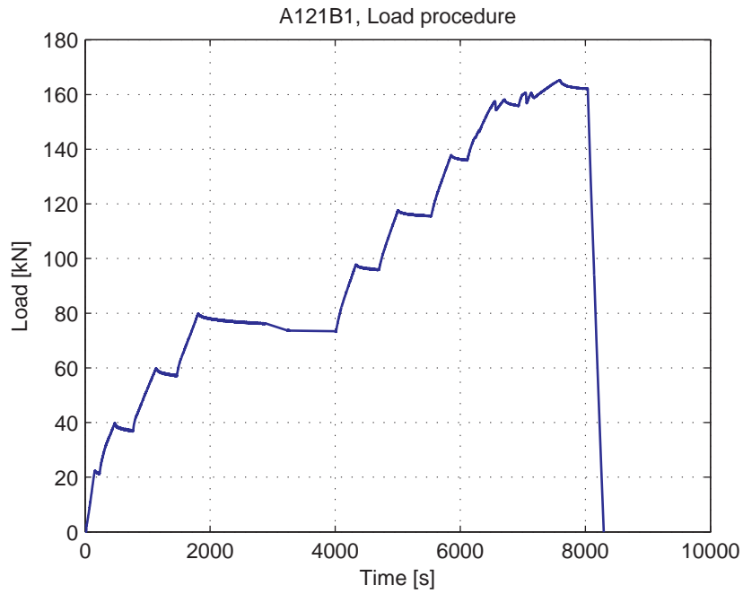
Fig. 5.4.3. Load-Time curve
