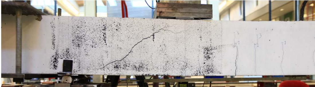
Fig. 5.72.1. Crack pattern after failure front side
