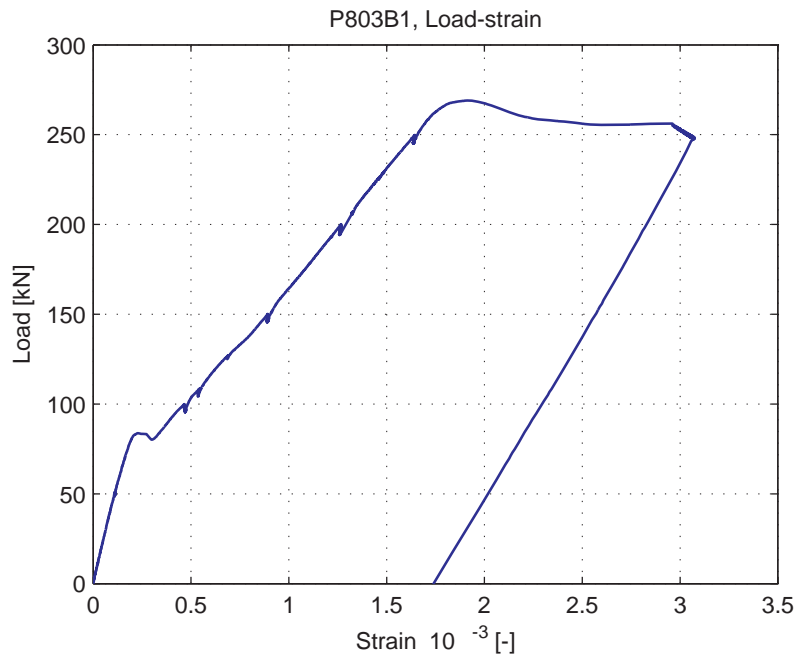
Fig. 5.90.11. Average strain over 1m length, measured at bottom of specimen (LVDT 14)
