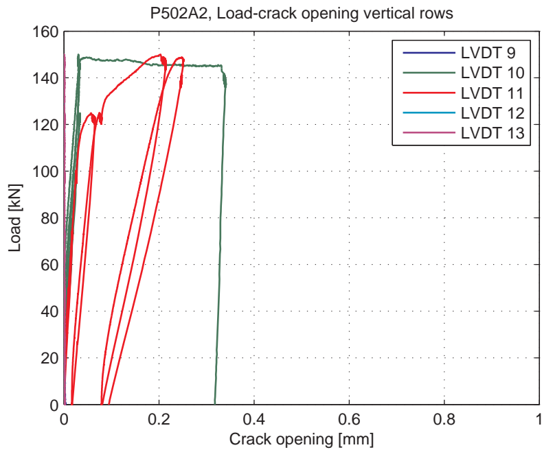
Fig. 5.81.7. Load-Crack opening for LVDT's 9-13 (vertical LVDT's)
