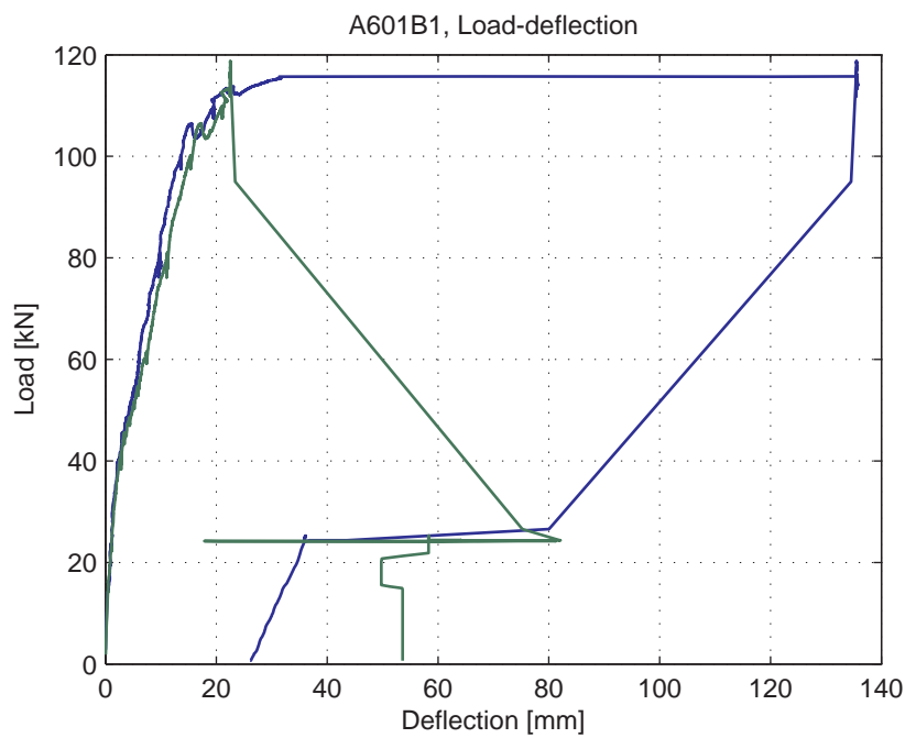
Fig. 5.33.4. Load-deflection curve
