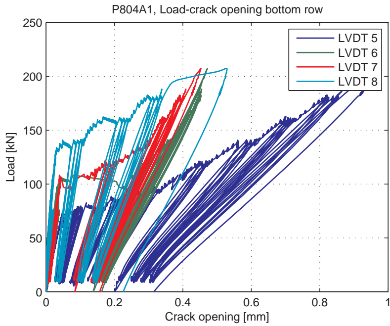
Fig. 5.92.8. Load-Crack opening for LVDT's 5-8 (bottom row)
