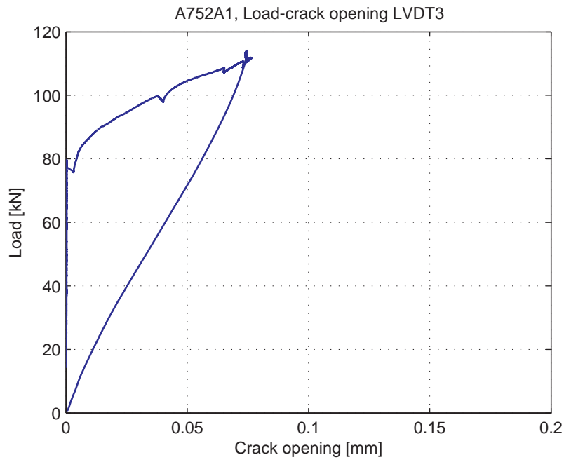
Fig. 5.26.7. Load-Crack opening for LVDT3
