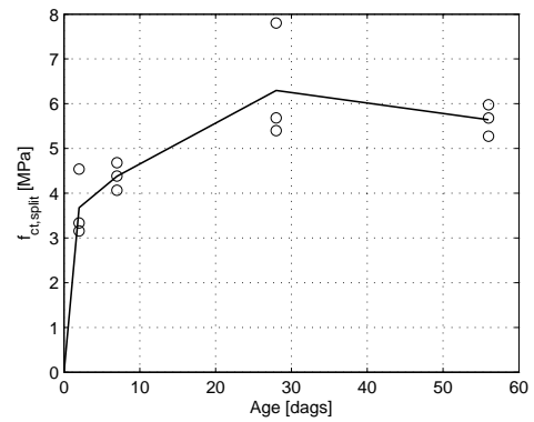
Fig. 2.2.2. F_{ct,split} development for cast 1
