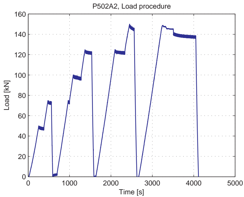
Fig. 5.81.4. Load-Time curve
