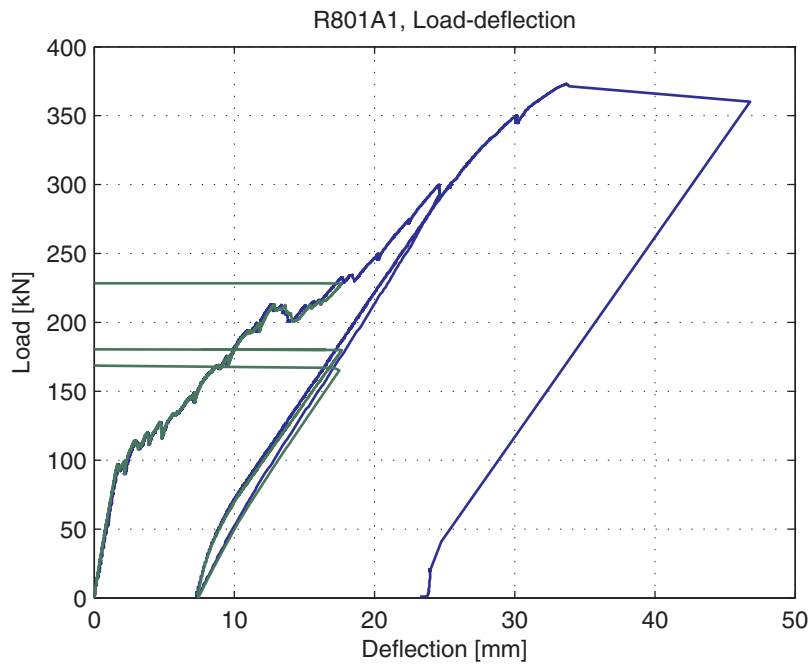
Fig. 5.100.5. Load-deflection curve
