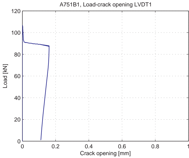
Fig. 5.24.5. Load-Crack opening for LVDT1
