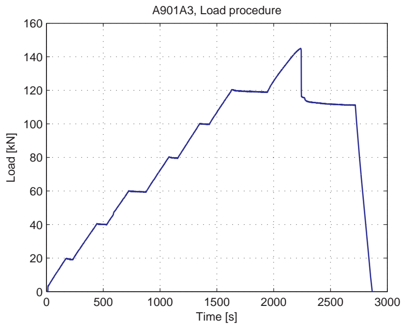
Fig. 5.14.3. Load-Time curve
