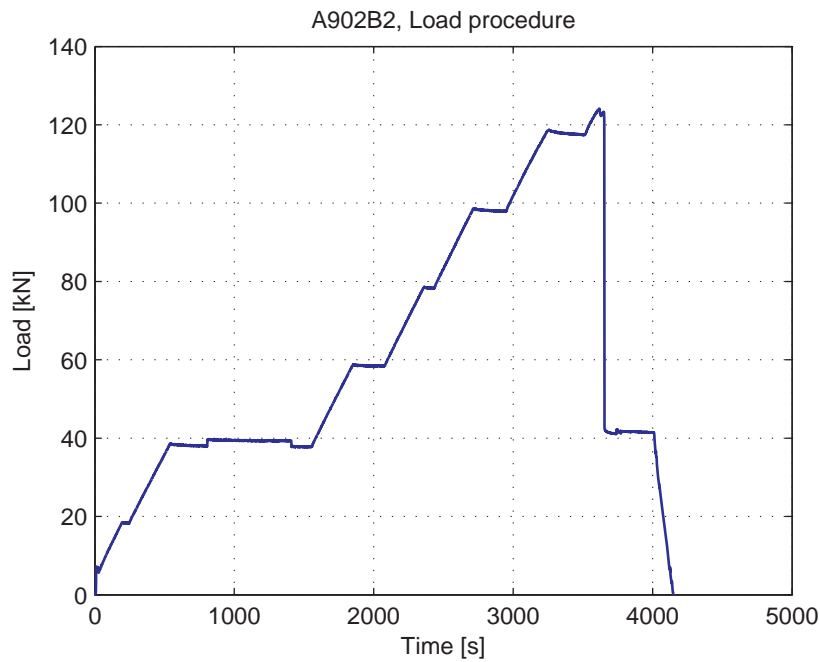
Fig. 5.21.3. Load-Time curve
