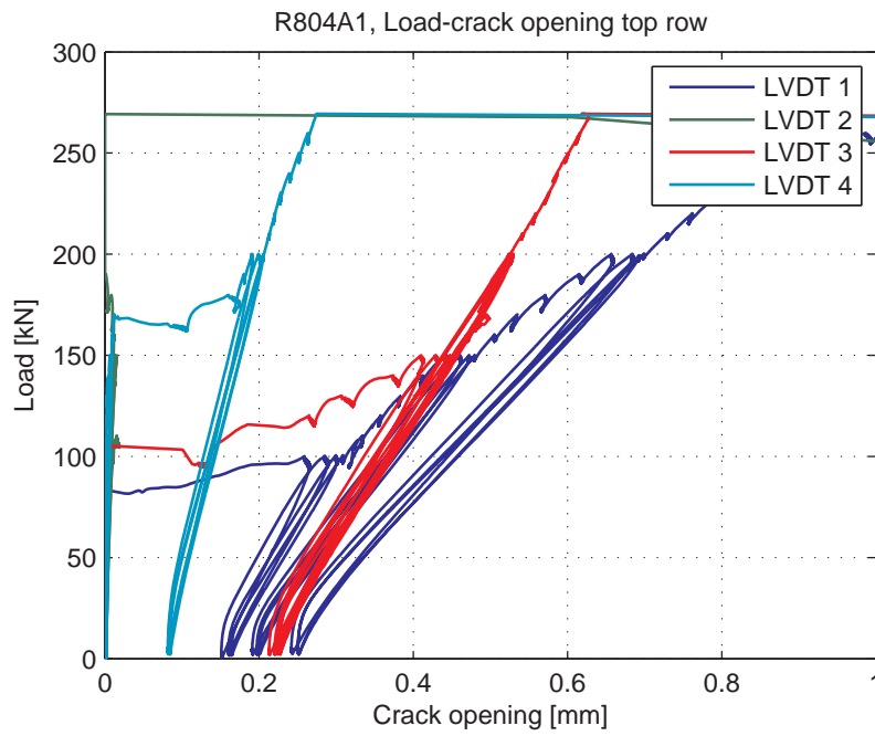
Fig. 5.106.6. Load-Crack opening for LVDT's 1-4 (top row)
