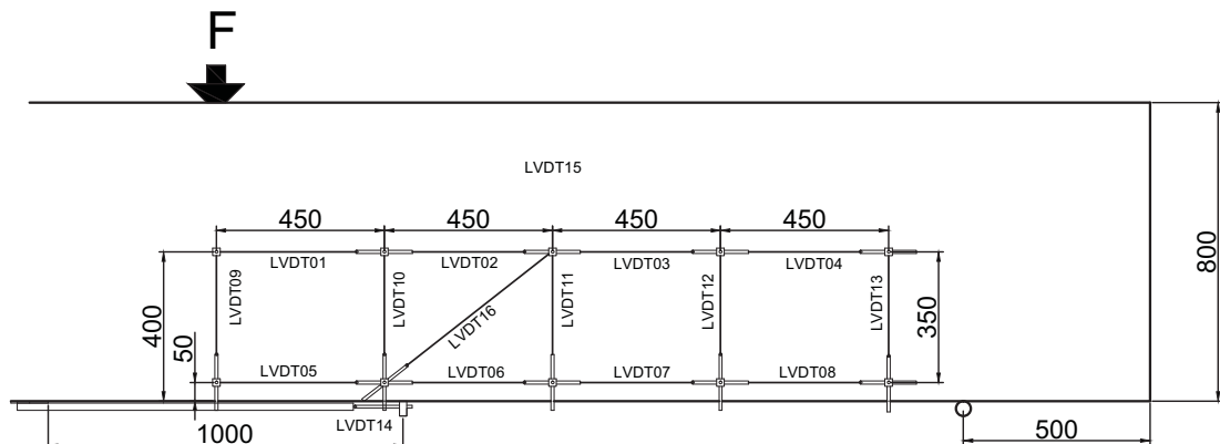
Fig. 5.103.3. LVDT layout and numbering for 800 mm deep beams
