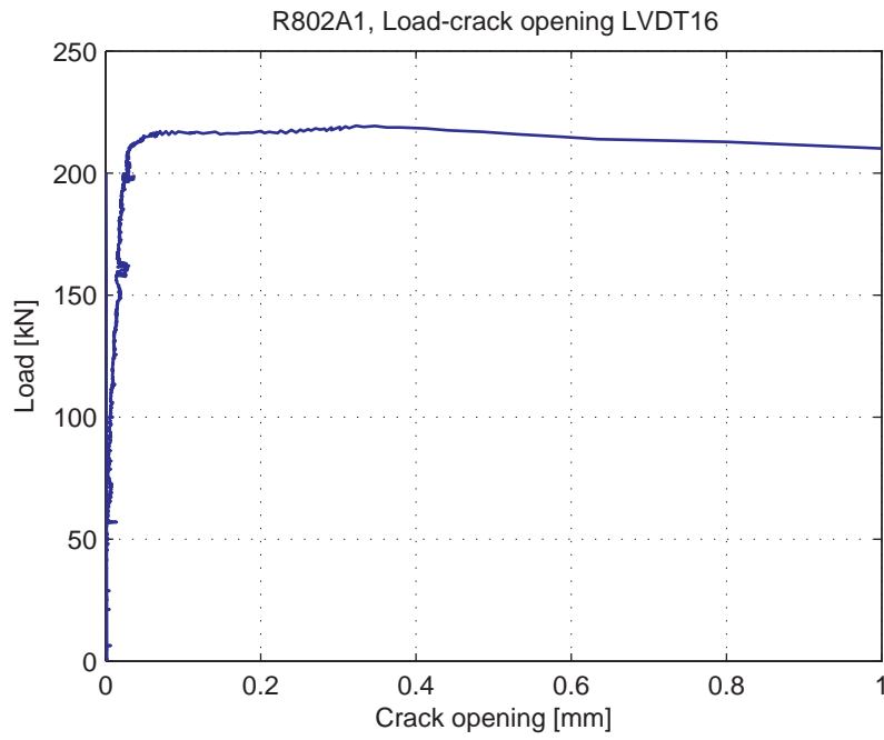
Fig. 5.102.9. Load-Crack opening for LVDT 16
