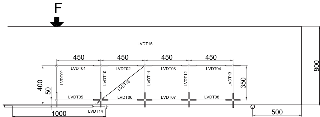
Fig. 5.87.3. LVDT layout and numbering for 800 mm deep beams
