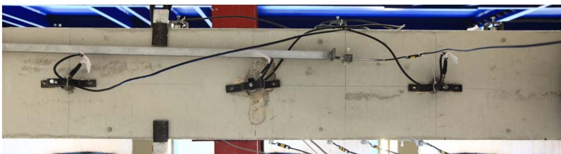
Fig. 5.57.4. Sensors used for Acoustic Emission measurements at bottom beam
