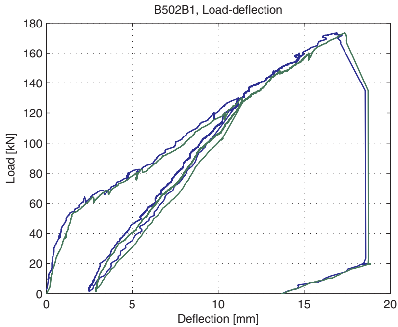
Fig. 5.53.4. Load-deflection curve
