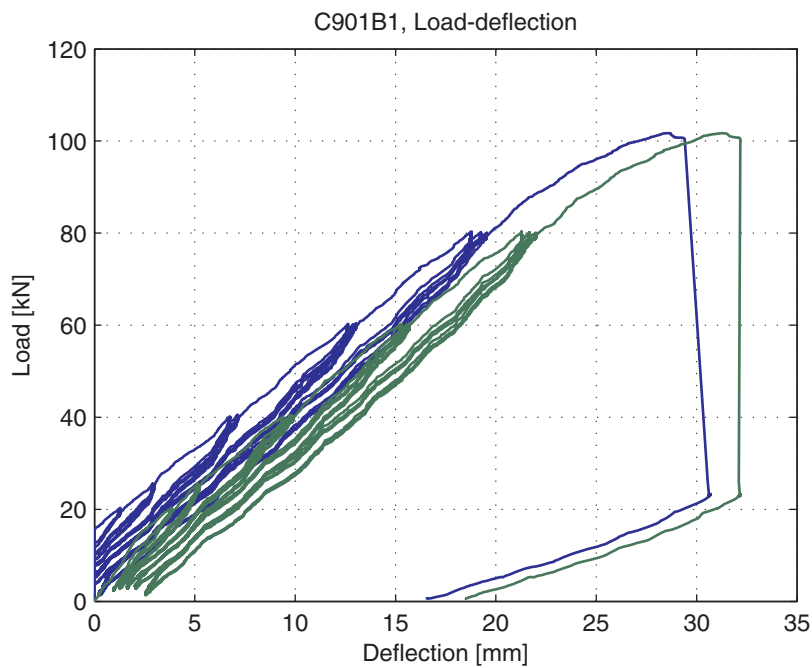
Fig. 5.57.6. Load-deflection curve
