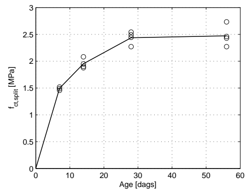
Fig. 2.2.6. F_{ct,split} development for cast 3
