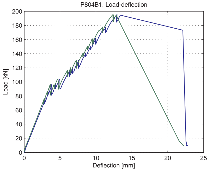
Fig. 5.94.5. Load-deflection curve
