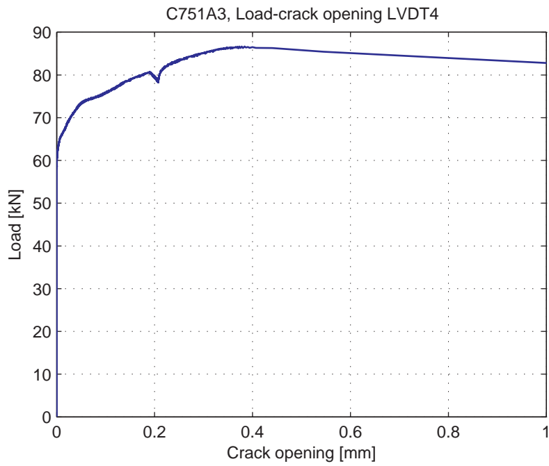
Fig. 5.60.5. Load-Crack opening for LVDT4
