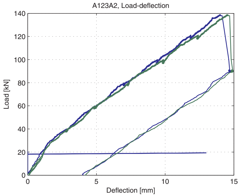
Fig. 5.9.4. Load-deflection curve
