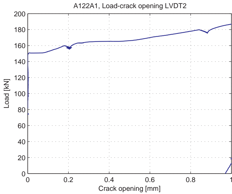
Fig. 5.5.6. Load-Crack opening for LVDT2
