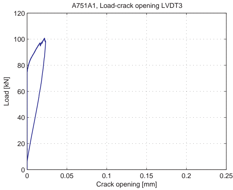
Fig. 5.22.7. Load-Crack opening for LVDT3
