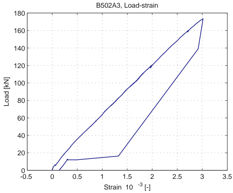
Fig. 5.52.9. Average strain over 1m length, measured at bottom of specimen (LVDT 3)
