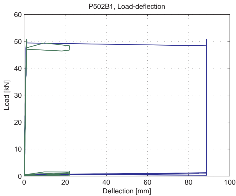
Fig. 5.82.7. Load-deflection curve for first part of test
