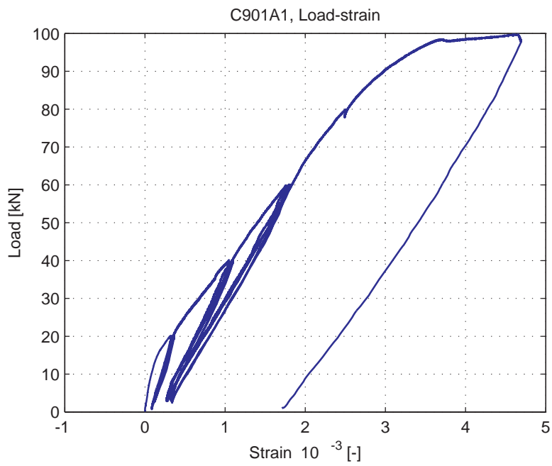
Fig. 5.54.6. Average strain over 1m length, measured at bottom of specimen (LVDT 3)
