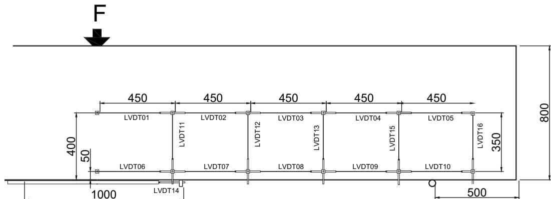
Fig. 5.107.3. LVDT layout and numbering for 800 mm deep beams
