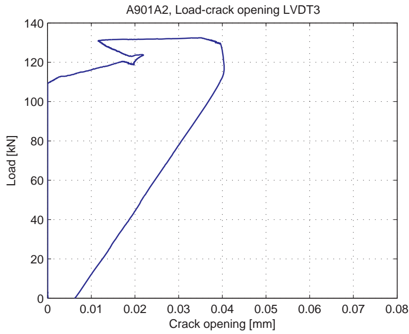
Fig. 5.13.7. Load-Crack opening for LVDT3
