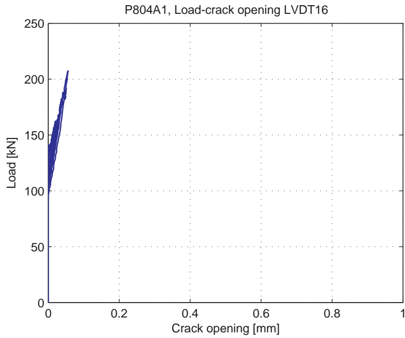
Fig. 5.92.12. Load-Crack opening for LVDT 16
