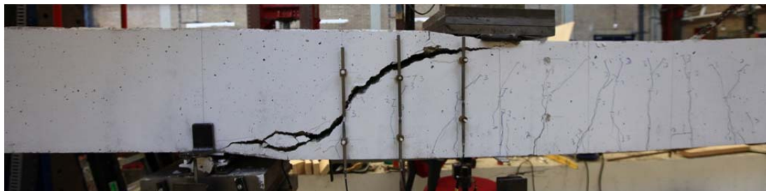
Fig. 5.64.1. Crack pattern after failure north side
