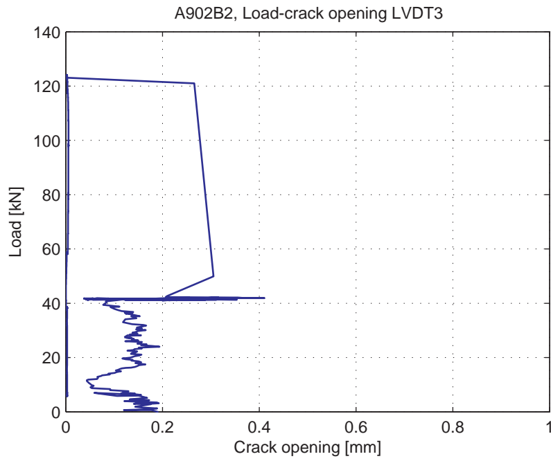
Fig. 5.21.7. Load-Crack opening for LVDT3
