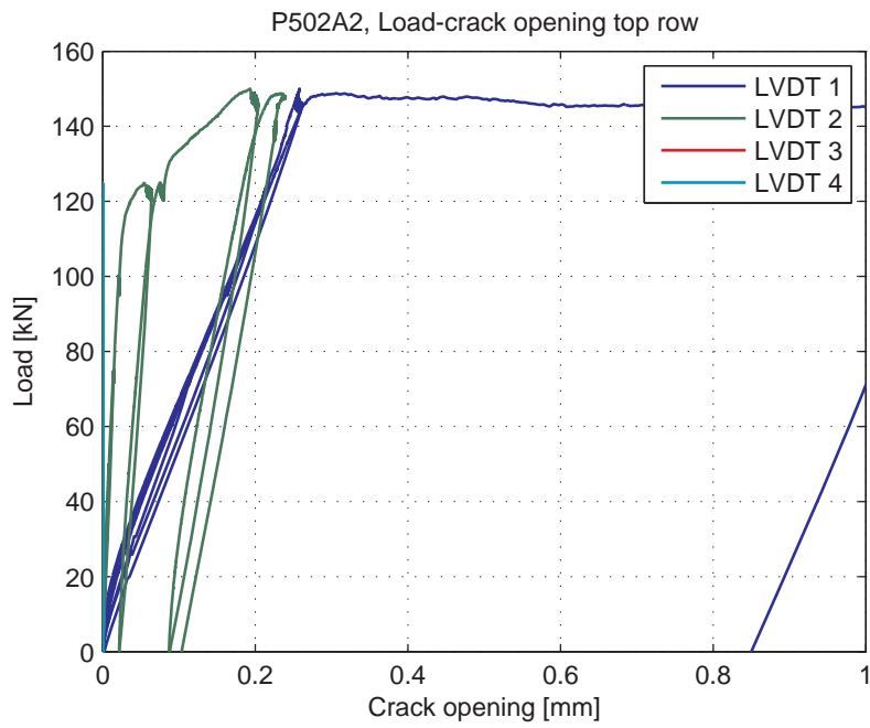
Fig. 5.81.6. Load-Crack opening for LVDT's 1-4 (top row)
