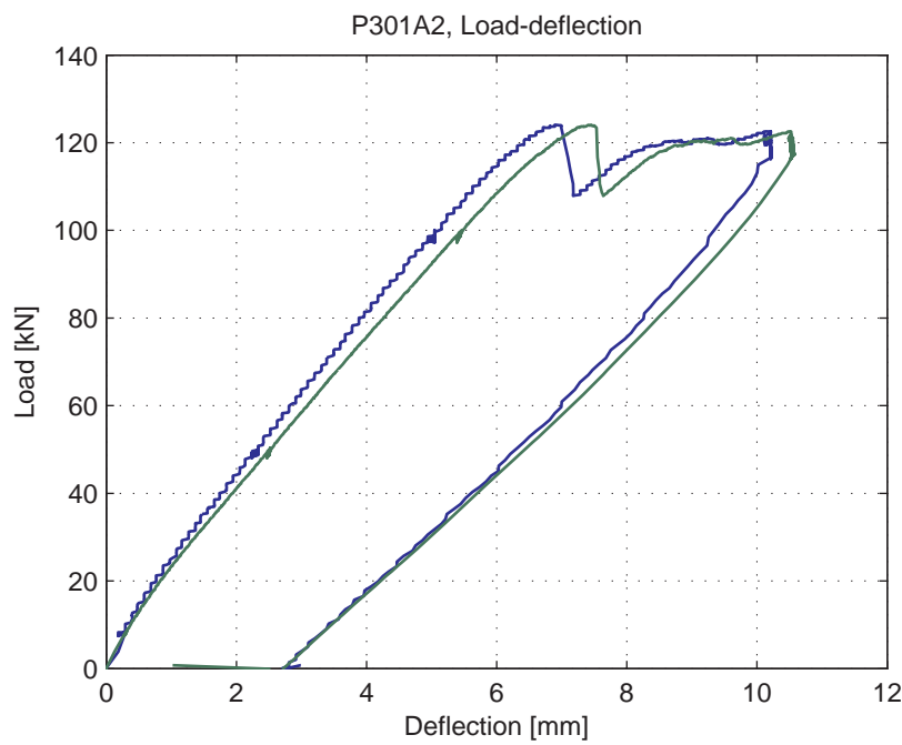
Fig. 5.72.5. Load-deflection curve
