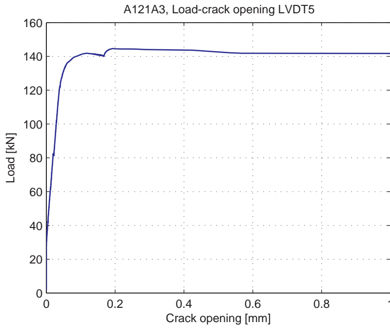
Fig. 5.3.9. Load-Crack opening for LVDT5
