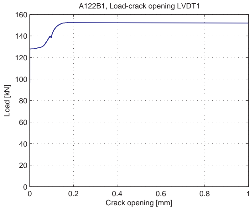
Fig. 5.6.5. Load-Crack opening for LVDT1
