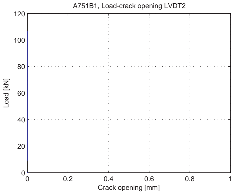
Fig. 5.24.6. Load-Crack opening for LVDT2
