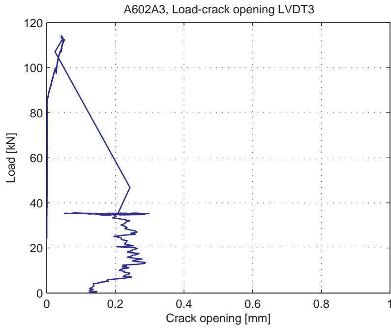
Fig. 5.37.7. Load-Crack opening for LVDT3
