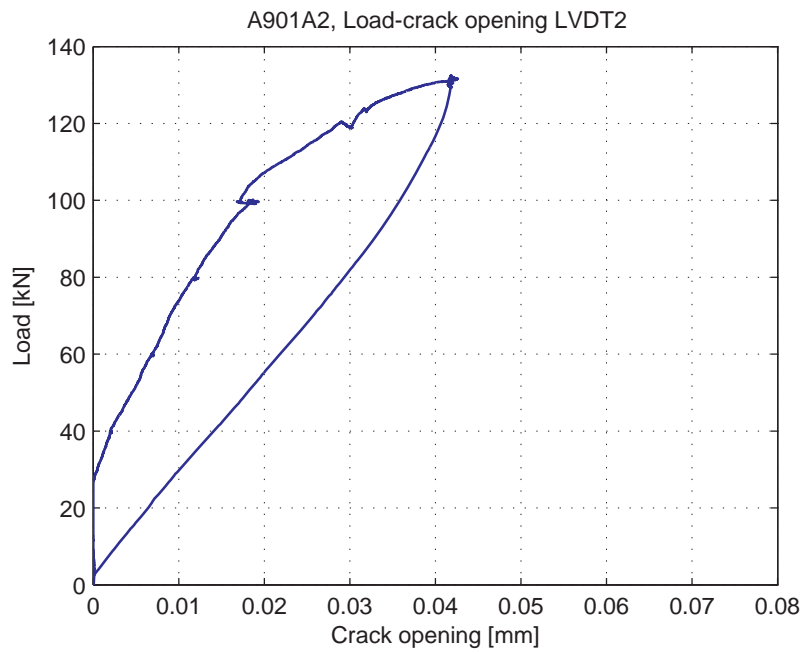
Fig. 5.13.6. Load-Crack opening for LVDT2
