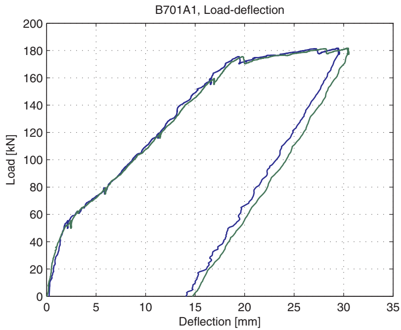
Fig. 5.40.4. Load-deflection curve
