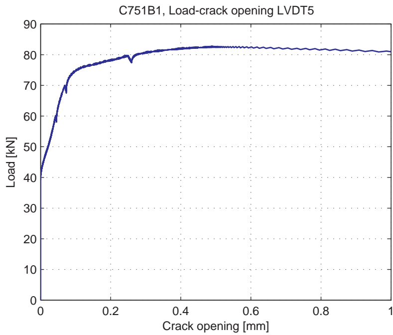
Fig. 5.61.6. Load-Crack opening for LVDT5
