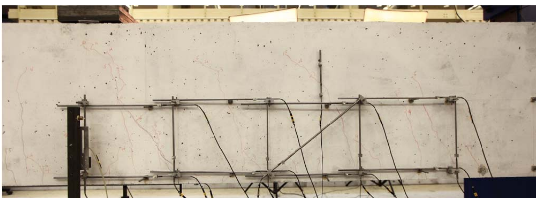
Fig. 5.90.2. Crack pattern after failure south side
