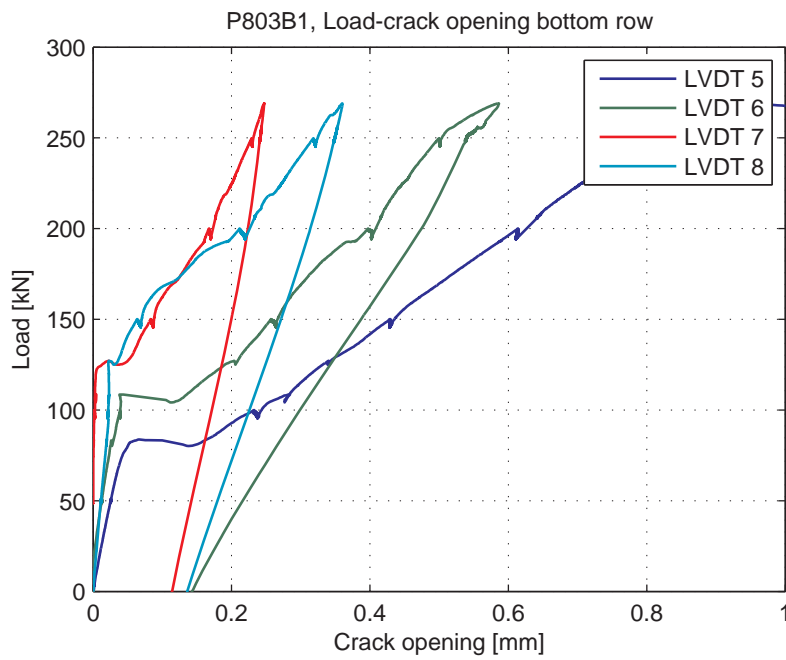
Fig. 5.90.8. Load-Crack opening for LVDT's 5-8 (bottom row)
