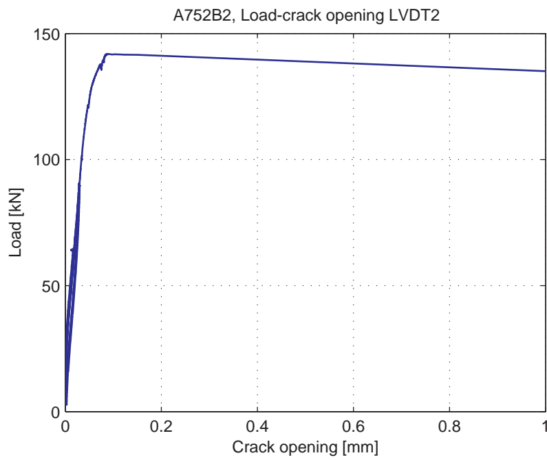
Fig. 5.30.6. Load-Crack opening for LVDT2
