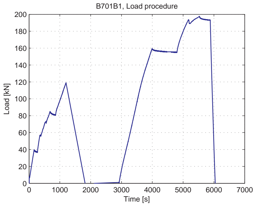
Fig. 5.43.3. Load-Time curve
