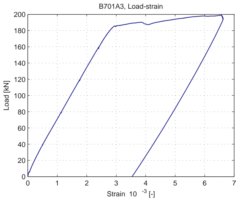
Fig. 5.42.8. Average strain over 1m length, measured at bottom of specimen (LVDT 3)
