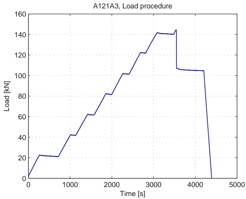
Fig. 5.3.3. Load-Time curve
