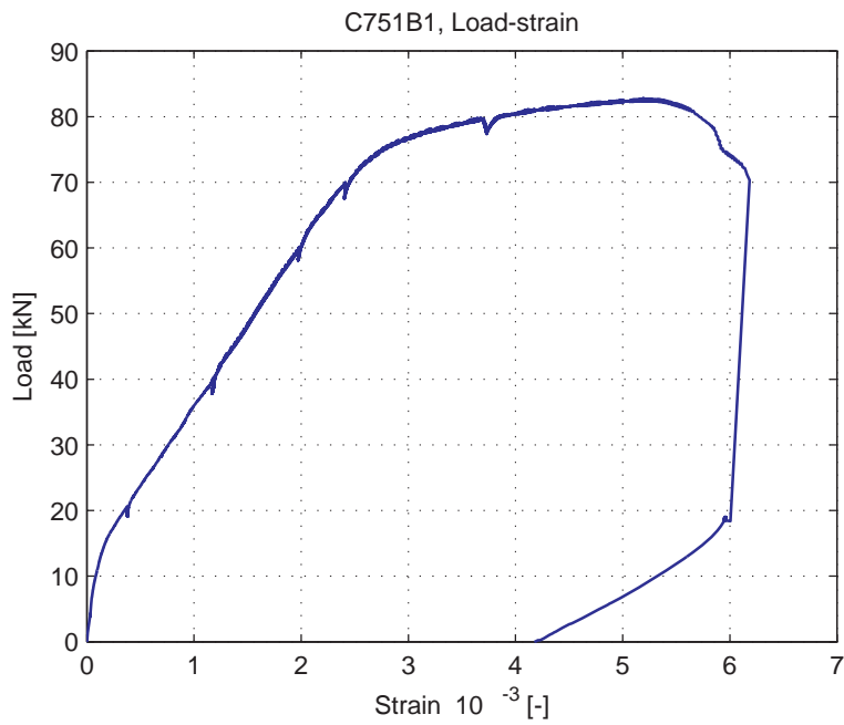
Fig. 5.61.8. Average strain over 1m length, measured at bottom of specimen (LVDT 3)
