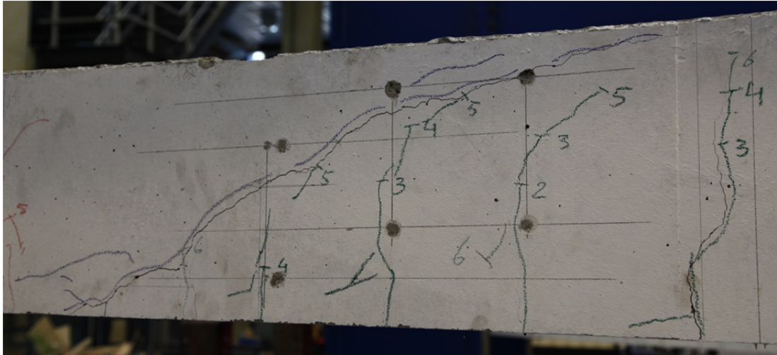
Fig. 5.27.1. Crack pattern after failure north side
