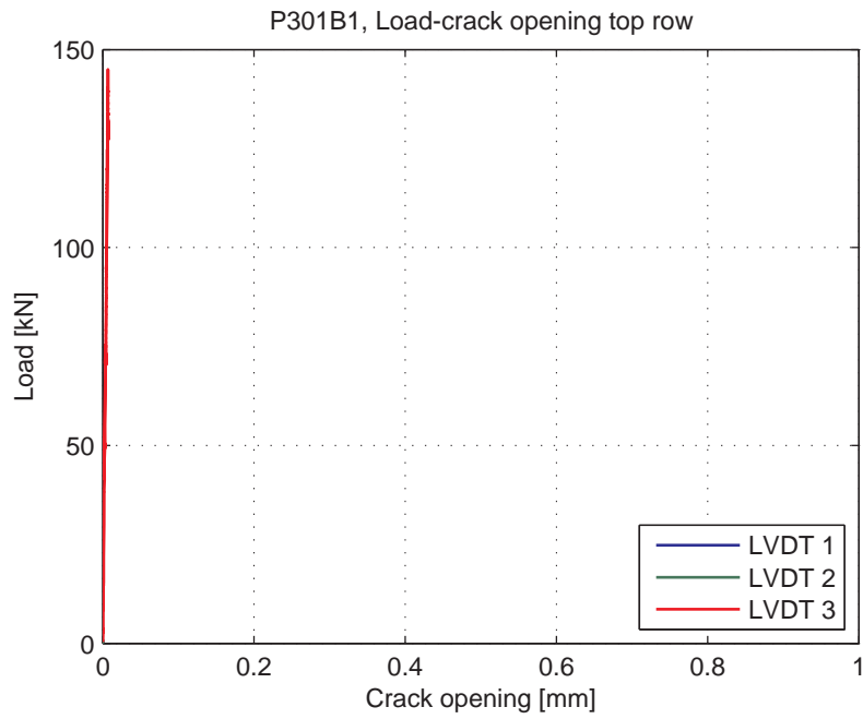
Fig. 5.75.6. Load-Crack opening for LVDT's 1-3 (top row)
