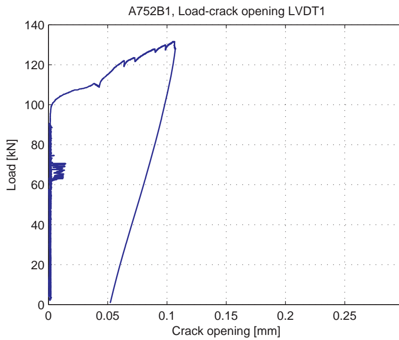
Fig. 5.29.6. Load-Crack opening for LVDT1
