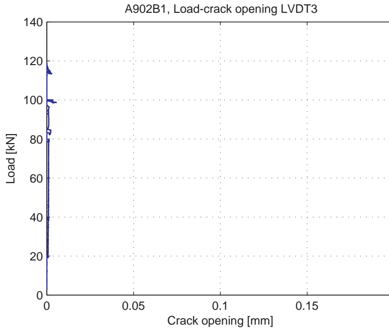
Fig. 5.20.7. Load-Crack opening for LVDT3
