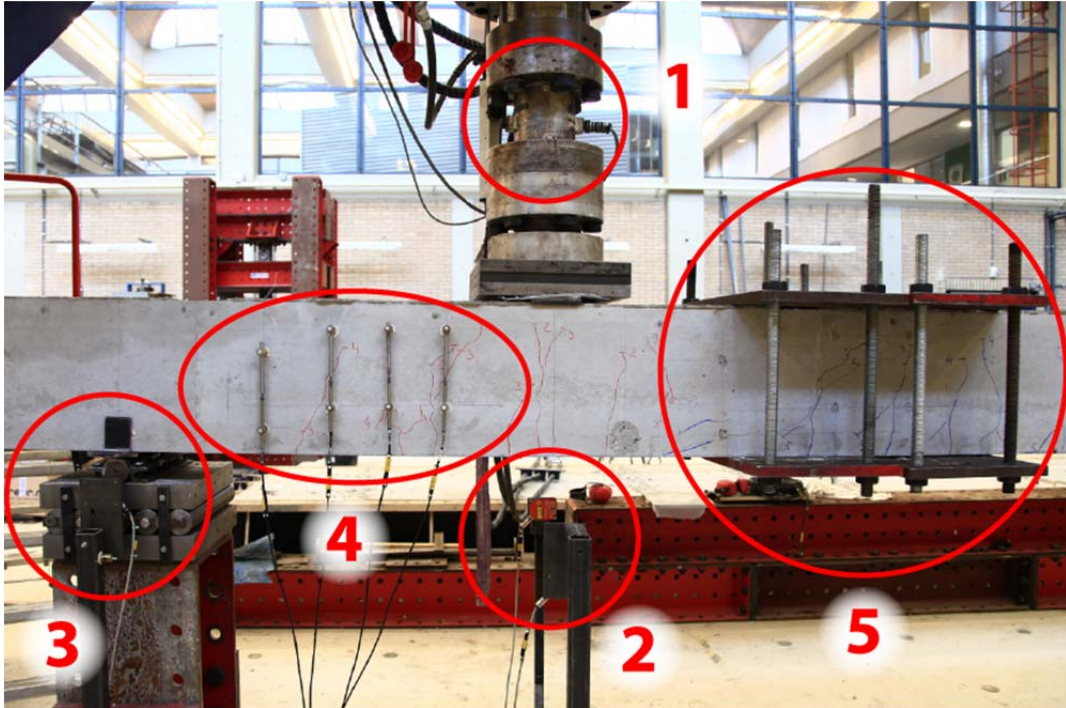
Fig. 3.2.1. Measurements (1-4) and strengthening of cracked specimen (5)
