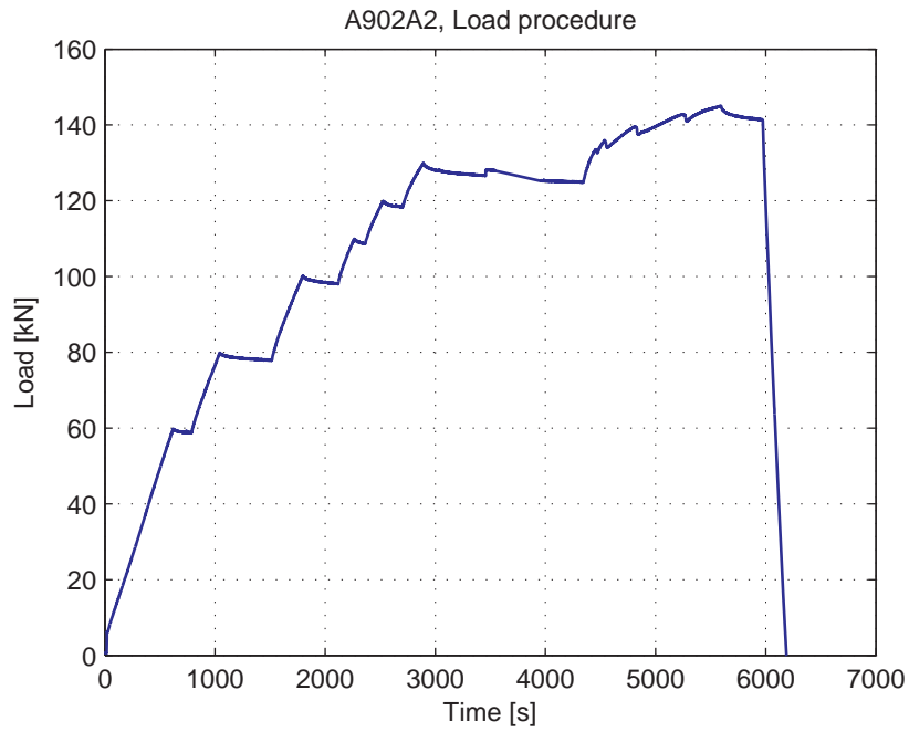
Fig. 5.18.3. Load-Time curve
