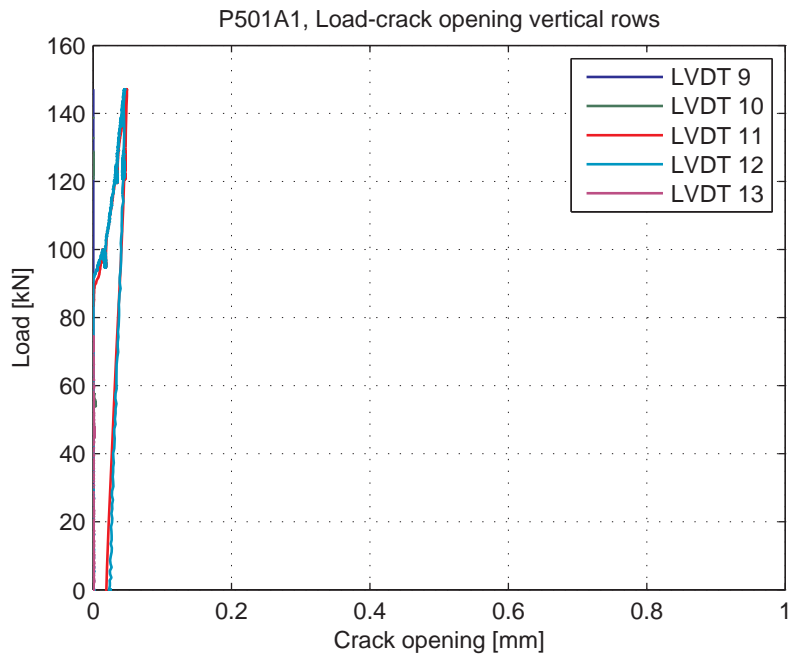
Fig. 5.76.7. Load-Crack opening for LVDT's 9-13 (vertical LVDT's)
