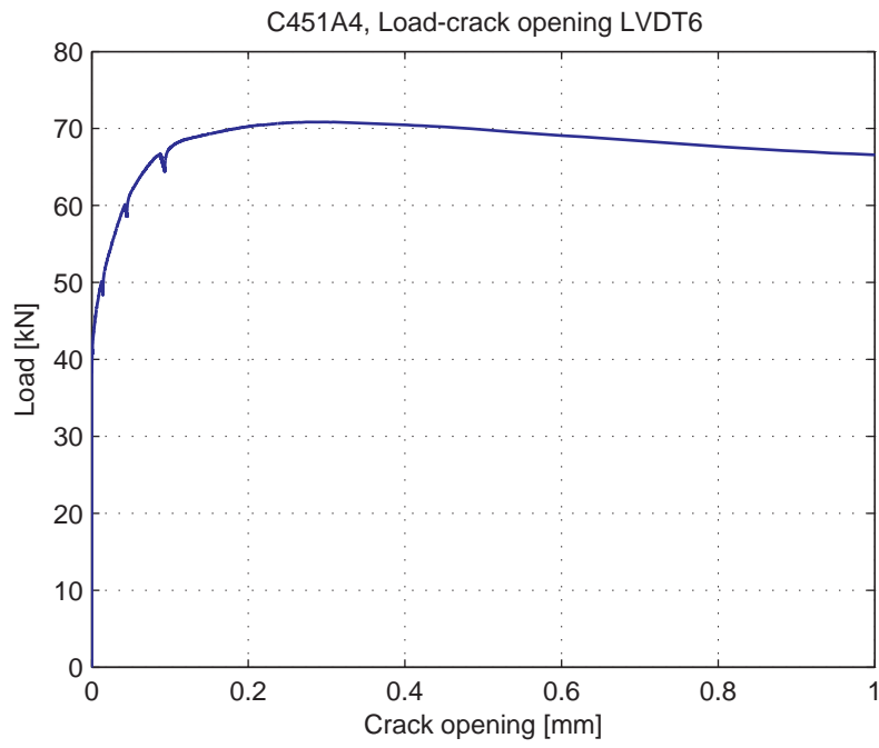
Fig. 5.65.7. Load-Crack opening for LVDT6
