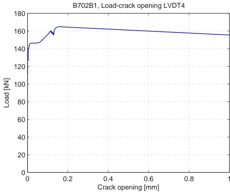
Fig. 5.46.5. Load-Crack opening for LVDT4
