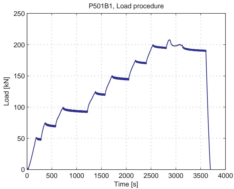
Fig. 5.78.4. Load-Time curve
