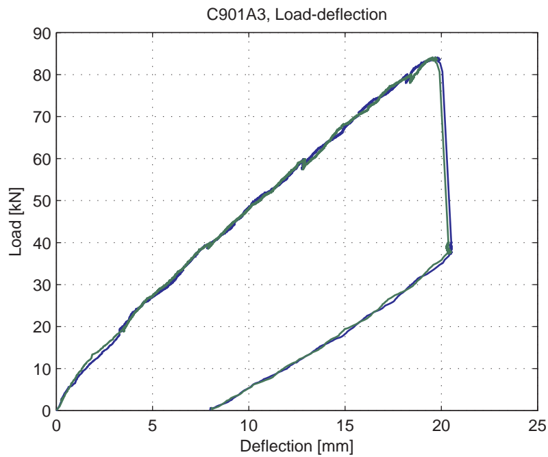
Fig. 5.56.4. Load-deflection curve
