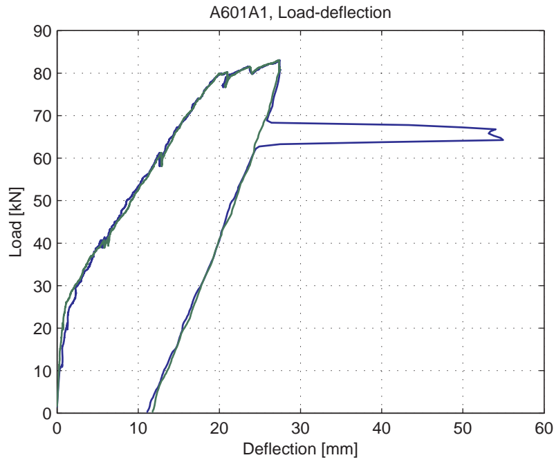
Fig. 5.31.2. Load-deflection curve
