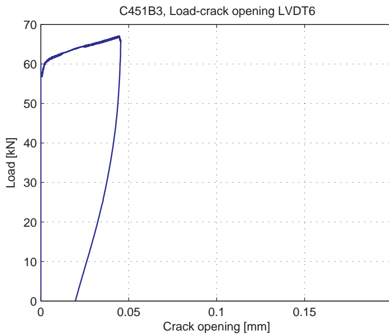
Fig. 5.69.8. Load-Crack opening for LVDT6
