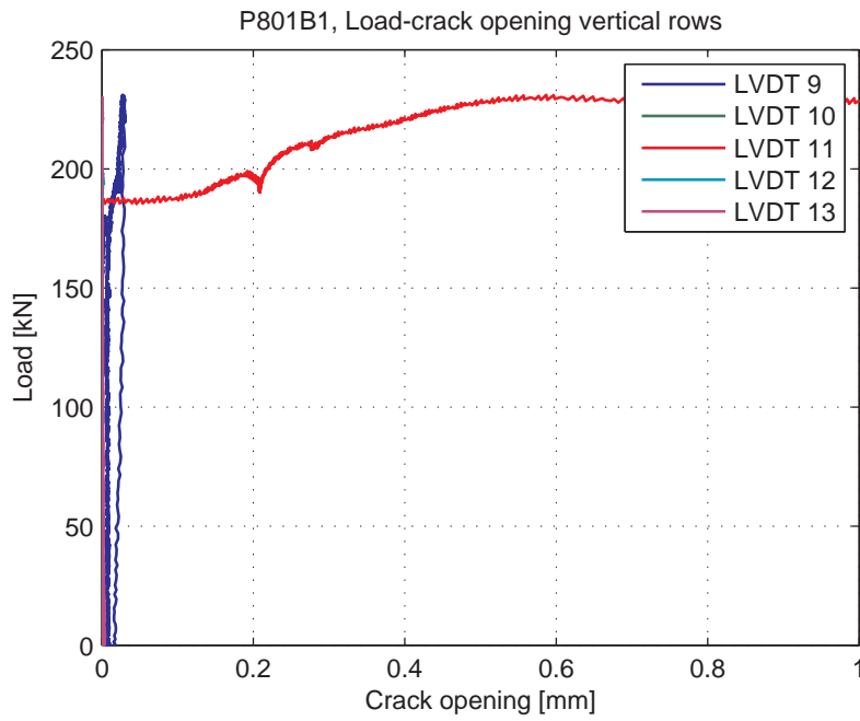
Fig. 5.86.8. Load-Crack opening for LVDT's 9-13 (vertical LVDT's)
