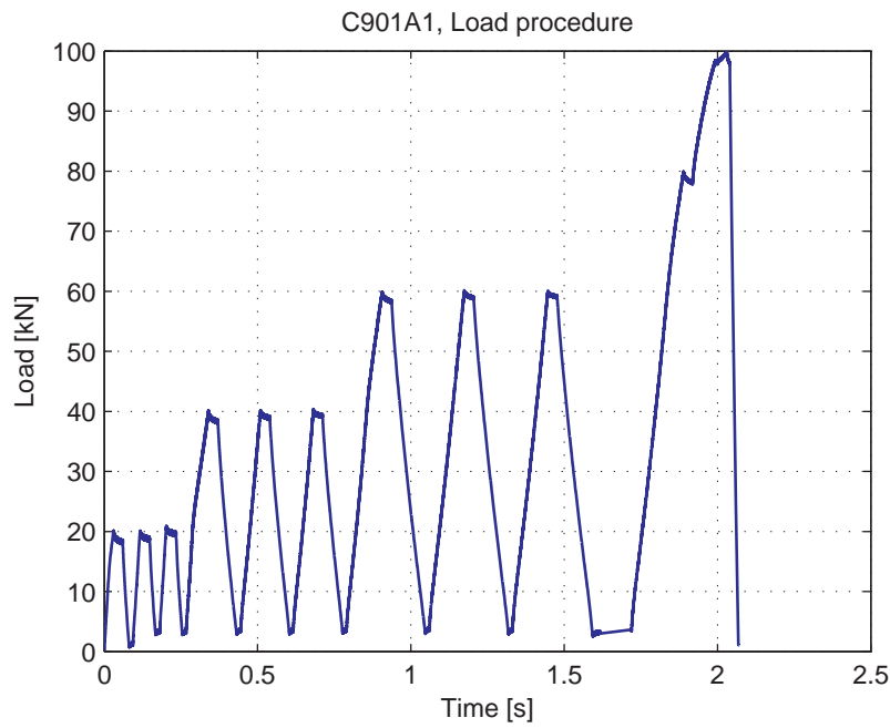
Fig. 5.54.1. Load-Time curve
