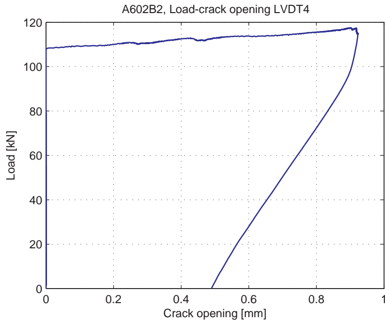
Fig. 5.39.5. Load-Crack opening for LVDT4
