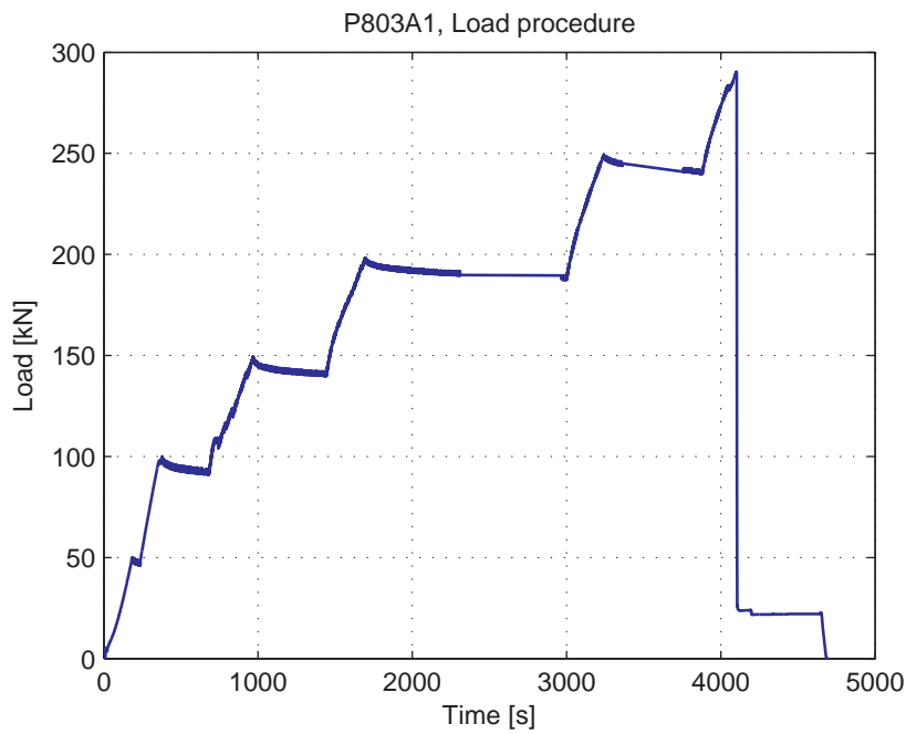
Fig. 5.89.4. Load-Time curve
