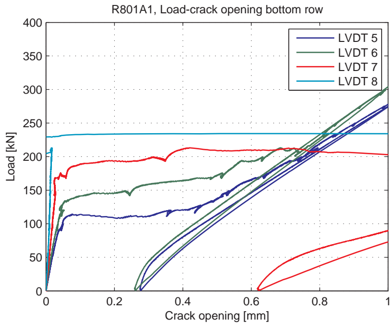
Fig. 5.100.8. Load-Crack opening for LVDT's 5-8 (bottom row)
