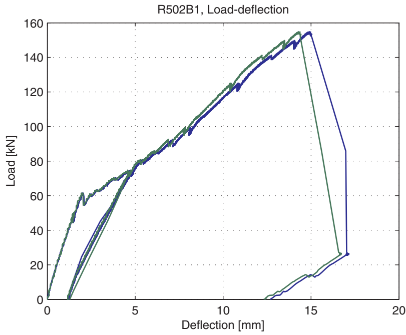
Fig. 5.99.5. Load-deflection curve
