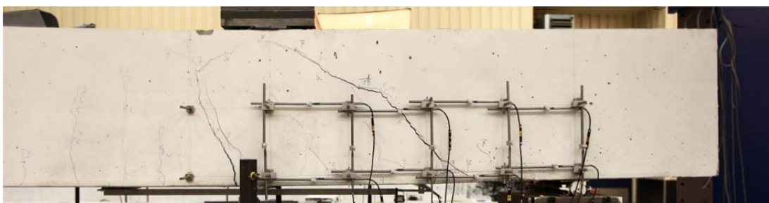
Fig. 5.79.2. Crack pattern after failure back side
