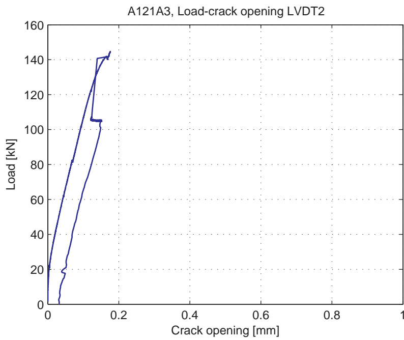
Fig. 5.3.6. Load-Crack opening for LVDT2
