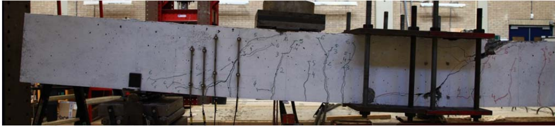
Fig. 5.34.1. Crack pattern after failure north side
