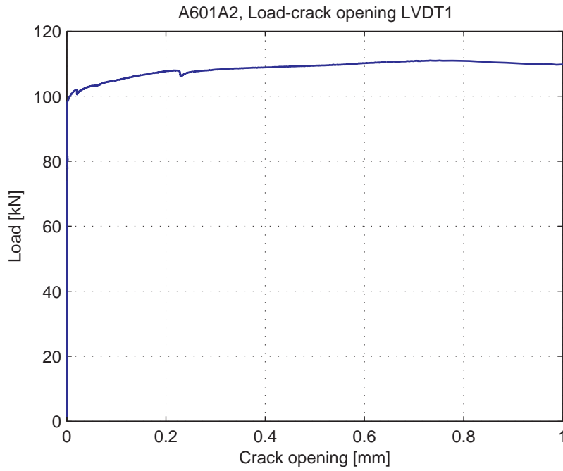
Fig. 5.32.5. Load-Crack opening for LVDT1
