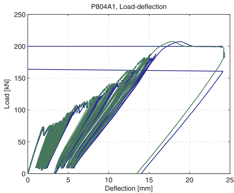
Fig. 5.92.5. Load-deflection curve
