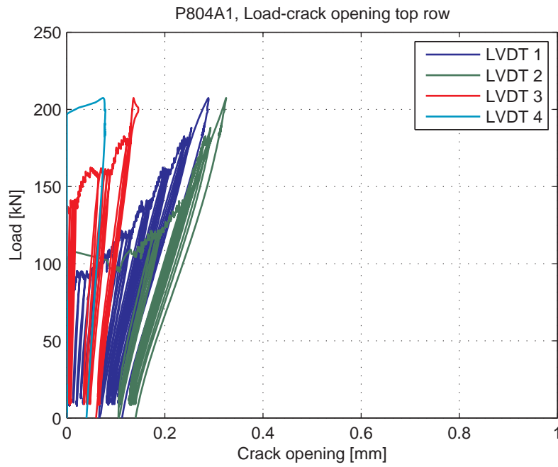
Fig. 5.92.6. Load-Crack opening for LVDT's 1-4 (top row)
