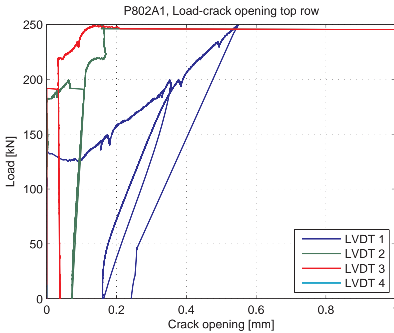
Fig. 5.87.6. Load-Crack opening for LVDT's 1-4 (top row)
