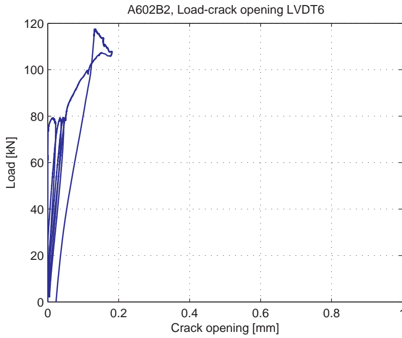
Fig. 5.39.7. Load-Crack opening for LVDT6
