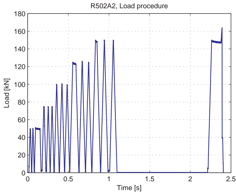
Fig. 5.98.3. Load-Time curve
