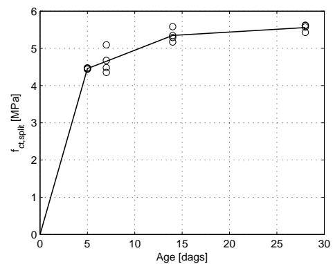
Fig. 2.2.8. F_{ct,split} development for cast 5
