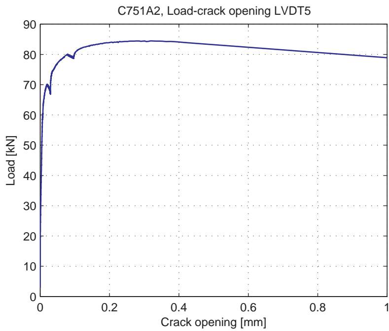
Fig. 5.59.6. Load-Crack opening for LVDT5
