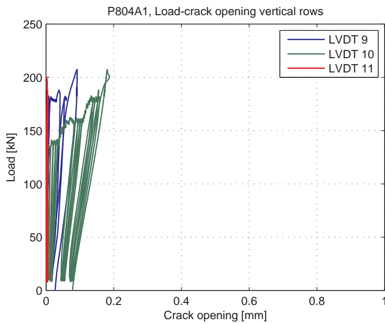
Fig. 5.92.7. Load-Crack opening for LVDT's 9-11 (vertical LVDT's)
