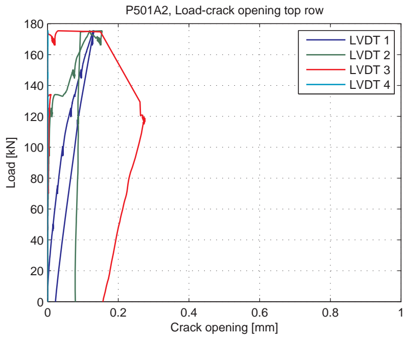
Fig. 5.77.6. Load-Crack opening for LVDT's 1-4 (top row)
