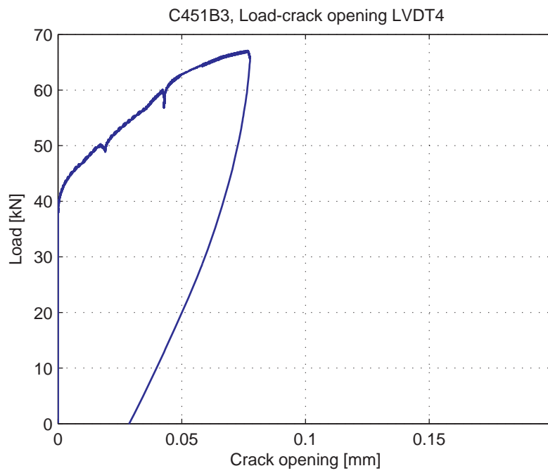
Fig. 5.69.6. Load-Crack opening for LVDT4
