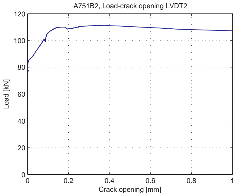
Fig. 5.25.6. Load-Crack opening for LVDT2
