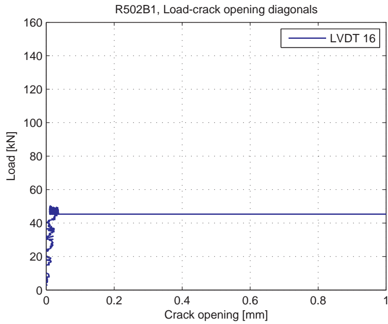
Fig. 5.99.9. Load-Crack opening for LVDT 16 (diagonal)
