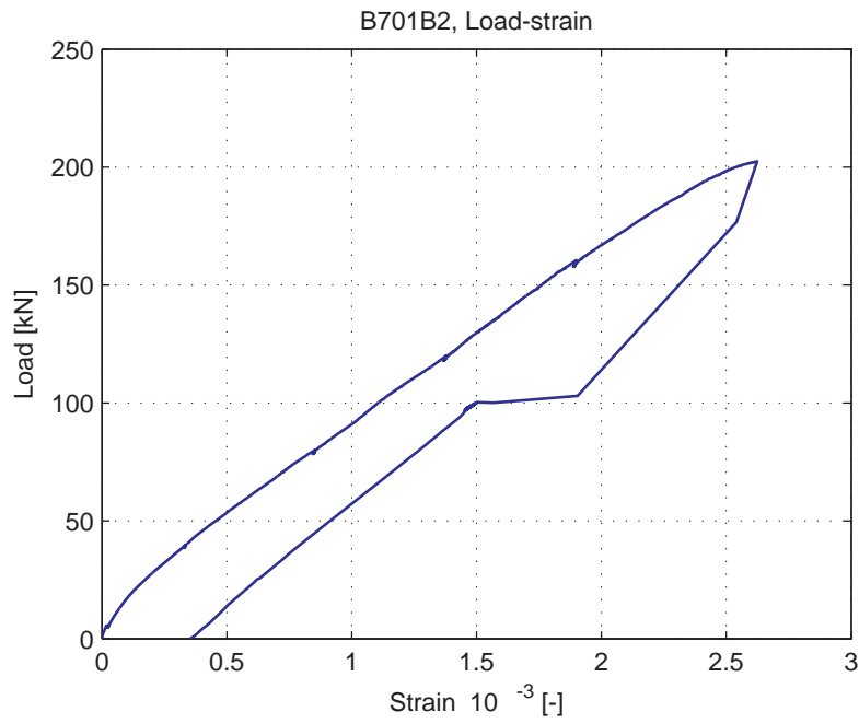
Fig. 5.44.9. Average strain over 1m length, measured at bottom of specimen (LVDT 3)
