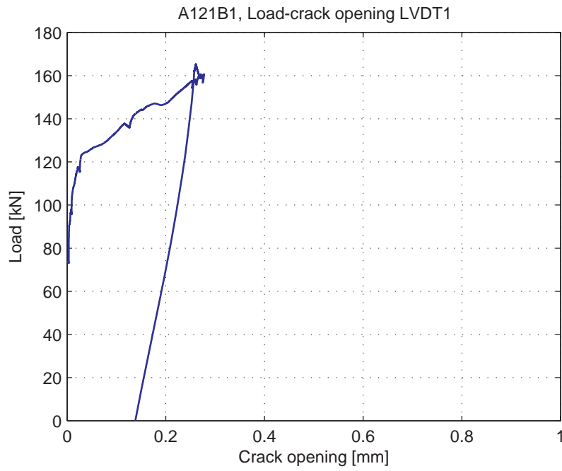
Fig. 5.4.5. Load-Crack opening for LVDT1
