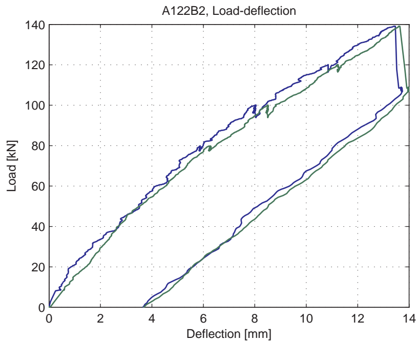
Fig. 5.7.4. Load-deflection curve
