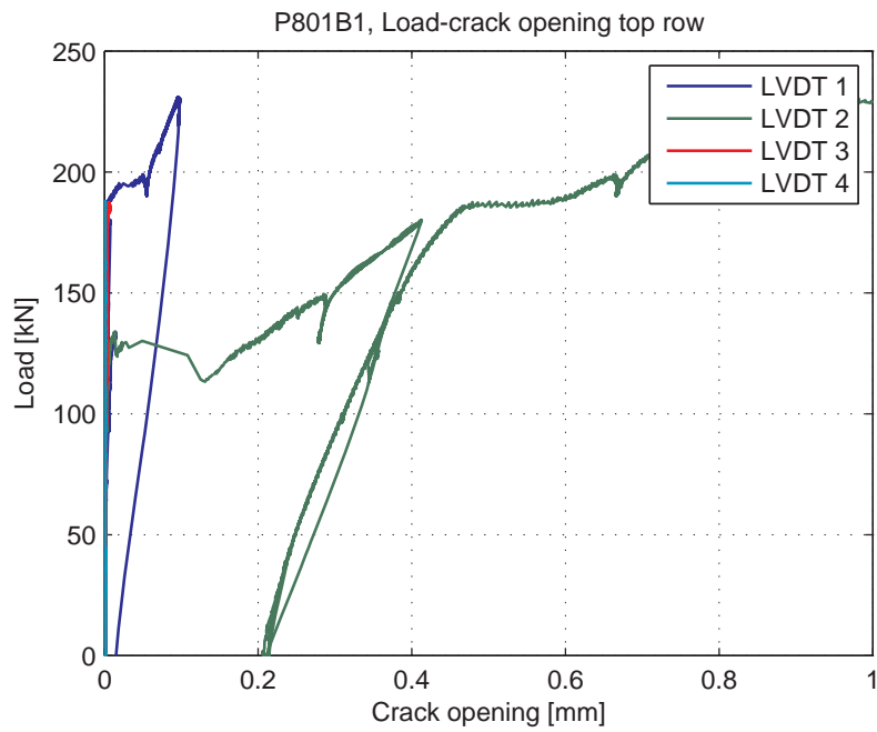
Fig. 5.86.7. Load-Crack opening for LVDT's 1-4 (top row)
