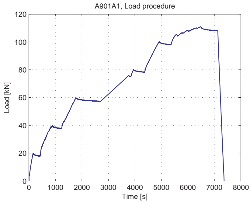
Fig. 5.12.3. Load-Time curve
