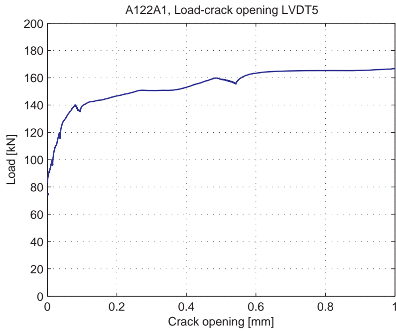
Fig. 5.5.8. Load-Crack opening for LVDT5
