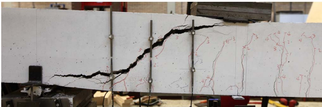
Fig. 5.68.1. Crack pattern after failure north side
