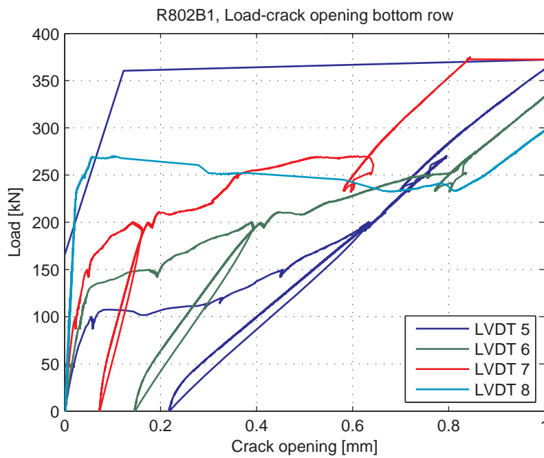
Fig. 5.103.8. Load-Crack opening for LVDT's 5-8 (bottom row)
