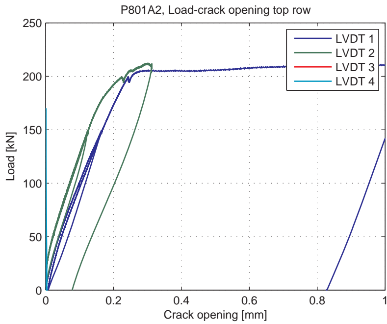
Fig. 5.84.5. Load-Crack opening for LVDT's 1-4 (top row)
