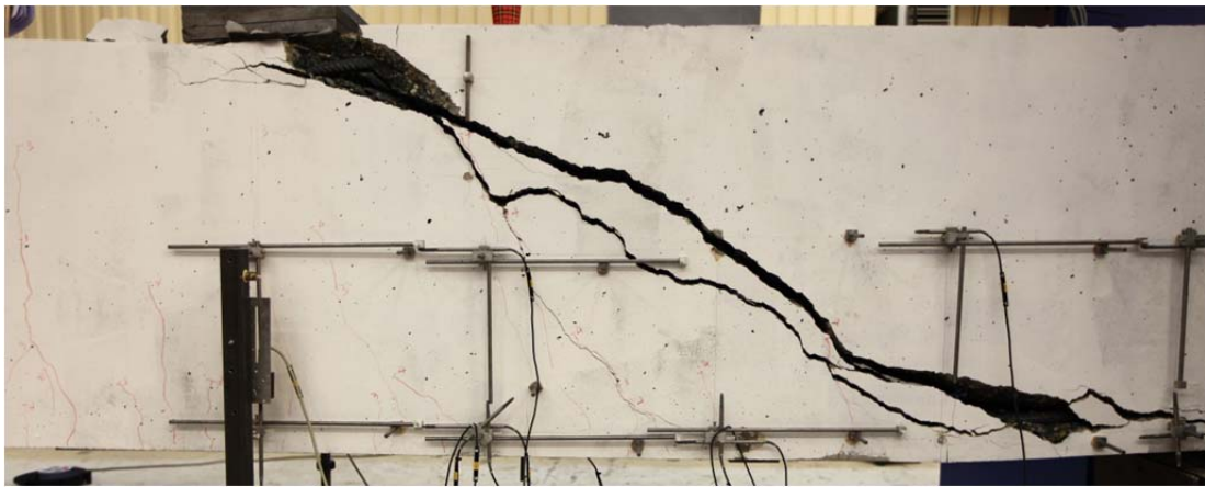
Fig. 5.103.2. Crack pattern after failure and LVDT layout at south side of beam
