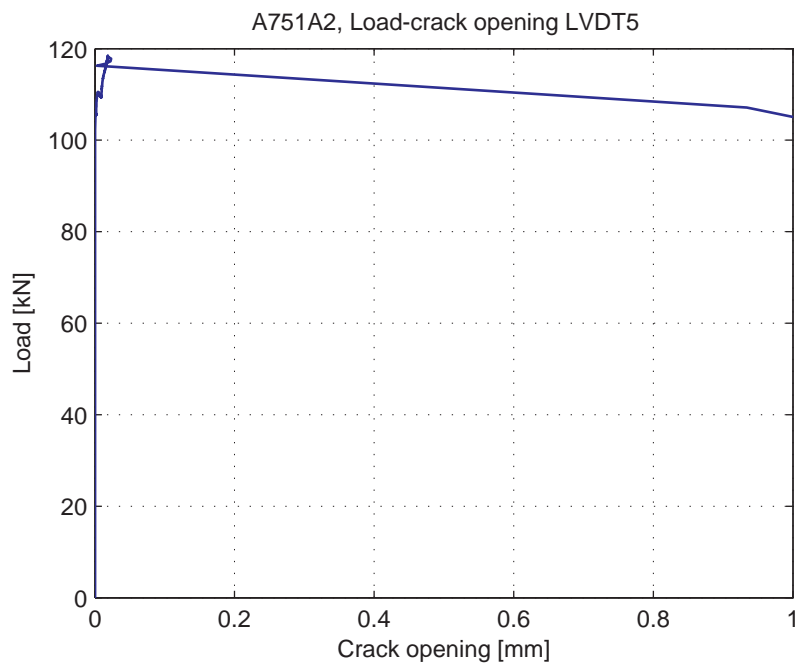
Fig. 5.23.8. Load-Crack opening for LVDT5
