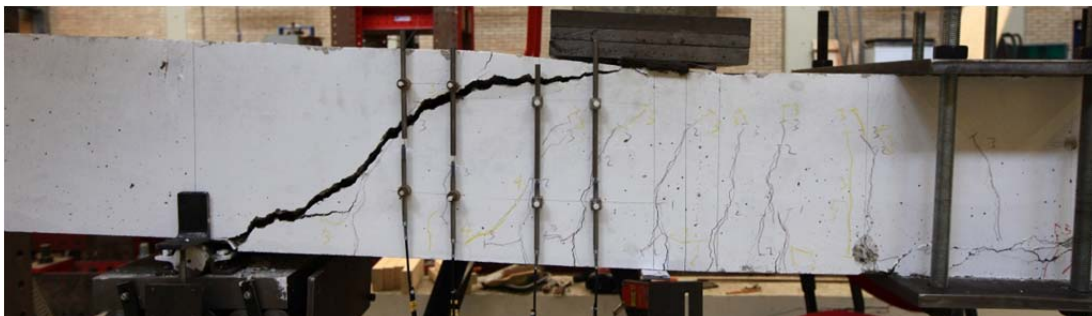
Fig. 5.70.1. Crack pattern after failure north side
