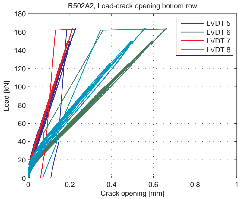
Fig. 5.98.7. Load-Crack opening for LVDT's 5-8 (bottom row)
