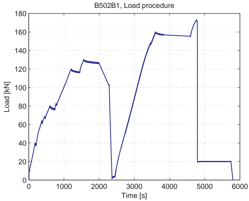
Fig. 5.53.3. Load-Time curve
