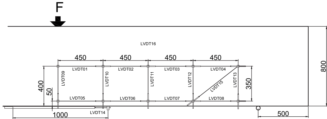
Fig. 5.94.3. LVDT layout and numbering for 800 mm deep beams
