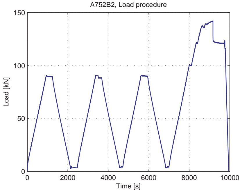
Fig. 5.30.3. Load-Time curve
