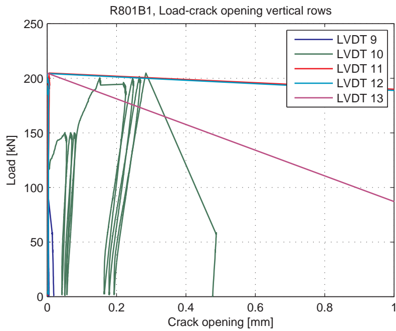
Fig. 5.101.7. Load-Crack opening for LVDT's 9-13 (vertical LVDT's)
