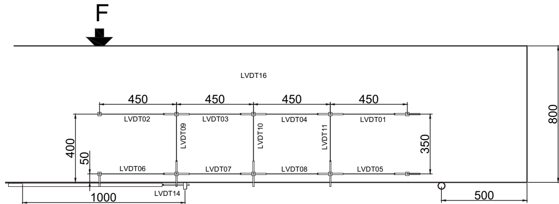
Fig. 5.93.2. LVDT layout and numbering for P804A2 beam
