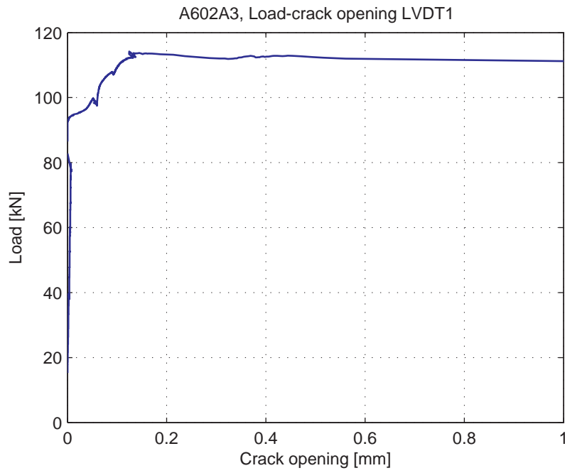
Fig. 5.37.5. Load-Crack opening for LVDT1
