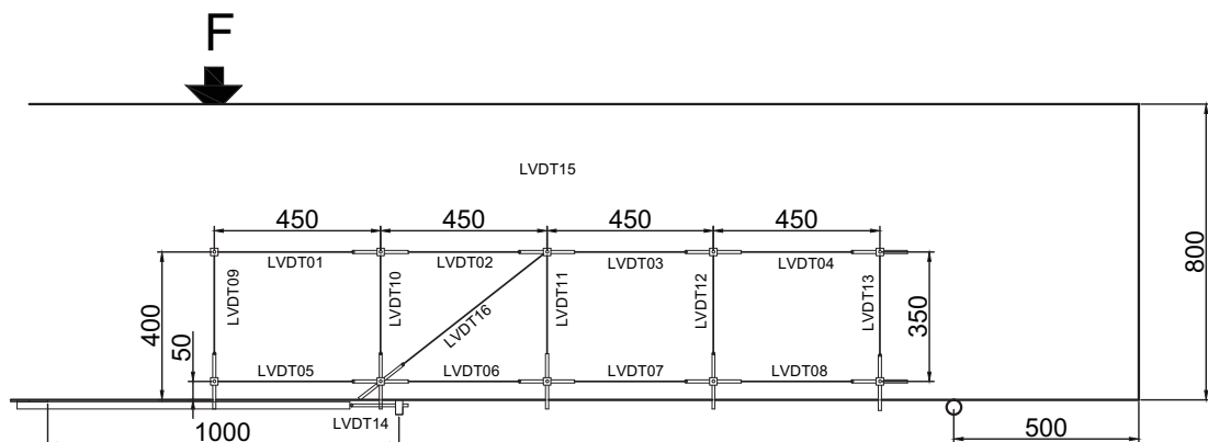
Fig. 5.83.2. LVDT layout and numbering for 800 mm deep beams
