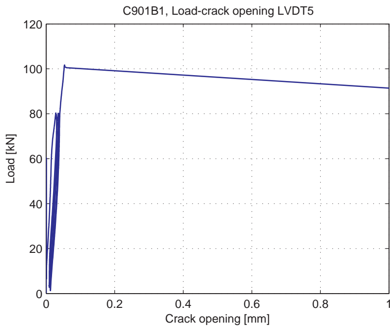
Fig. 5.57.8. Load-Crack opening for LVDT5
