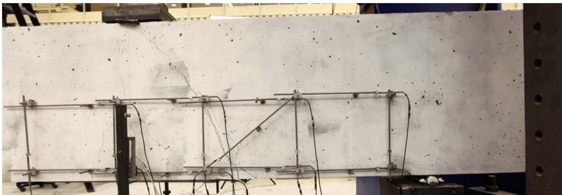
Fig. 5.86.2. Crack pattern after failure south side
