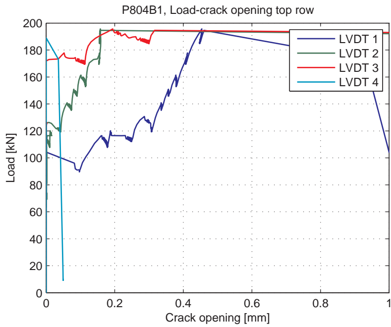
Fig. 5.94.6. Load-Crack opening for LVDT's 1-4 (top row)
