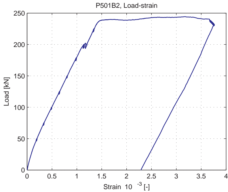
Fig. 5.79.9. Average strain over 1m length, measured at bottom of specimen (LVDT 14)
