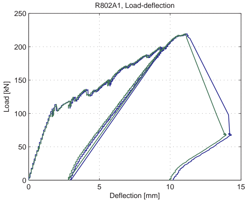
Fig. 5.102.5. Load-deflection curve
