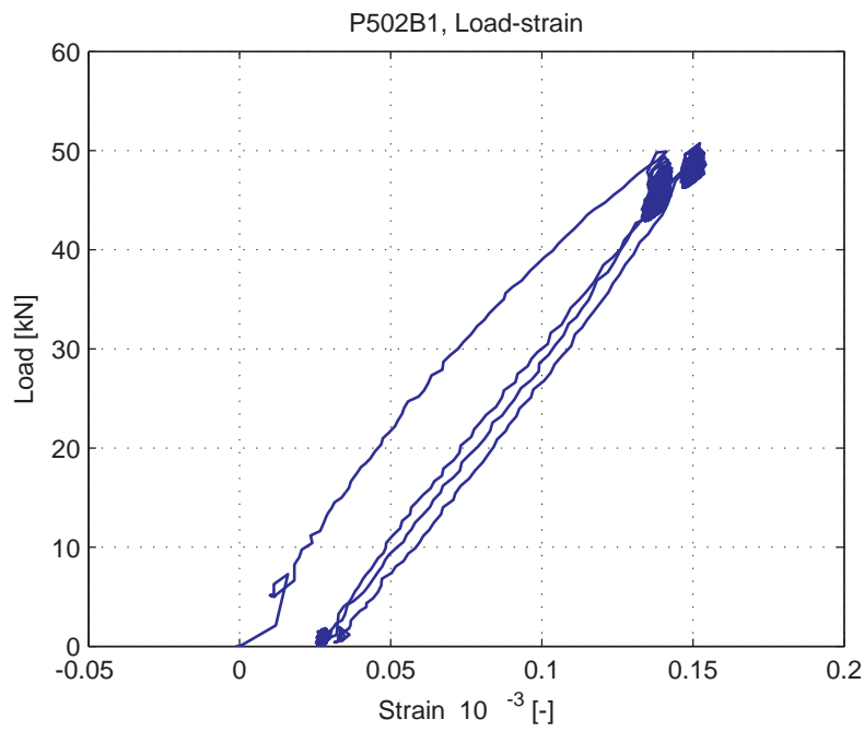
Fig. 5.82.13. Average strain over 1m length for first part of test, measured at bottom of specimen (LVDT 13)
