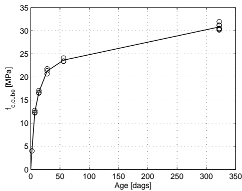
Fig. 2.2.5. F_{c,cube} development for cast 3
