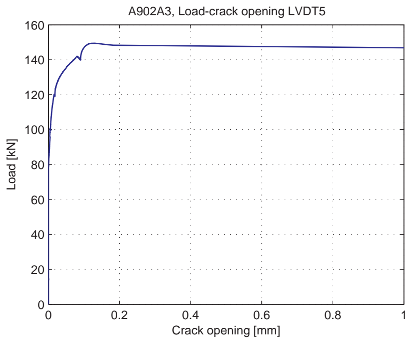
Fig. 5.19.8. Load-Crack opening for LVDT5
