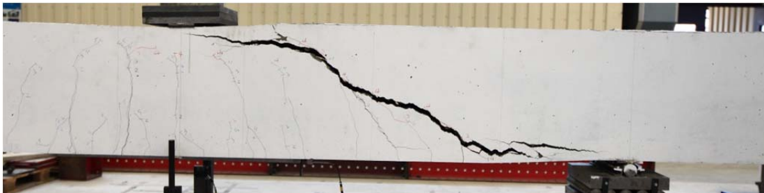
Fig. 5.48.2. Crack pattern after failure south side
