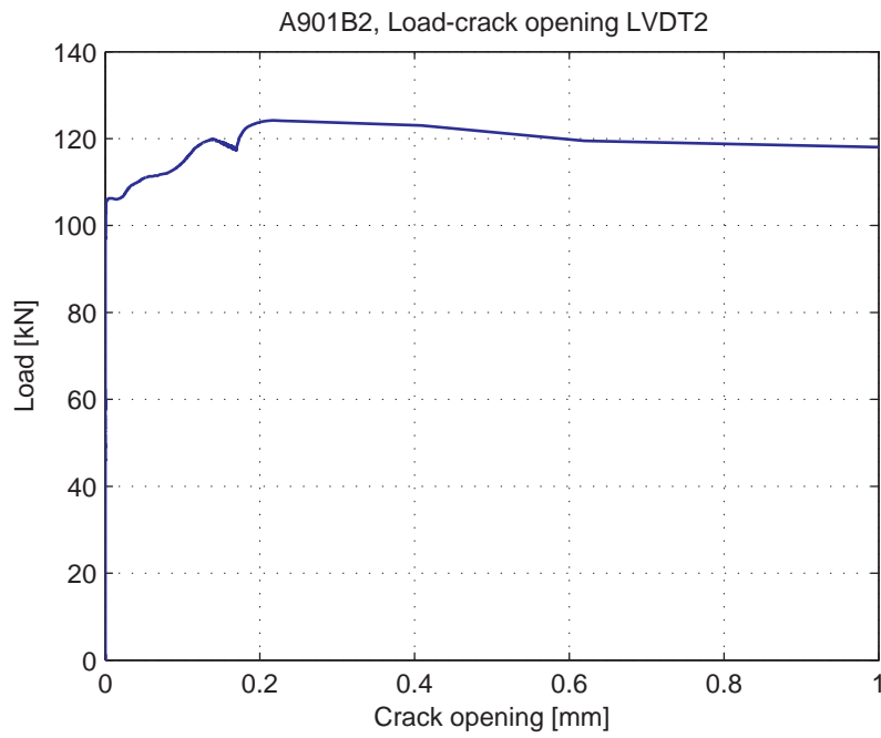
Fig. 5.16.6. Load-Crack opening for LVDT2
