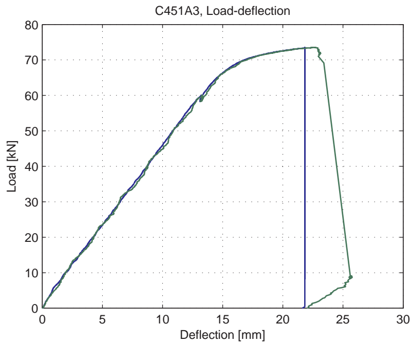
Fig. 5.64.4. Load-deflection curve
