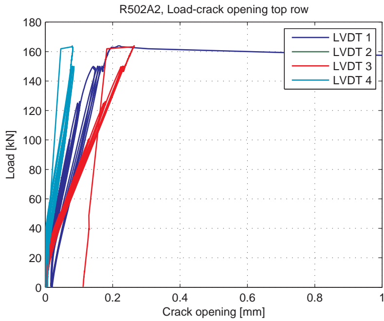
Fig. 5.98.5. Load-Crack opening for LVDT's 1-4 (top row)
