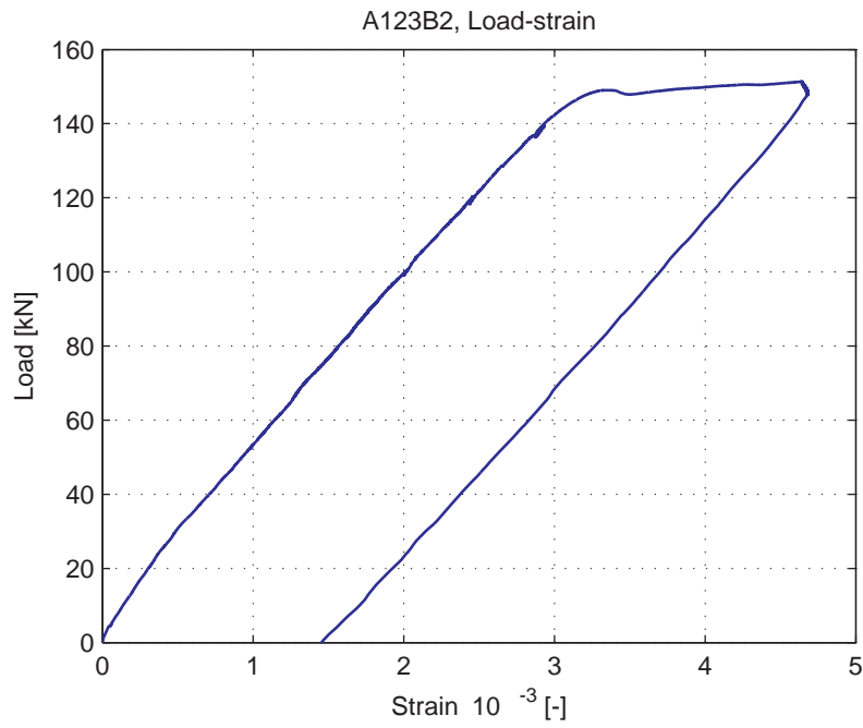
Fig. 5.11.9. Average strain over 1m length, measured at bottom of specimen (LVDT 3)
