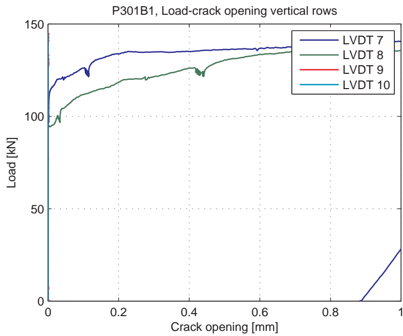
Fig. 5.75.7. Load-Crack opening for LVDT's 7-10 (vertical LVDT's)
