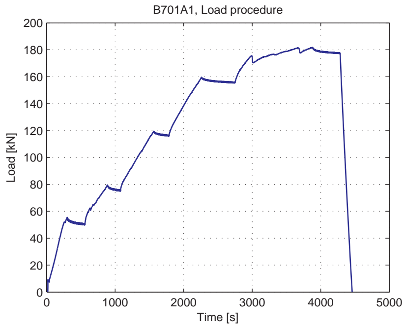
Fig. 5.40.3. Load-Time curve
