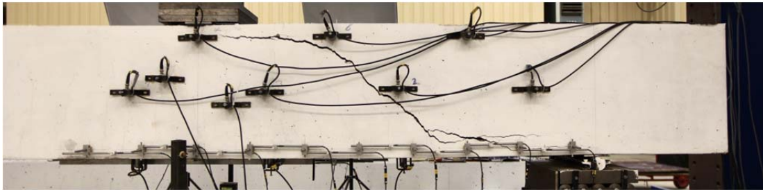
Fig. 5.96.2. Crack pattern after failure south side and sensors used for Acoustic Emissions measurements
