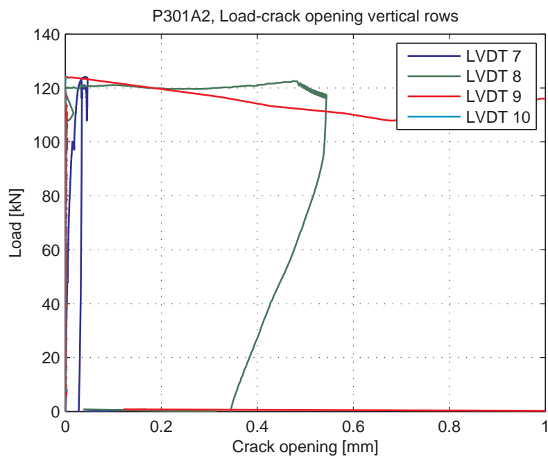
Fig. 5.72.7. Load-Crack opening for LVDT's 7-10 (vertical LVDT's)
