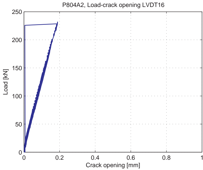
Fig. 5.93.11. Load-Crack opening for LVDT 16
