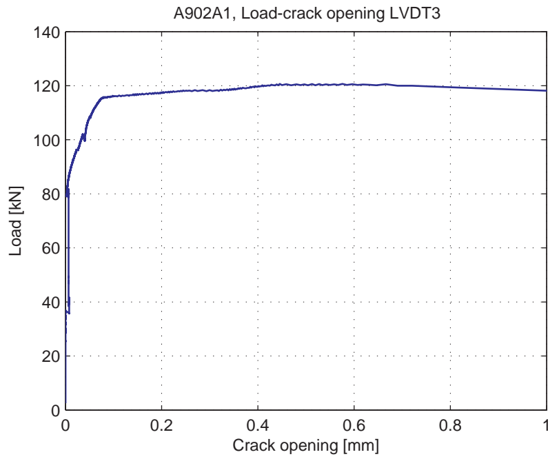
Fig. 5.17.7. Load-Crack opening for LVDT3
