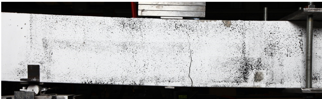
Fig. 5.73.1. Crack pattern after failure front side
