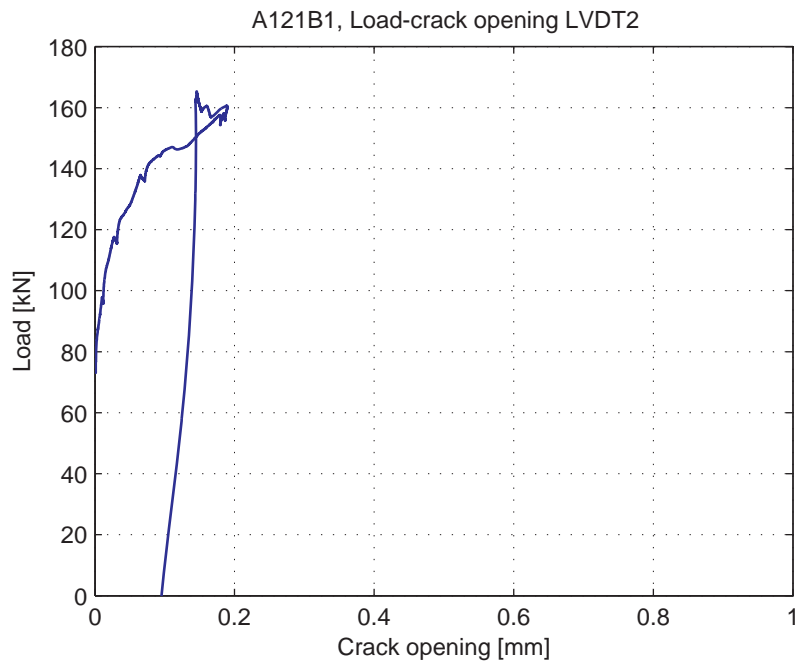
Fig. 5.4.6. Load-Crack opening for LVDT2
