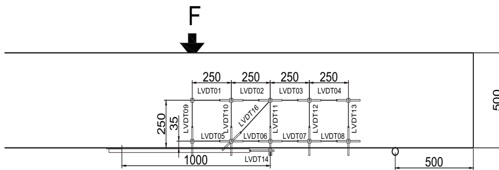
Fig. 5.95.3. LVDT layout and numbering for 500 mm deep beams
