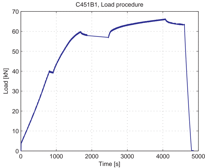
Fig. 5.67.3. Load-Time curve
