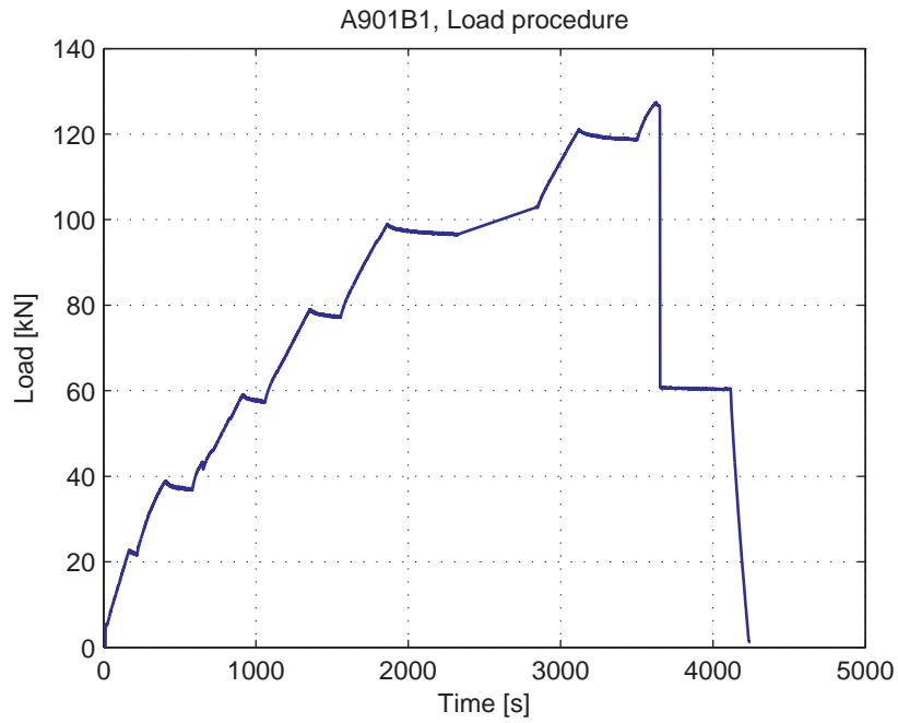
Fig. 5.15.3. Load-Time curve
