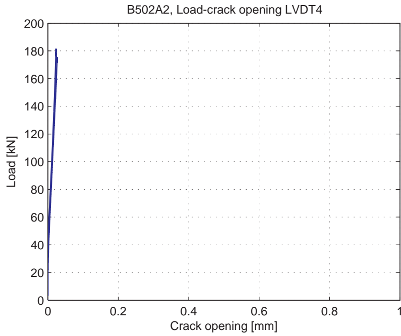
Fig. 5.51.5. Load-Crack opening for LVDT4
