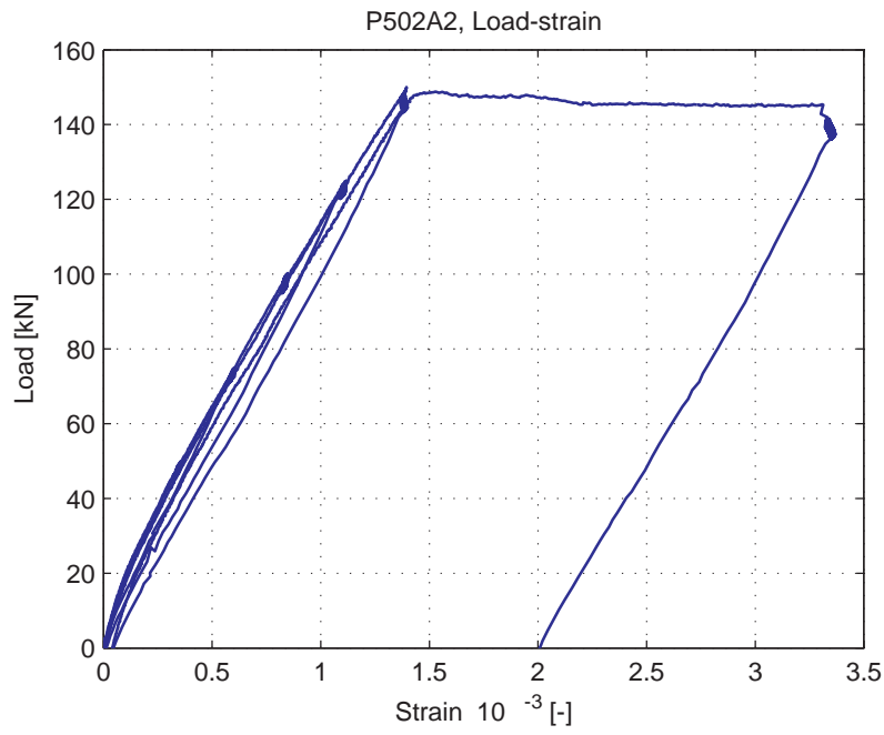
Fig. 5.81.9. Average strain over 1m length, measured at bottom of specimen (LVDT 14)
