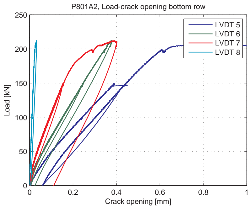
Fig. 5.84.7. Load-Crack opening for LVDT's 5-8 (bottom row)
