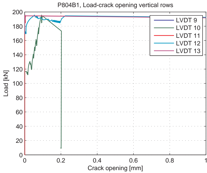
Fig. 5.94.7. Load-Crack opening for LVDT's 9-13 (vertical LVDT's)
