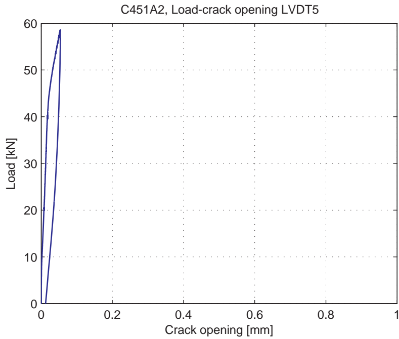
Fig. 5.63.6. Load-Crack opening for LVDT5
