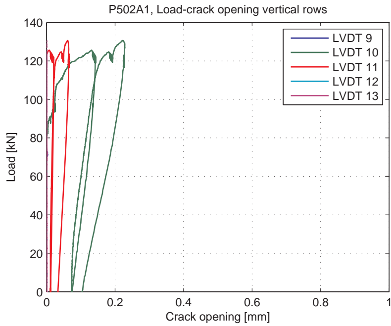
Fig. 5.80.7. Load-Crack opening for LVDT's 9-13 (vertical LVDT's)
