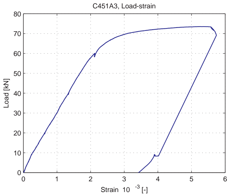
Fig. 5.64.8. Average strain over 1m length, measured at bottom of specimen (LVDT 3)
