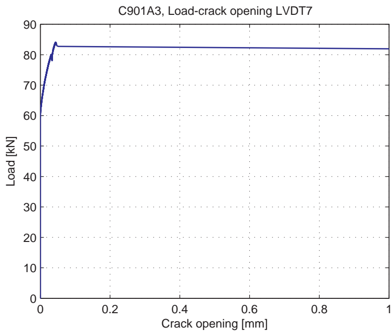
Fig. 5.56.8. Load-Crack opening for LVDT7
