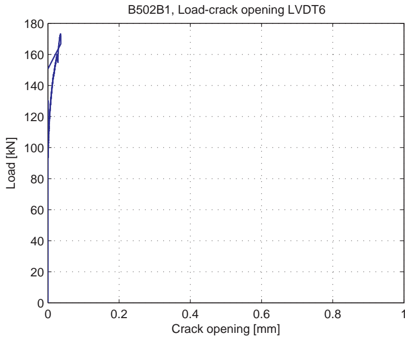
Fig. 5.53.7. Load-Crack opening for LVDT6
