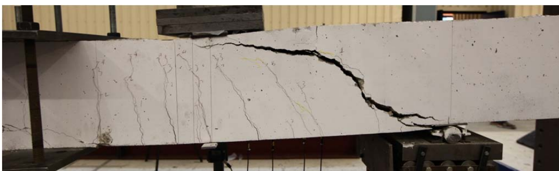
Fig. 5.70.2. Crack pattern after failure south side
