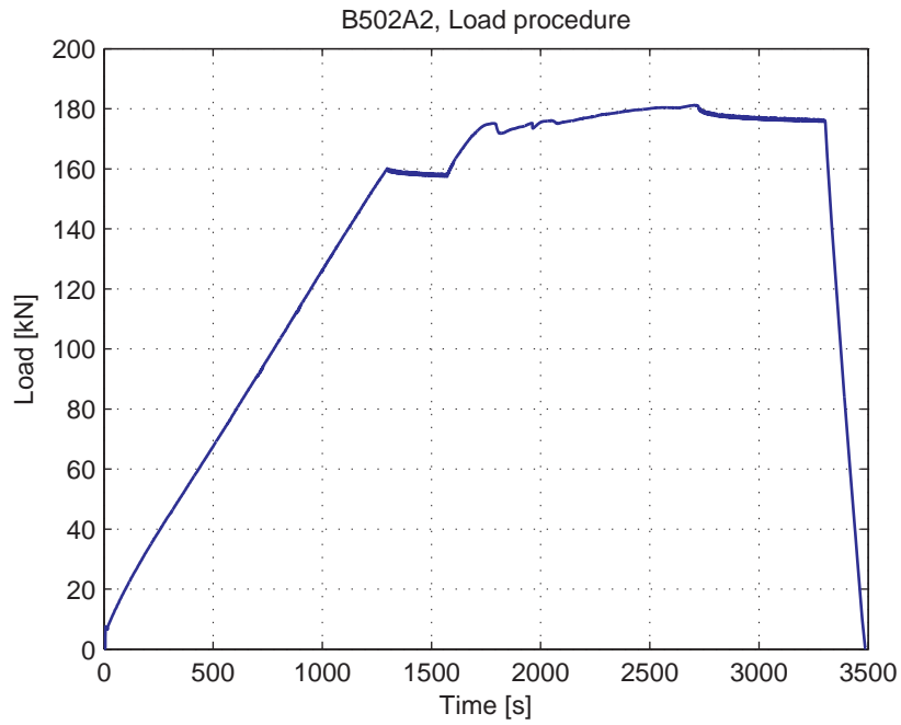
Fig. 5.51.3. Load-Time curve
