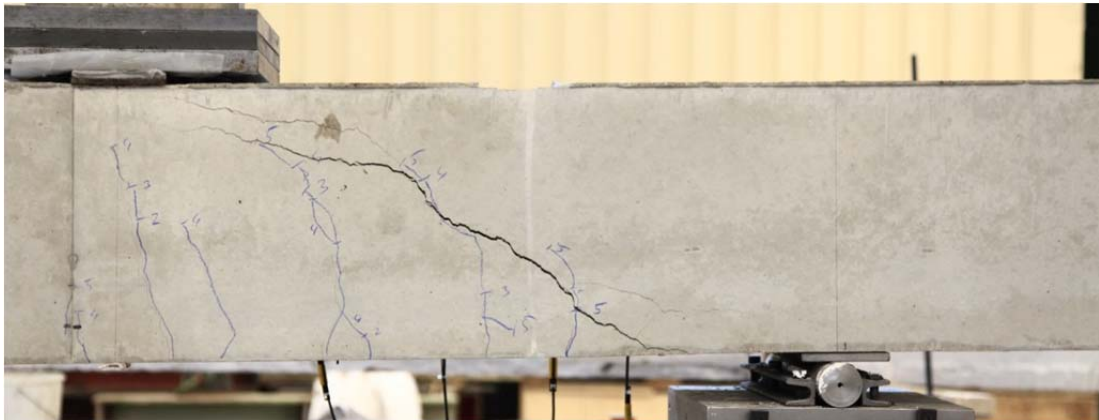
Fig. 5.24.2. Crack pattern after failure south side
