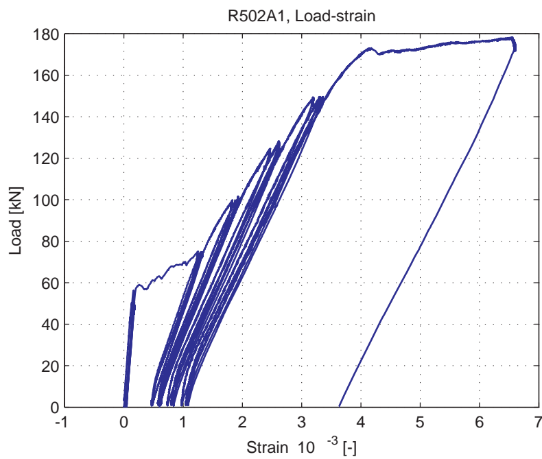
Fig. 5.97.11. Average strain over 1m length, measured at bottom of specimen (LVDT 14)
