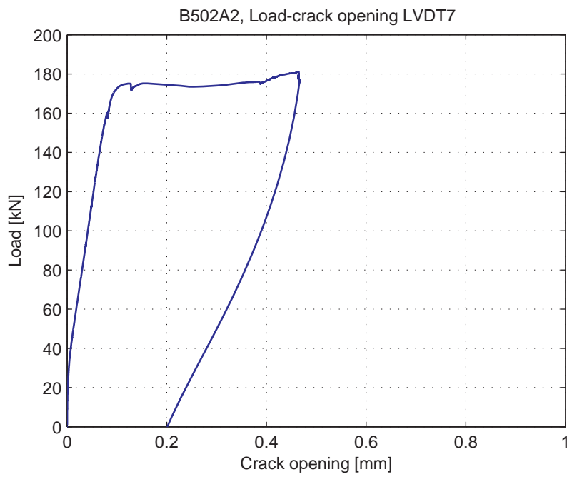
Fig. 5.51.8. Load-Crack opening for LVDT7
