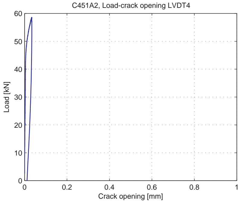
Fig. 5.63.5. Load-Crack opening for LVDT4
