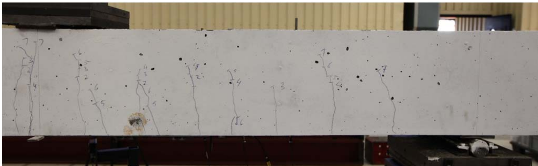
Fig. 5.10.2. Crack pattern after failure south side
