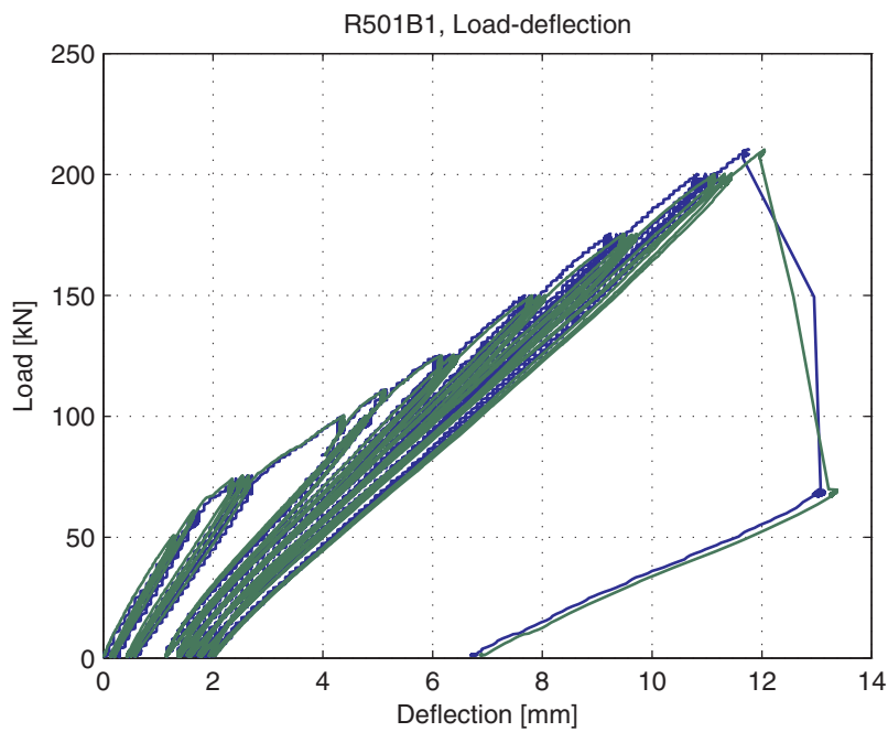
Fig. 5.96.5. Load-deflection curve
