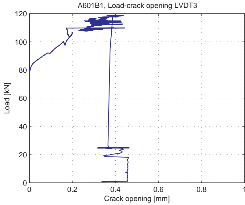
Fig. 5.33.7. Load-Crack opening for LVDT3
