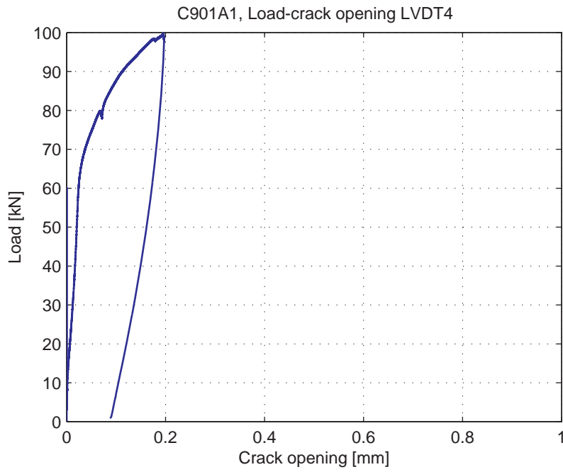
Fig. 5.54.3. Load-Crack opening for LVDT4
