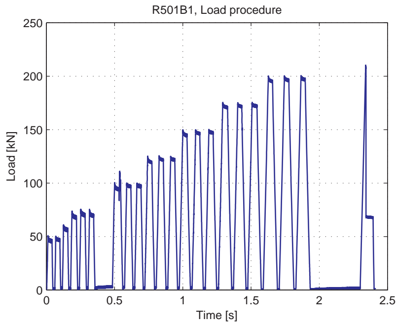
Fig. 5.96.4. Load-Time curve
