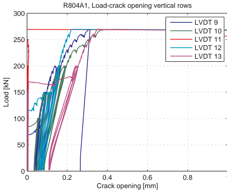
Fig. 5.106.7. Load-Crack opening for LVDT's 9-13 (vertical LVDT's)
