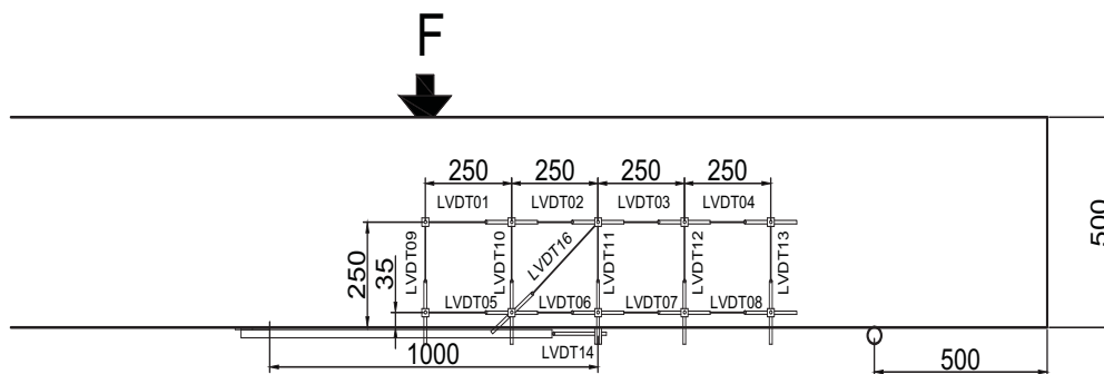
Fig. 5.82.3. LVDT layout and numbering for 500 mm deep beams
