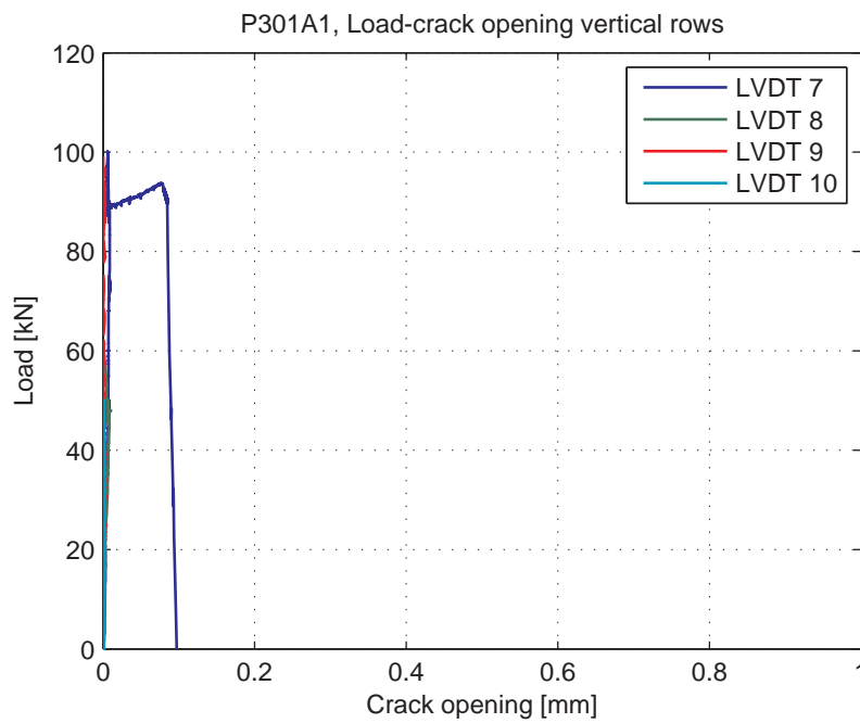
Fig. 5.71.6. Load-Crack opening for LVDT's 7-10 (vertical LVDT's)
