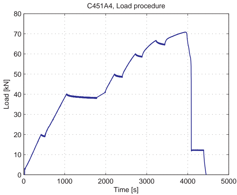
Fig. 5.65.3. Load-Time curve
