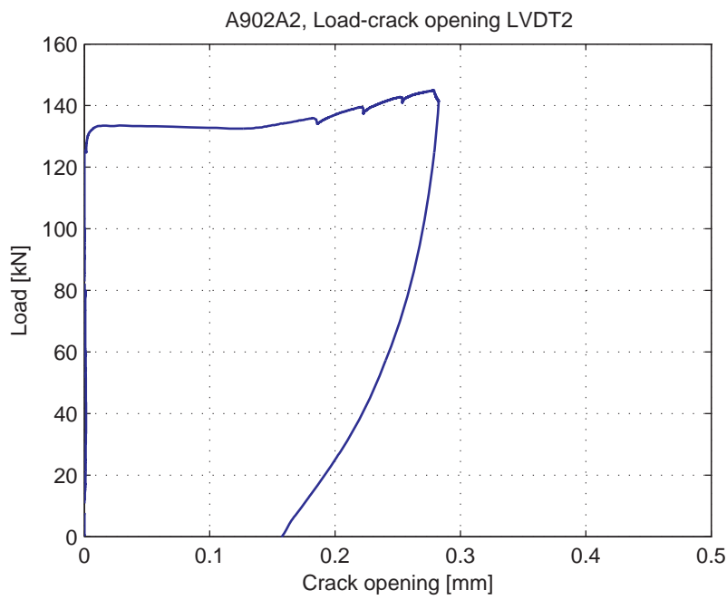
Fig. 5.18.6. Load-Crack opening for LVDT2
