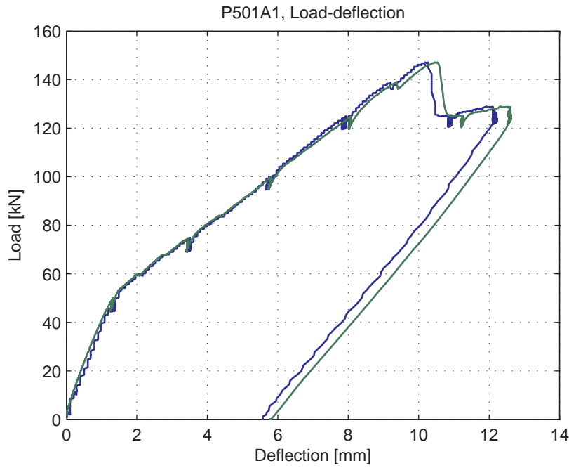
Fig. 5.76.5. Load-deflection curve
