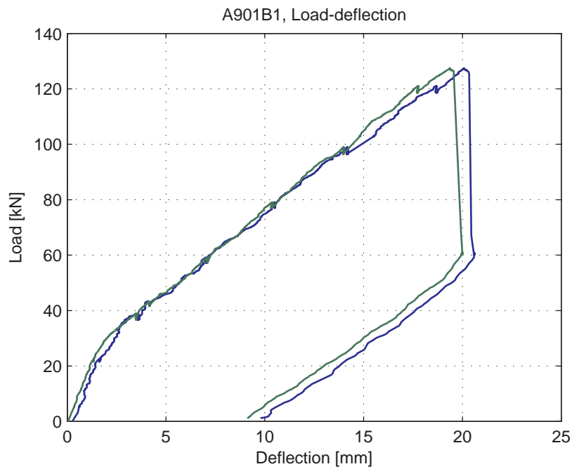
Fig. 5.15.4. Load-deflection curve
