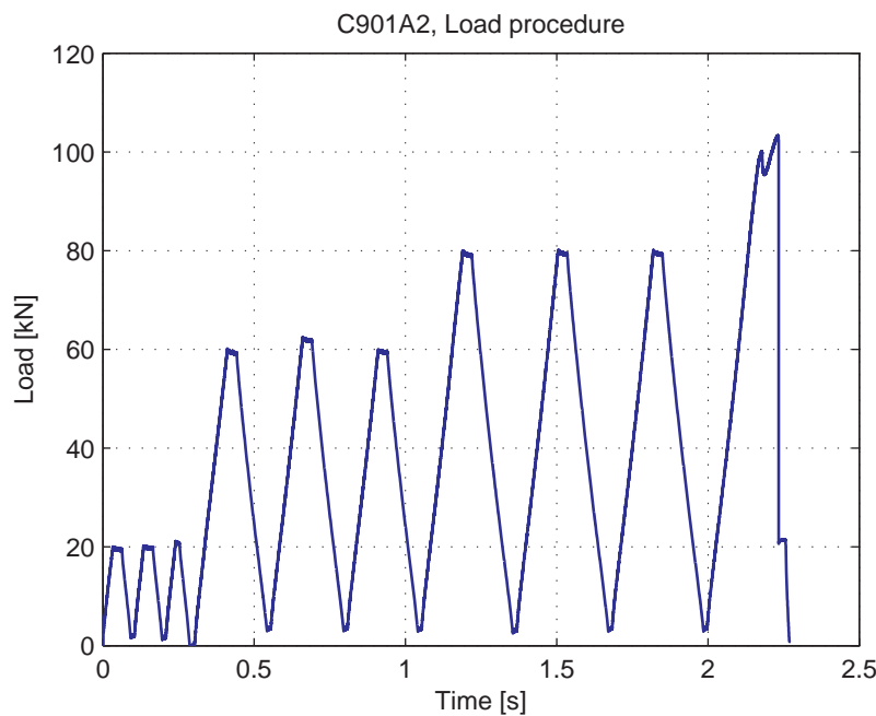
Fig. 5.55.3. Load-Time curve
