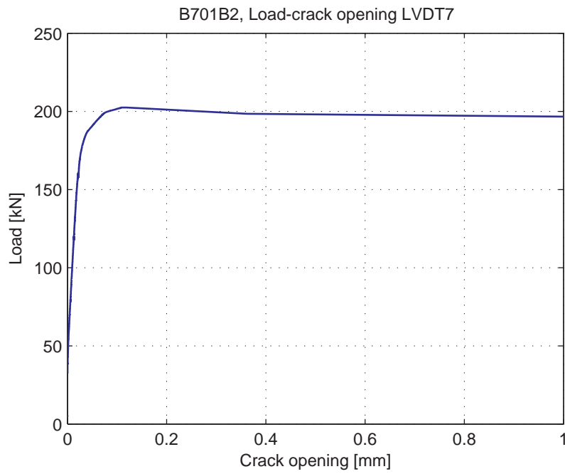
Fig. 5.44.8. Load-Crack opening for LVDT7
