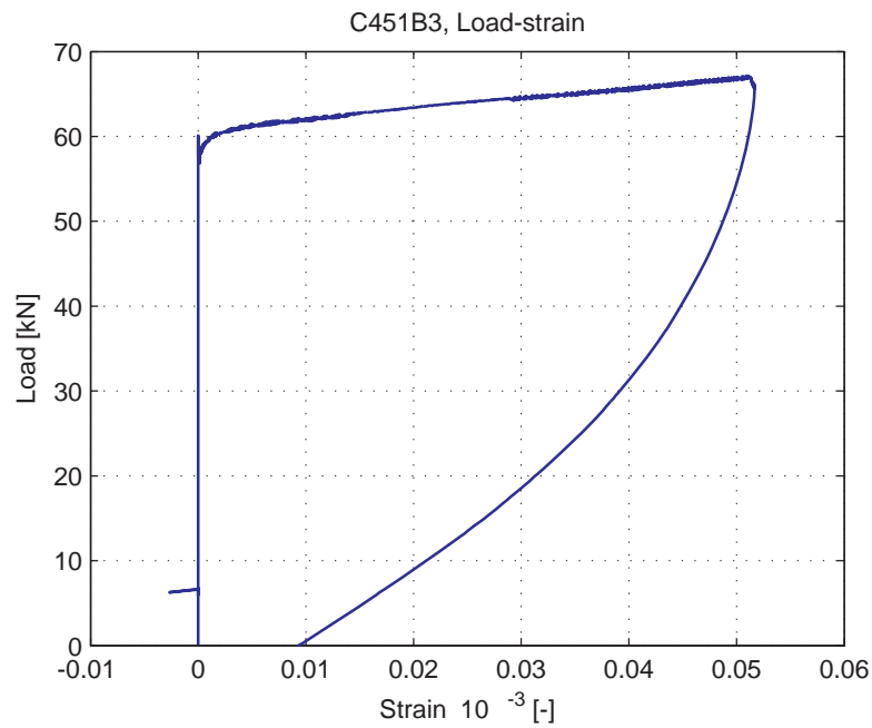
Fig. 5.69.9. Average strain over 1m length, measured at bottom of specimen (LVDT 3)
