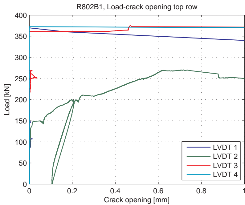
Fig. 5.103.6. Load-Crack opening for LVDT's 1-4 (top row)
