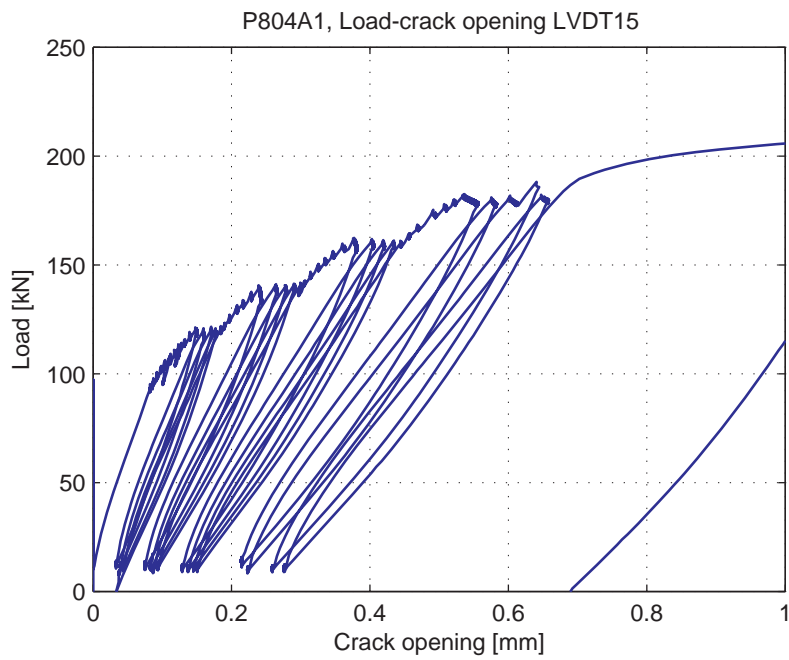
Fig. 5.92.11. Load-Crack opening for LVDT 15
