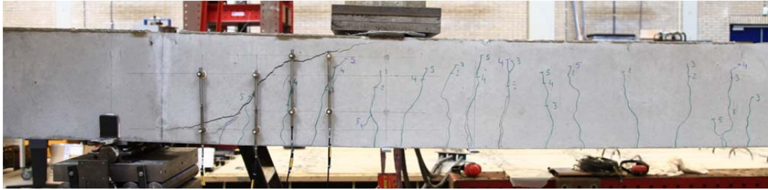
Fig. 5.23.1. Crack pattern after failure north side
