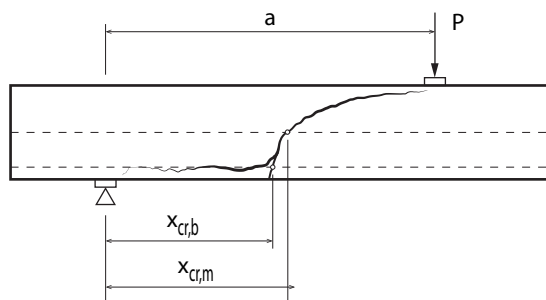
Fig. 3.2.5. Definition of shear crack location at bottom reinforcement of specimen ( x_{cr,b} ) and centre of the specimen ( x_{cr,m} ).
