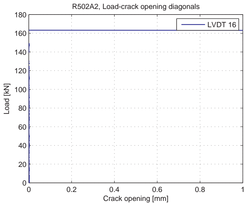
Fig. 5.98.8. Load-Crack opening for LVDT 16 (diagonal)
