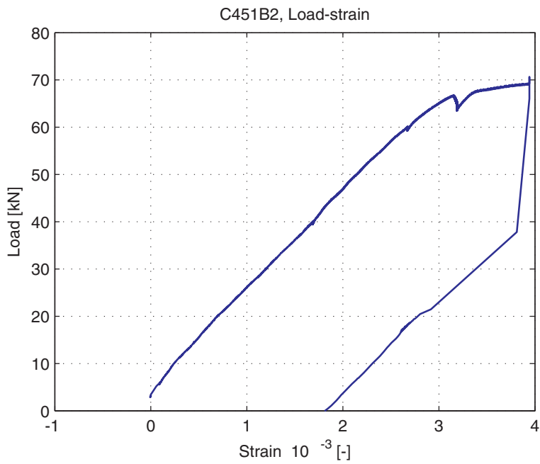
Fig. 5.68.8. Average strain over 1m length, measured at bottom of specimen (LVDT 3)
