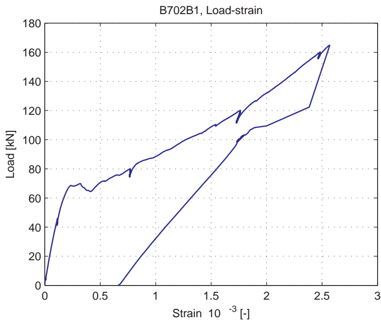
Fig. 5.46.8. Average strain over 1m length, measured at bottom of specimen (LVDT 3)
