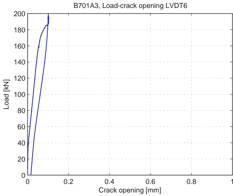
Fig. 5.42.7. Load-Crack opening for LVDT6
