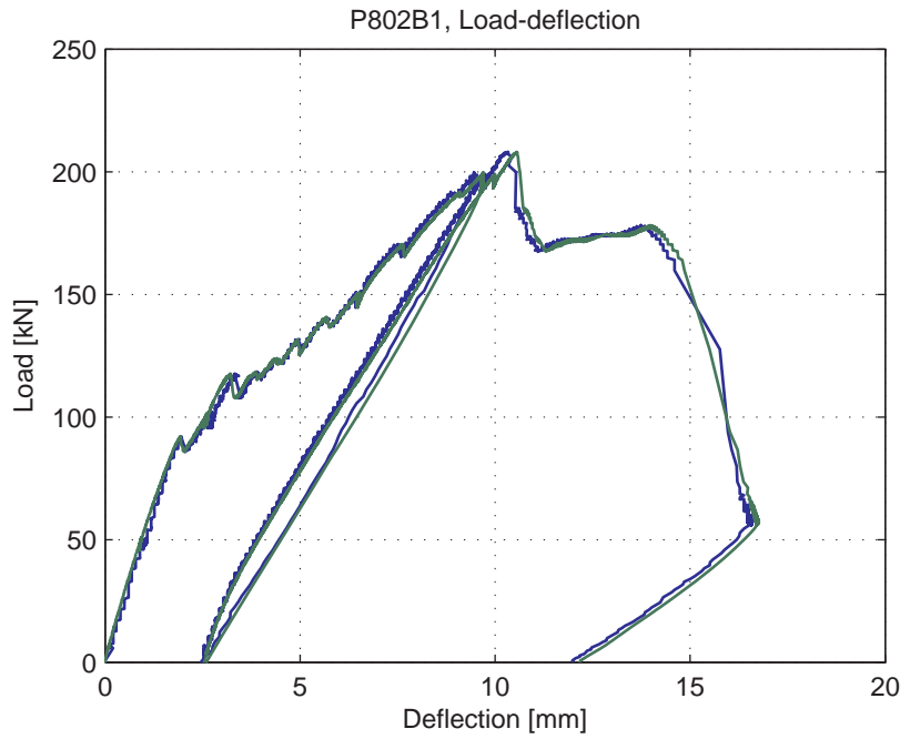
Fig. 5.88.5. Load-deflection curve
