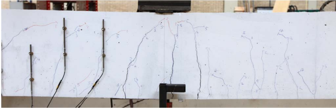
Fig. 5.51.1. Crack pattern after failure north side
