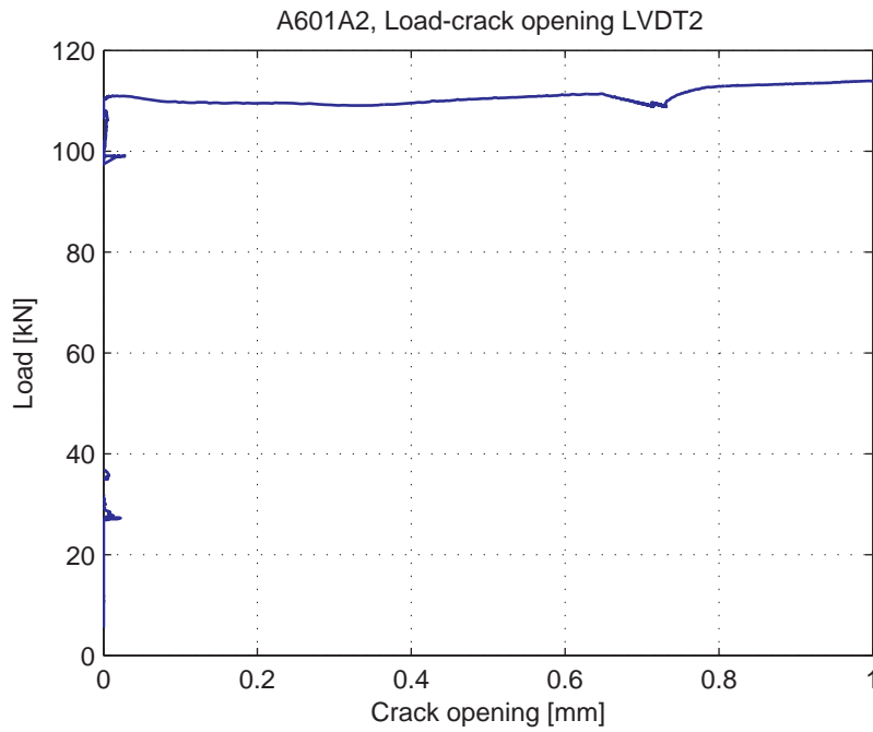
Fig. 5.32.6. Load-Crack opening for LVDT2
