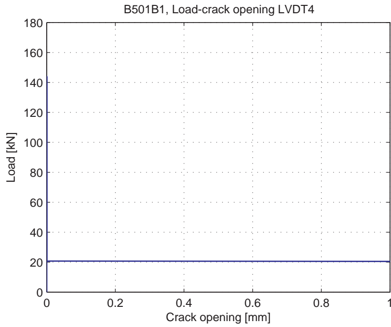
Fig. 5.49.5. Load-Crack opening for LVDT4
