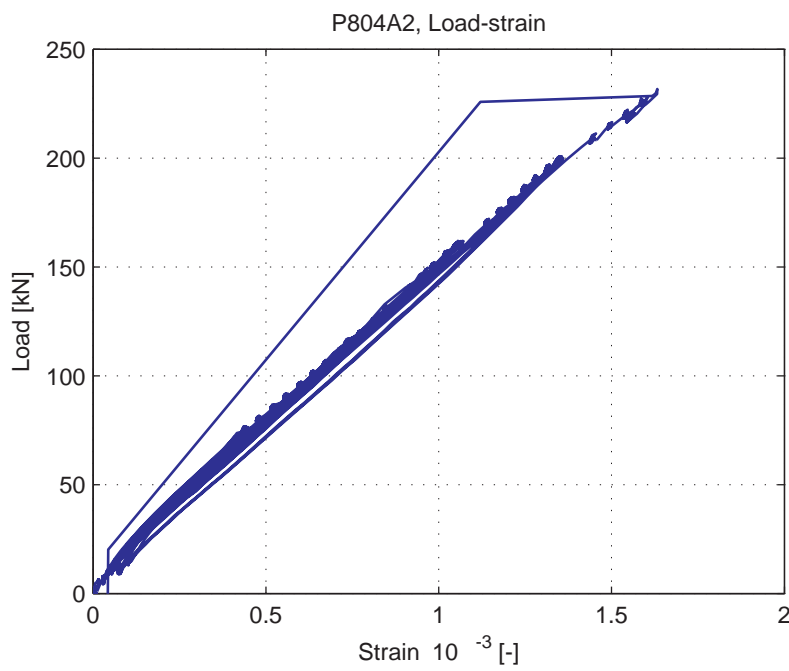
Fig. 5.93.12. Average strain over 1m length, measured at bottom of specimen (LVDT 14)
