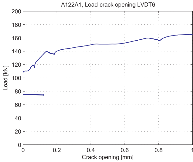
Fig. 5.5.9. Load-Crack opening for LVDT6
