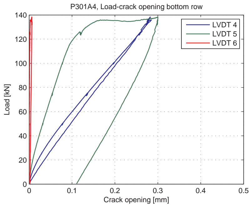
Fig. 5.74.8. Load-Crack opening for LVDT's 4-6 (bottom row)
