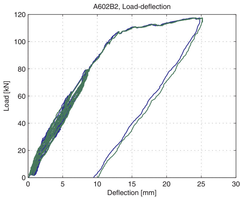
Fig. 5.39.4. Load-deflection curve
