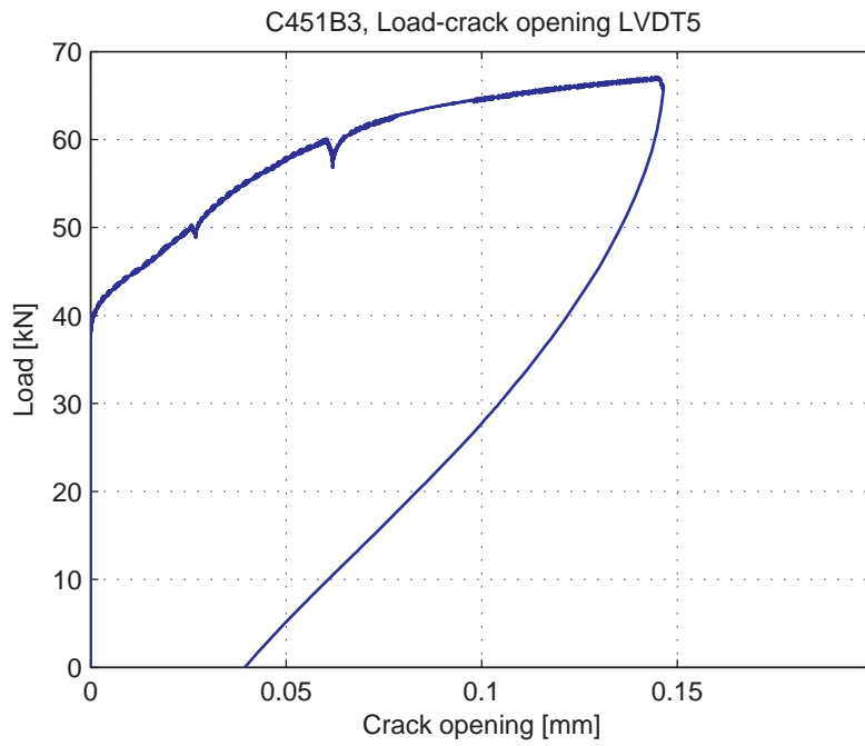
Fig. 5.69.7. Load-Crack opening for LVDT5
