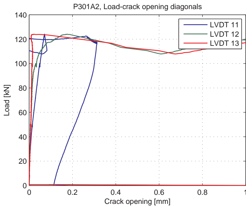
Fig. 5.72.9. Load-Crack opening for LVDT's 11-13 (diagonal)
