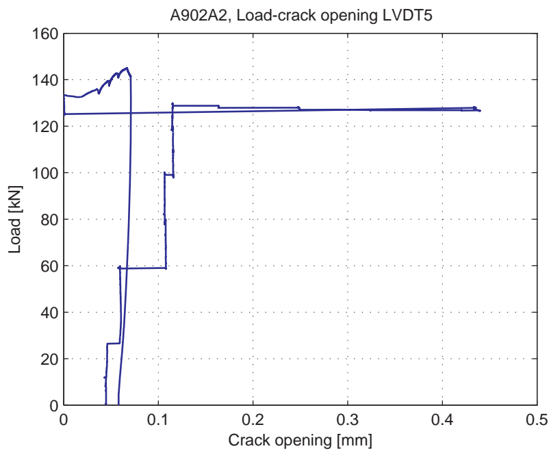
Fig. 5.18.8. Load-Crack opening for LVDT5
