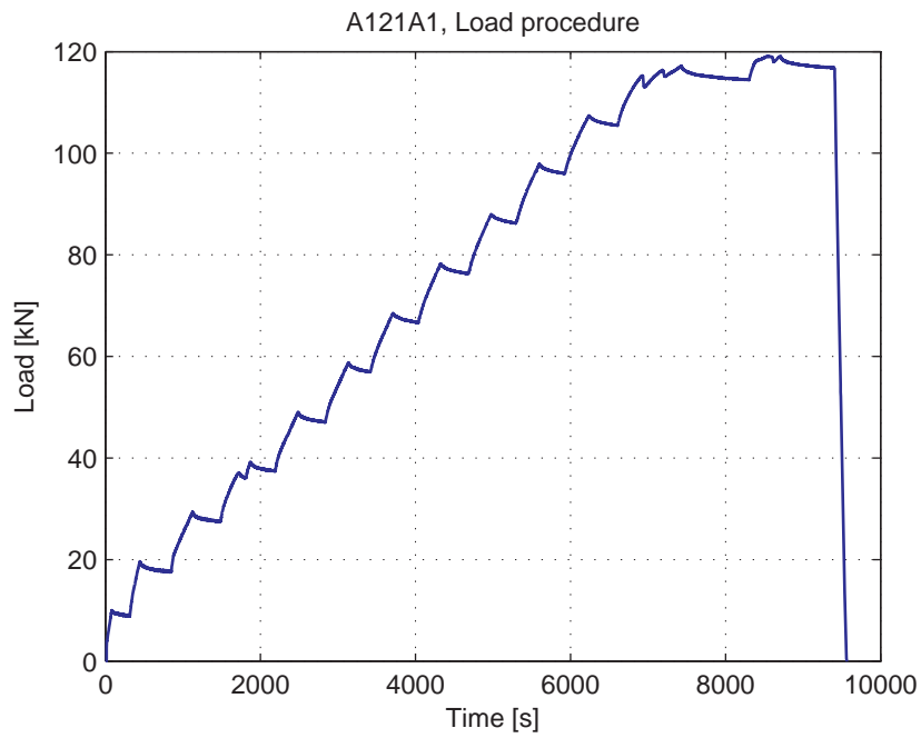
Fig. 5.1.3. Load-Time curve
