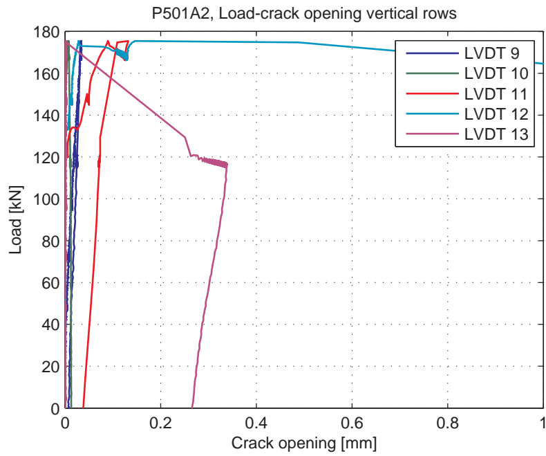
Fig. 5.77.7. Load-Crack opening for LVDT's 9-13 (vertical LVDT's)
