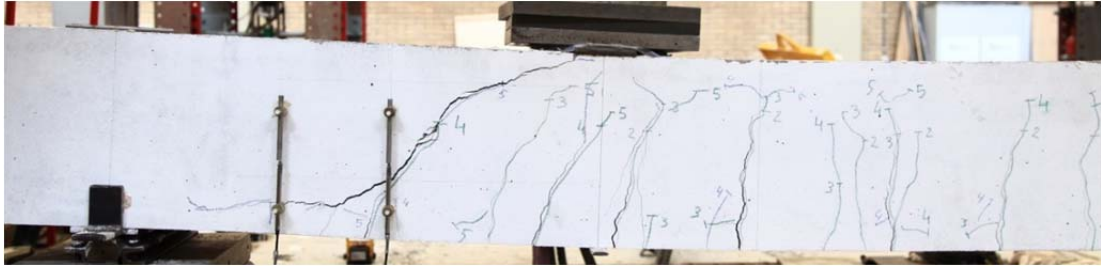
Fig. 5.32.1. Crack pattern after failure north side
