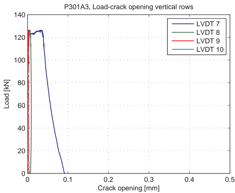
Fig. 5.73.7. Load-Crack opening for LVDT's 7-10 (vertical LVDT's)
