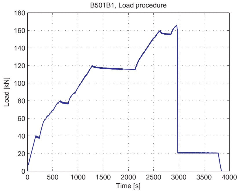
Fig. 5.49.3. Load-Time curve
