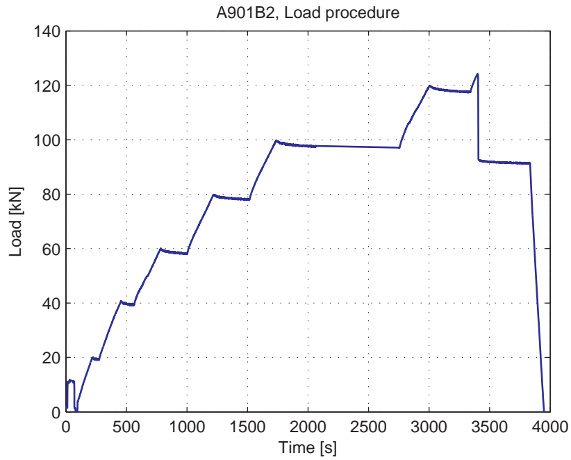
Fig. 5.16.3. Load-Time curve
