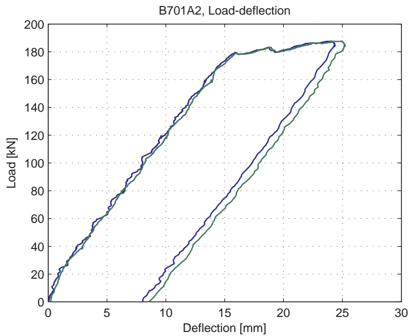
Fig. 5.41.4. Load-deflection curve
