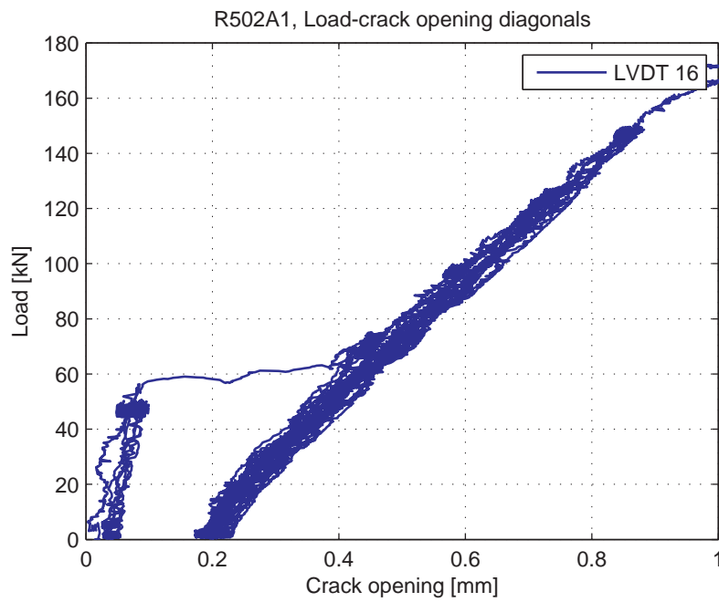
Fig. 5.97.9. Load-Crack opening for LVDT 16 (diagonal)
