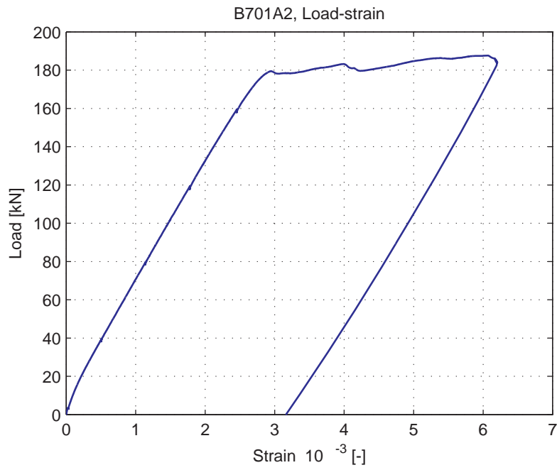
Fig. 5.41.5. Average strain over 1m length, measured at bottom of specimen (LVDT 3)
