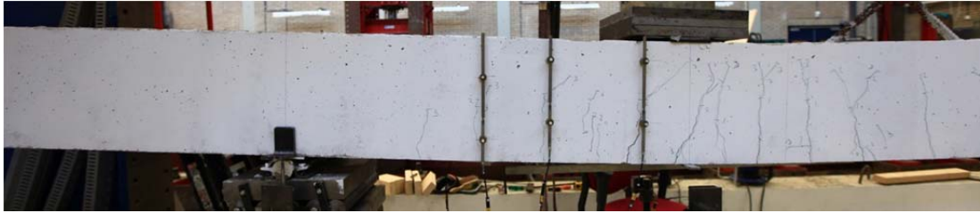
Fig. 5.63.1. Crack pattern after failure north side
