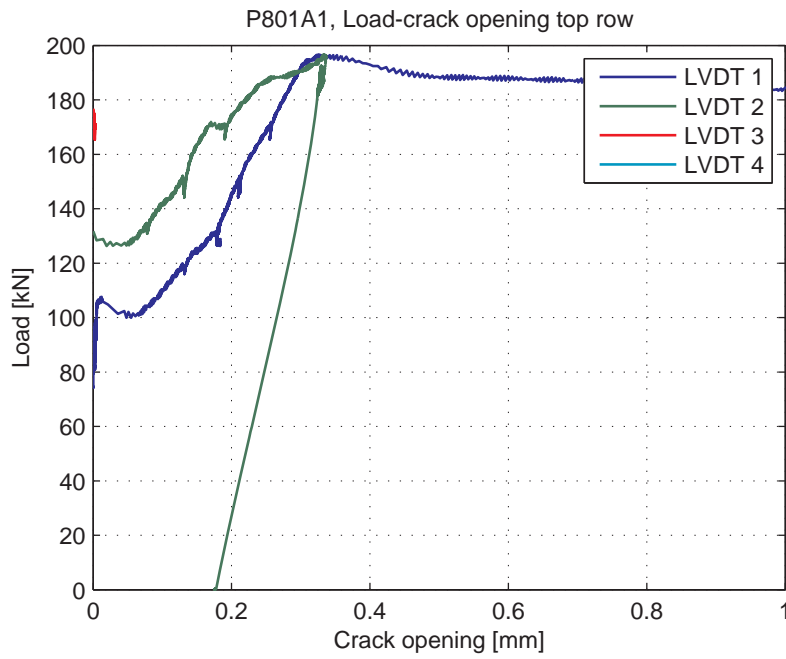
Fig. 5.83.5. Load-Crack opening for LVDT's 1-4 (top row)
