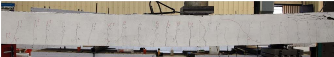
Fig. 5.18.2. Crack pattern after failure south side
