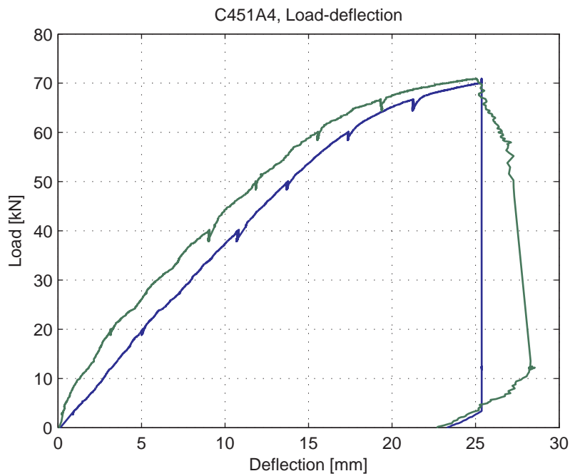
Fig. 5.65.4. Load-deflection curve
