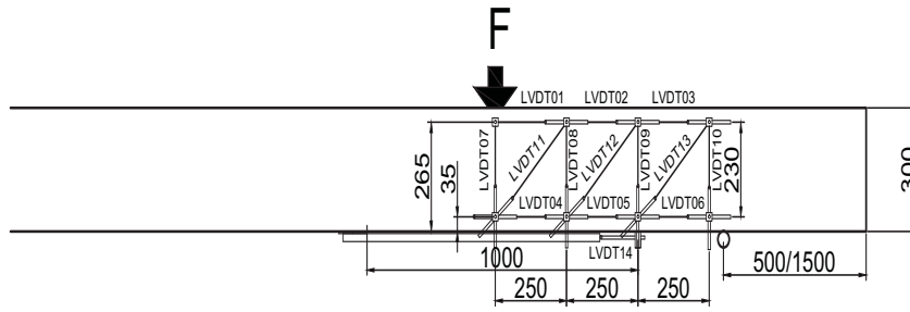
Fig. 5.73.3. LVDT layout and numbering for 300 mm deep beams
