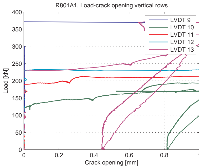
Fig. 5.100.7. Load-Crack opening for LVDT's 9-13 (vertical LVDT's)
