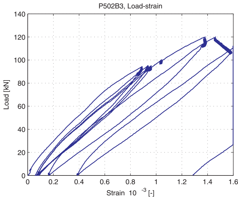
Fig. 5.82.15. Average strain over 1m length for third part of test, measured at bottom of specimen (LVDT 13)
