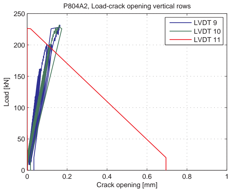
Fig. 5.93.6. Load-Crack opening for LVDT's 9-11 (vertical LVDT's)
