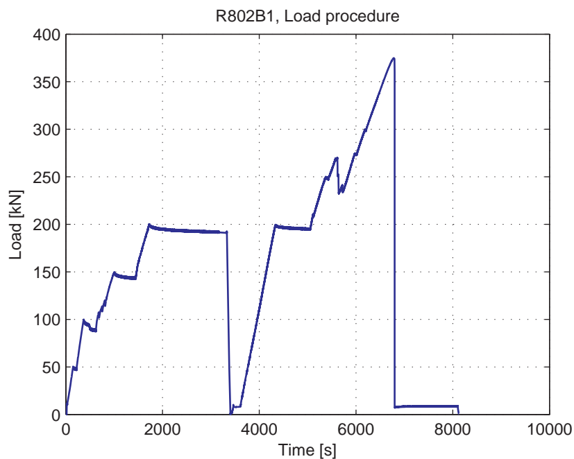
Fig. 5.103.4. Load-Time curve
