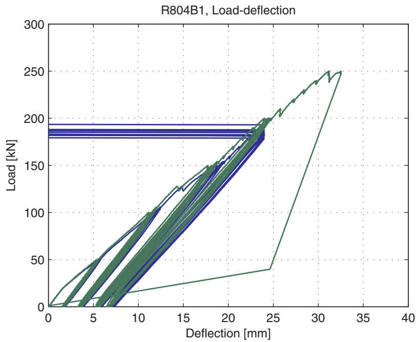
Fig. 5.107.5. Load-deflection curve
