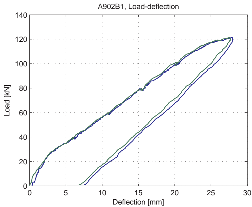
Fig. 5.20.4. Load-deflection curve
