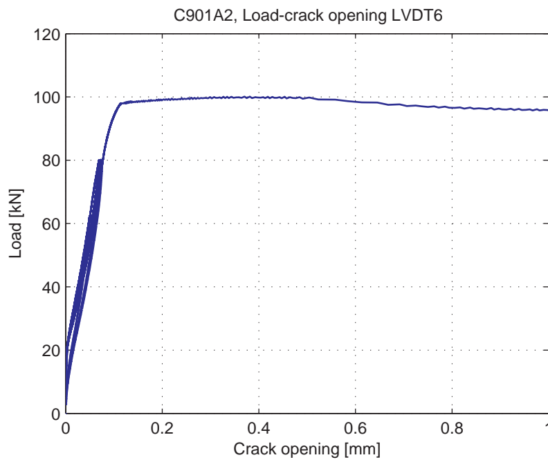
Fig. 5.55.7. Load-Crack opening for LVDT6
