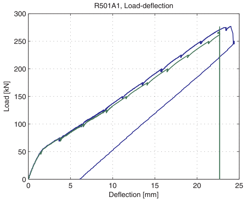
Fig. 5.95.5. Load-deflection curve
