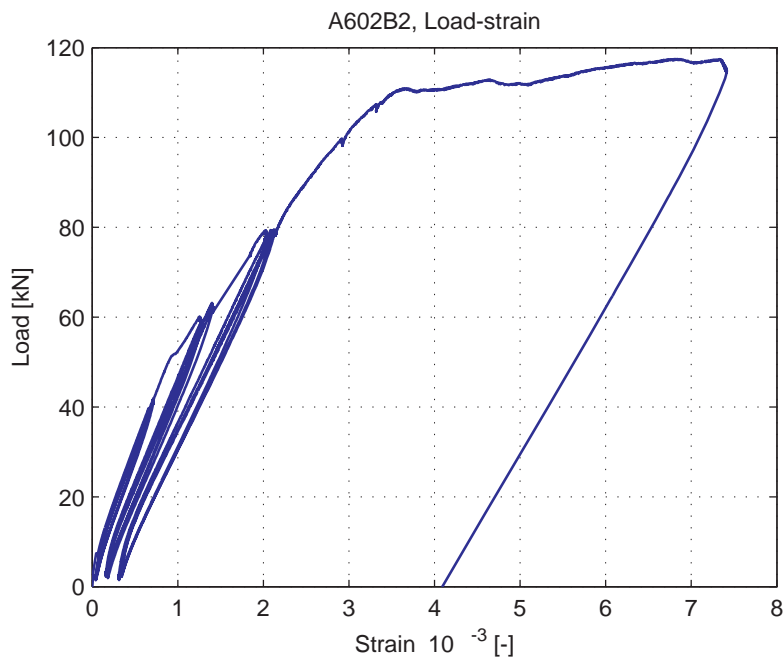
Fig. 5.39.8. Average strain over 1m length, measured at bottom of specimen (LVDT 3)
