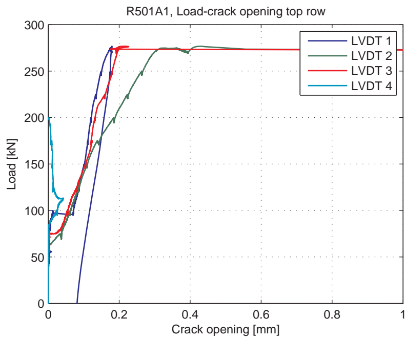
Fig. 5.95.6. Load-Crack opening for LVDT's 1-4 (top row)
