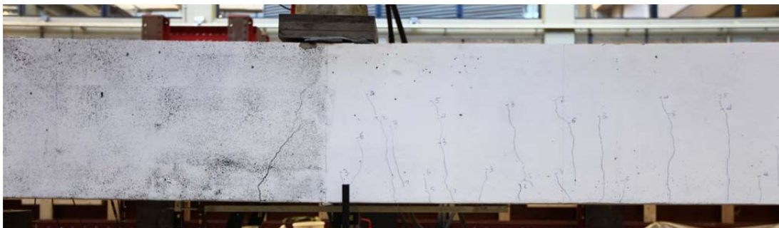
Fig. 5.78.1. Crack pattern after failure front side
