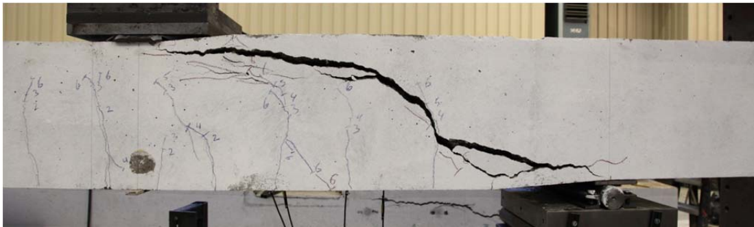
Fig. 5.21.2. Crack pattern after failure south side
