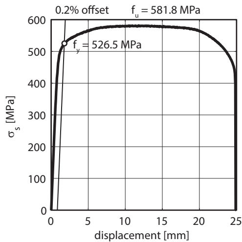
Fig. 2.2.18. Determination of f_y in tests which no clear yielding plateau could be distinguished.
