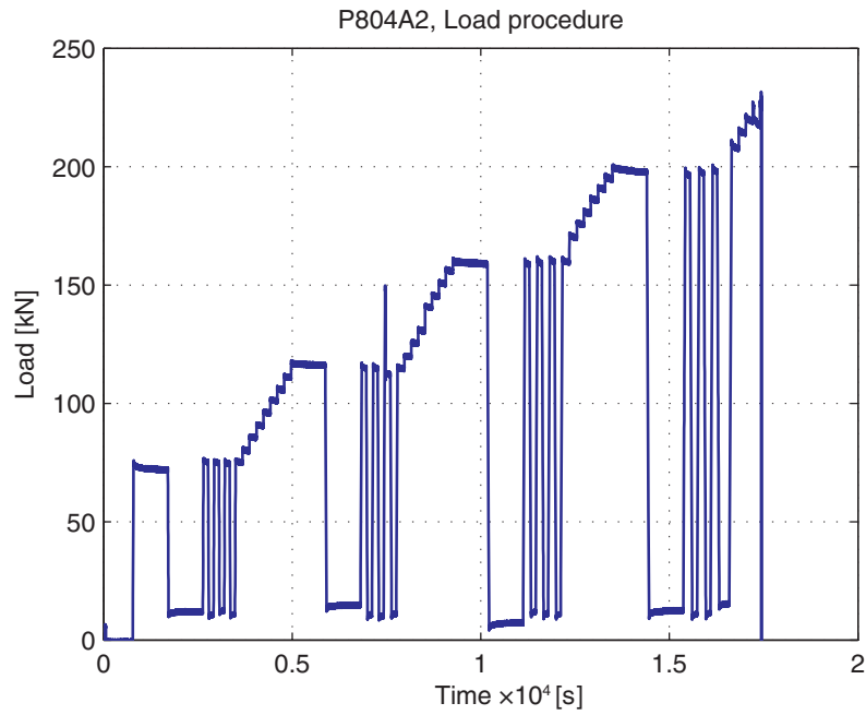
Fig. 5.93.3. Load-Time curve
