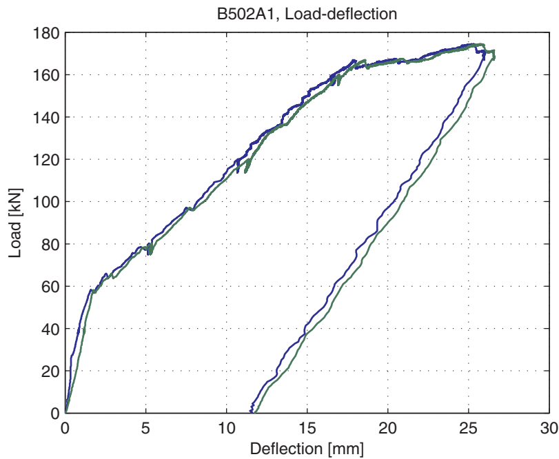
Fig. 5.50.4. Load-deflection curve
