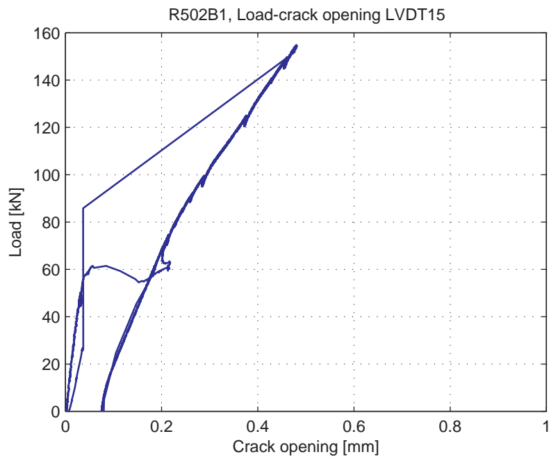
Fig. 5.99.10. Load-Crack opening for LVDT 15
