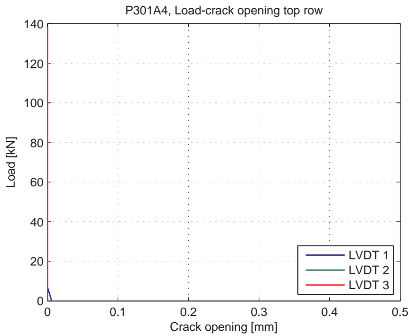
Fig. 5.74.6. Load-Crack opening for LVDT's 1-3 (top row)
