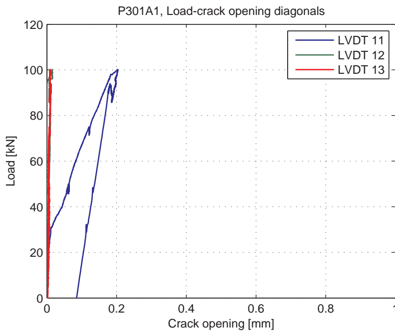
Fig. 5.71.8. Load-Crack opening for LVDT's 11-13 (diagonal)
