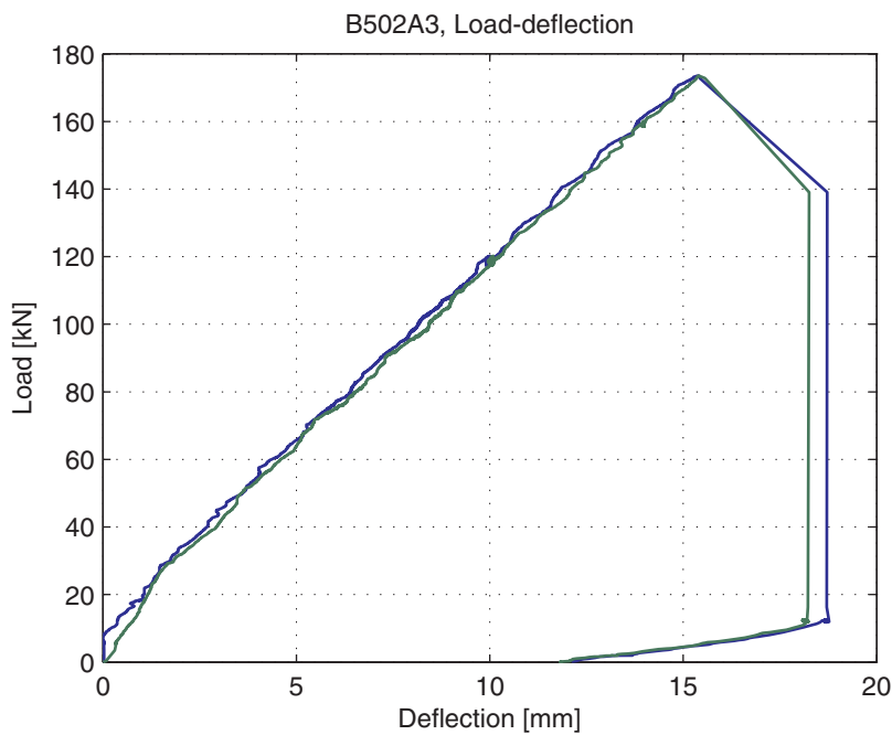
Fig. 5.52.4. Load-deflection curve
