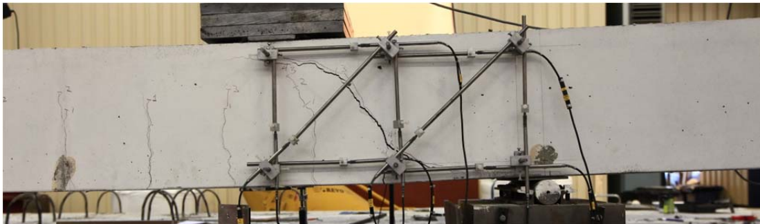
Fig. 5.75.2. Crack pattern after failure back side
