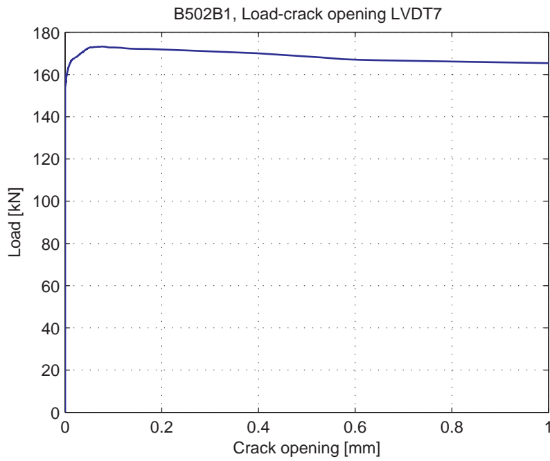
Fig. 5.53.8. Load-Crack opening for LVDT7
