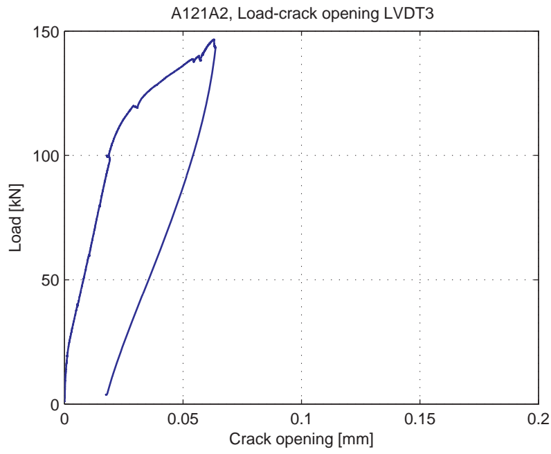
Fig. 5.2.7. Load-Crack opening for LVDT3
