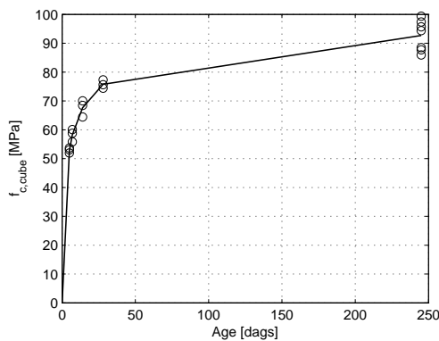
Fig. 2.2.7. F_{c,cube} development for cast 5
