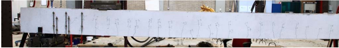
Fig. 5.5.1. Crack pattern after failure north side
