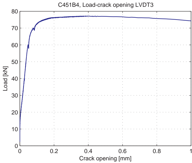
Fig. 5.70.5. Load-Crack opening for LVDT3
