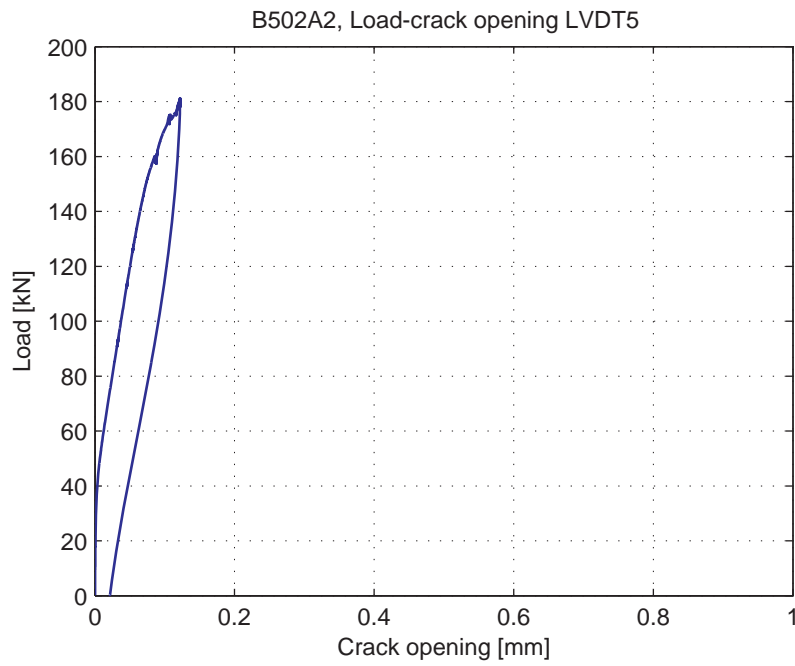
Fig. 5.51.6. Load-Crack opening for LVDT5
