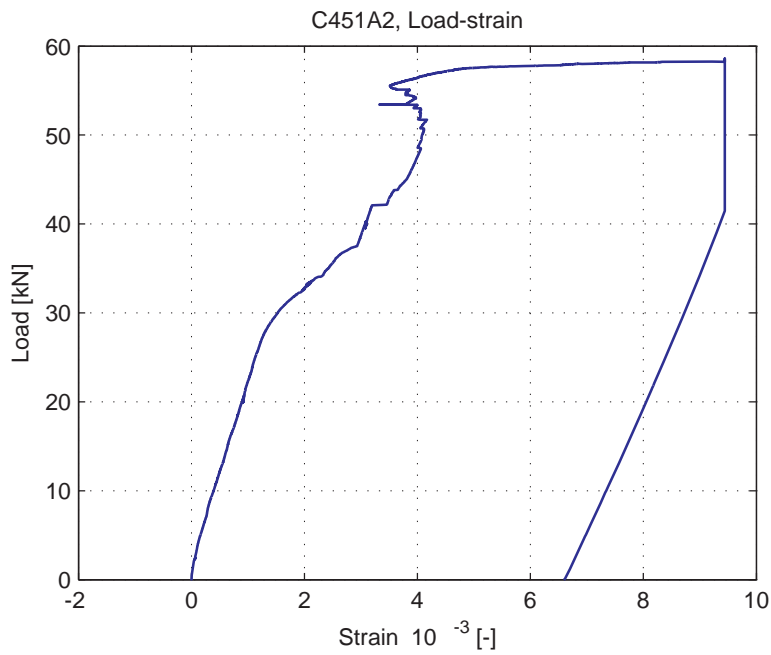
Fig. 5.63.8. Average strain over 1m length, measured at bottom of specimen (LVDT 3)
