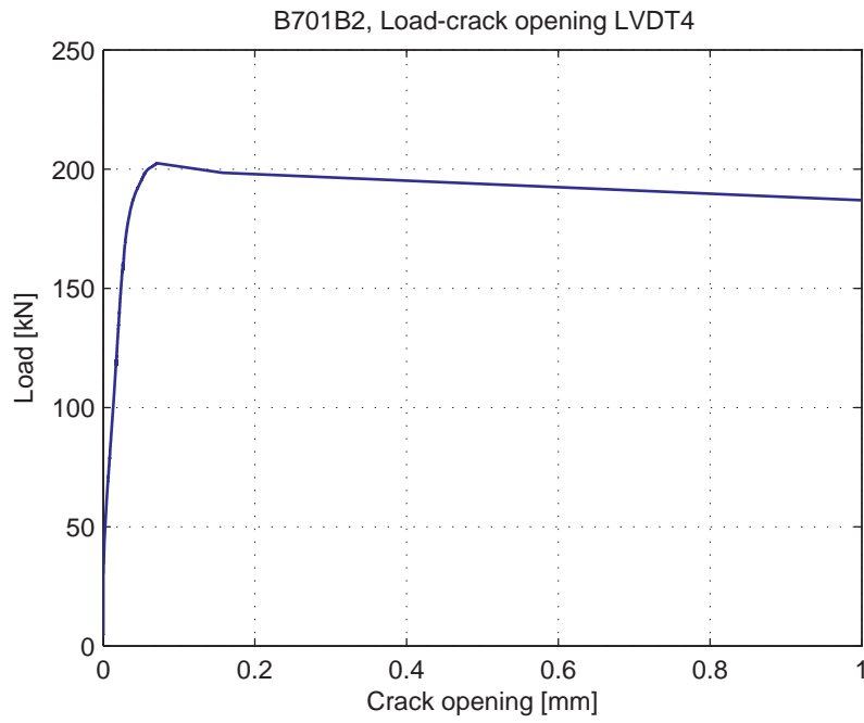
Fig. 5.44.5. Load-Crack opening for LVDT4
