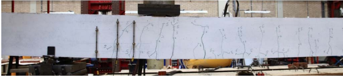
Fig. 5.35.1. Crack pattern after failure north side
