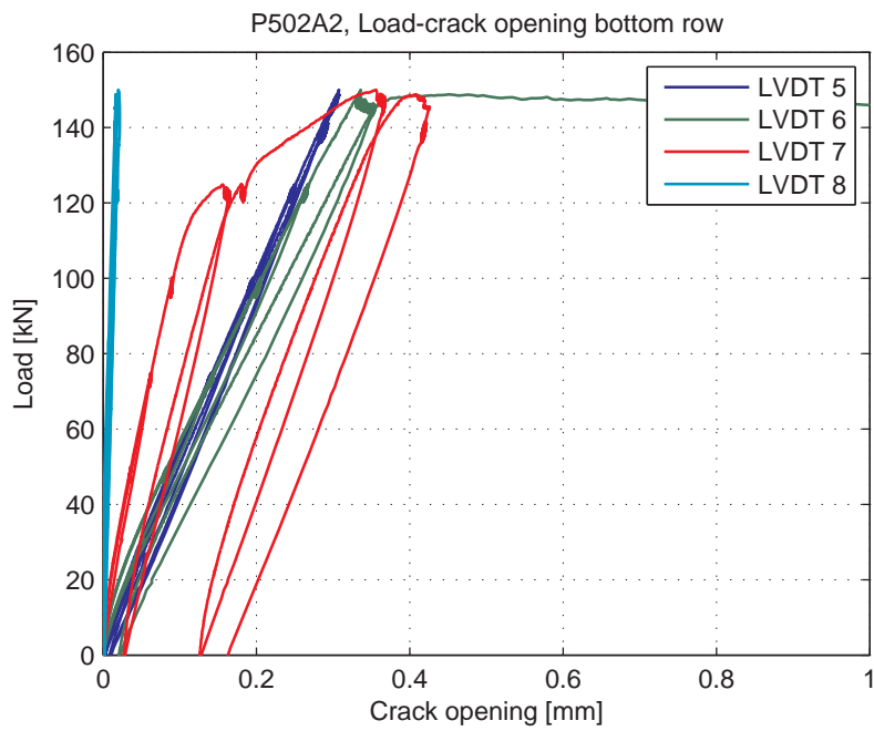
Fig. 5.81.8. Load-Crack opening for LVDT's 5-8 (bottom row)
