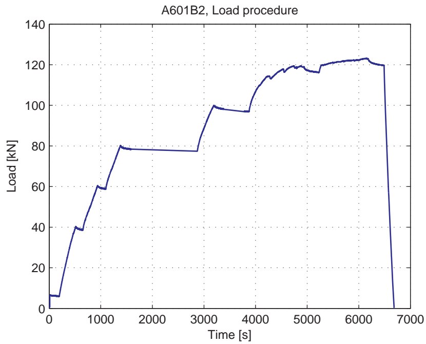
Fig. 5.34.3. Load-Time curve
