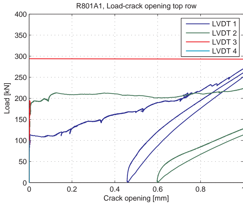
Fig. 5.100.6. Load-Crack opening for LVDT's 1-4 (top row)
