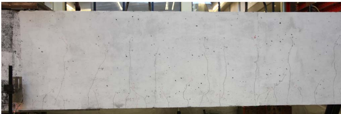
Fig. 5.90.1. Crack pattern after failure north side
