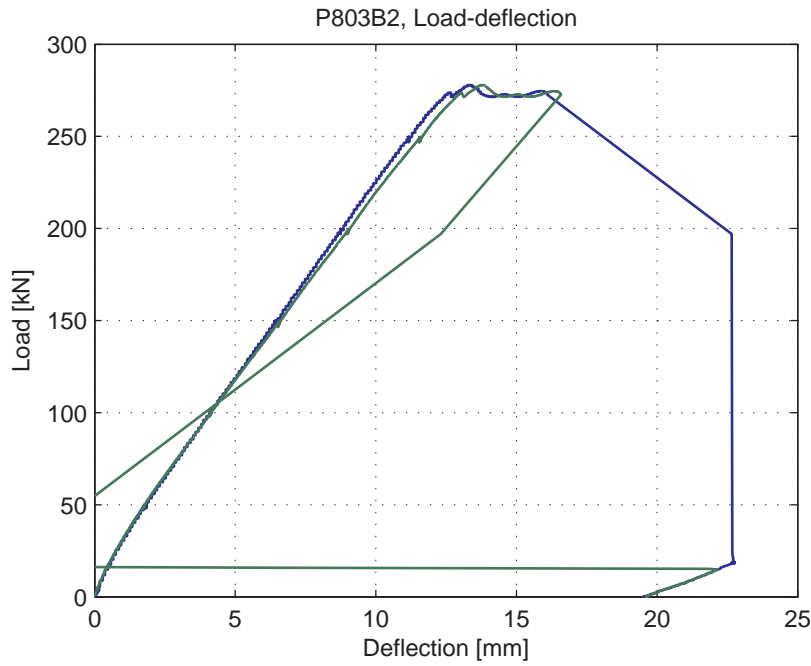
Fig. 5.91.5. Load-deflection curve
