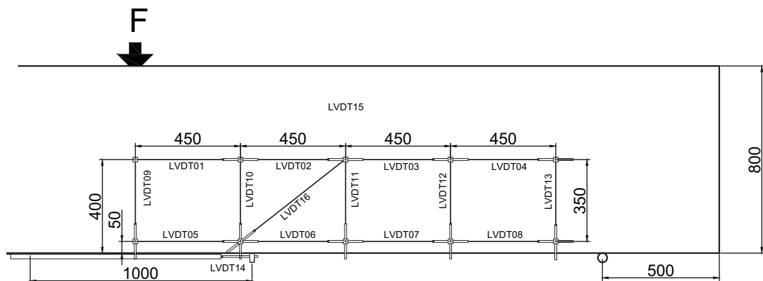
Fig. 5.86.4. LVDT layout and numbering for 800 mm deep beams
