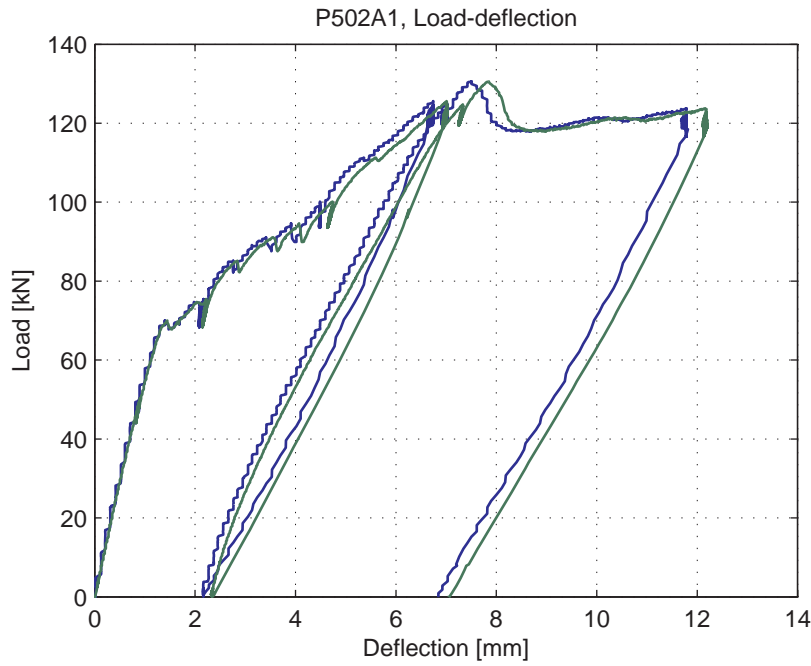
Fig. 5.80.5. Load-deflection curve
