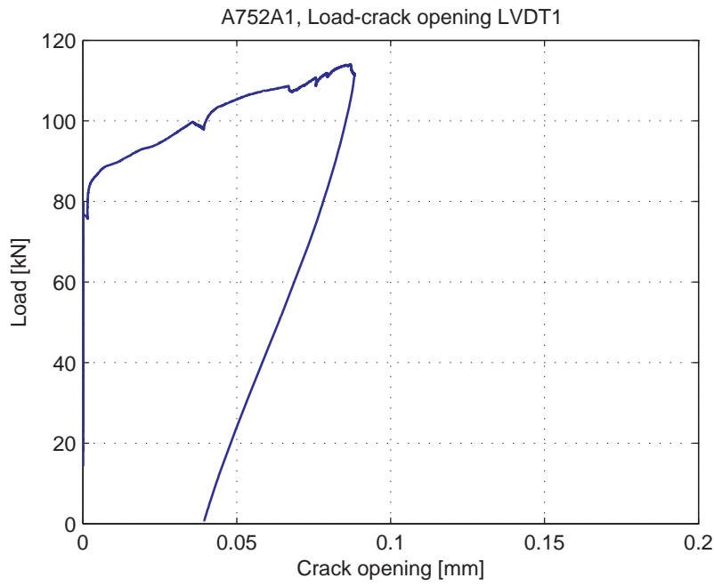
Fig. 5.26.5. Load-Crack opening for LVDT1
