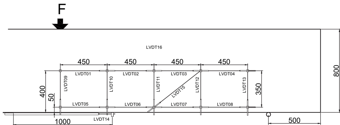
Fig. 5.101.3. LVDT layout and numbering for 800 mm deep beams
