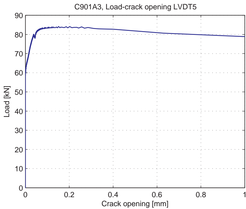
Fig. 5.56.6. Load-Crack opening for LVDT5
