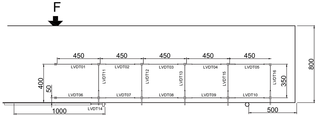
Fig. 5.105.3. LVDT layout and numbering for 800 mm deep beams
