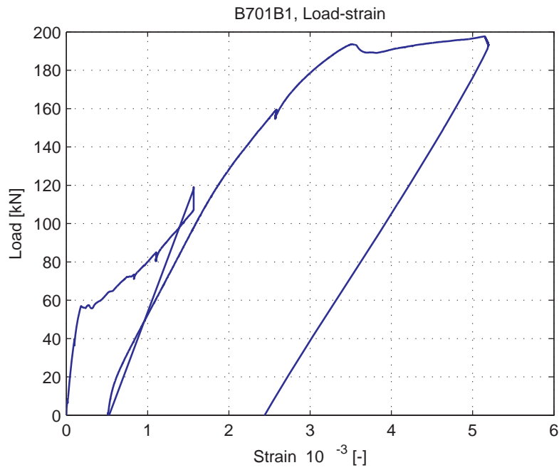
Fig. 5.43.9. Average strain over 1m length, measured at bottom of specimen (LVDT 3)
