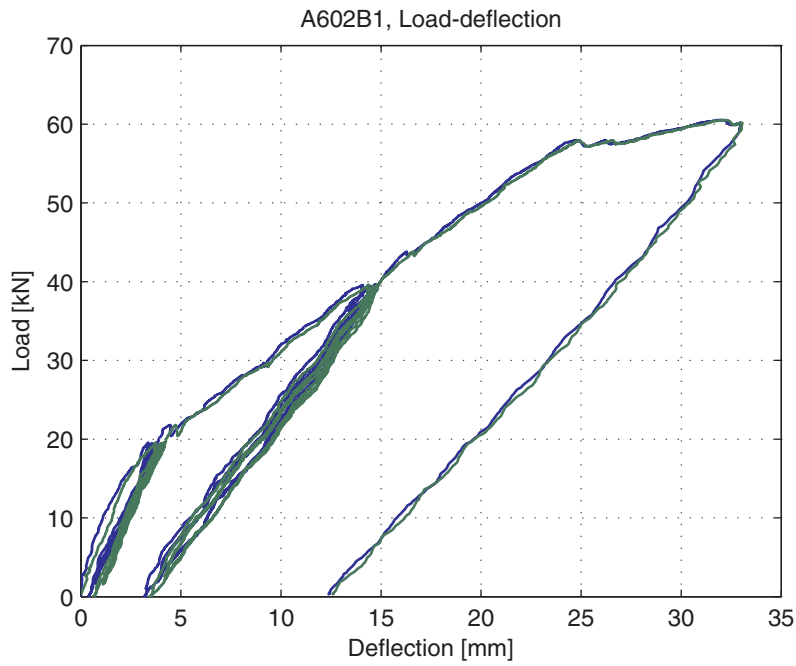
Fig. 5.38.5. Load-deflection curve
