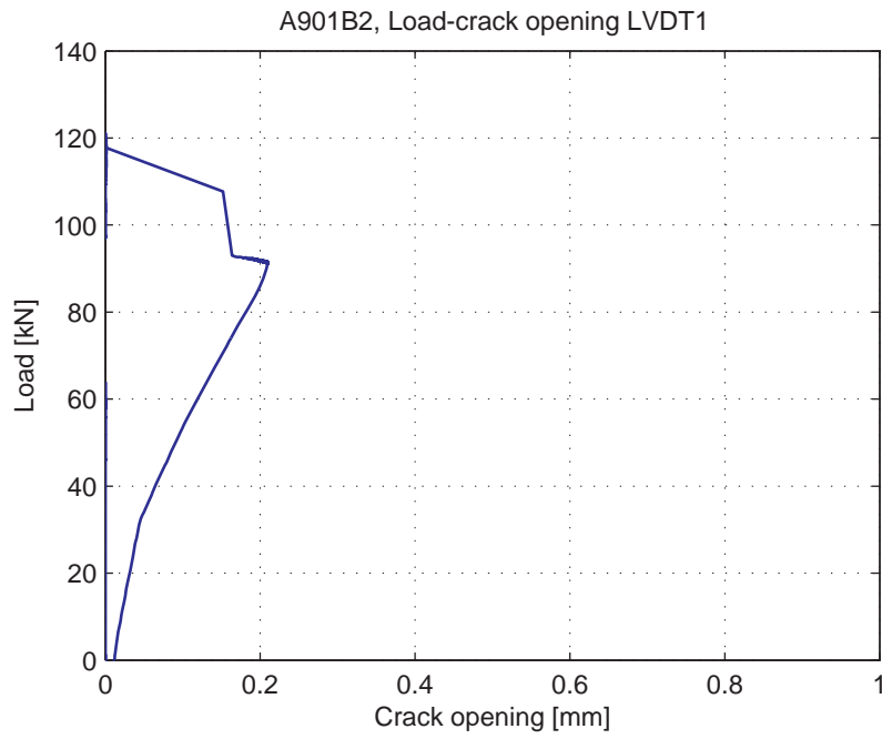
Fig. 5.16.5. Load-Crack opening for LVDT1
