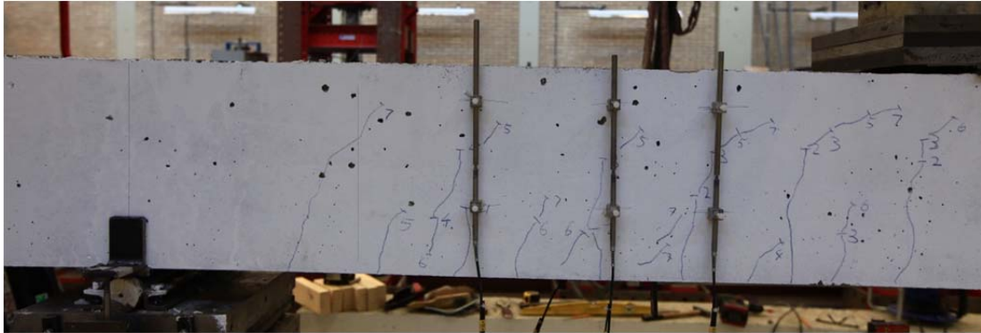
Fig. 5.10.1. Crack pattern after failure north side
