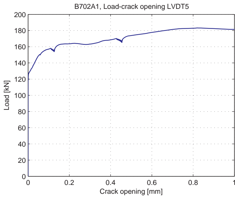
Fig. 5.45.6. Load-Crack opening for LVDT5
