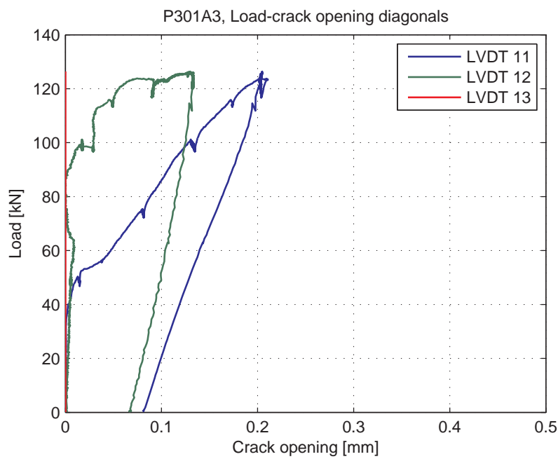
Fig. 5.73.9. Load-Crack opening for LVDT's 11-13 (diagonal)
