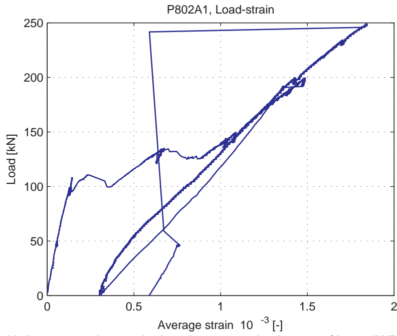
Fig. 5.87.11. Average strain over 1m length, measured at bottom of beam (LVDT 14)
