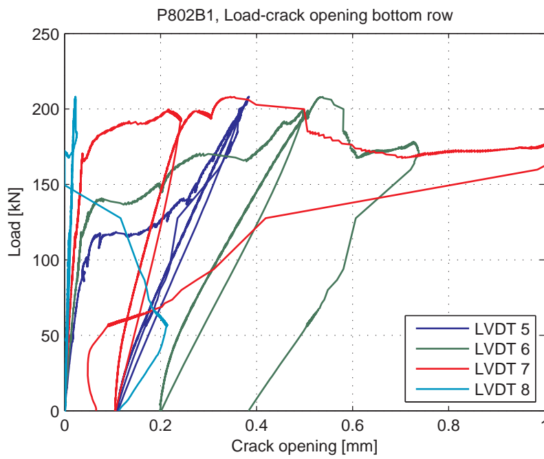
Fig. 5.88.8. Load-Crack opening for LVDT's 5-8 (bottom row)
