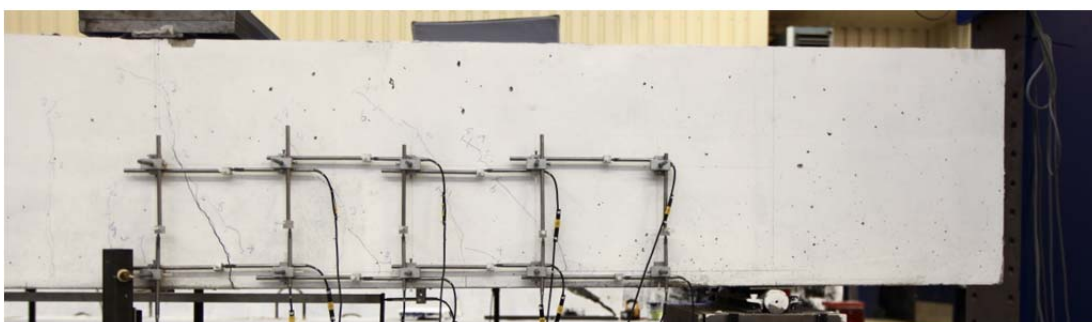
Fig. 5.78.2. Crack pattern after failure back side
