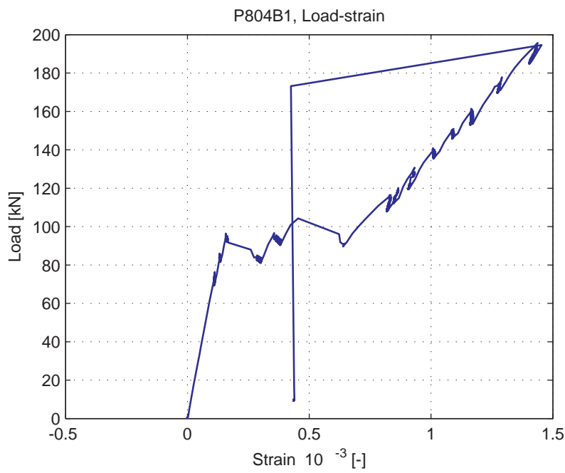
Fig. 5.94.10. Average strain over 1m length, measured at bottom of specimen (LVDT 14)
