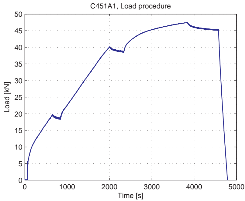
Fig. 5.62.3. Load-Time curve
