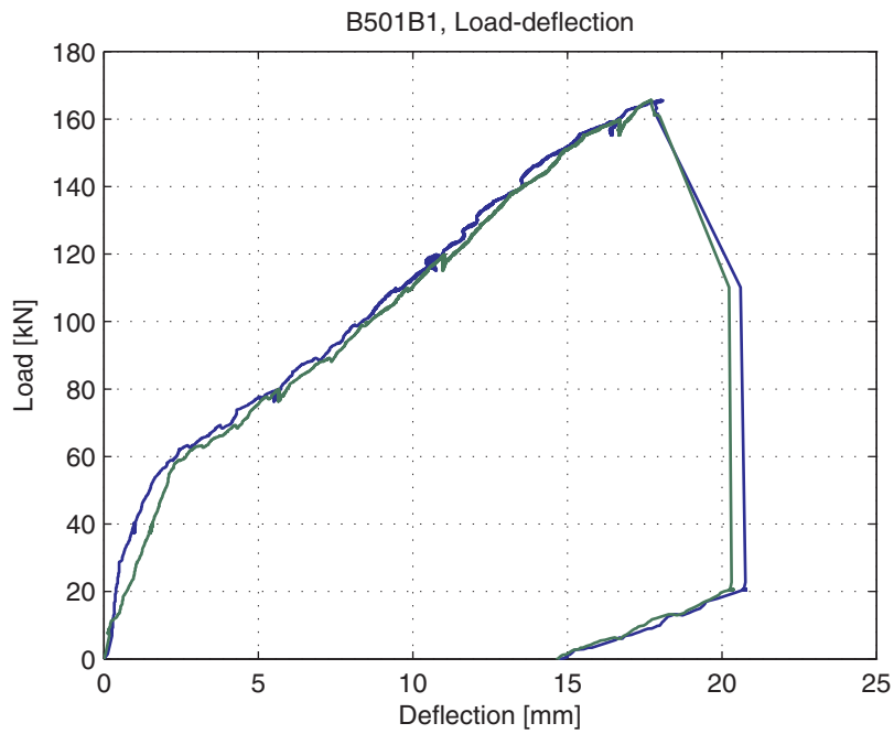
Fig. 5.49.4. Load-deflection curve
