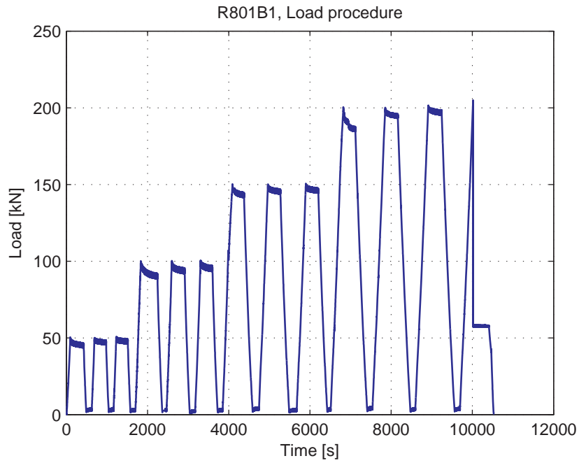
Fig. 5.101.4. Load-Time curve
