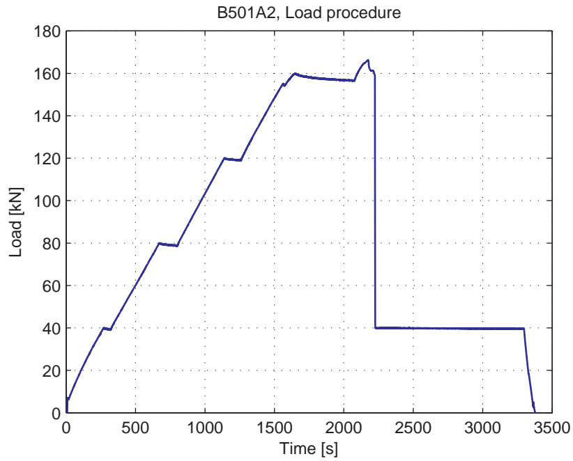
Fig. 5.48.3. Load-Time curve
