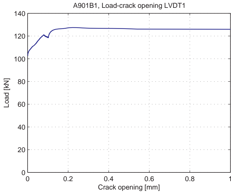
Fig. 5.15.5. Load-Crack opening for LVDT1
