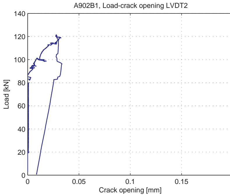
Fig. 5.20.6. Load-Crack opening for LVDT2
