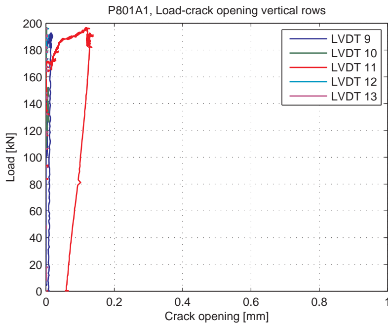
Fig. 5.83.6. Load-Crack opening for LVDT's 9-13 (vertical LVDT's)
