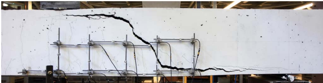
Fig. 5.99.2. Crack pattern after failure west side
