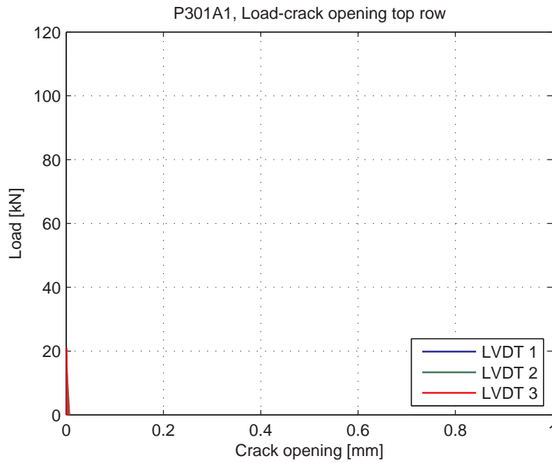
Fig. 5.71.5. Load-Crack opening for LVDT's 1-3 (top row)
