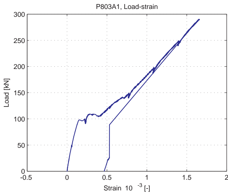
Fig. 5.89.10. Average strain over 1m length, measured at bottom of specimen (LVDT 14)
