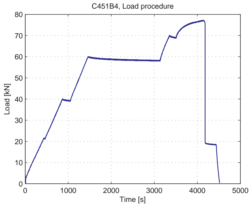
Fig. 5.70.3. Load-Time curve
