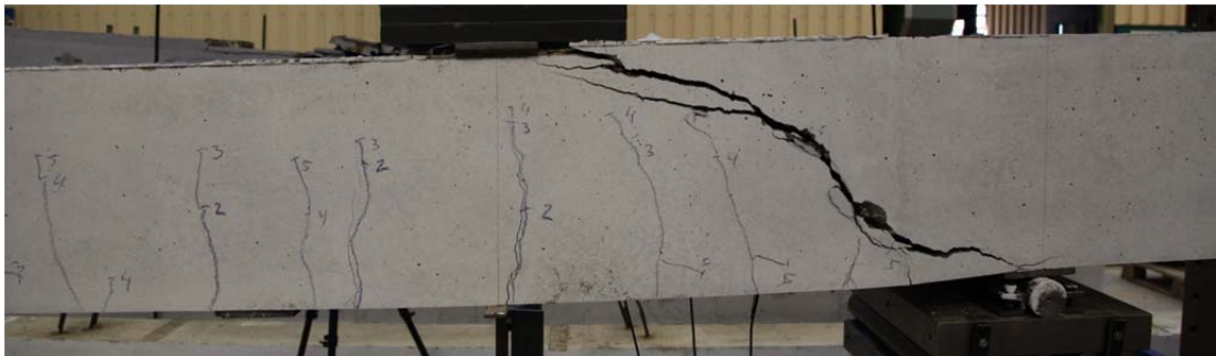
Fig. 5.37.2. Crack pattern after failure south side
