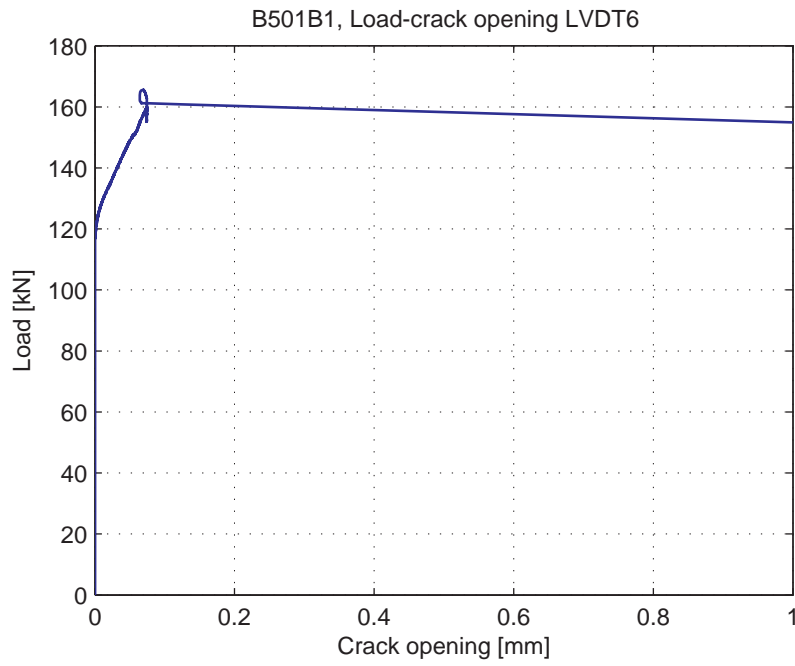
Fig. 5.49.7. Load-Crack opening for LVDT6
