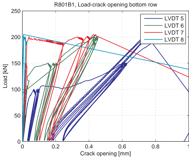
Fig. 5.101.8. Load-Crack opening for LVDT's 5-8 (bottom row)
