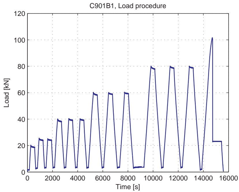
Fig. 5.57.5. Load-Time curve
