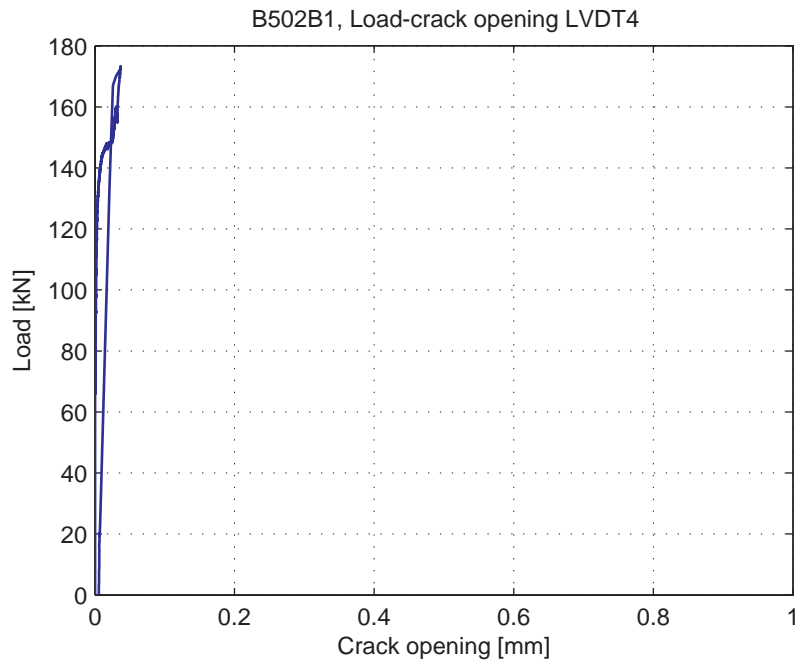
Fig. 5.53.5. Load-Crack opening for LVDT4
