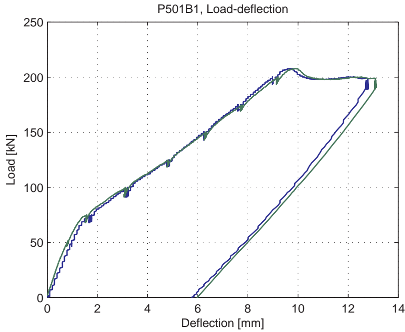
Fig. 5.78.5. Load-deflection curve
