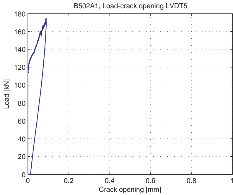
Fig. 5.50.6. Load-Crack opening for LVDT5
