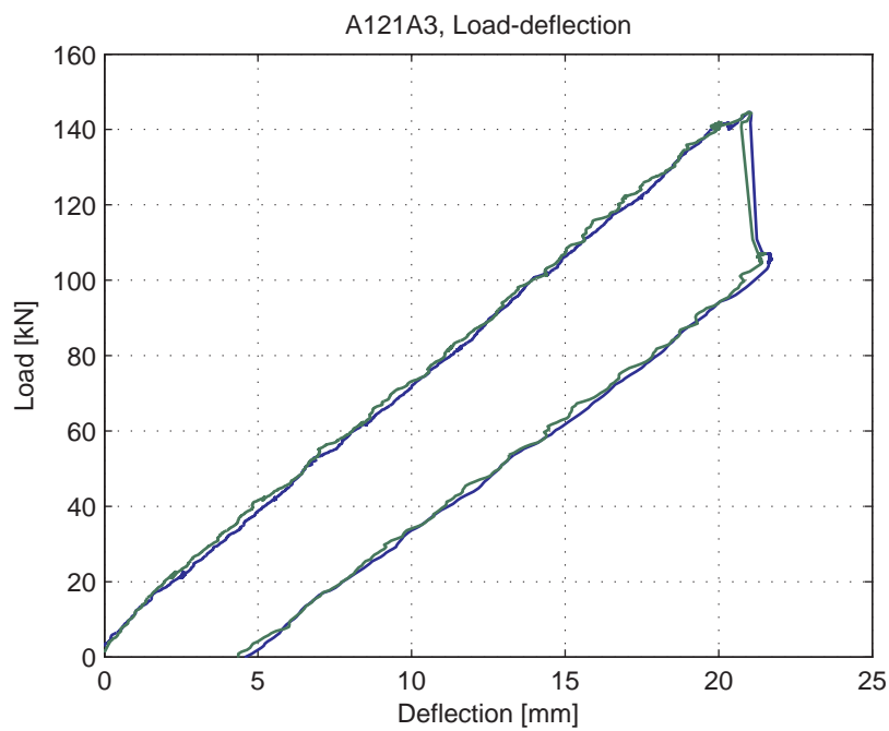
Fig. 5.3.4. Load-deflection curve
