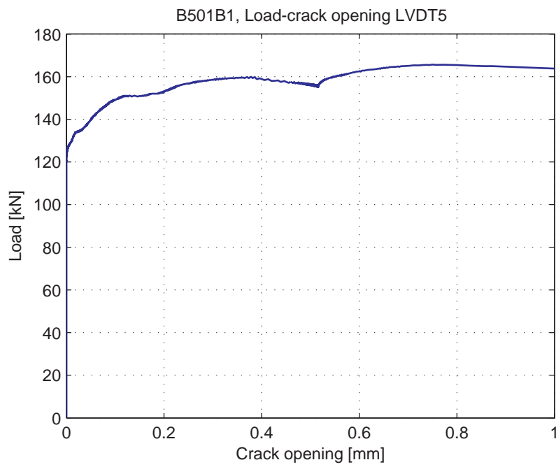
Fig. 5.49.6. Load-Crack opening for LVDT5
