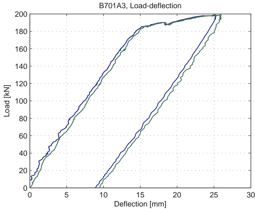
Fig. 5.42.4. Load-deflection curve
