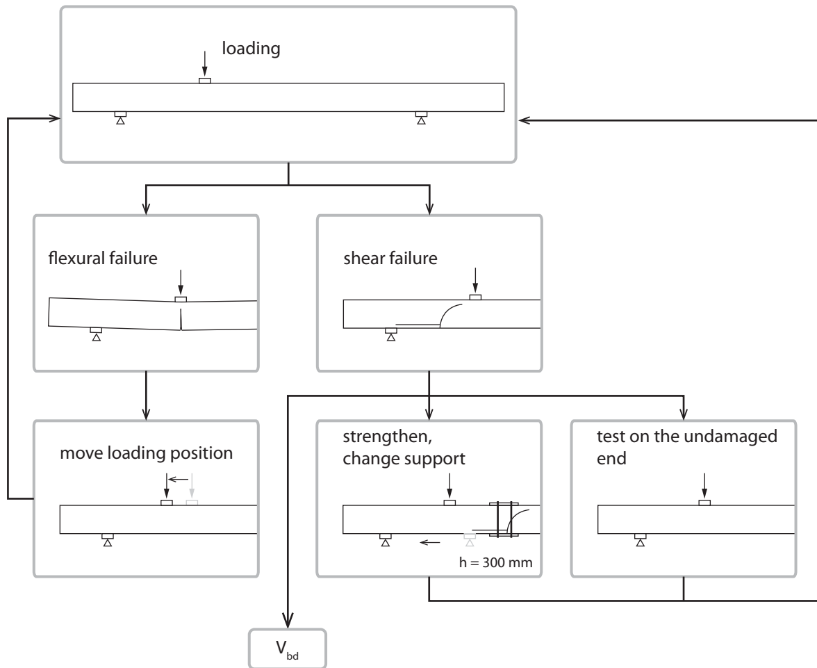
Fig. 3.1.2. Flow chat of the test program for a given beam configuration.
