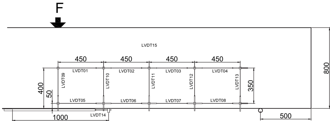
Fig. 5.102.3. LVDT layout and numbering for 800 mm deep beams
