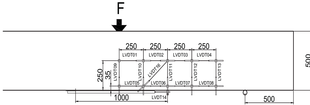
Fig. 5.80.3. LVDT layout and numbering for 500 mm deep beams
