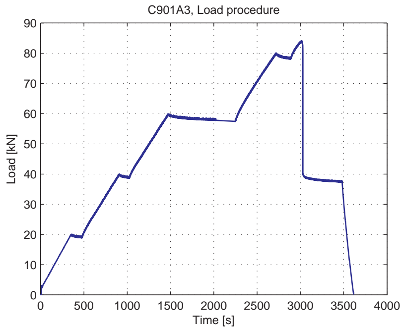
Fig. 5.56.3. Load-Time curve
