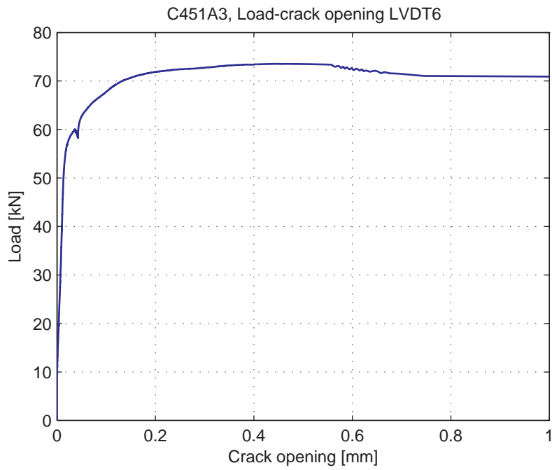
Fig. 5.64.7. Load-Crack opening for LVDT6
