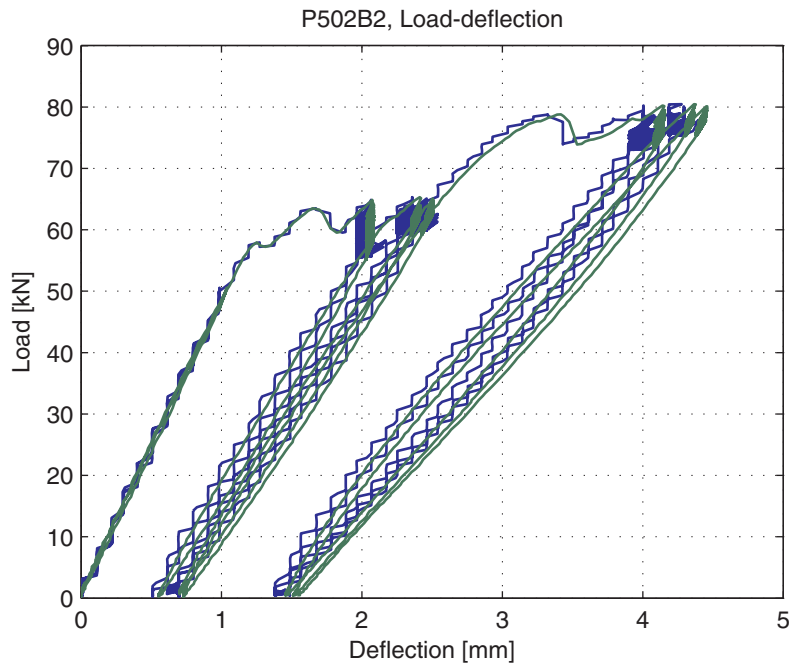
Fig. 5.82.8. Load-deflection curve for second part of test
