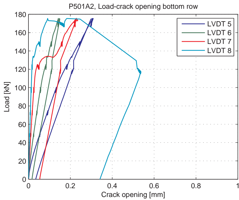
Fig. 5.77.8. Load-Crack opening for LVDT's 5-8 (bottom row)
