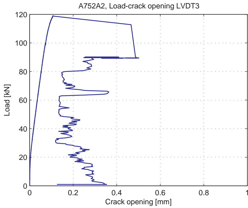
Fig. 5.27.7. Load-Crack opening for LVDT3
