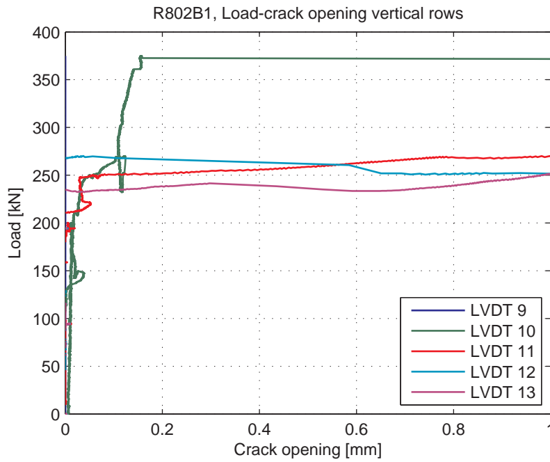
Fig. 5.103.7. Load-Crack opening for LVDT's 9-13 (vertical LVDT's)
