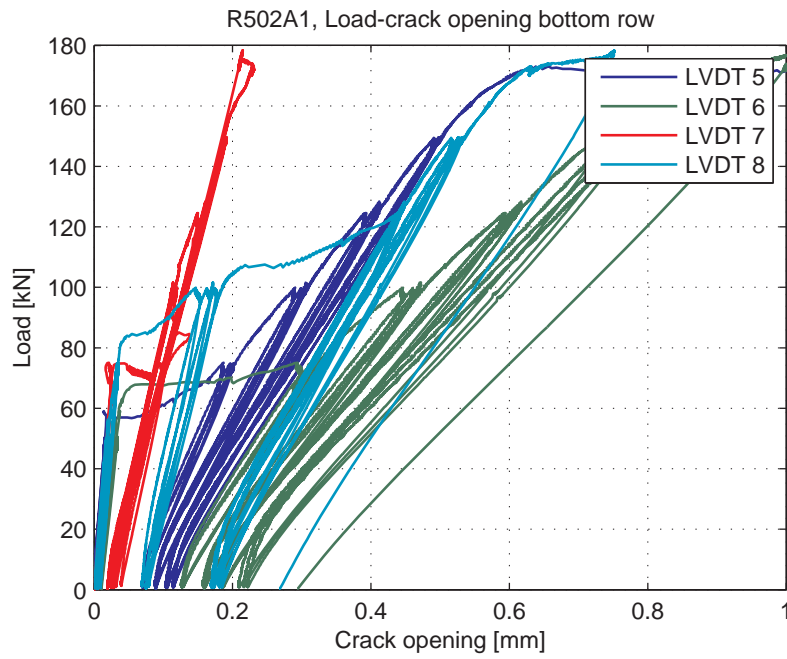
Fig. 5.97.8. Load-Crack opening for LVDT's 5-8 (bottom row)
