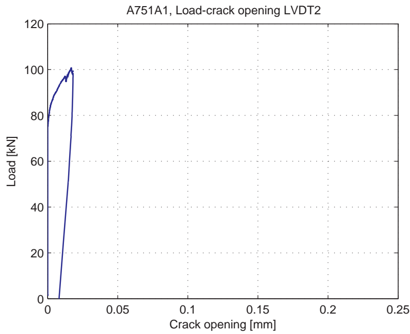
Fig. 5.22.6. Load-Crack opening for LVDT2
