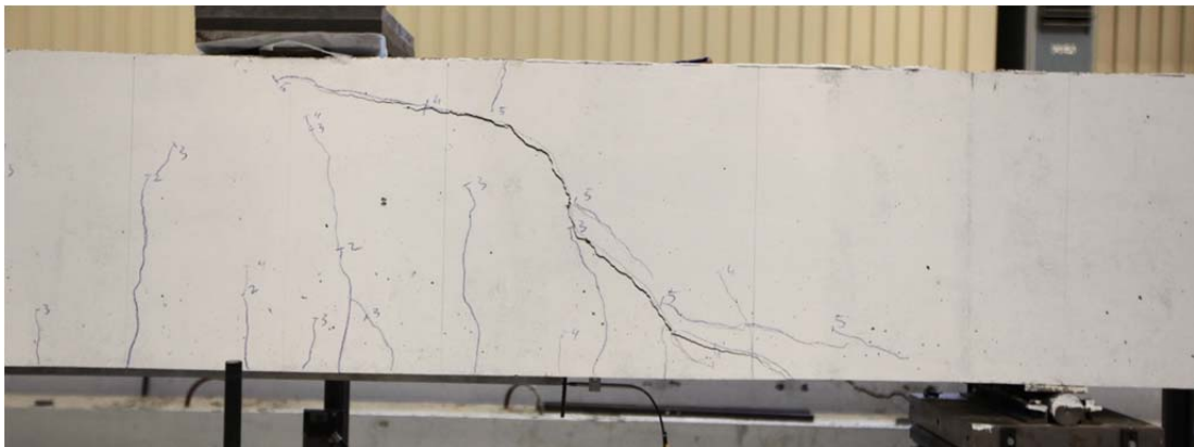
Fig. 5.45.2. Crack pattern after failure south side
