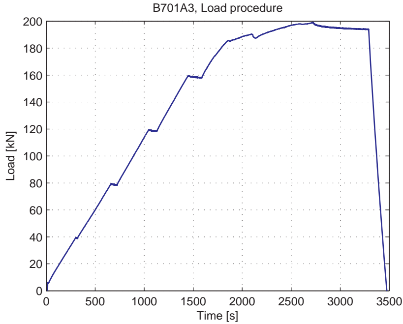
Fig. 5.42.3. Load-Time curve
