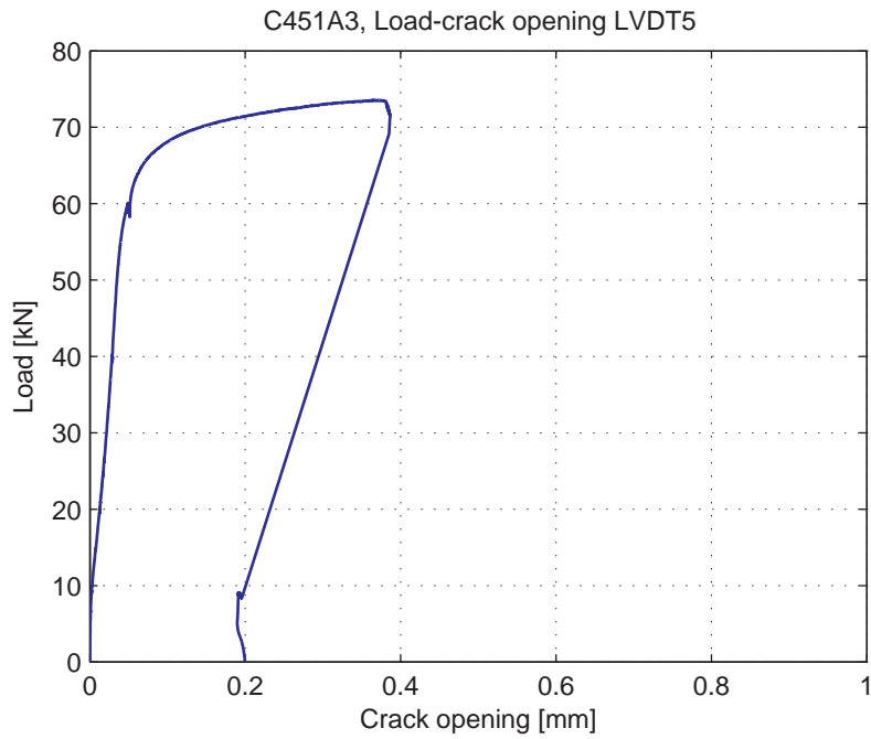
Fig. 5.64.6. Load-Crack opening for LVDT5
