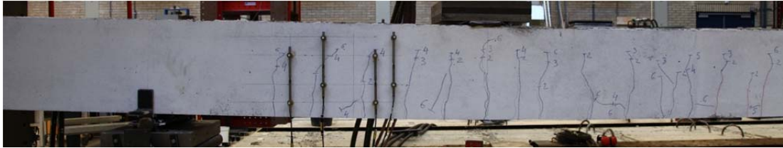
Fig. 5.20.1. Crack pattern after failure north side
