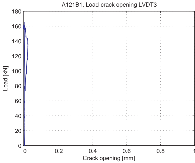
Fig. 5.4.7. Load-Crack opening for LVDT3
