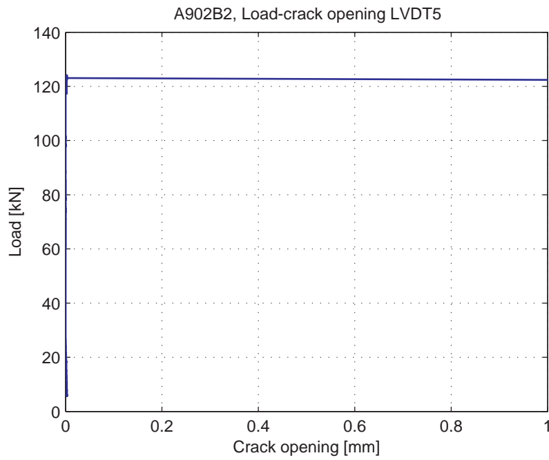
Fig. 5.21.8. Load-Crack opening for LVDT5
