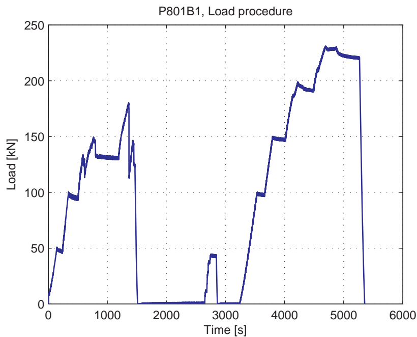
Fig. 5.86.5. Load-Time curve
