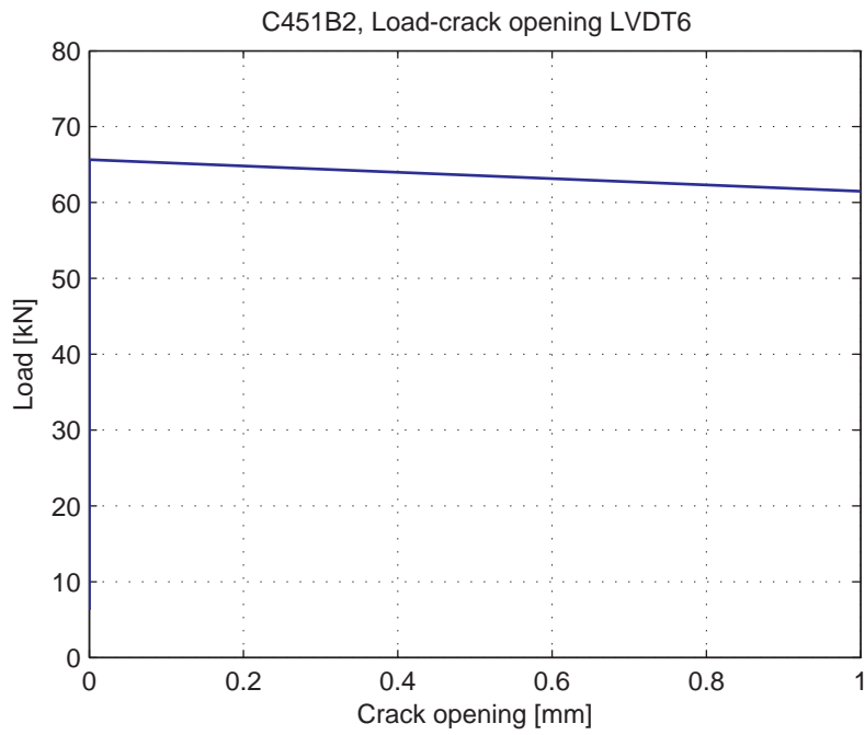
Fig. 5.68.7. Load-Crack opening for LVDT6
