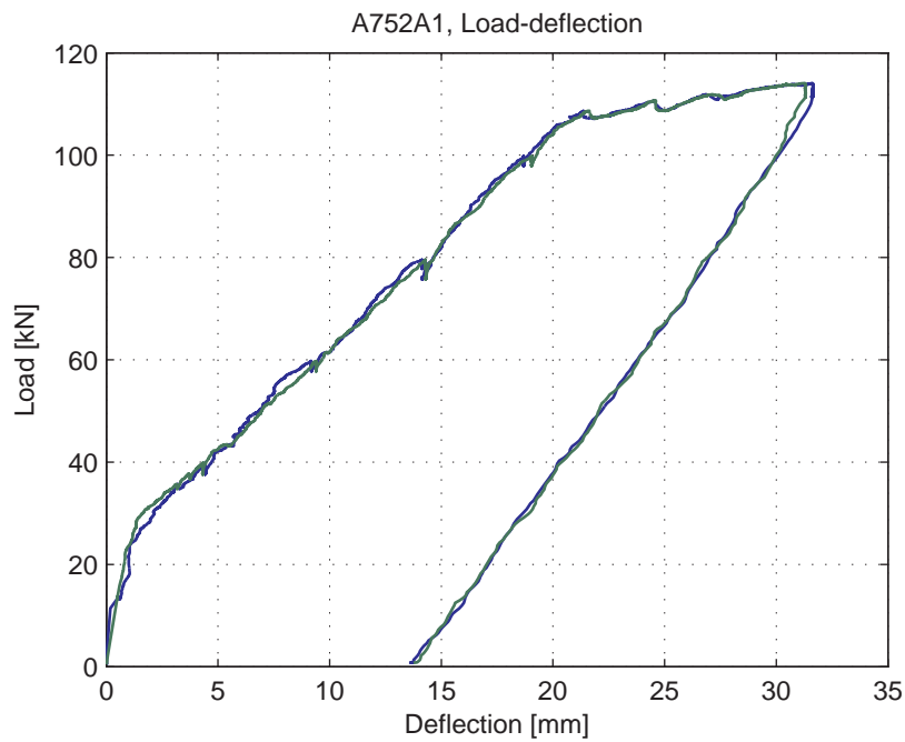
Fig. 5.26.4. Load-deflection curve
