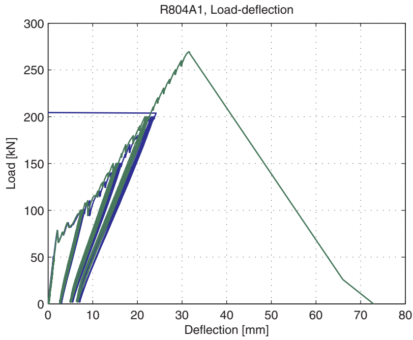
Fig. 5.106.5. Load-deflection curve
