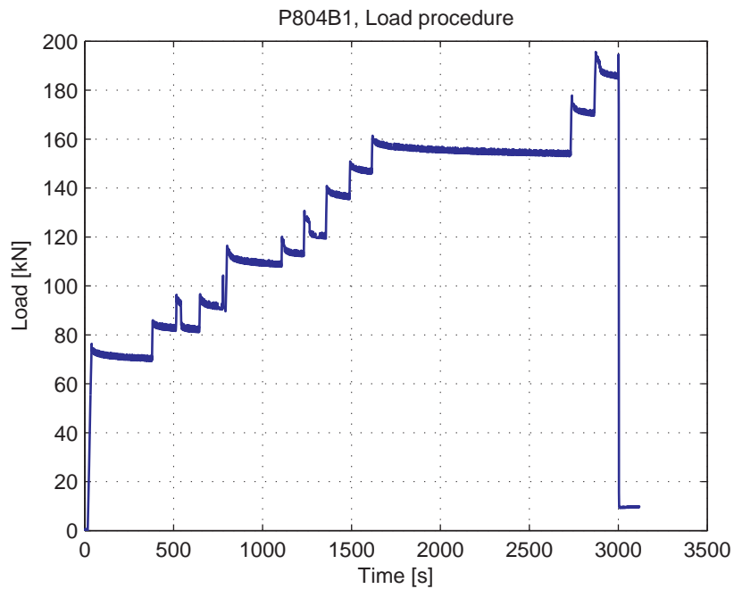
Fig. 5.94.4. Load-Time curve
