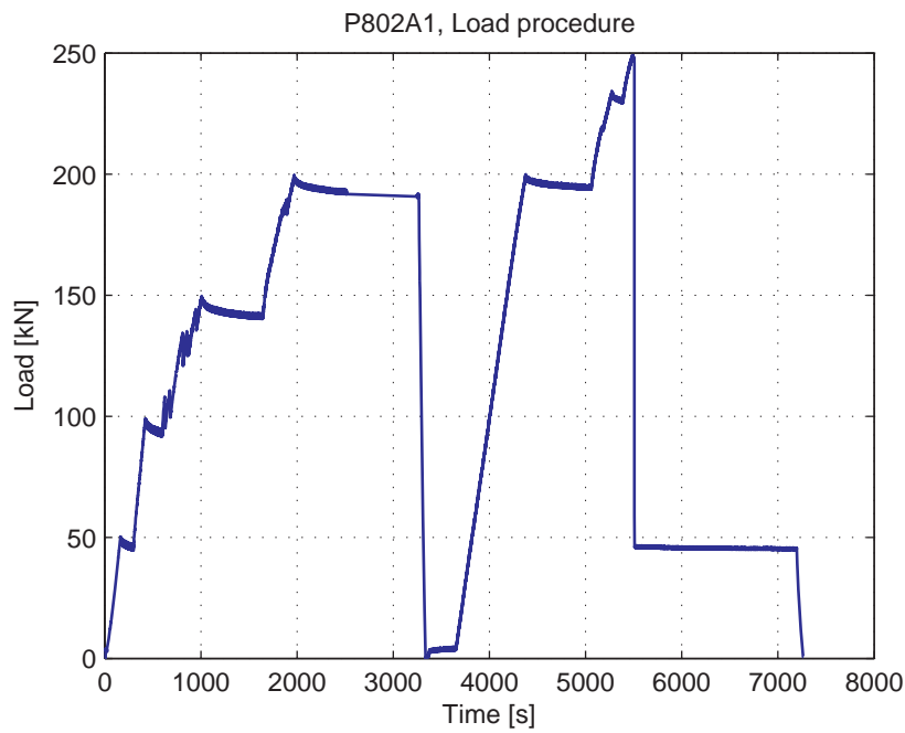
Fig. 5.87.4. Load-Time curve
