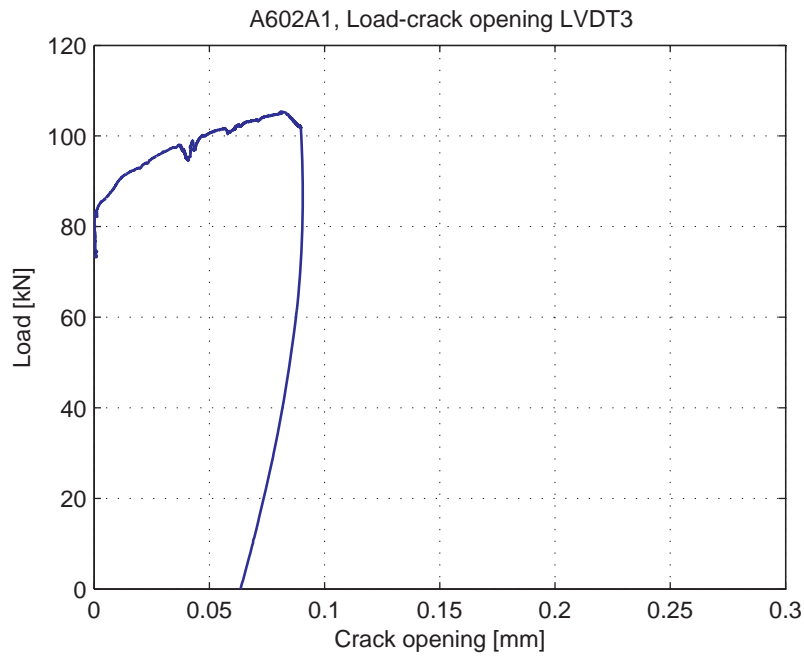
Fig. 5.35.7. Load-Crack opening for LVDT3
