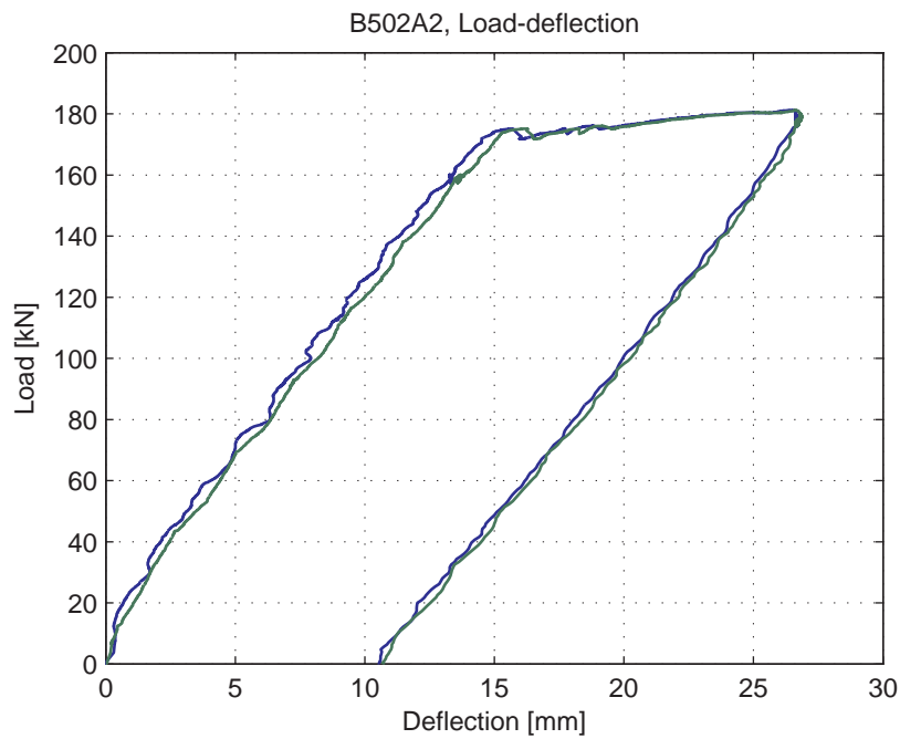
Fig. 5.51.4. Load-deflection curve
