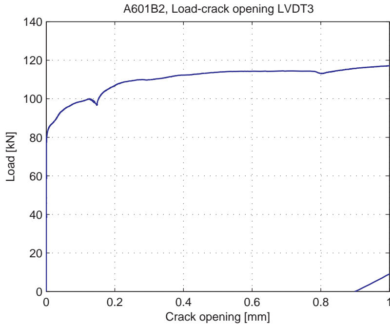
Fig. 5.34.7. Load-Crack opening for LVDT3
