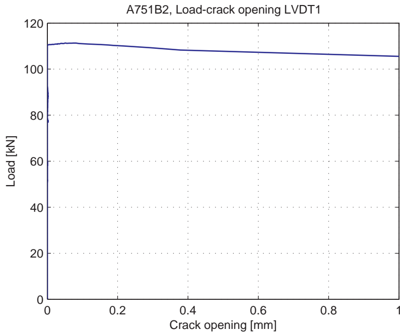
Fig. 5.25.5. Load-Crack opening for LVDT1
