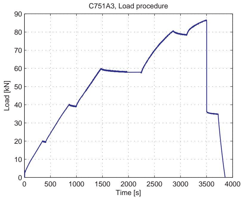
Fig. 5.60.3. Load-Time curve
