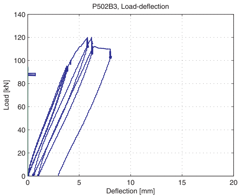
Fig. 5.82.9. Load-deflection curve for third part of test
