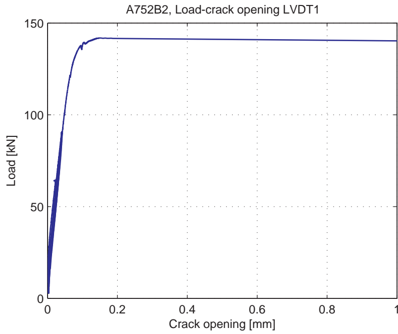
Fig. 5.30.5. Load-Crack opening for LVDT1
