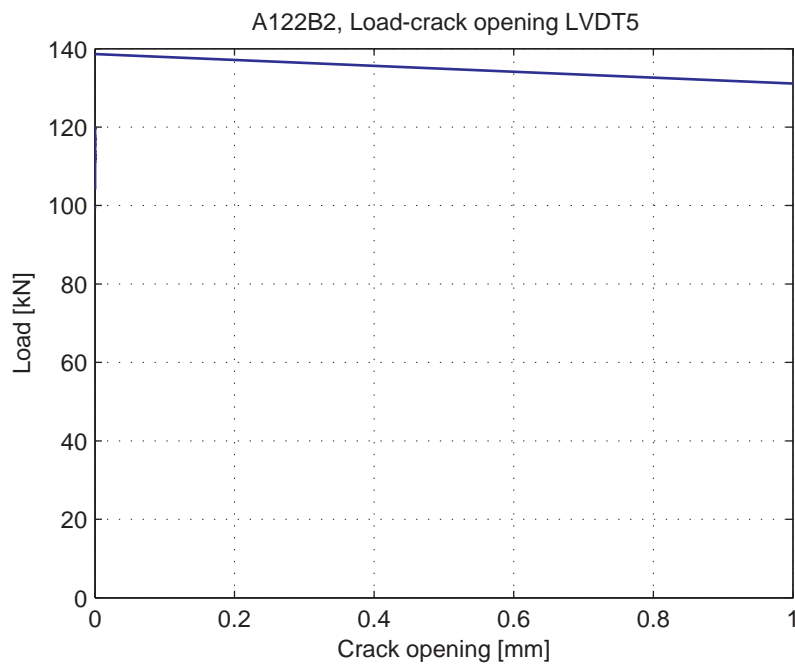
Fig. 5.7.8. Load-Crack opening for LVDT5
