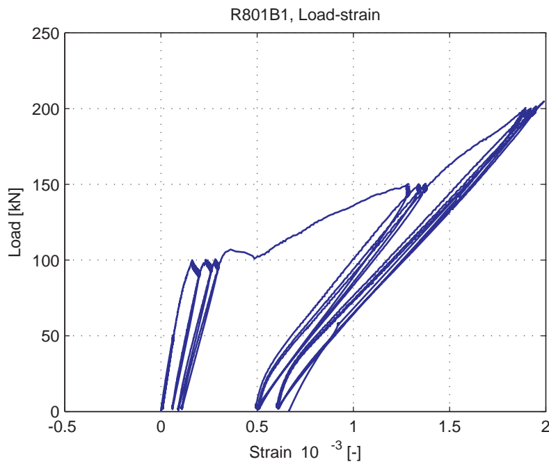
Fig. 5.101.11. Average strain over 1m length, measured at bottom of specimen (LVDT 14)
