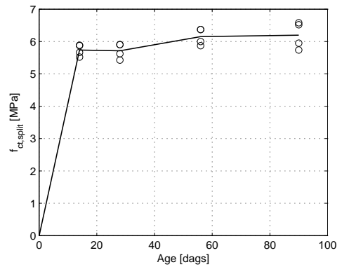
Fig. 2.2.16. F_{ct,split} development for cast 9
