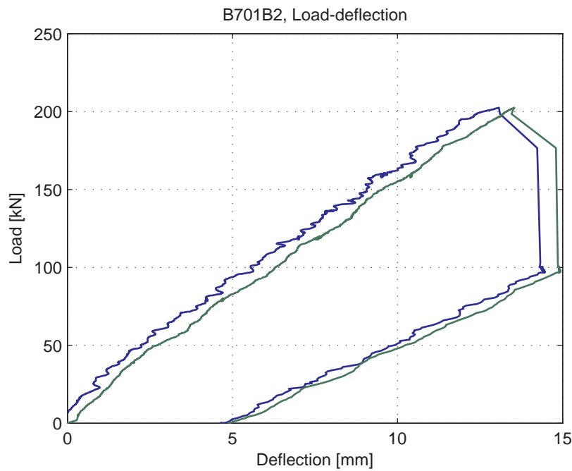
Fig. 5.44.4. Load-deflection curve
