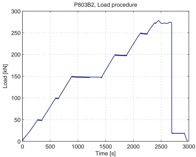
Fig. 5.91.4. Load-Time curve
