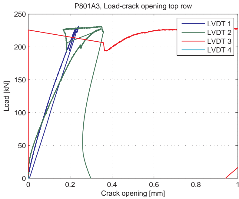
Fig. 5.85.6. Load-Crack opening for LVDT's 1-4 (top row)
