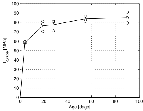
Fig. 2.2.13. F_{c,cube} development for cast 8
