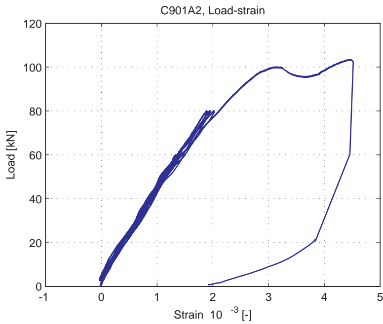
Fig. 5.55.9. Average strain over 1m length, measured at bottom of specimen (LVDT 3)
