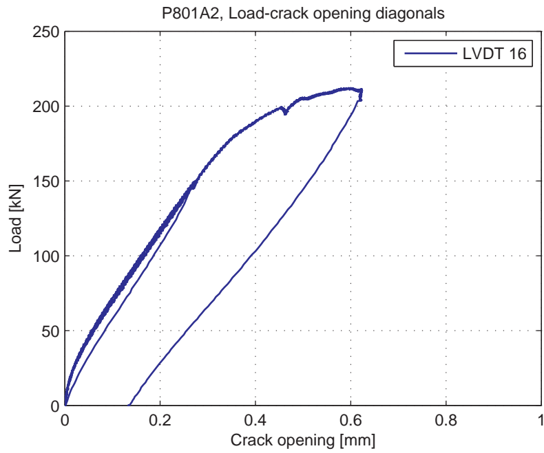
Fig. 5.84.8. Load-Crack opening for LVDT 16 (diagonal)
