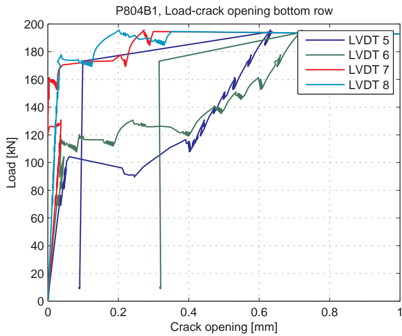
Fig. 5.94.8. Load-Crack opening for LVDT's 5-8 (bottom row)
