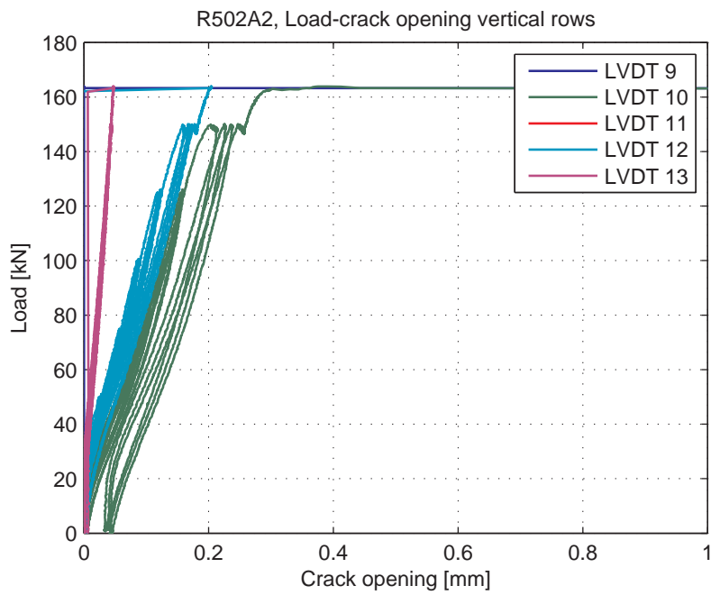
Fig. 5.98.6. Load-Crack opening for LVDT's 9-13 (vertical LVDT's)
