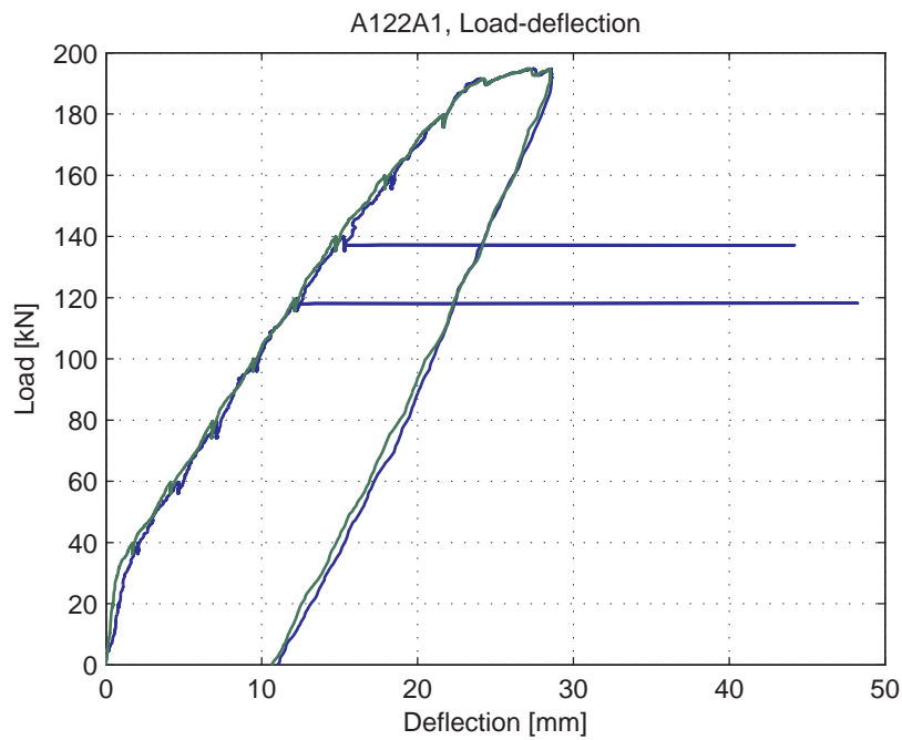
Fig. 5.5.4. Load-deflection curve
