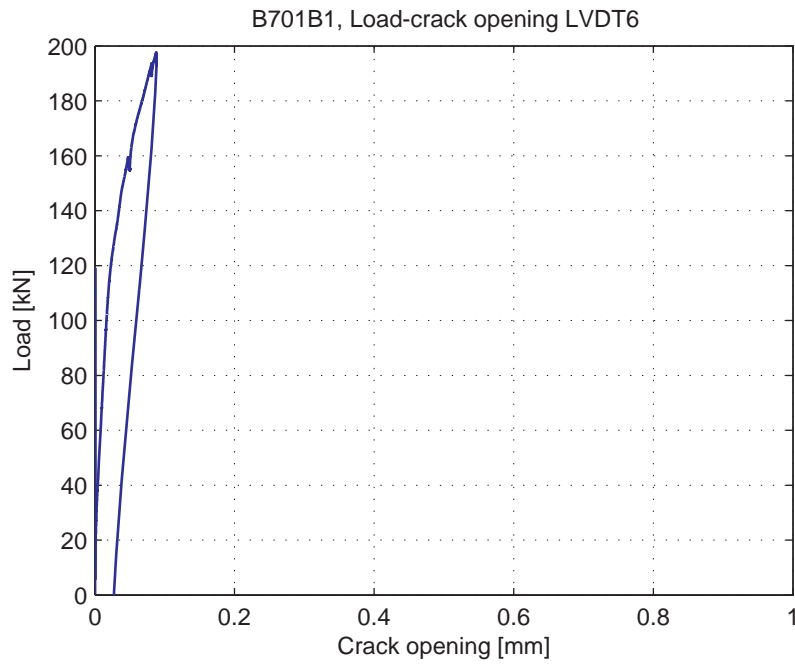
Fig. 5.43.7. Load-Crack opening for LVDT6
