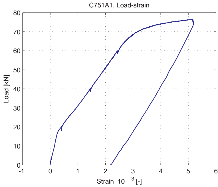
Fig. 5.58.5. Average strain over 1m length, measured at bottom of specimen (LVDT 3)
