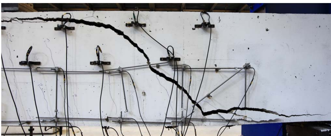
Fig. 5.94.2. Crack pattern after failure west side
