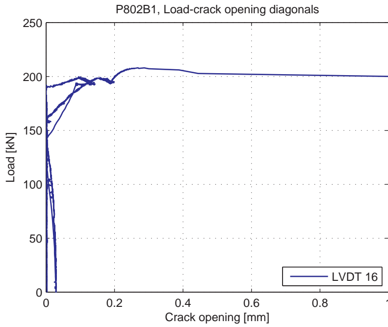
Fig. 5.88.9. Load-Crack opening for LVDT 16 (diagonal)
