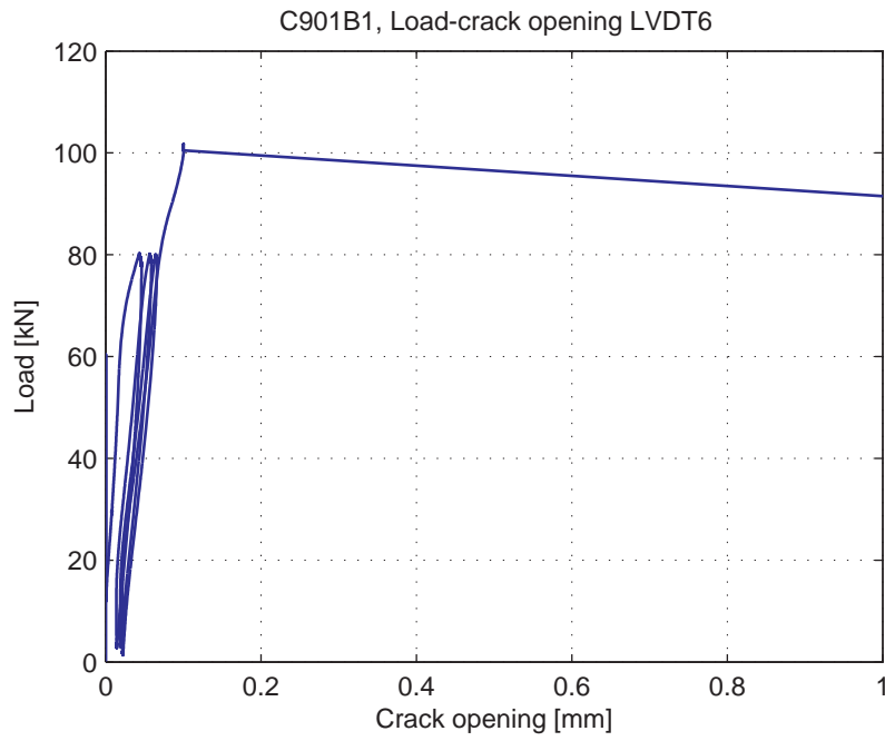
Fig. 5.57.9. Load-Crack opening for LVDT6
