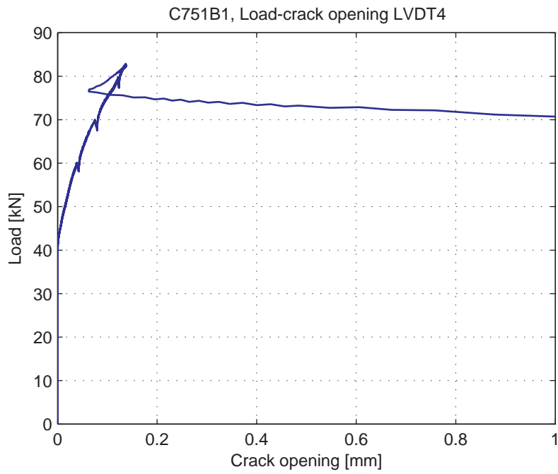
Fig. 5.61.5. Load-Crack opening for LVDT4
