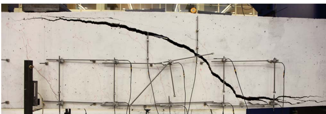
Fig. 5.91.2. Crack pattern after failure south side
