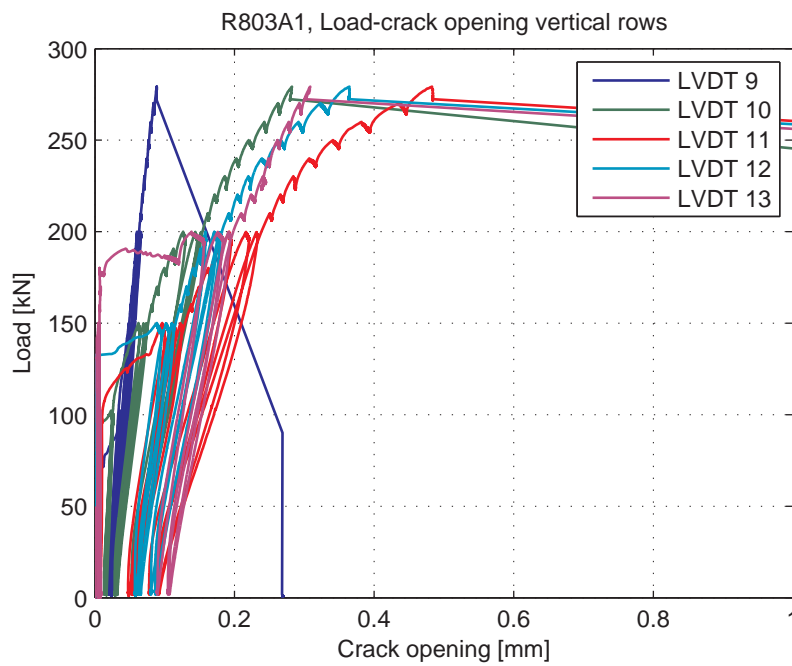
Fig. 5.104.7. Load-Crack opening for LVDT's 9-13 (vertical LVDT's)
