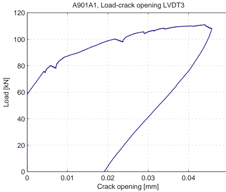
Fig. 5.12.7. Load-Crack opening for LVDT3
