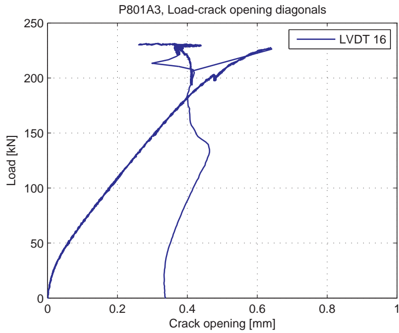
Fig. 5.85.9. Load-Crack opening for LVDT 16 (diagonal)
