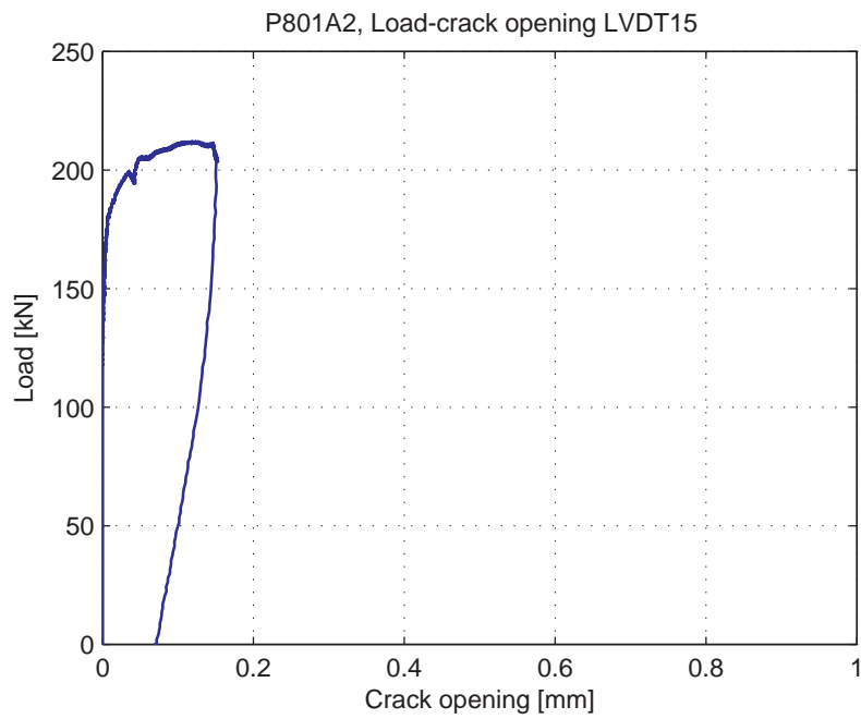
Fig. 5.84.9. Load-Crack opening for LVDT 15
