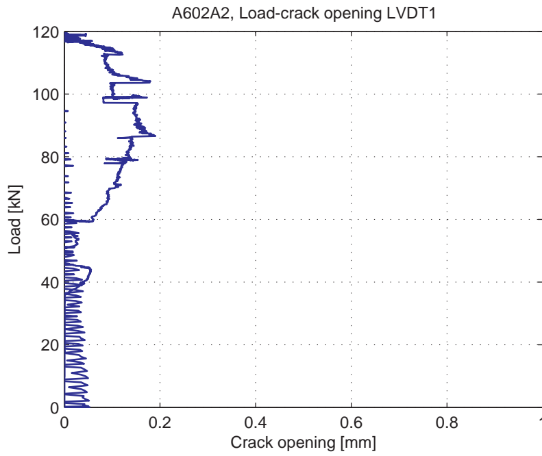
Fig. 5.36.5. Load-Crack opening for LVDT1
