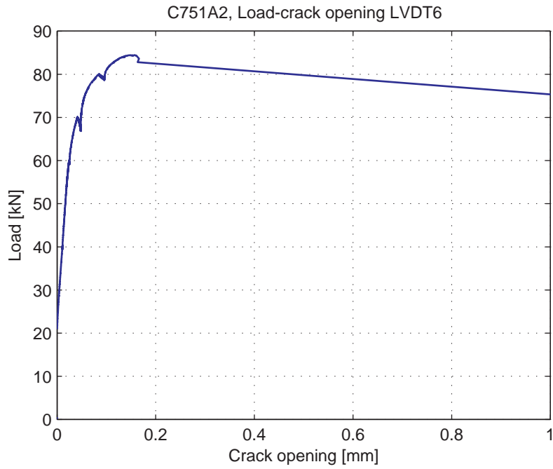
Fig. 5.59.7. Load-Crack opening for LVDT6
