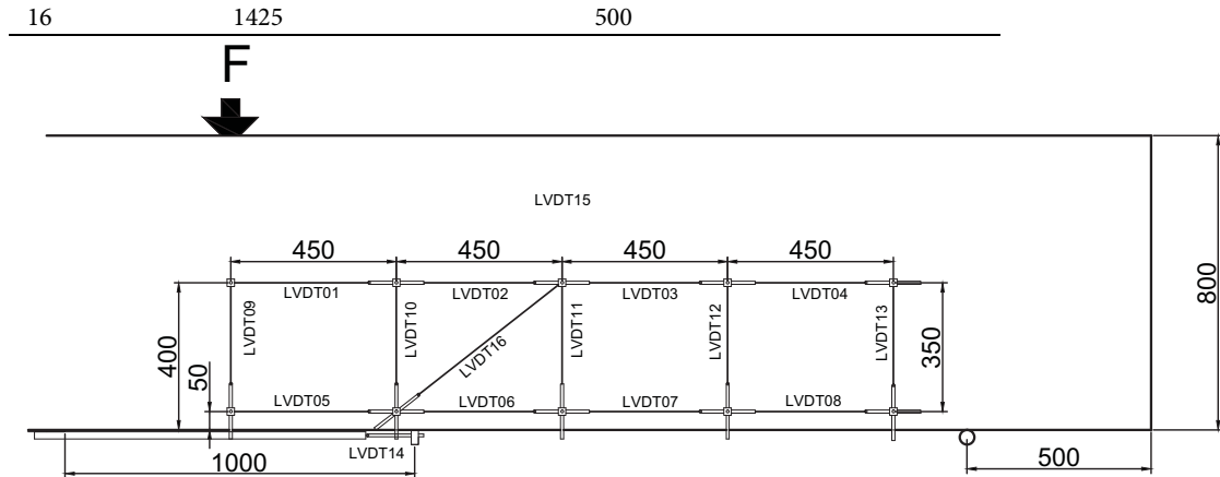
Fig. 5.91.3. LVDT layout and numbering for 800 mm deep beams
