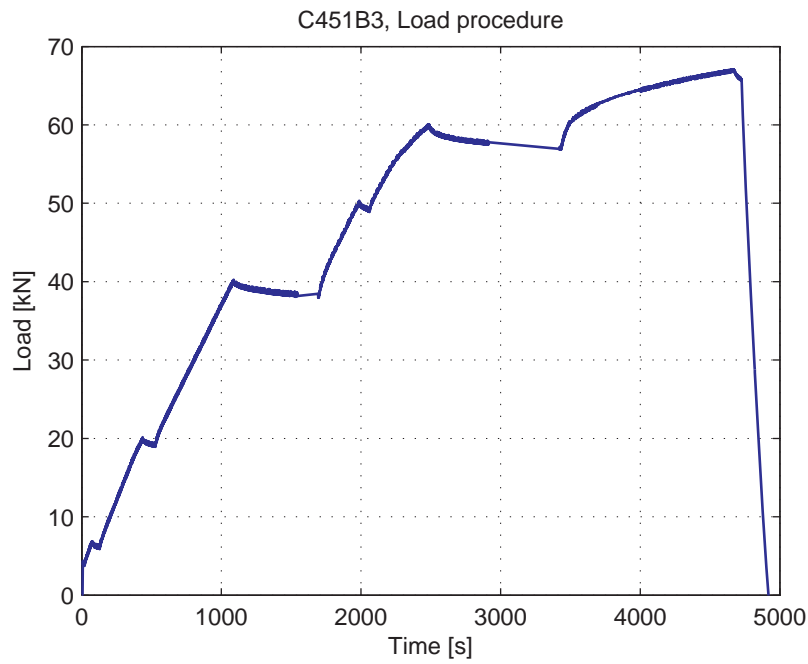
Fig. 5.69.3. Load-Time curve
