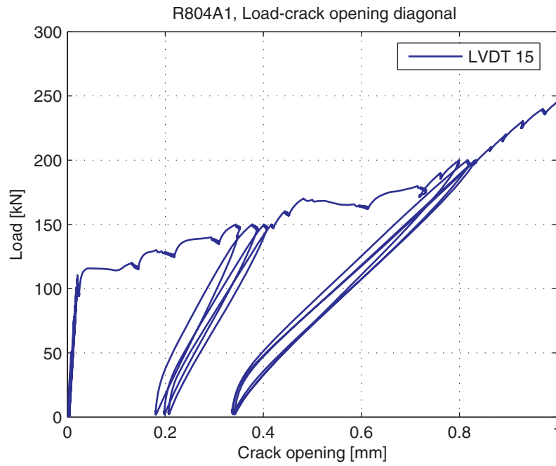
Fig. 5.106.9. Load-Crack opening for LVDT 15 (diagonal)
