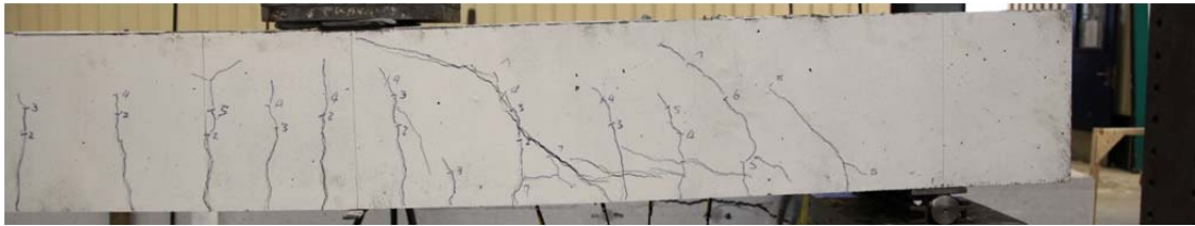
Fig. 5.4.2. Crack pattern after failure south side
