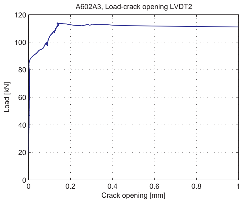
Fig. 5.37.6. Load-Crack opening for LVDT2
