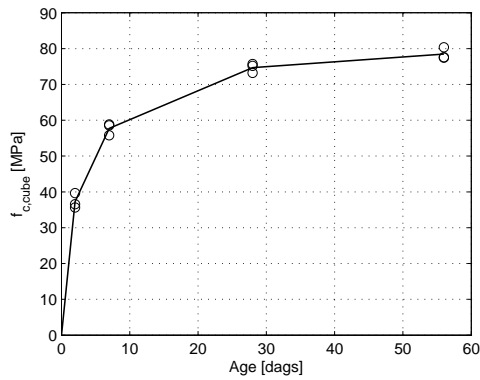
Fig. 2.2.1. F_{c,cube} development for cast 1
