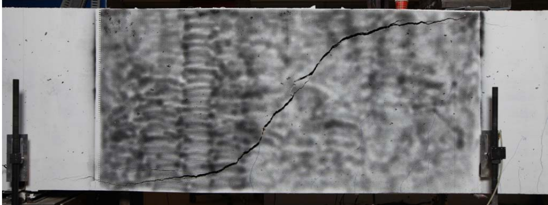
Fig. 5.102.1. Crack pattern after failure at north side of beam
