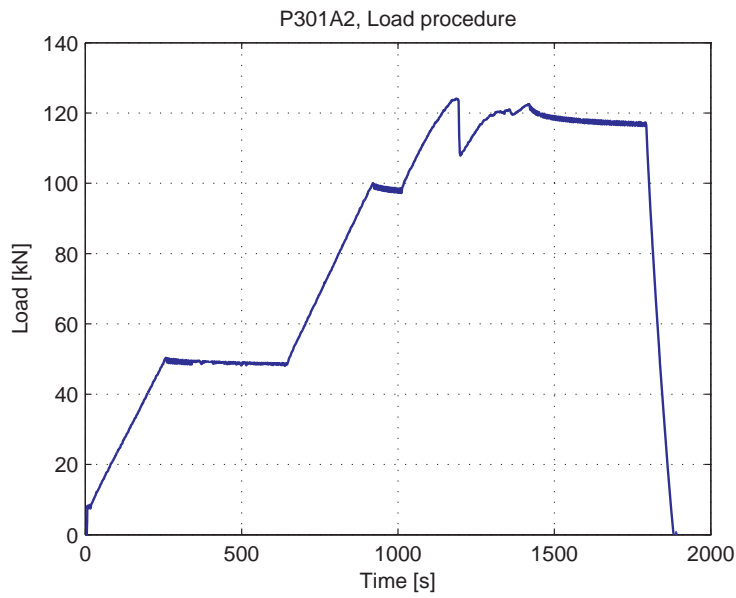
Fig. 5.72.4. Load-Time curve
