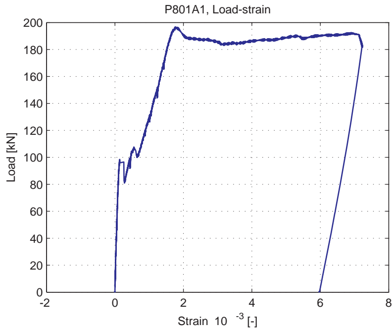
Fig. 5.83.9. Average strain over 1m length, measured at bottom of specimen (LVDT 14)
