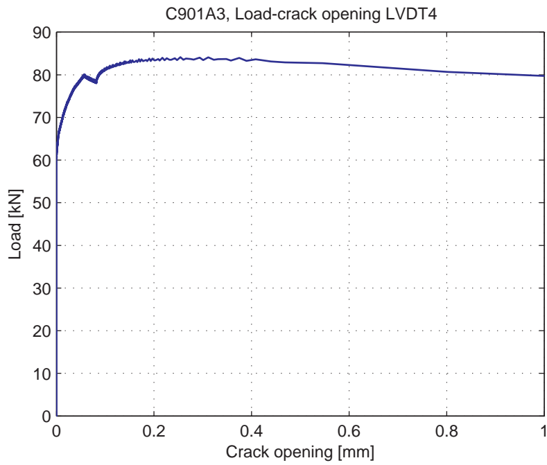
Fig. 5.56.5. Load-Crack opening for LVDT4
