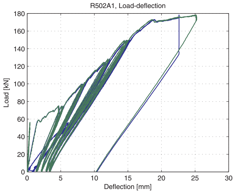
Fig. 5.97.5. Load-deflection curve
