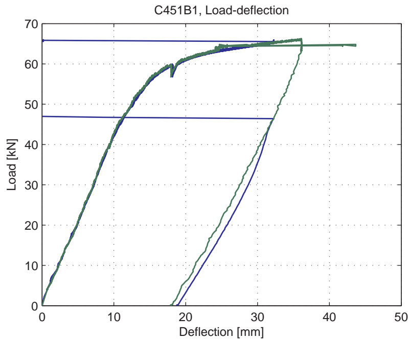
Fig. 5.67.4. Load-deflection curve
