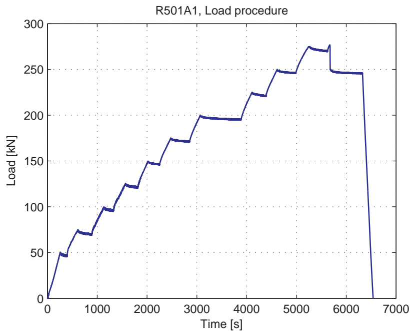
Fig. 5.95.4. Load-Time curve
