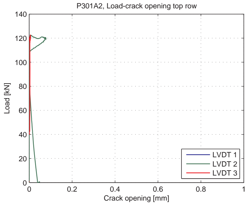
Fig. 5.72.6. Load-Crack opening for LVDT's 1-3 (top row)
