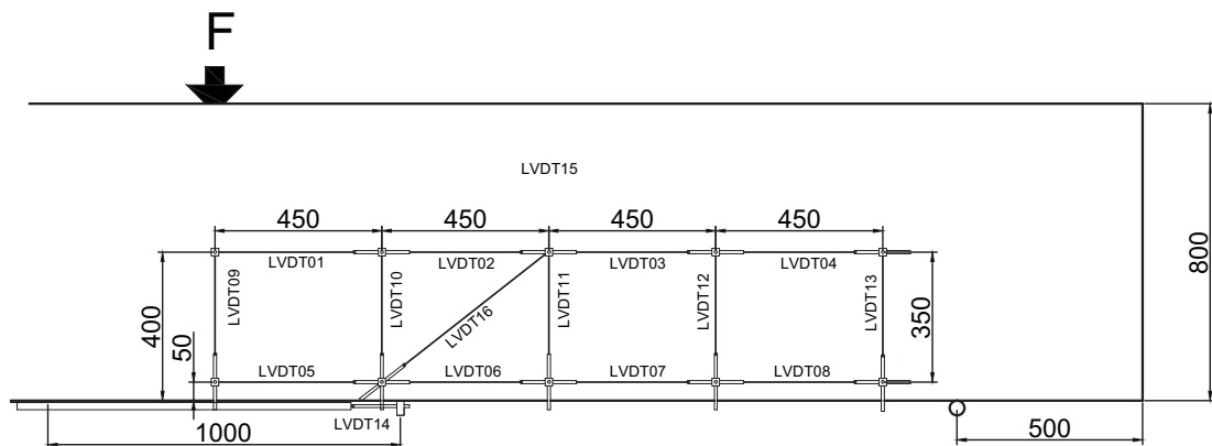
Fig. 5.100.3. LVDT layout and numbering for 800 mm deep beams
