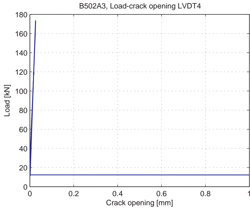
Fig. 5.52.5. Load-Crack opening for LVDT4
