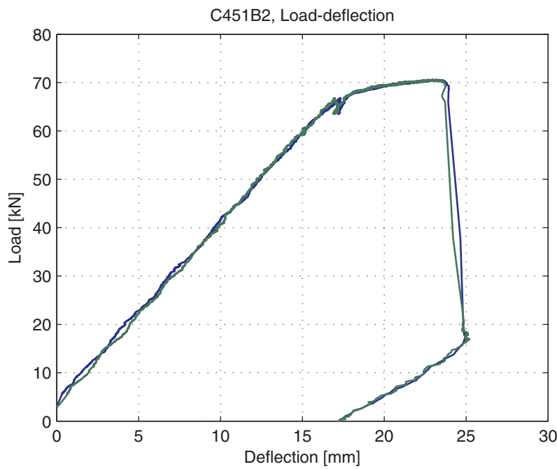
Fig. 5.68.4. Load-deflection curve
