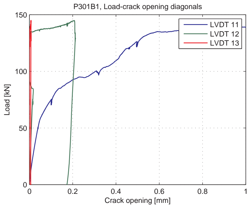
Fig. 5.75.9. Load-Crack opening for LVDT's 11-13 (diagonal)
