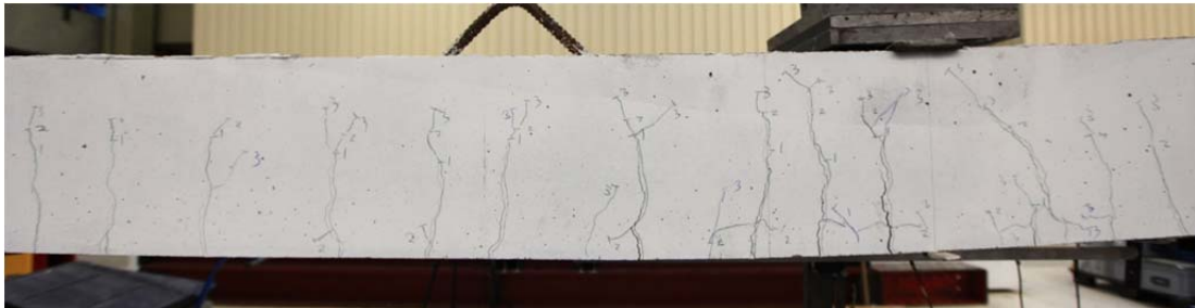
Fig. 5.63.2. Crack pattern after failure south side
