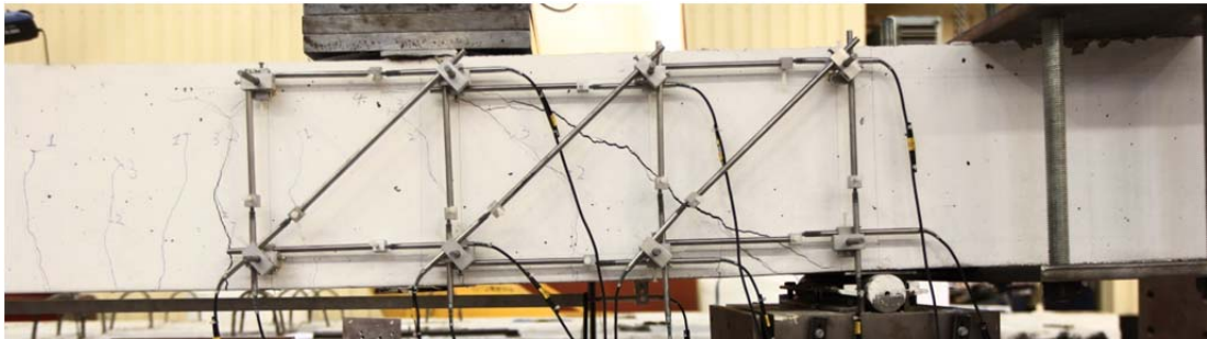
Fig. 5.72.2. Crack pattern after failure back side
