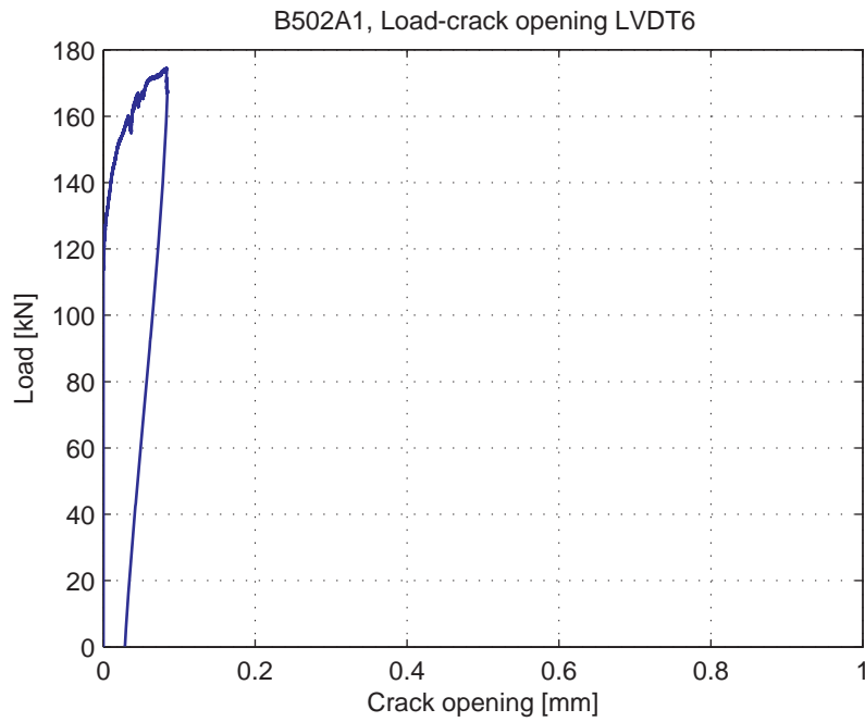
Fig. 5.50.7. Load-Crack opening for LVDT6
