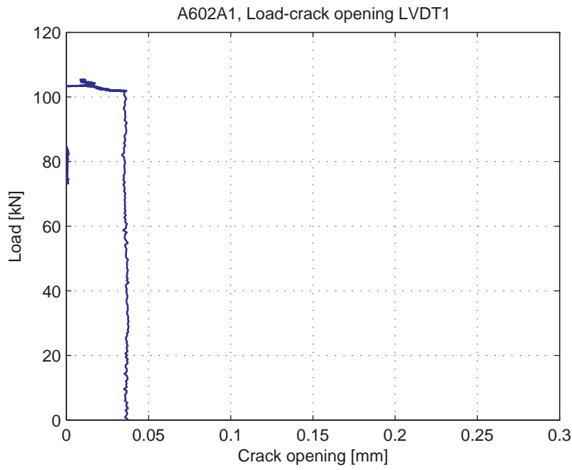
Fig. 5.35.5. Load-Crack opening for LVDT1
