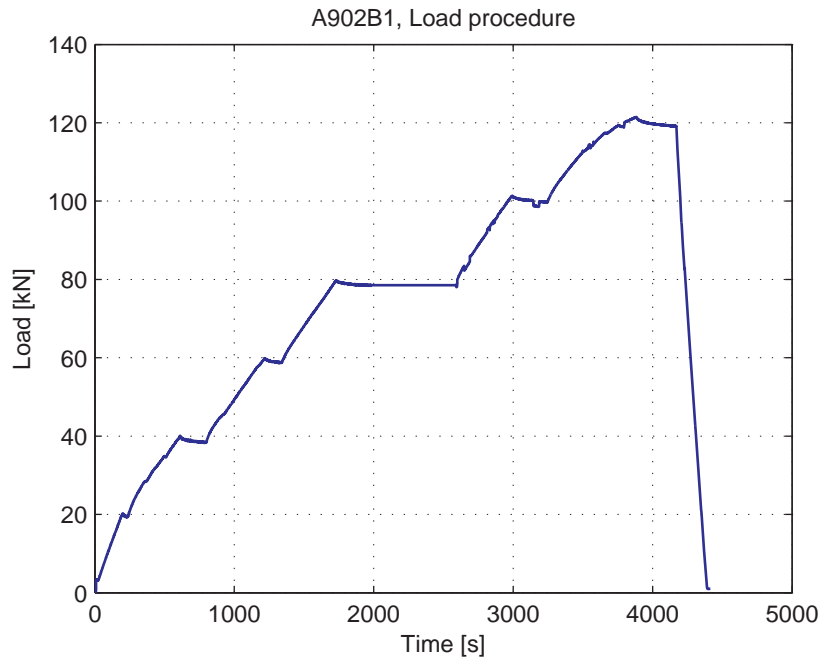
Fig. 5.20.3. Load-Time curve
