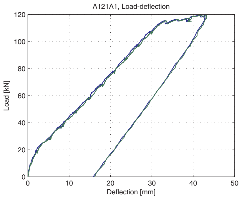
Fig. 5.1.4. Load-deflection curve
