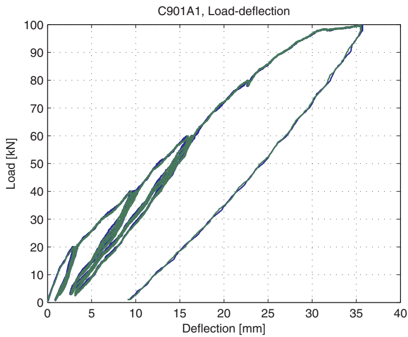
Fig. 5.54.2. Load-deflection curve
