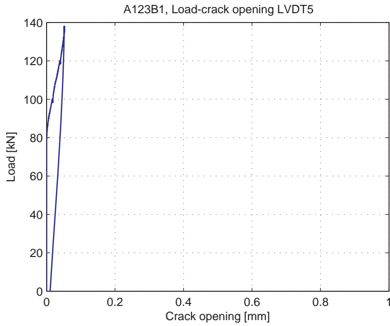
Fig. 5.10.6. Load-Crack opening for LVDT5
