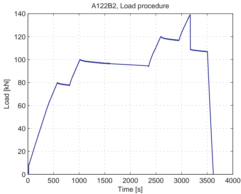
Fig. 5.7.3. Load-Time curve
