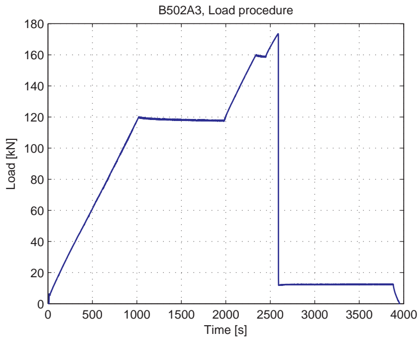
Fig. 5.52.3. Load-Time curve
