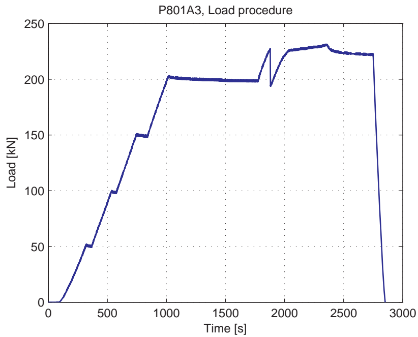
Fig. 5.85.4. Load-Time curve
