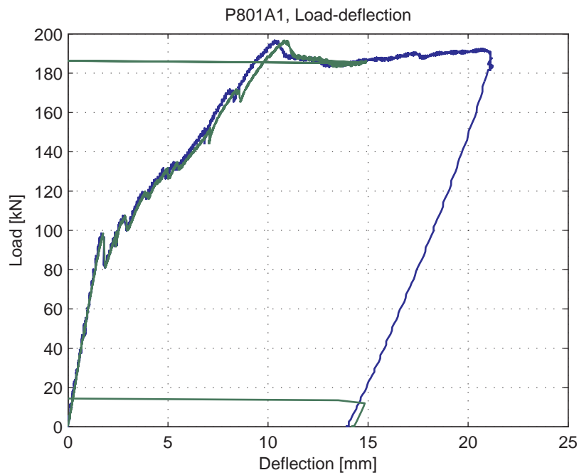
Fig. 5.83.4. Load-deflection curve
