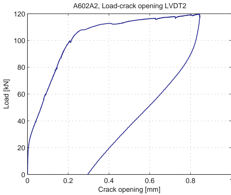
Fig. 5.36.6. Load-Crack opening for LVDT2
