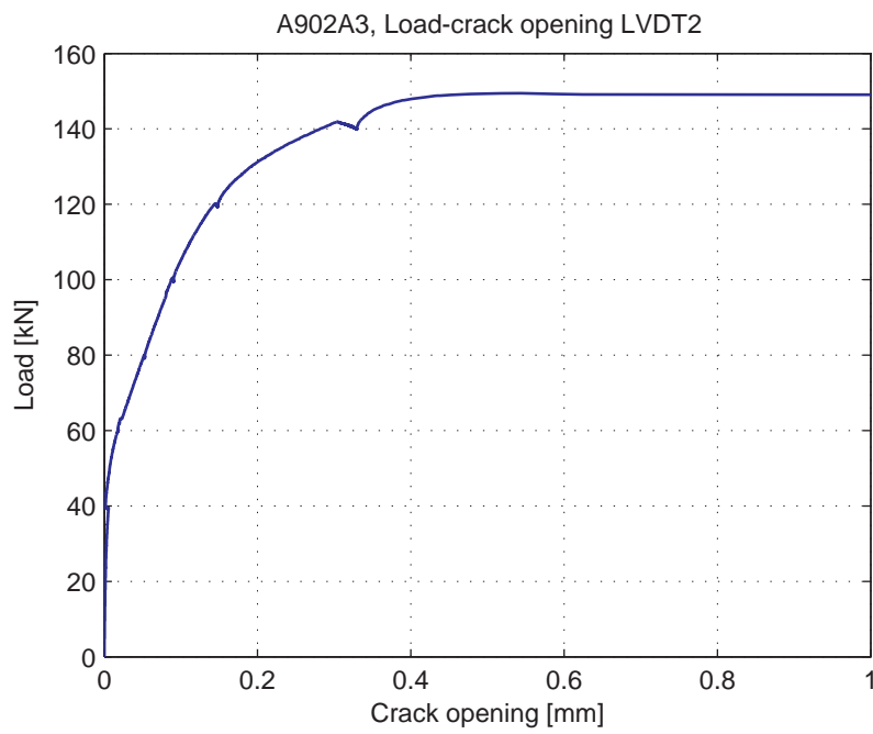
Fig. 5.19.6. Load-Crack opening for LVDT2
