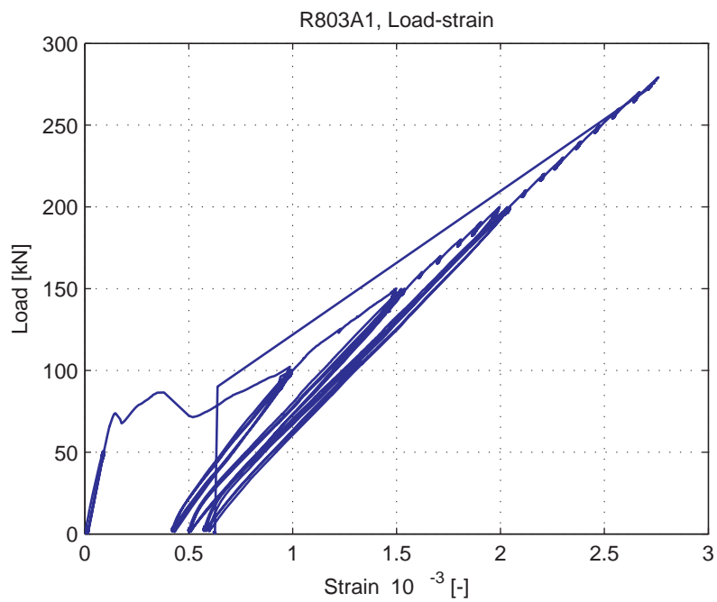
Fig. 5.104.11. Average strain over 1m length, measured at bottom of specimen (LVDT 14)
