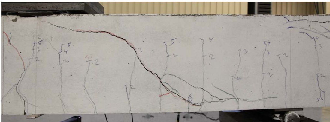
Fig. 5.19.2. Crack pattern after failure south side
