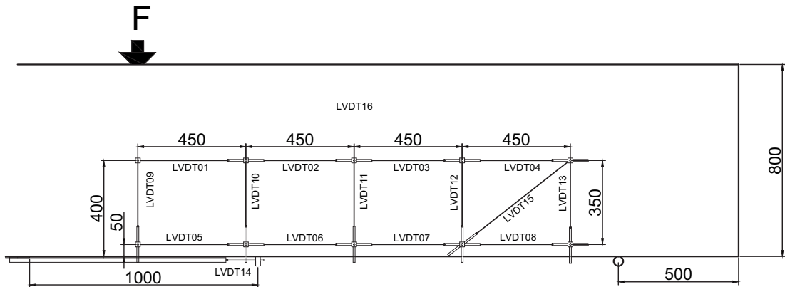
Fig. 5.106.3. LVDT layout and numbering for 800 mm deep beams
