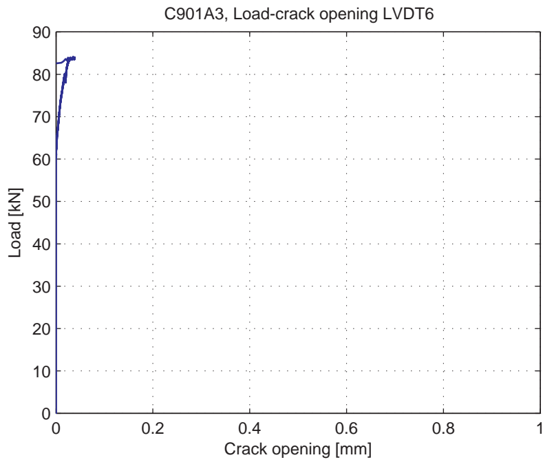
Fig. 5.56.7. Load-Crack opening for LVDT6
