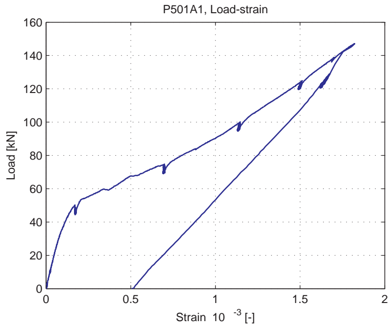
Fig. 5.76.9. Average strain over 1m length, measured at bottom of specimen (LVDT 14)
