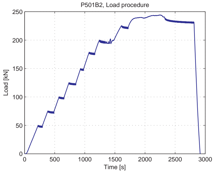
Fig. 5.79.4. Load-Time curve
