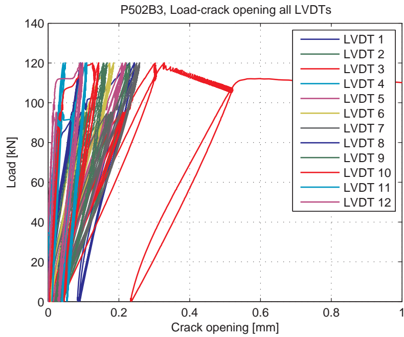
Fig. 5.82.12. Load-Crack opening third part of test for all LVDT's
