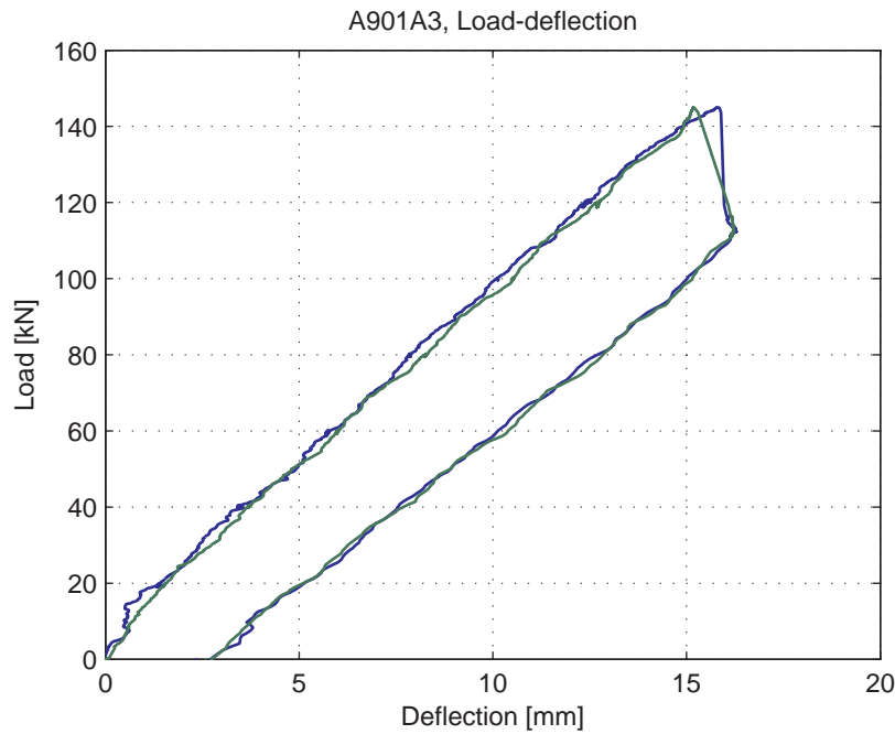
Fig. 5.14.4. Load-deflection curve
