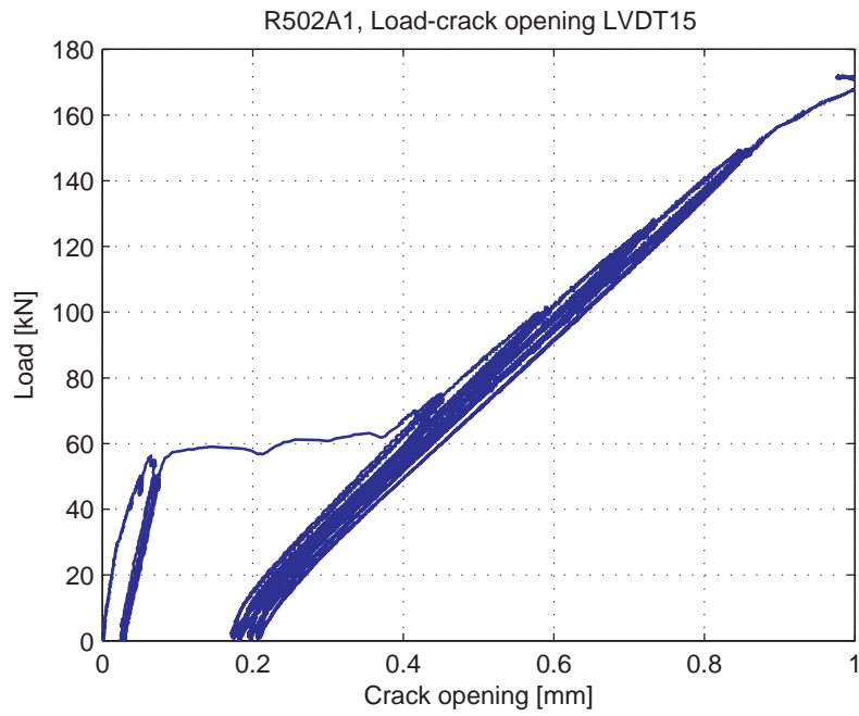
Fig. 5.97.10. Load-Crack opening for LVDT 15
