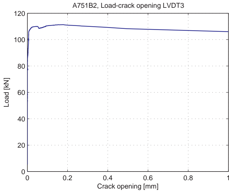
Fig. 5.25.7. Load-Crack opening for LVDT3
