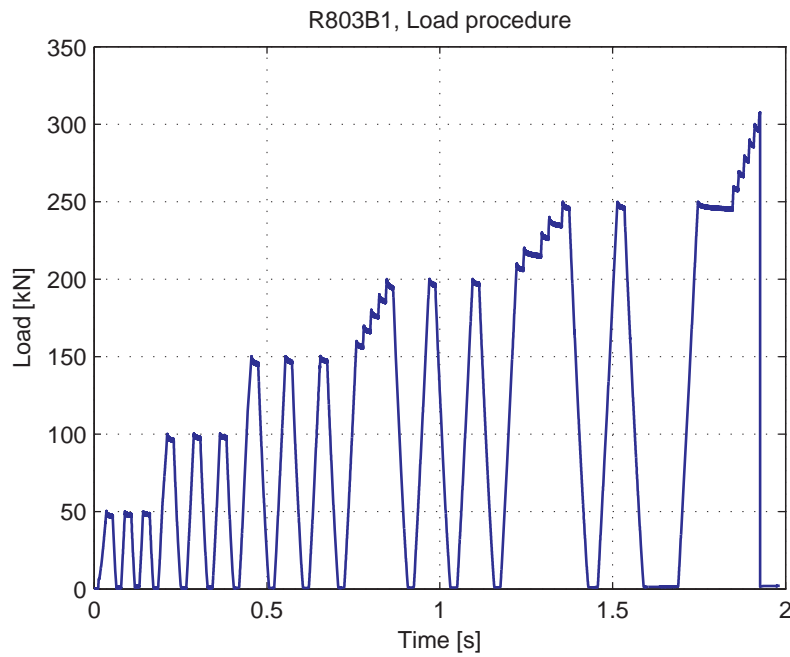
Fig. 5.105.4. Load-Time curve
