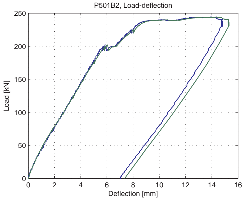
Fig. 5.79.5. Load-deflection curve
