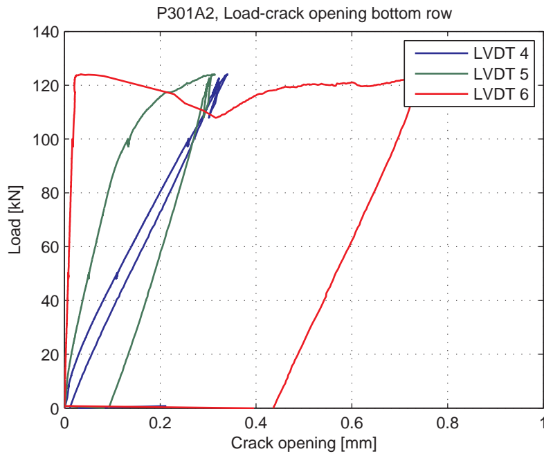
Fig. 5.72.8. Load-Crack opening for LVDT's 4-6 (bottom row)
