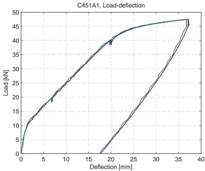
Fig. 5.62.4. Load-deflection curve
