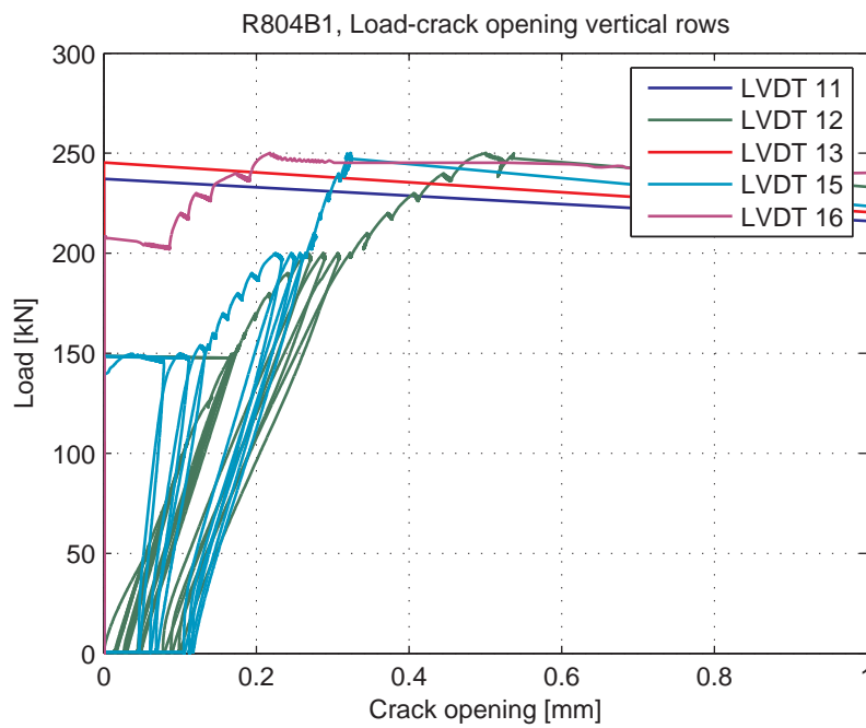
Fig. 5.107.7. Load-Crack opening for LVDT's 9-13 (vertical LVDT's)
