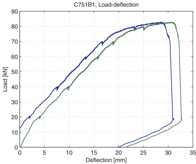
Fig. 5.61.4. Load-deflection curve
