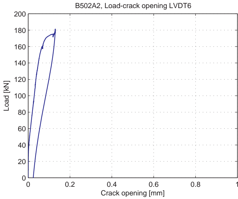
Fig. 5.51.7. Load-Crack opening for LVDT6
