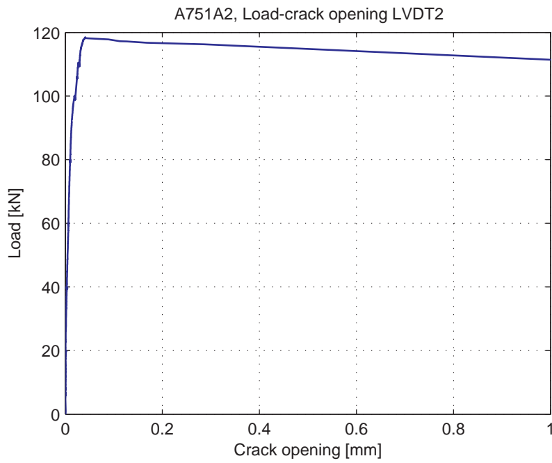
Fig. 5.23.6. Load-Crack opening for LVDT2
