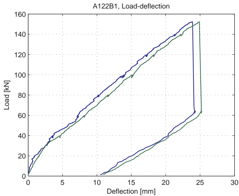
Fig. 5.6.4. Load-deflection curve
