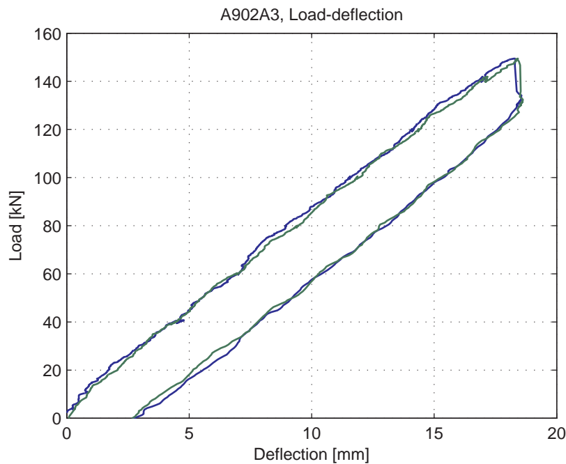
Fig. 5.19.4. Load-deflection curve
