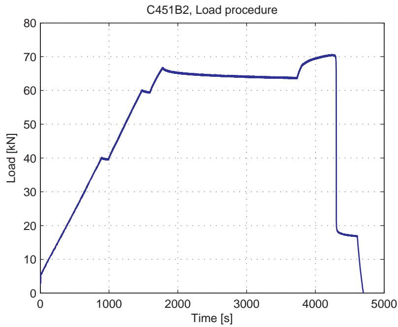
Fig. 5.68.3. Load-Time curve
