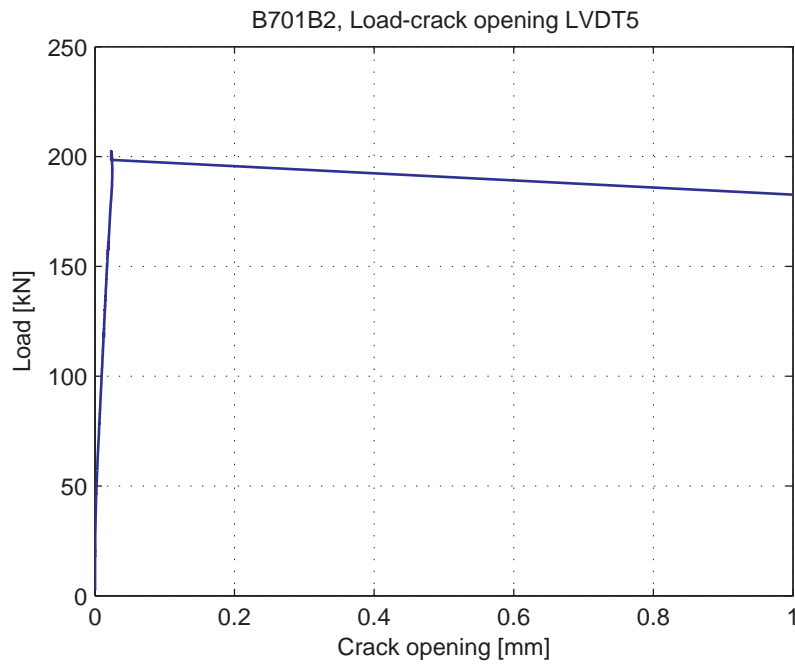
Fig. 5.44.6. Load-Crack opening for LVDT5
