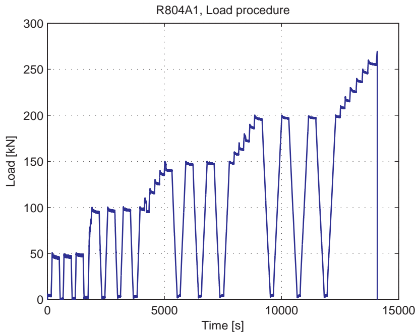
Fig. 5.106.4. Load-Time curve
