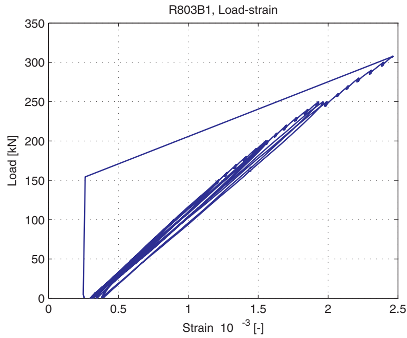
Fig. 5.105.9. Average strain over 1m length, measured at bottom of specimen (LVDT 14)
