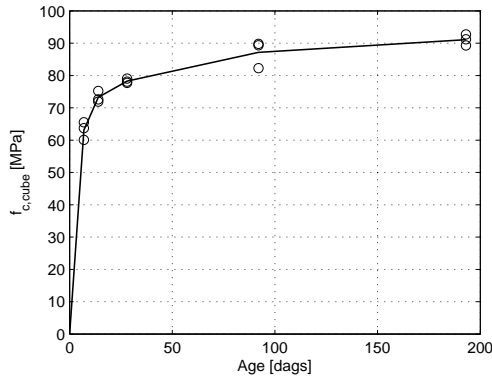
Fig. 2.2.9. F_{c,cube} development for cast 6
