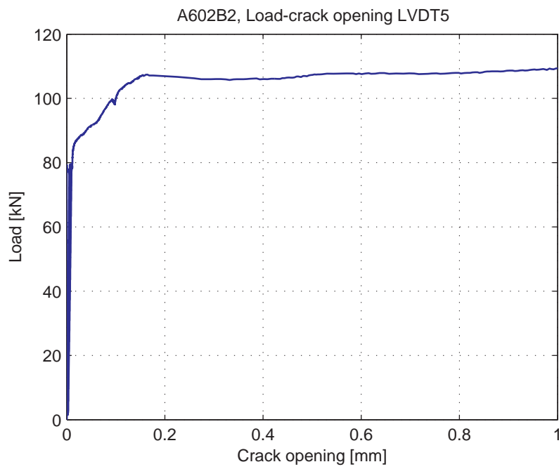
Fig. 5.39.6. Load-Crack opening for LVDT5
