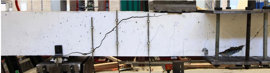
Fig. 5.9.1. Crack pattern after failure north side
