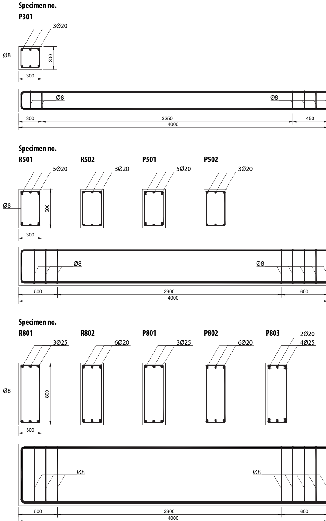
Fig. 2.3.2. Reinforcement layout for tested specimens in P and R series
