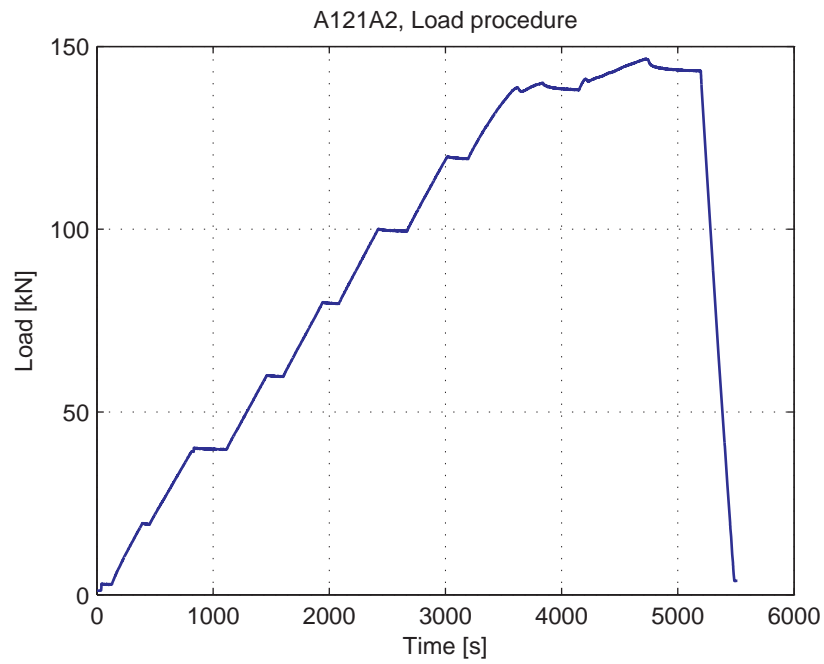
Fig. 5.2.3. Load-Time curve
