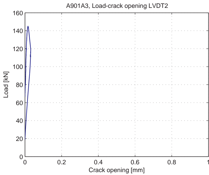
Fig. 5.14.6. Load-Crack opening for LVDT2
