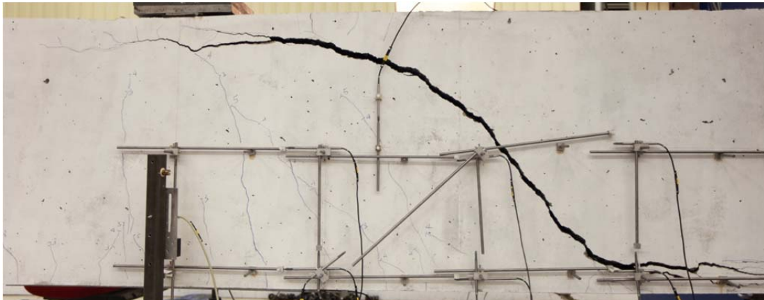
Fig. 5.87.2. Crack pattern after failure and LVDT layout at south side of beam
