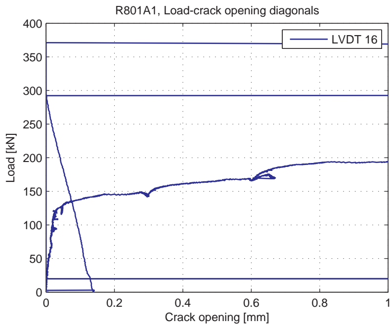
Fig. 5.100.9. Load-Crack opening for LVDT 16 (diagonal)
