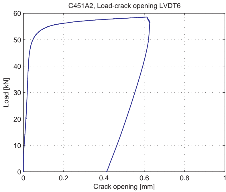
Fig. 5.63.7. Load-Crack opening for LVDT6
