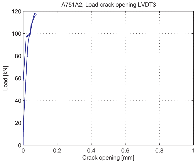
Fig. 5.23.7. Load-Crack opening for LVDT3
