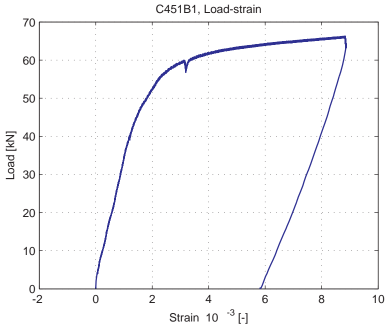
Fig. 5.67.8. Average strain over 1m length, measured at bottom of specimen (LVDT 3)
