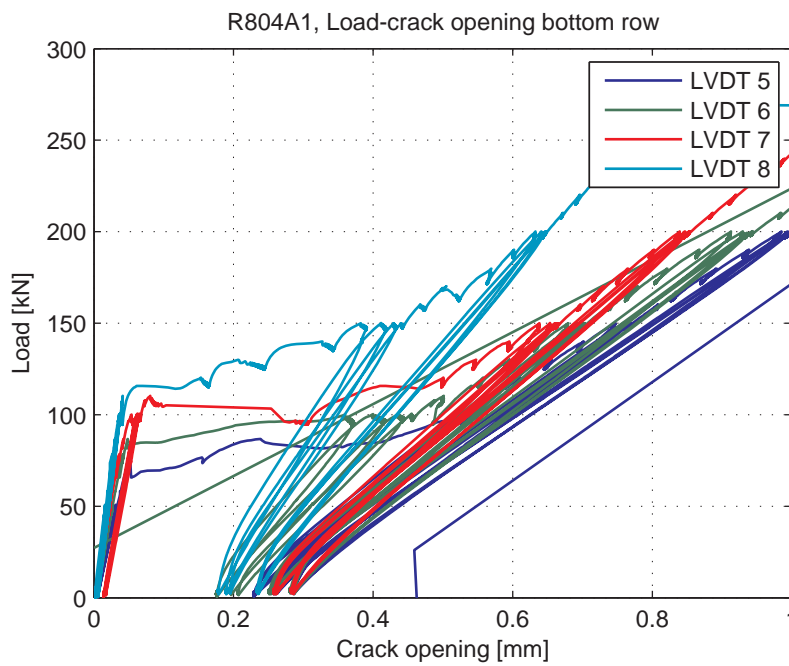
Fig. 5.106.8. Load-Crack opening for LVDT's 5-8 (bottom row)
