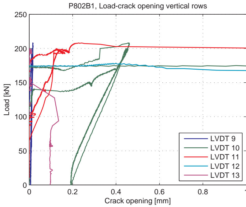
Fig. 5.88.7. Load-Crack opening for LVDT's 9-13 (vertical LVDT's)
