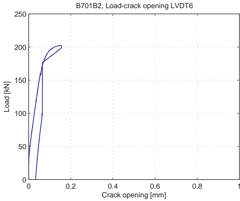
Fig. 5.44.7. Load-Crack opening for LVDT6
