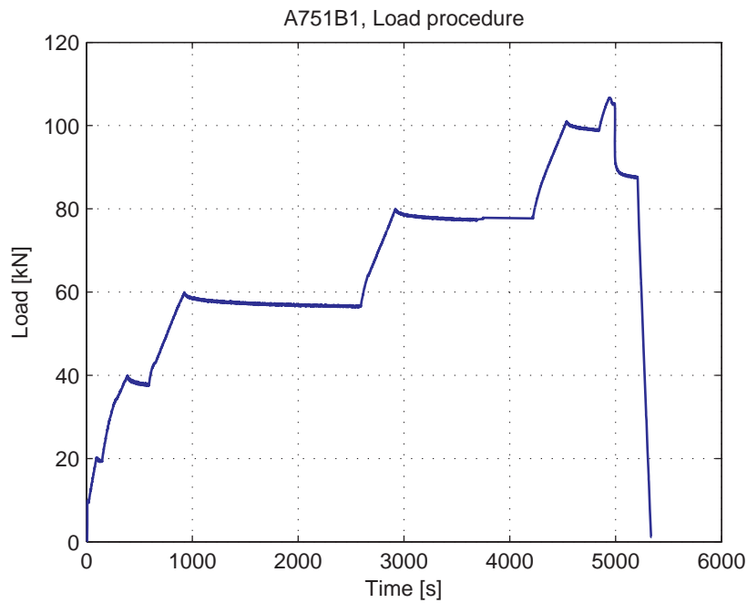
Fig. 5.24.3. Load-Time curve
