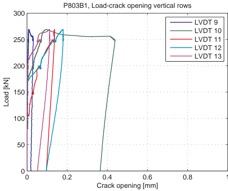
Fig. 5.90.7. Load-Crack opening for LVDT's 9-13 (vertical LVDT's)
