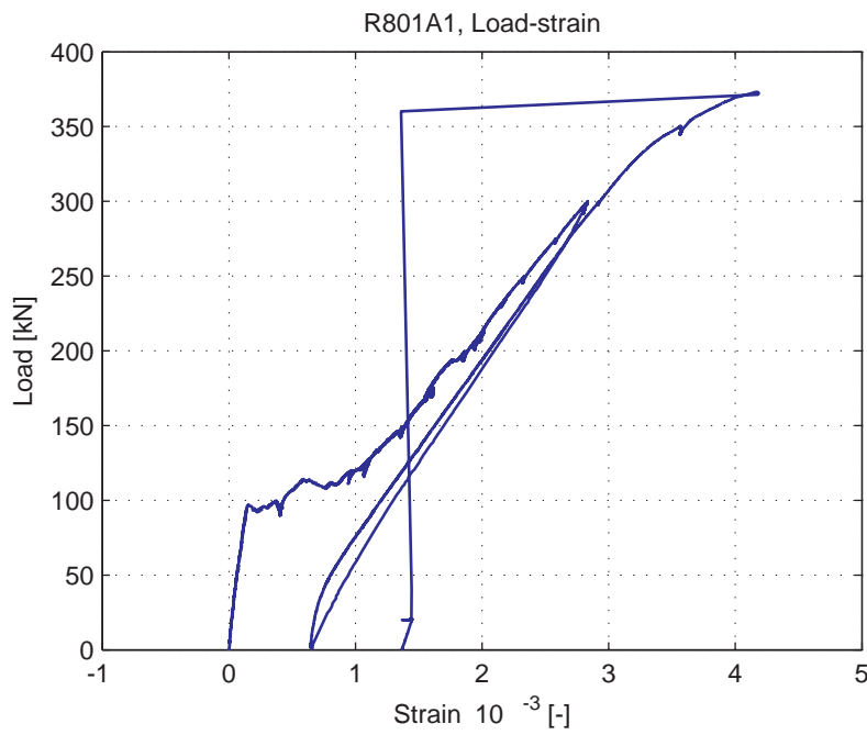
Fig. 5.100.11. Average strain over 1m length, measured at bottom of specimen (LVDT 14)
