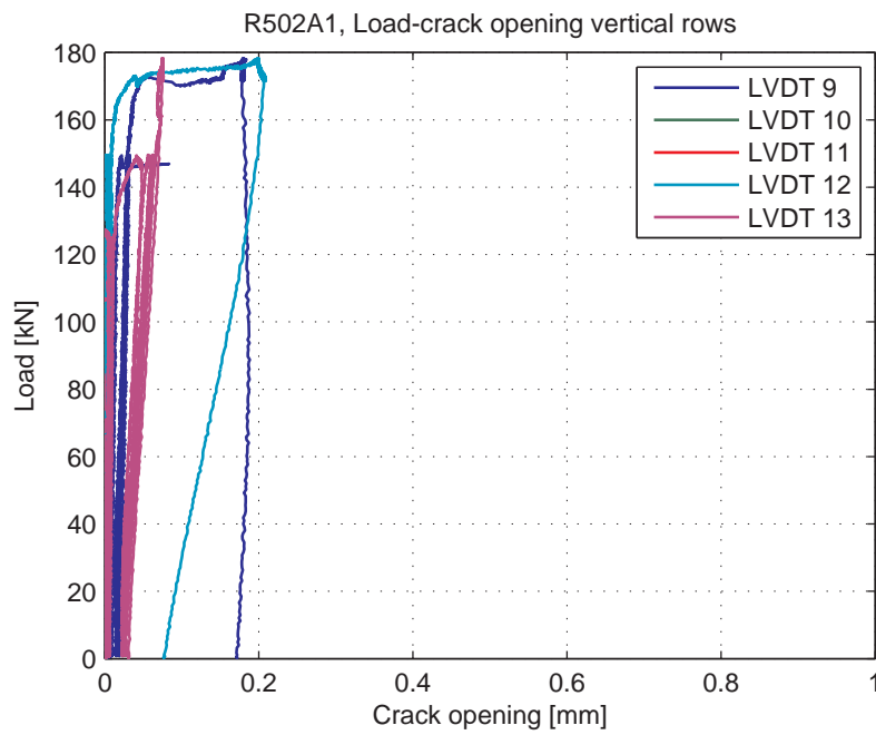
Fig. 5.97.7. Load-Crack opening for LVDT's 9-13 (vertical LVDT's)
