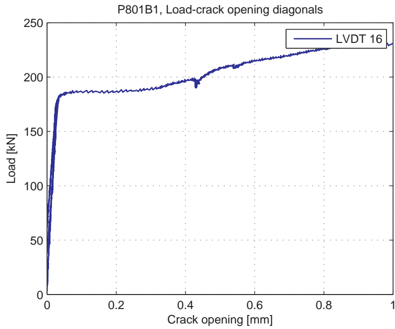
Fig. 5.86.10. Load-Crack opening for LVDT 16 (diagonal)
