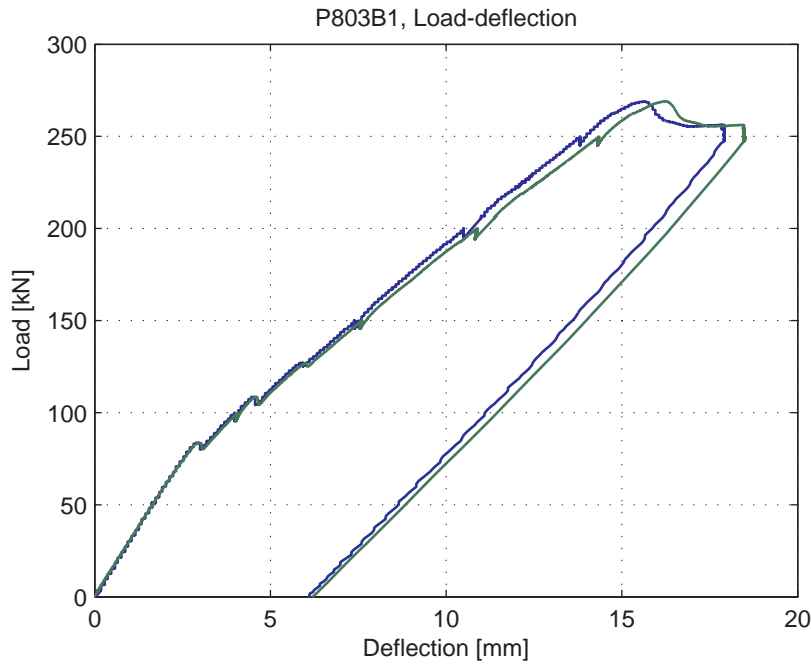
Fig. 5.90.5. Load-deflection curve
