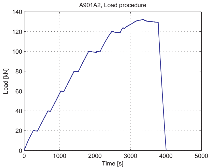
Fig. 5.13.3. Load-Time curve
