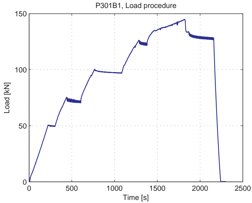
Fig. 5.75.4. Load-Time curve
