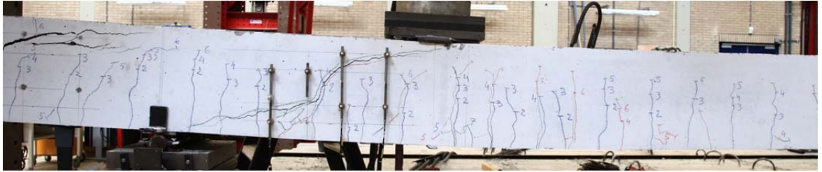
Fig. 5.19.1. Crack pattern after failure north side
