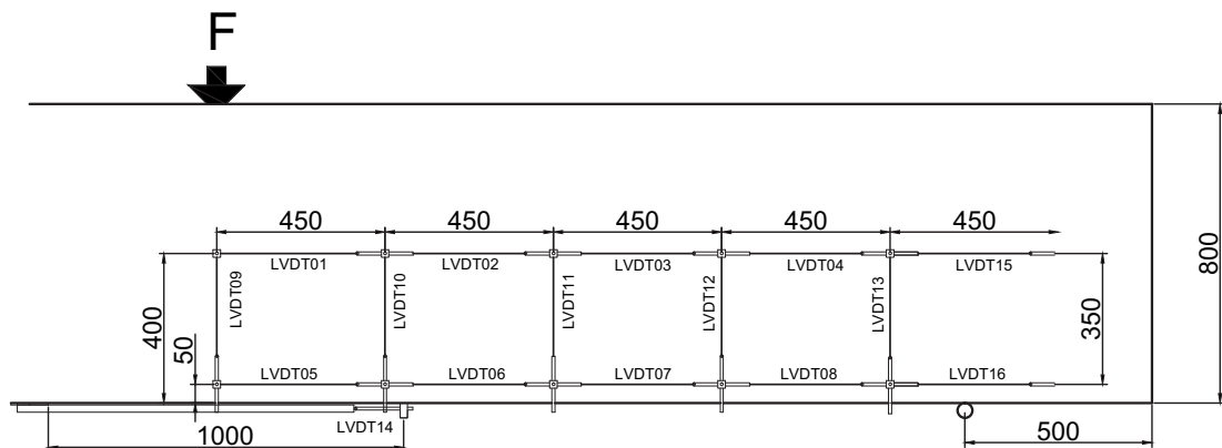
Fig. 5.104.3. LVDT layout and numbering for 800 mm deep beams
