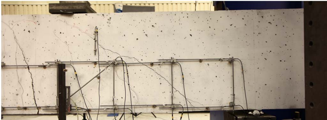
Fig. 5.85.2. Crack pattern after failure south side
