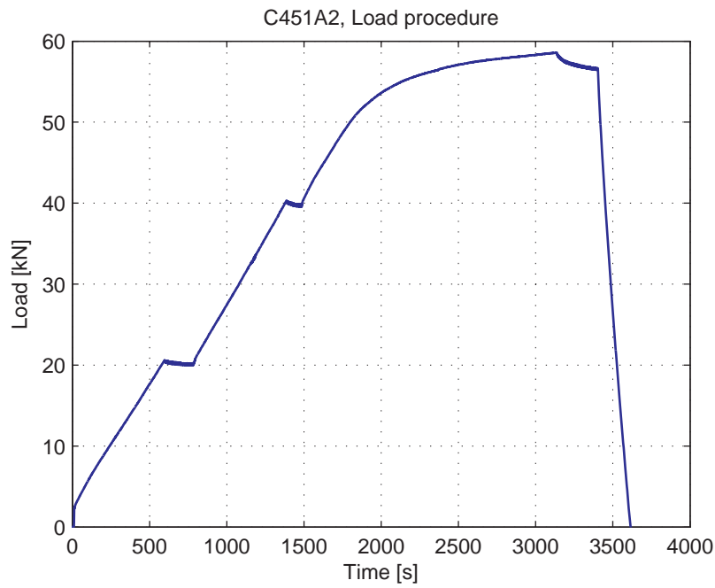
Fig. 5.63.3. Load-Time curve
