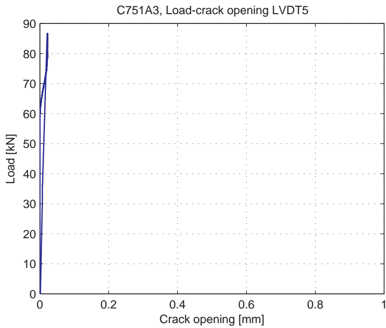
Fig. 5.60.6. Load-Crack opening for LVDT5
