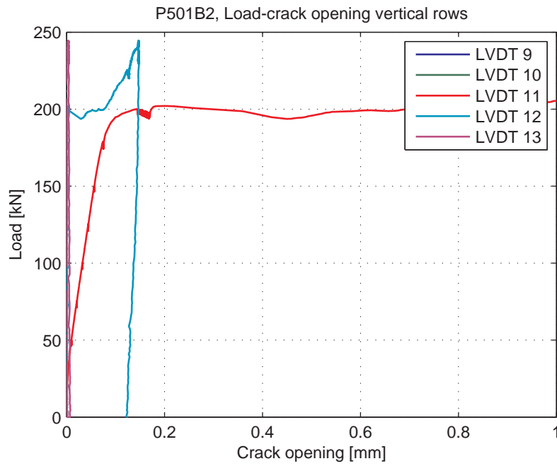
Fig. 5.79.7. Load-Crack opening for LVDT's 9-13 (vertical LVDT's)
