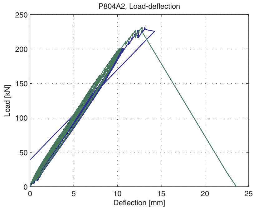
Fig. 5.93.4. Load-deflection curve
