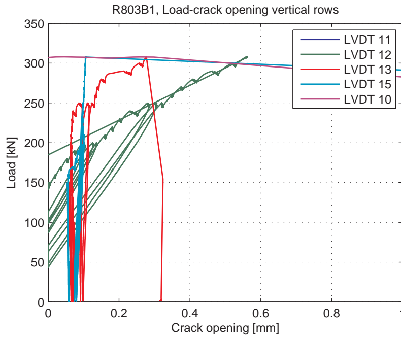
Fig. 5.105.7. Load-Crack opening for LVDT's 9-13 (vertical LVDT's)
