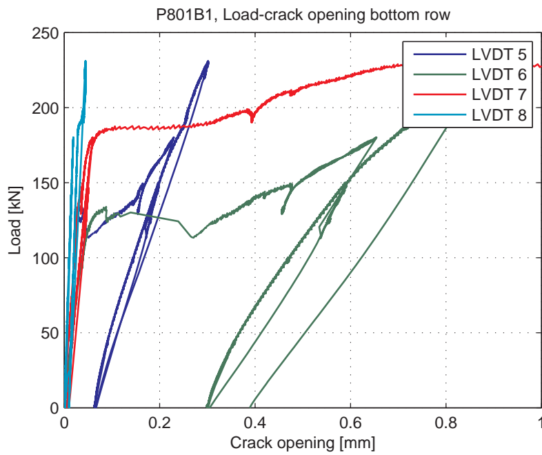
Fig. 5.86.9. Load-Crack opening for LVDT's 5-8 (bottom row)
