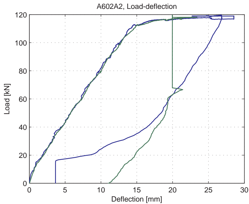
Fig. 5.36.4. Load-deflection curve
