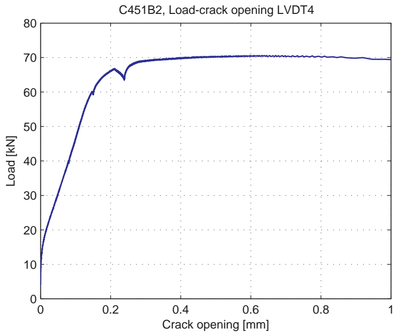
Fig. 5.68.5. Load-Crack opening for LVDT4
