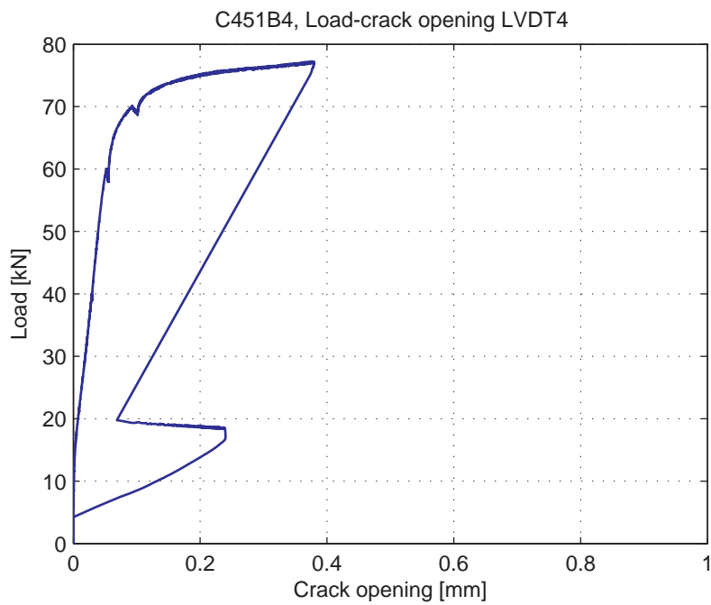
Fig. 5.70.6. Load-Crack opening for LVDT4
