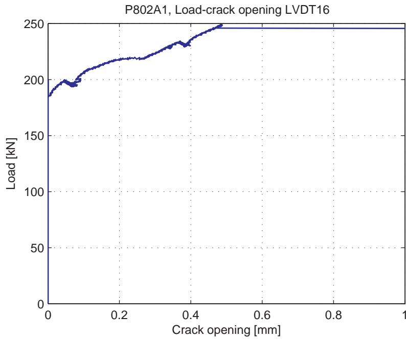
Fig. 5.87.9. Load-Crack opening for LVDT16 (diagonal)
