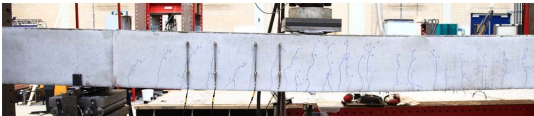
Fig. 5.12.1. Crack pattern after failure north side
