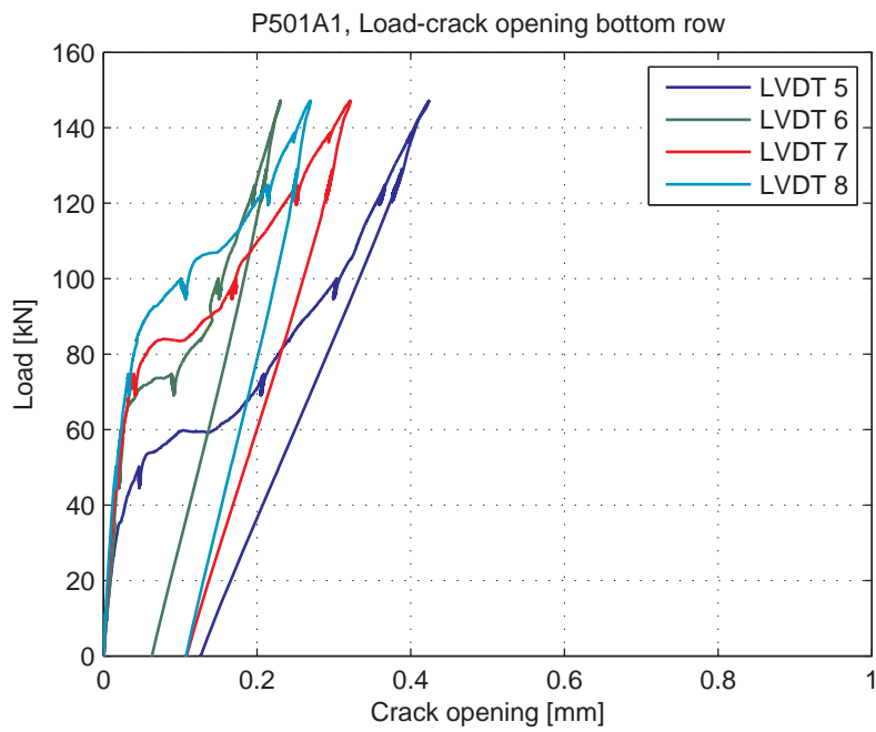
Fig. 5.76.8. Load-Crack opening for LVDT's 5-8 (bottom row)
