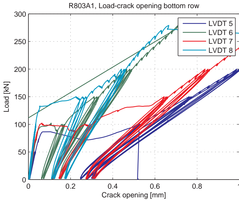
Fig. 5.104.8. Load-Crack opening for LVDT's 5-8 (bottom row)
