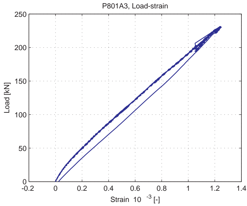
Fig. 5.85.11. Average strain over 1m length, measured at bottom of specimen (LVDT 14)
