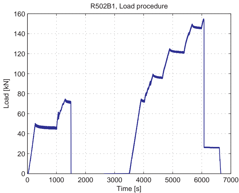
Fig. 5.99.4. Load-Time curve
