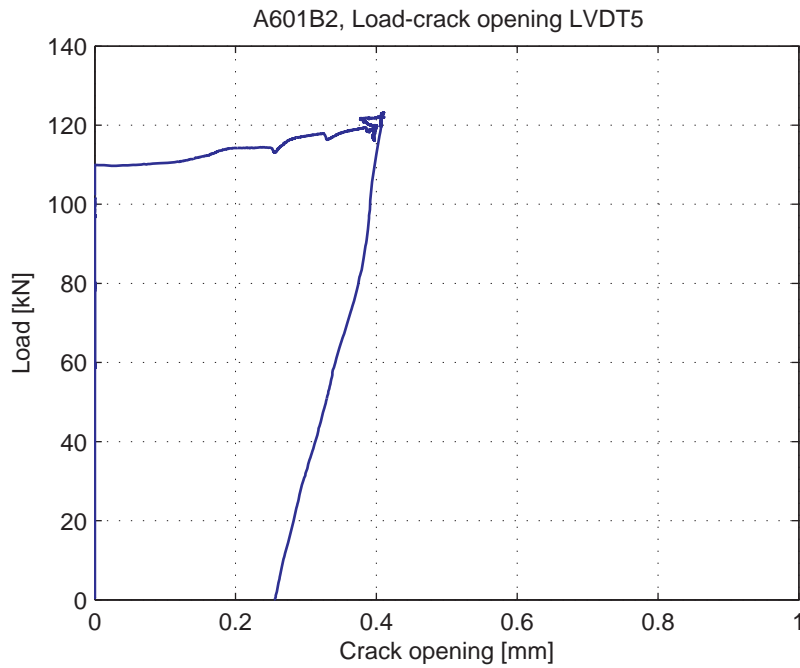
Fig. 5.34.8. Load-Crack opening for LVDT5
