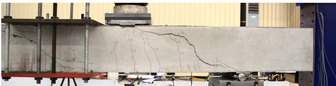
Fig. 5.16.2. Crack pattern after failure south side
