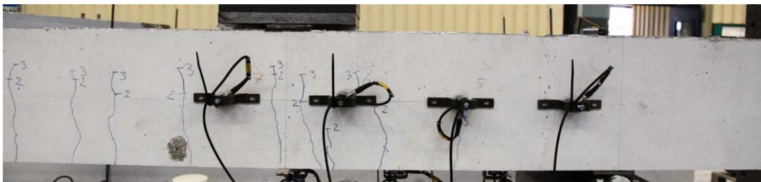
Fig. 5.29.3. Sensors used for Acoustic Emission measurements
