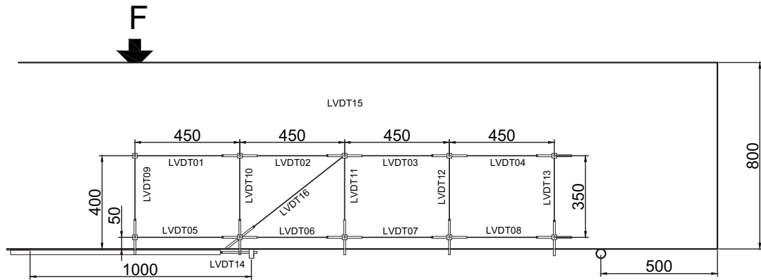
Fig. 5.85.3. LVDT layout and numbering for 800 mm deep beams
