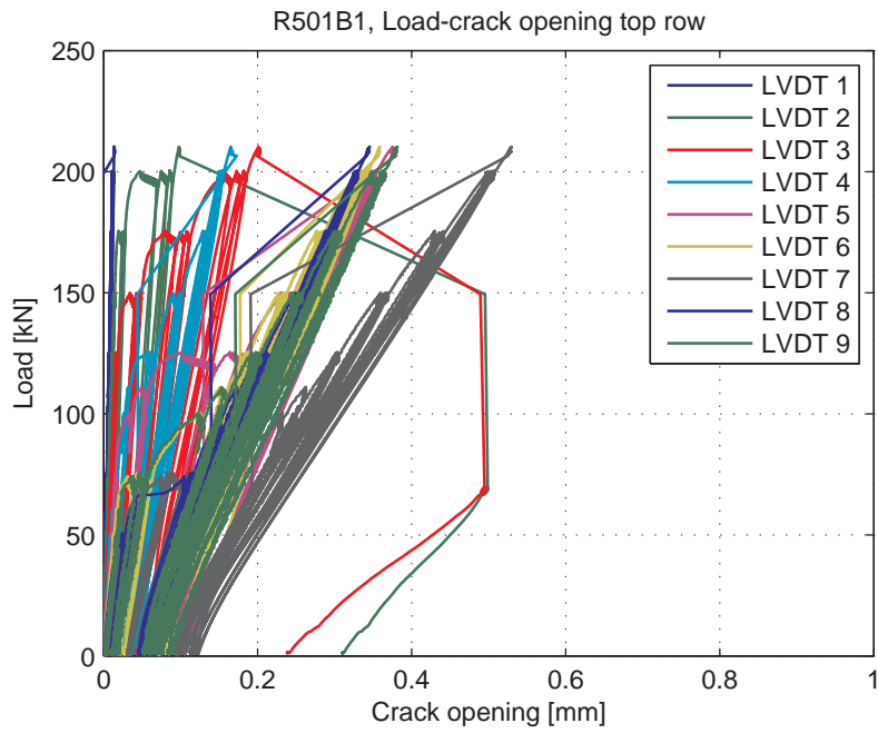
Fig. 5.96.6. Load-Crack opening for LVDT's 1-9
