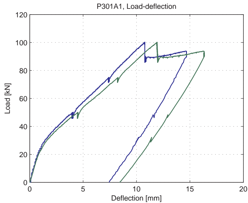
Fig. 5.71.4. Load-deflection curve
