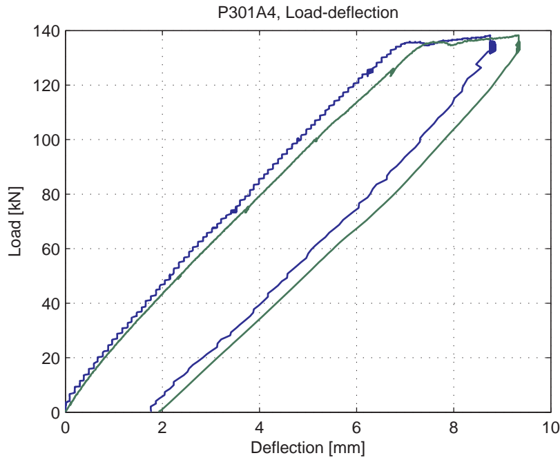
Fig. 5.74.5. Load-deflection curve
