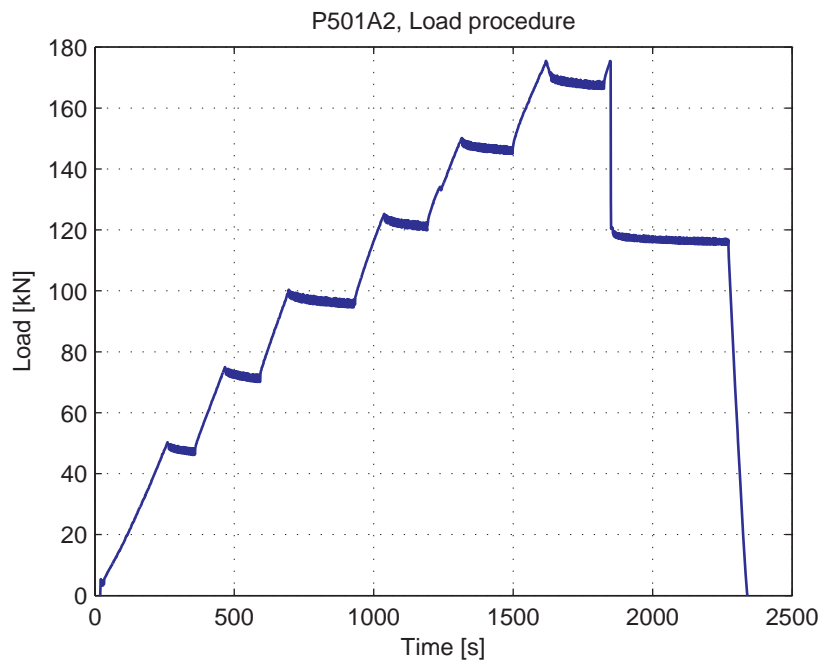
Fig. 5.77.4. Load-Time curve
