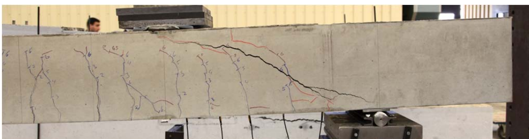
Fig. 5.14.2. Crack pattern after failure south side
