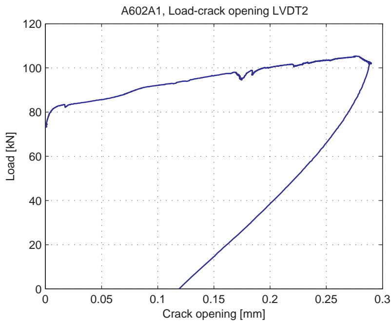
Fig. 5.35.6. Load-Crack opening for LVDT2
