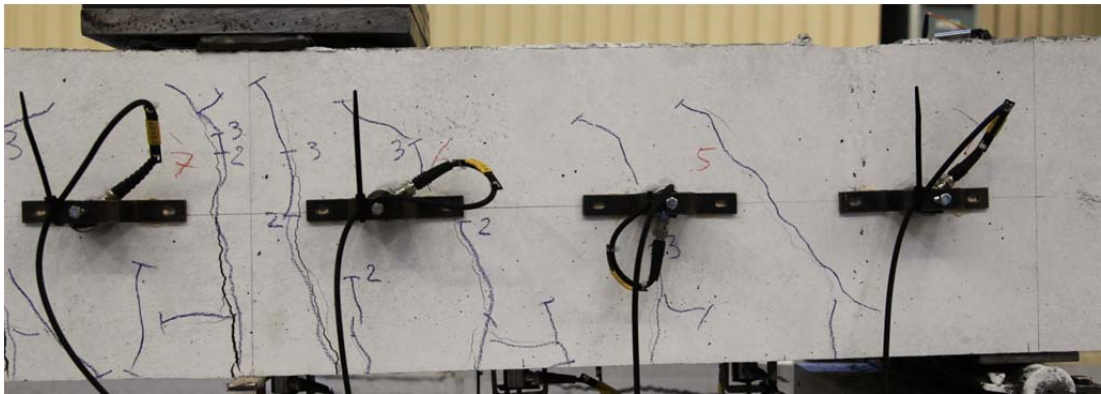
Fig. 5.29.2. Crack pattern after failure south side
