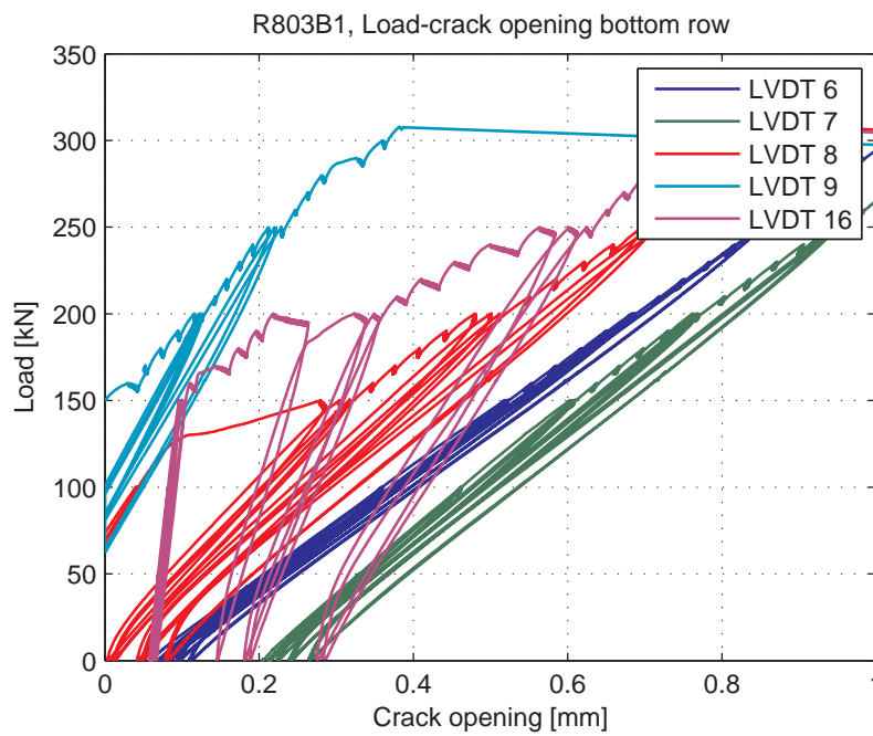
Fig. 5.105.8. Load-Crack opening for LVDT's 5-8 (bottom row)
