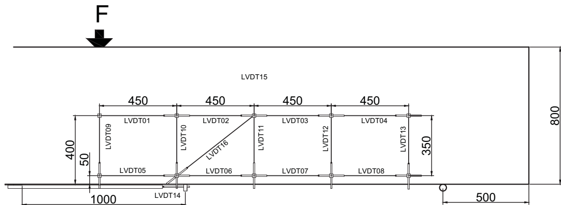
Fig. 5.88.3. LVDT layout and numbering for 800 mm deep beams
