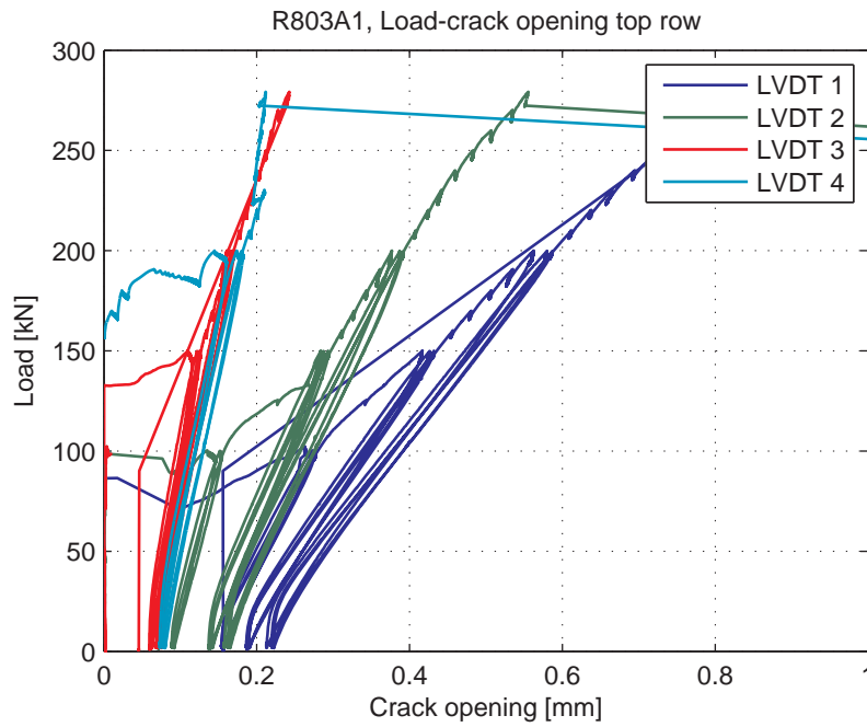
Fig. 5.104.6. Load-Crack opening for LVDT's 1-4 (top row)
