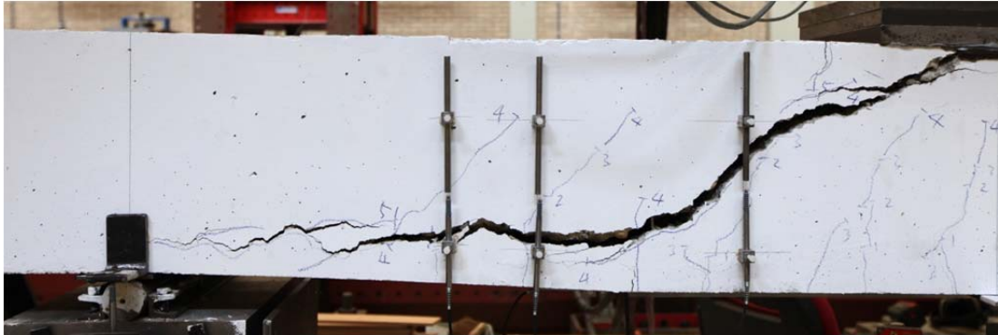
Fig. 5.61.1. Crack pattern after failure north side
