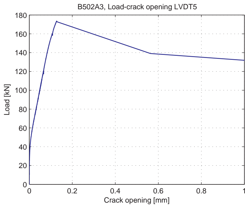
Fig. 5.52.6. Load-Crack opening for LVDT5
