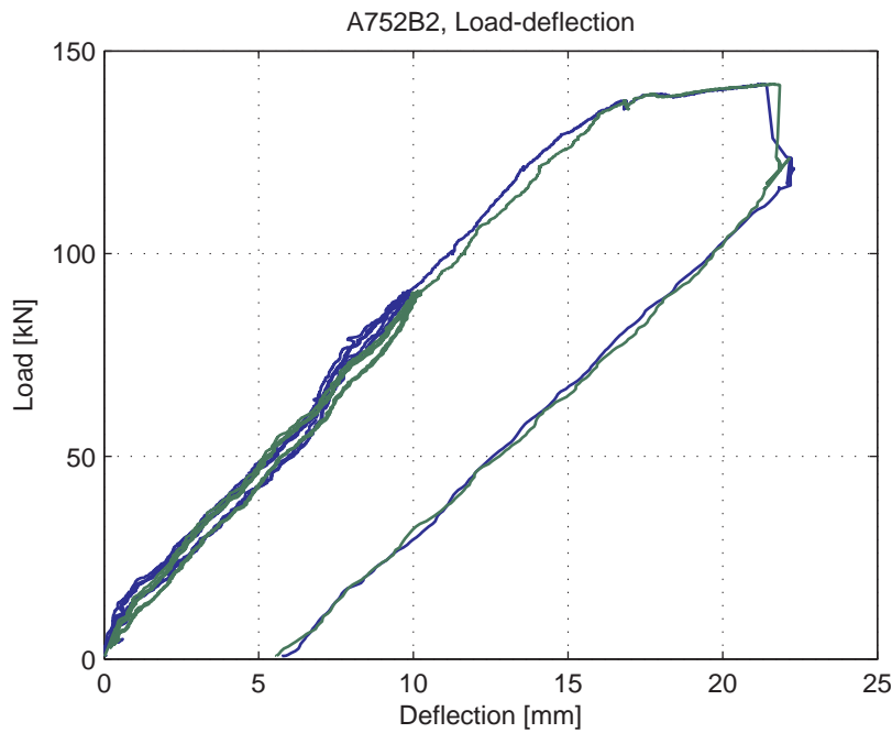
Fig. 5.30.4. Load-deflection curve
