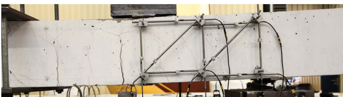
Fig. 5.73.2. Crack pattern after failure back side
