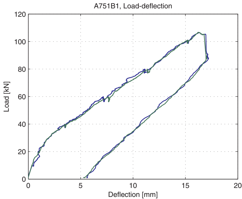
Fig. 5.24.4. Load-deflection curve
