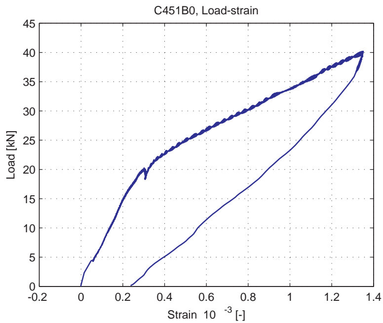
Fig. 5.66.3. Average strain over 1m length, measured at bottom of specimen (LVDT 3)
