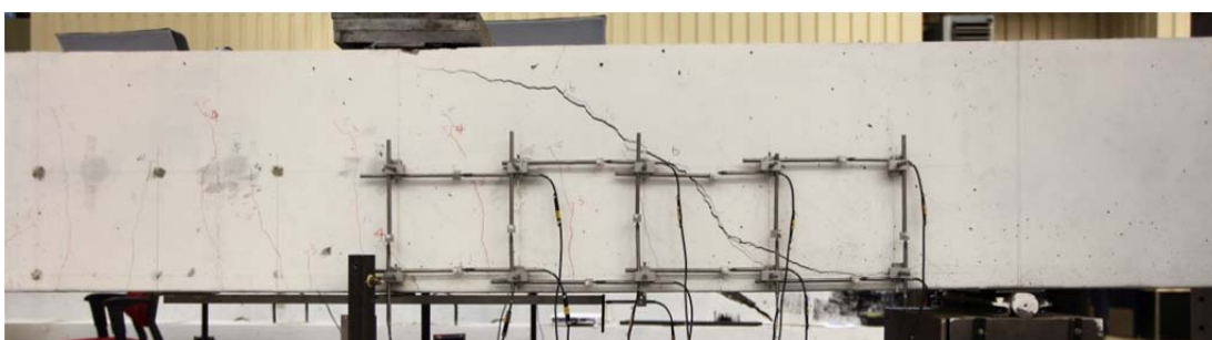
Fig. 5.77.2. Crack pattern after failure back side
