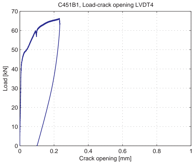
Fig. 5.67.5. Load-Crack opening for LVDT4
