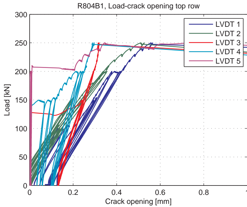
Fig. 5.107.6. Load-Crack opening for LVDT's 1-4 (top row)
