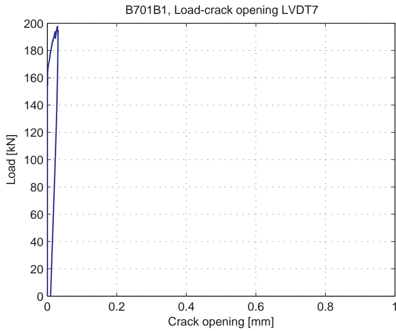
Fig. 5.43.8. Load-Crack opening for LVDT7
