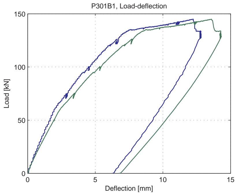
Fig. 5.75.5. Load-deflection curve
