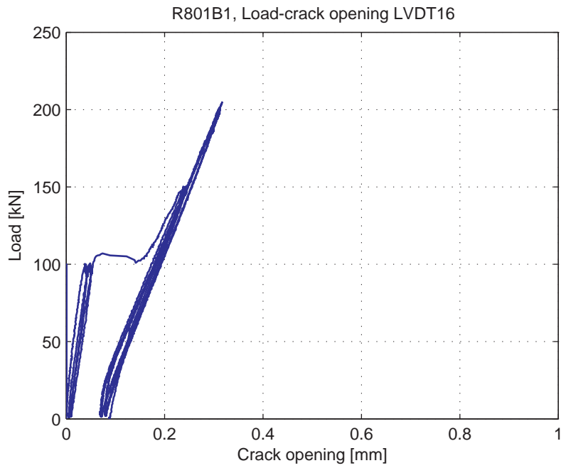
Fig. 5.101.10. Load-Crack opening for LVDT 16
