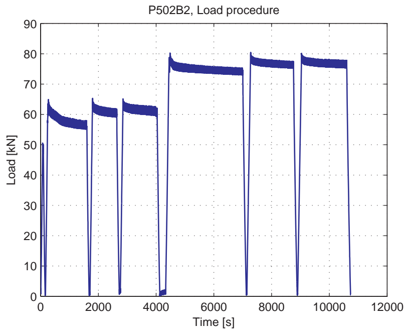
Fig. 5.82.5. Load-Time curve for second part of test
