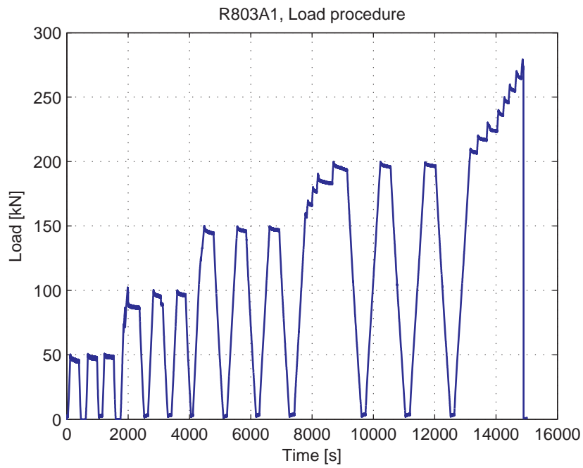
Fig. 5.104.4. Load-Time curve
