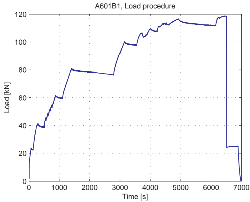
Fig. 5.33.3. Load-Time curve
