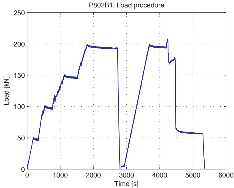
Fig. 5.88.4. Load-Time curve
