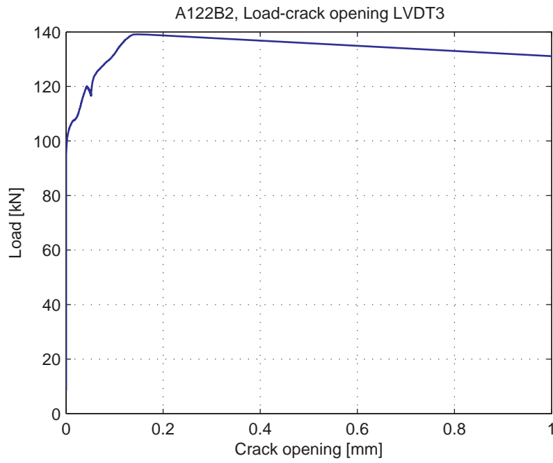
Fig. 5.7.7. Load-Crack opening for LVDT3
