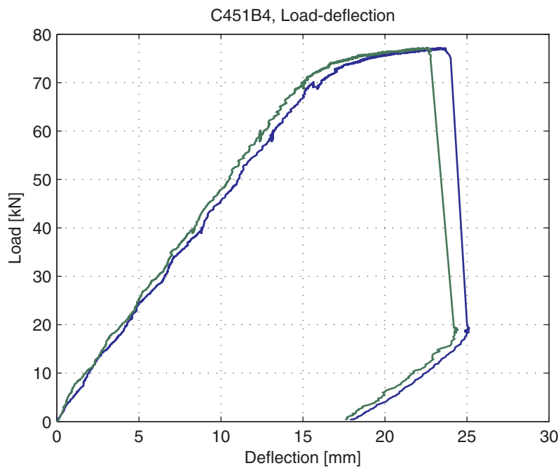
Fig. 5.70.4. Load-deflection curve
