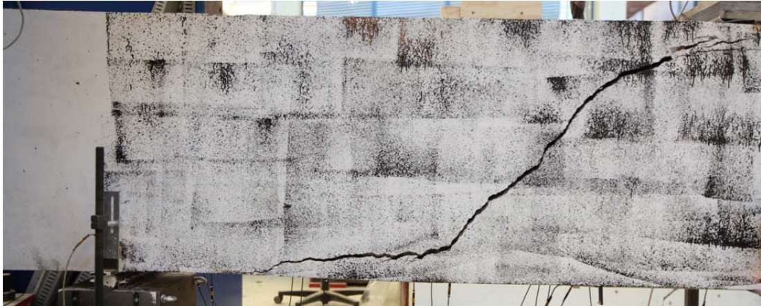
Fig. 5.88.1. Crack pattern after failure at north side of beam
