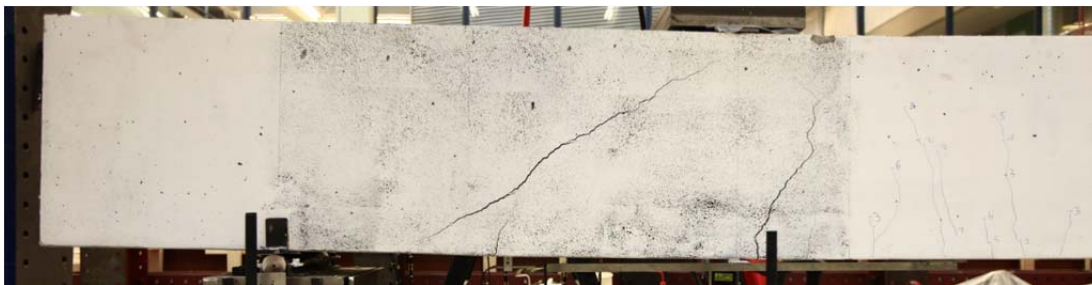
Fig. 5.79.1. Crack pattern after failure front side
