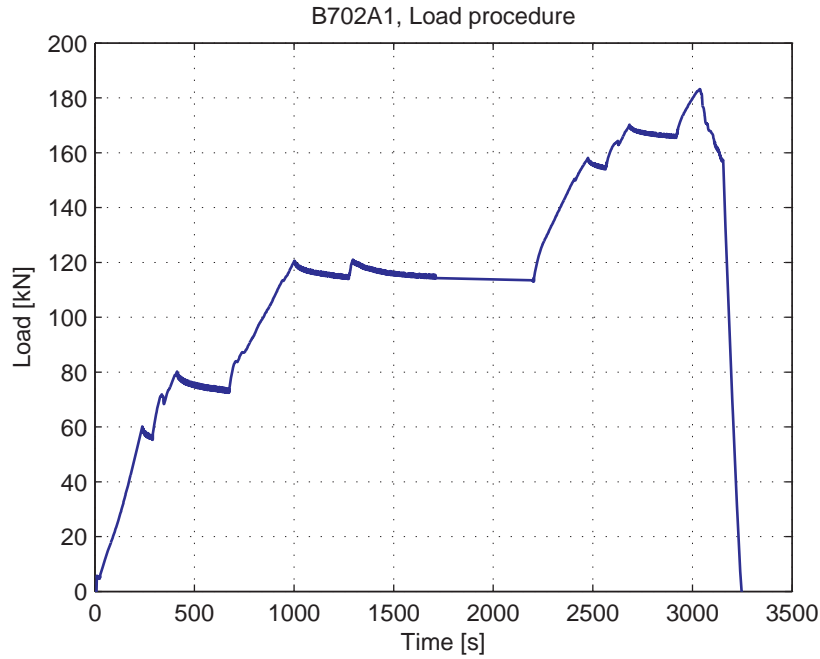
Fig. 5.45.3. Load-Time curve
