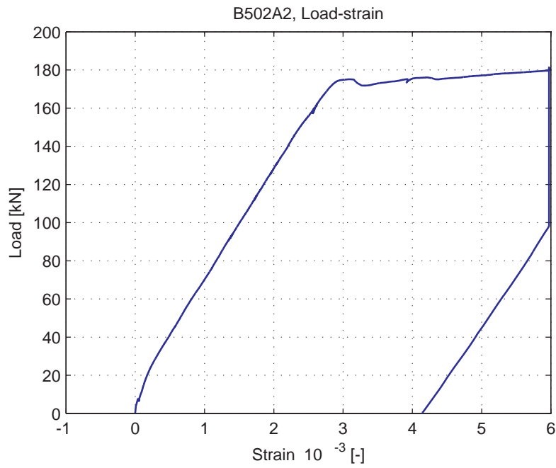
Fig. 5.51.9. Average strain over 1m length, measured at bottom of specimen (LVDT 3)
