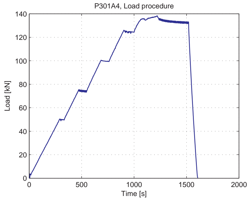
Fig. 5.74.4. Load-Time curve
