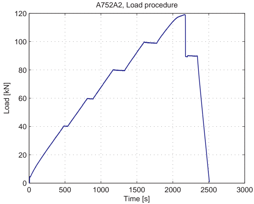
Fig. 5.27.3. Load-Time curve
