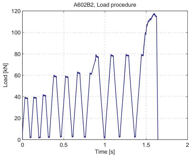
Fig. 5.39.3. Load-Time curve
