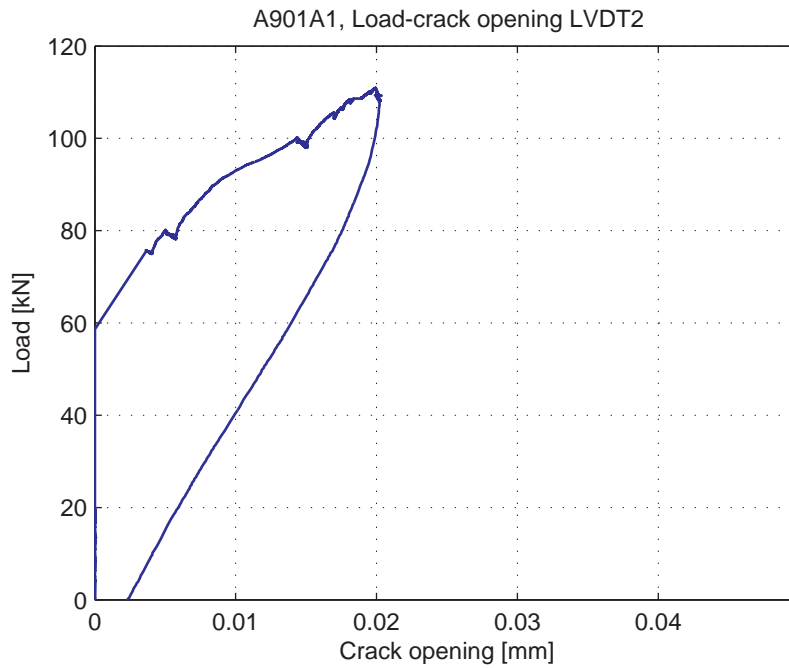
Fig. 5.12.6. Load-Crack opening for LVDT2
