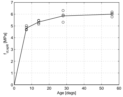
Fig. 2.2.12. F_{ct,split} development for cast 7
