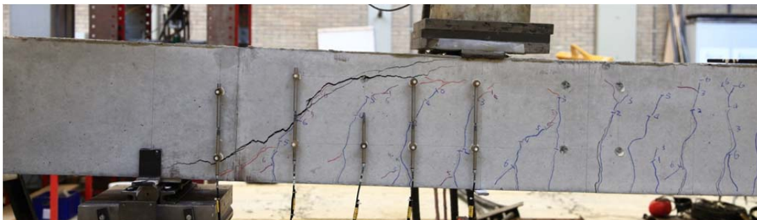
Fig. 5.14.1. Crack pattern after failure north side
