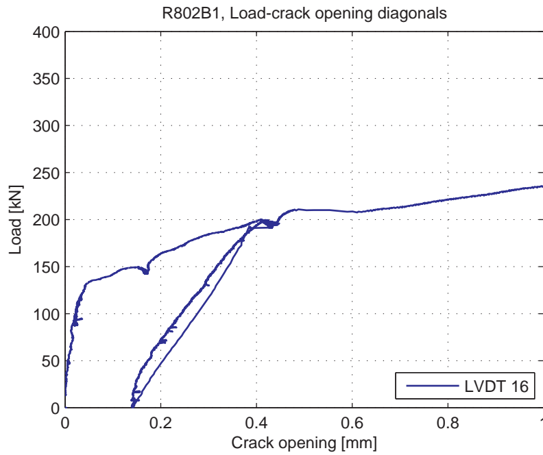
Fig. 5.103.9. Load-Crack opening for LVDT 16 (diagonal)
