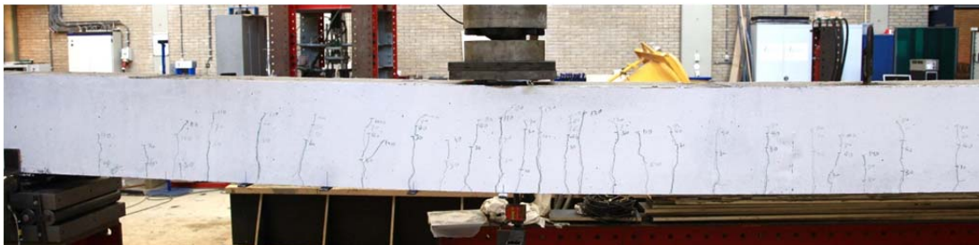
Fig. 5.1.1. Crack pattern after failure north side
