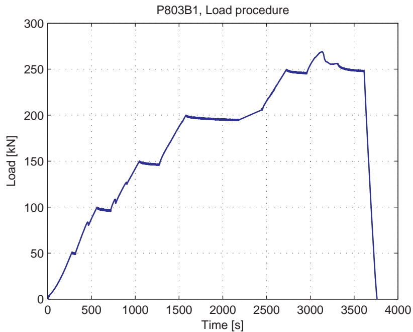
Fig. 5.90.4. Load-Time curve
