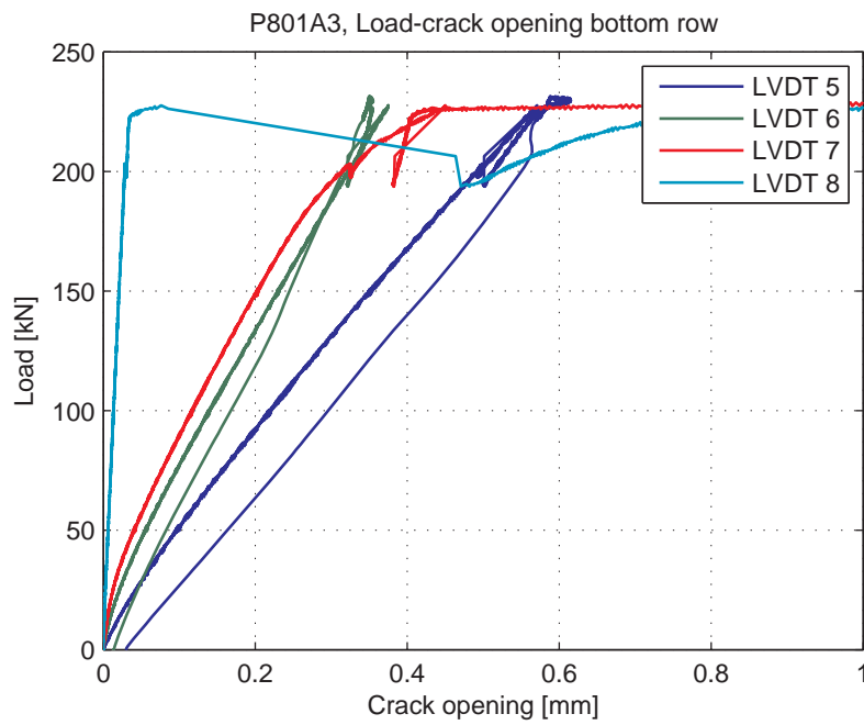
Fig. 5.85.8. Load-Crack opening for LVDT's 5-8 (bottom row)
