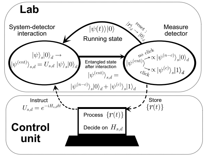
FIG. 1. Basic design of the measurement-driven state preparation. The procedure starts with a given initial state \rho_{\text{in}} and proceeds with a protocol, as described in Definition 1, until a good approximation of the target state |\psi_{\text{targ}}\rangle is achieved. The control unit decides on the system-detector interaction unitary U_{s,d} based on the stored record of detector readouts. We focus on constructing an optimized policy for decision making, such that the target state is prepared as quickly as possible.
