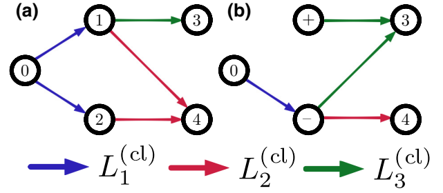
FIG. 6. Possible configurations of quantum subgraphs in a QSM, exemplified by the five-vertex subgraph of a hypothetical QSM. (a) The click-action graphs for the three operators V_{1,2,3} that form the family of couplings. The operators have the form V_1 = \gamma_1 (|1\rangle - |2\rangle)\langle 0| , V_2 = \gamma_2 |4\rangle\langle (|1\rangle - |2\rangle) , V_3 = \gamma_3 |3\rangle\langle 1| . The graphs for the no-click actions are not shown, as their form can be deduced from the graphs for click actions. In the present basis, the V_1 click is manifest as a superposition, the V_2 click—as an interference, and the V_3 click corresponds to a semiclassical evolution. (b) Quantum state machine for the coupling family from the previous panel, depicted in a different basis. The basis transformation is |\pm\rangle = (|1\rangle \pm |2\rangle)/\sqrt{2} . In this case, the basis transformation removes the quantum elements in the L_{1,2}^{(cl)} graphs, however, it turns L_3^{(cl)} into an interference element. Note that there is no basis transformation that would turn such a QSM into a classical one. This statement follows from the uniqueness of the Jordan canonical form for operators V_2 and V_3 .
