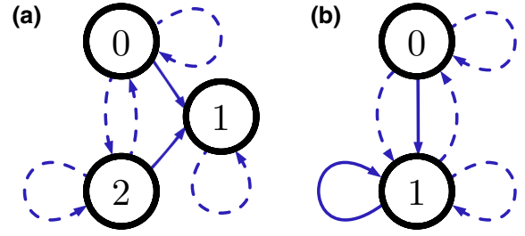
FIG. 4. Examples of steering graphs (see definition in Sec. V A). (a) Steering graphs on a three-level system, corresponding to the coupling V_s = \gamma(|1\rangle\langle 0| + |1\rangle\langle 2|) . Graph L^{(\text{cl})} for click action is depicted with solid arrows and the graph L^{(\text{ncl})} for no-click action with dashed arrows. Due to the identity operator in Eq. (29), every vertex is decorated with a self-loop from the L^{(\text{ncl})} graph. To see how the rest of L^{(\text{ncl})} can be deduced from L^{(\text{cl})} , consider the example of e_{02}^{(\text{ncl})} (dashed arrow from state 0 to 2). According to the graphical approach from Sec. V A, one is to follow edge e_{01}^{(\text{cl})} (solid arrow from 0 to 1) forward and then e_{21}^{(\text{cl})} (solid arrow from 2 to 1) backward—and thus manages to travel from state 0 to 2, in correspondence to e_{02}^{(\text{ncl})} . (b) Steering graphs on a two-level system, as defined by the coupling V_s = \gamma(|1\rangle\langle 1| + |1\rangle\langle 0|) . Following the same rule as above, intervertex edges of L^{(\text{ncl})} can be deduced from L^{(\text{cl})} . For example, by following the edge e_{11}^{(\text{cl})} forward and then the edge e_{01}^{(\text{cl})} backward, one performs a transition from state 1 to state 0, thus reproducing the edge e_{10}^{(\text{ncl})} from L^{(\text{ncl})} .
