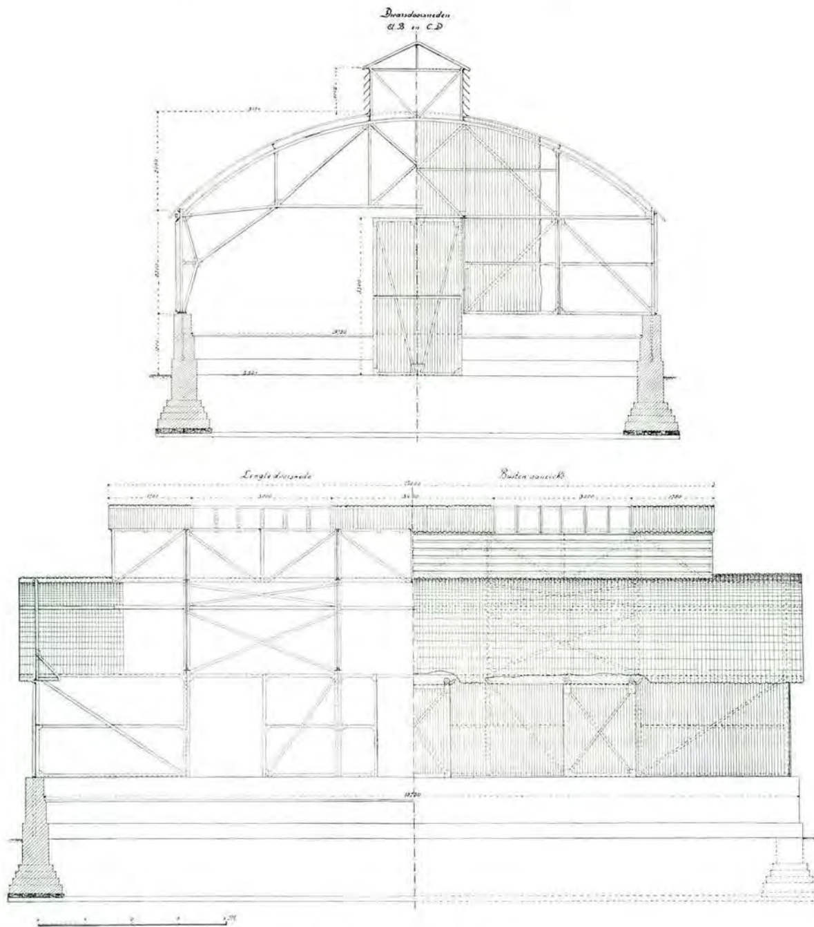
Fig. 17. Steenkolenloods.
