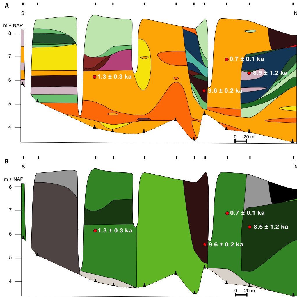
FIGURE 6 Cross-sections of the valley-fill (location in Figure 3C) including the OSL and ^{14}\text{C} sample locations. (A) Lithological cross-section. (B) Lithogenetic cross-section. Legend indicated in Figure 5
