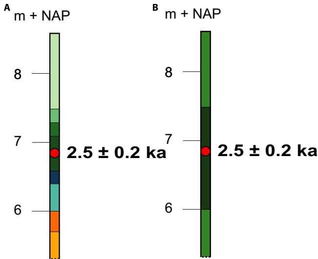
FIGURE 8 Borehole of the valley-fill (location in Figure 3C) including the OSL location. (A) Lithological sequence. (B) Lithogenetic sequence. Legend indicated in Figure 5
