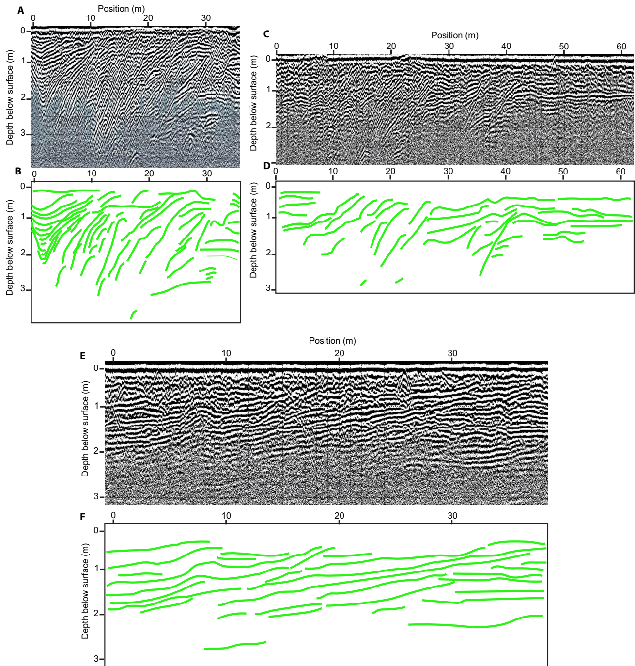
FIGURE 4 GPR transect examples. Locations are shown in Figure 3. (A, C, E) Plain GPR data. (B, D, F) Interpreted subsurface strata
