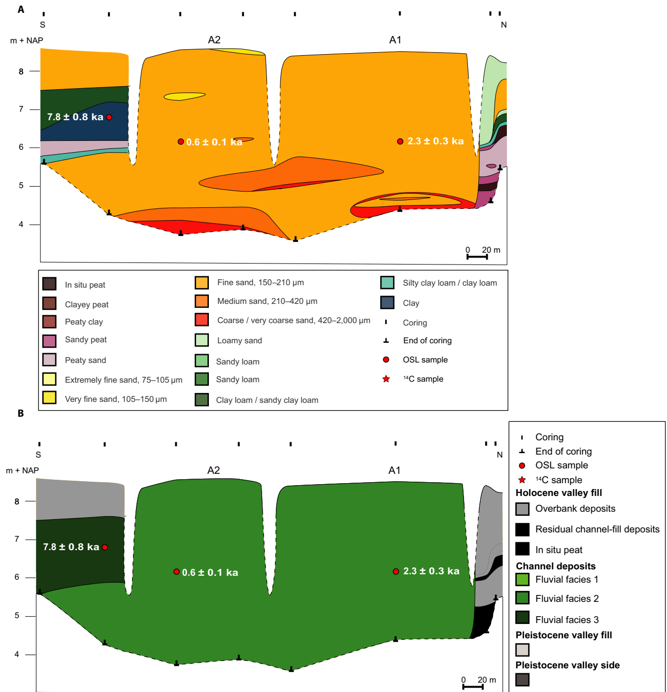
FIGURE 5 Cross-sections of the valley-fill (location in Figure 3A) including the OSL sample locations. (A) Lithological cross-section. (B) Lithogenetic cross-section. Location of the bend complex A-1 and A-2 are indicated (see Figure 2D)
