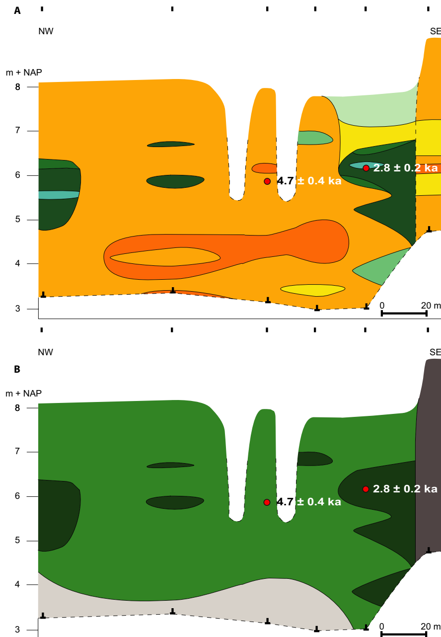
FIGURE 9 Cross-sections of the valley-fill (location in Figure 3E) including the OSL sample locations. (A) Lithological cross-section. (B) Lithogenetic cross-section. Legend indicated in Figure 5
