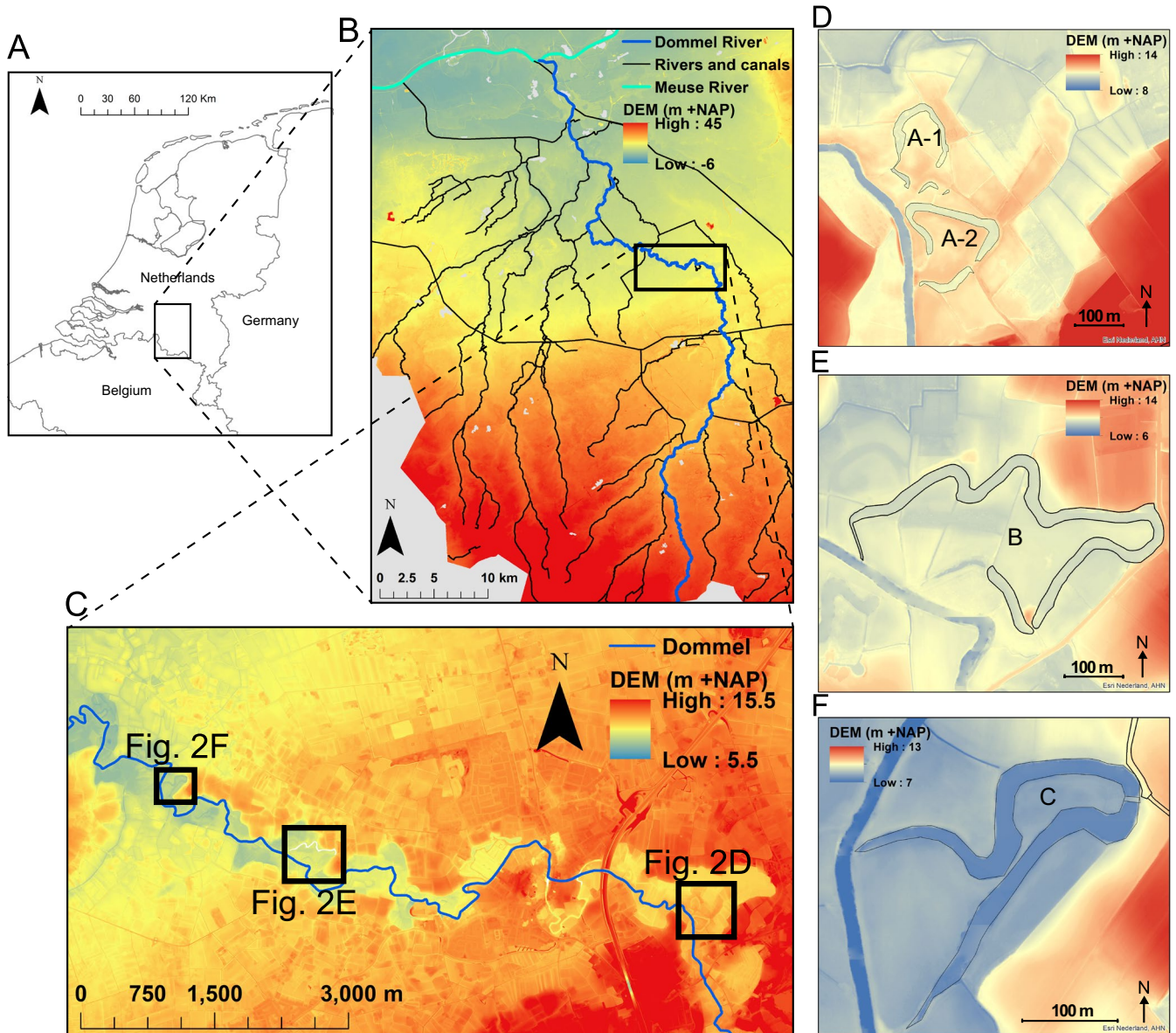
FIGURE 2 Maps of the Dommel River. (A) Map showing the location of the Dommel River in The Netherlands. (B) A digital elevation map (DEM, Actueel Hoogtebestand Nederland, 0.5 x 0.5 m grid) (Van Heerd and Van't Zand, 1999) of the Dutch section of the Dommel river. All study sites are indicated. (C) DEM of the three study locations A,B and C, showing the oxbow bend complexes (D through F)
