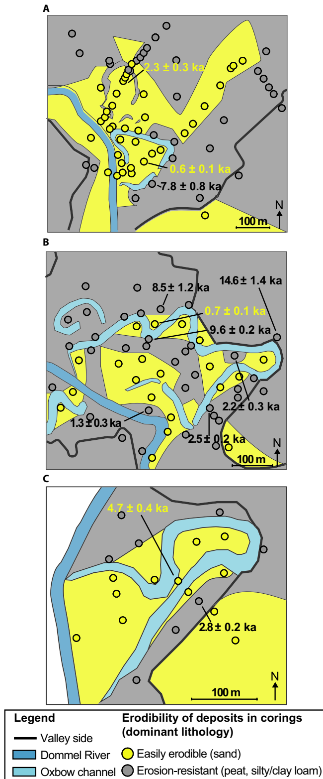
FIGURE 11 Simplified lithological maps showing the coring and dating (OSL and ^{14}\text{C} ) locations. Colours of the cores indicate the erodibility and dominant lithology at that location; map colours are based on spatial interpretation, based on coring information, surface morphology and GPR cross-sections. Ages shown in black are obtained on erosion-resistant material, while those in yellow are from easily erodible deposits
