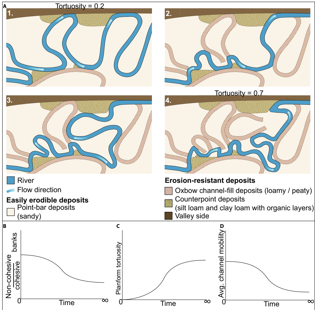
FIGURE 12 Self-constraining of a meandering river illustrated. (A) Conceptual maps showing the potential development of floodplain deposits and channel planform of a self-constraining river, assuming that neck cut-offs and counterpoint deposits immediately form erosion-resistant layers at the moment of cut-off or deposition. The tortuosity is indicated for the first and last timeframe. Conceptual graphs showing the long-term evolution of (B) bank cohesiveness, (C) planform tortuosity, and (D) average channel mobility
