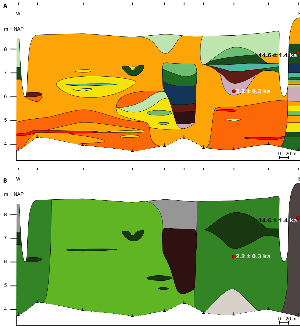
FIGURE 7 Cross-sections of the valley-fill (location in Figure 3C) including the OSL and ^{14}\text{C} sample locations. (A) Lithological cross-section. (B) Lithogenetic cross-section. Legend indicated in Figure 5
