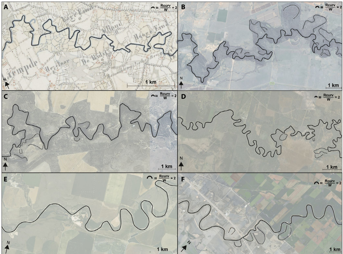
FIGURE 1 River planforms throughout the world, A through D showing tortuous meandering planforms, and E and F showing relatively classical meandering planforms, derived from Google Earth satellite imagery (2018) for B through F. All planforms are scaled to five predicted meander amplitudes (Carlston, 1965). (A) Dommel River in The Netherlands before the channelization, the planform was derived from the Topographical Military Map (TMK) dating from 1837 CE (Van der Linden, 1973) (51°34′12.3″N 5°24′43.6″E). (B) Murrumbidgee River in Australia (34°26′23.6″S 145°29′43.5″E). (C) Barwon River in Australia (30°00′00.0″S 147°58′00.0″E). (D) San Antonio River in USA (28°32′28.6″N 97°04′25.7″W). (E) Waterton River in Canada (49°26′22.87″N 113°27′33.36″W). (F) Assiniboine River in Canada (49°58′20.82″N 98°7′20.61″W)
