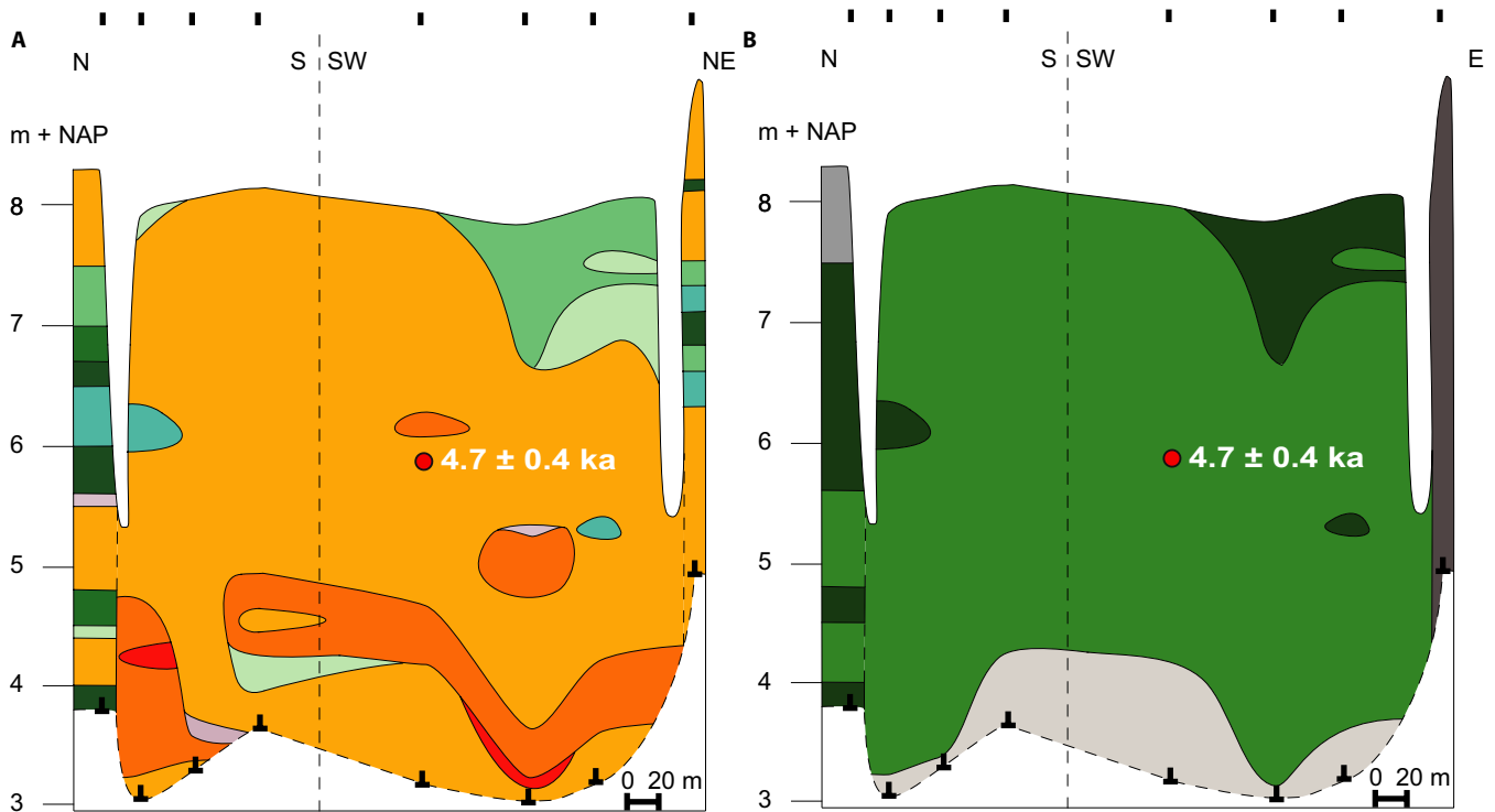
FIGURE 10 Cross-sections of the valley-fill (location in Figure 3E) including the OSL sample locations. (A) Lithological cross-section. (B) Lithogenetic cross-section. Legend indicated in Figure 5
