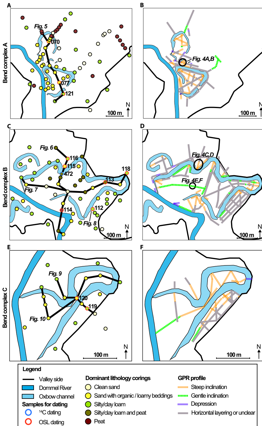
FIGURE 3 Maps of the study locations. (A, C, E) Simplified maps showing the coring, dating and transect locations. The colour infill of the coring locations indicate the main lithology that was found. The lines indicate the transects shown in Figures 5 through 10. The numbers refer to the last three digits of the OSL and ^{14}\text{C} sample codes, and indicate the sampling locations (Table 1). (B, D, F) Simplified maps showing the GPR profile locations; colours denote the observed structures. Some examples are given in Figure 4
