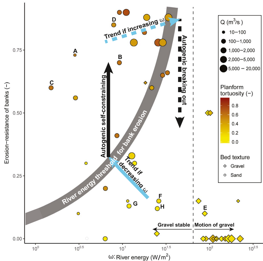
FIGURE 13 Erosion-resistance of banks (proxy: average silt-plus-clay fraction of river banks) plotted against river energy (proxy: potential specific stream power, \omega ) for a dataset of 47 rivers (Van den Berg, 1995; Kleinhans and Van den Berg, 2011). For each of the data points, effective channel-forming discharge ( Q ) (Kleinhans and Van den Berg, 2011), planform tortuosity and bed texture are shown. The thick grey line represents the minimum river energy needed to erode the river banks (Woodyer et al. , 1979; Page et al. , 2003; Julian and Torres, 2006; Kleinhans and Van den Berg, 2011). The thick arrows indicate the hysteresis cycle of self-constraining and breaking out, in black and blue the autogenic and allogenic processes, respectively. Dashed arrows represent hypothetical arrows. The labelled rivers correspond to rivers shown in Figure 1, or reconstructed Late-Glacial (LG) systems (see methods section on reconstruction). A through D refer to rivers with sharp bends, E through H refer to rivers with classical meandering planforms: A) Dommel River (Figure 1A), (B) Murrumbidgee River (Figure 1B), (C) Barwon River (Figure 1C), (D) San Antonio River (Figure 1D), (E) Waterton River (Figure 1E), (F) Assiniboine River (Figure 1F), (G) Late-Glacial Dommel River, (H) Late-Glacial Niers River
