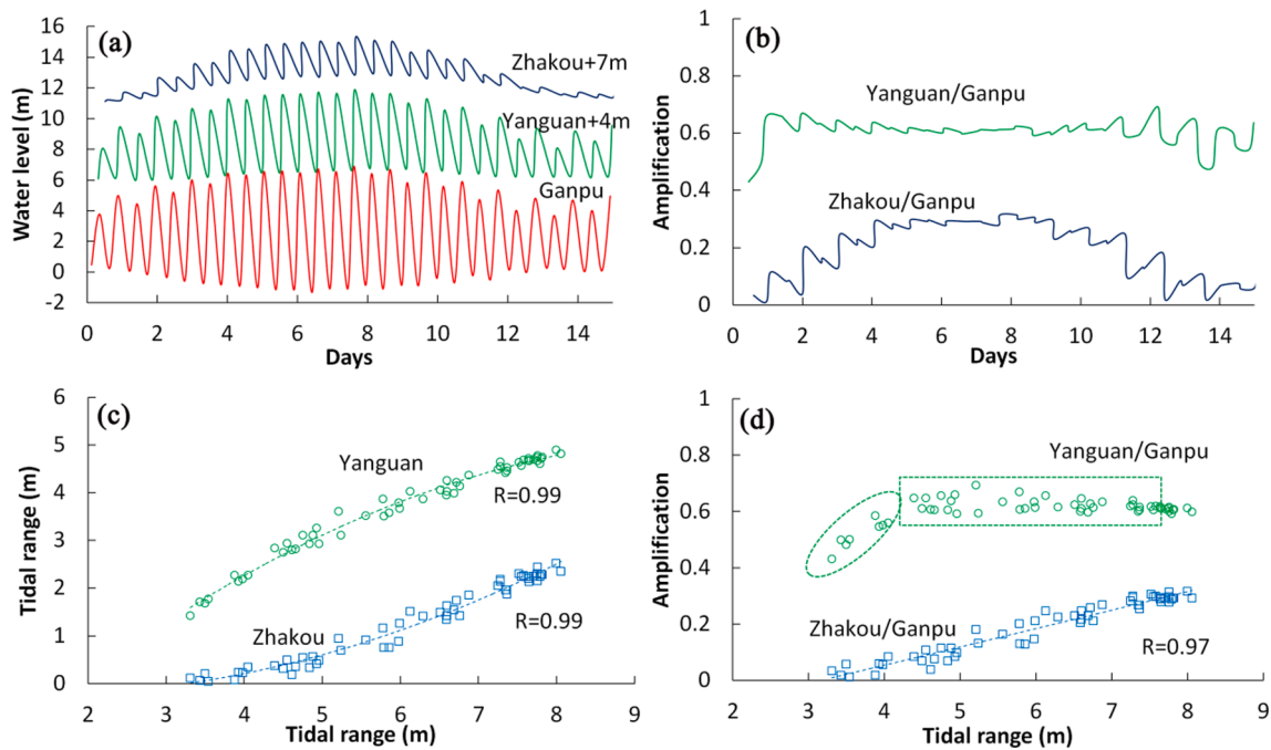
Fig. 5. Time series of water levels at Zhakou, Yanguan and Ganpu in October 2018 (a), and the corresponding amplification factors (b). The relationships between the tidal ranges (c) and the amplifications (d) at Zhakou and Yanguan and the tidal range at Ganpu.
