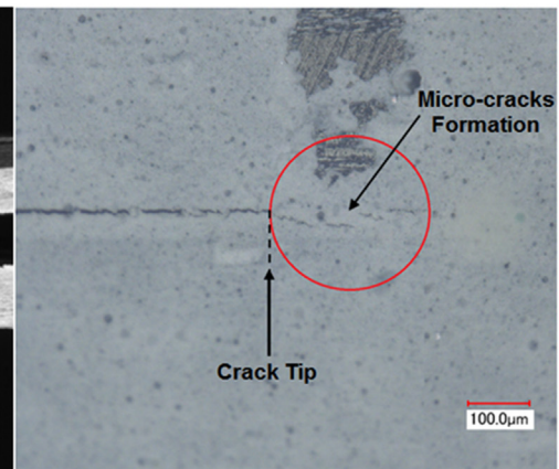
Fig. 4. (a) Schematic of fracture process zone in laminated composites; (b) Photograph of fiber bridging behind the crack tip and (c) Optical micrograph of the micro-cracks formation around the crack tip at magnification of 300 \times . The test was performed by the present authors.
