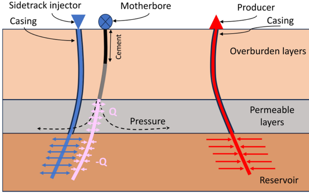
Figure 6: Schematic view of the sidetrack well, the motherbore (original injection well) and the production well. The grey section of the motherbore is assumed inactive and the pink part is assumed to be hydraulically connected to the reservoir.
