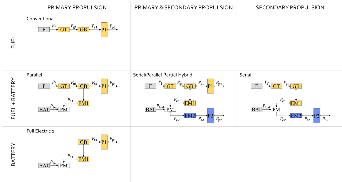
Figure 2: Notional representation of powertrain architectures, adapted from De Vries et al. 6 and Bonnin & Hoogreef. 2
