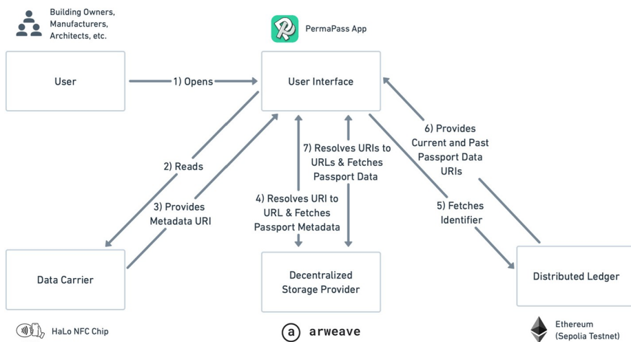
Figure 4. System architecture for reading a passport Source: Created by the authors
