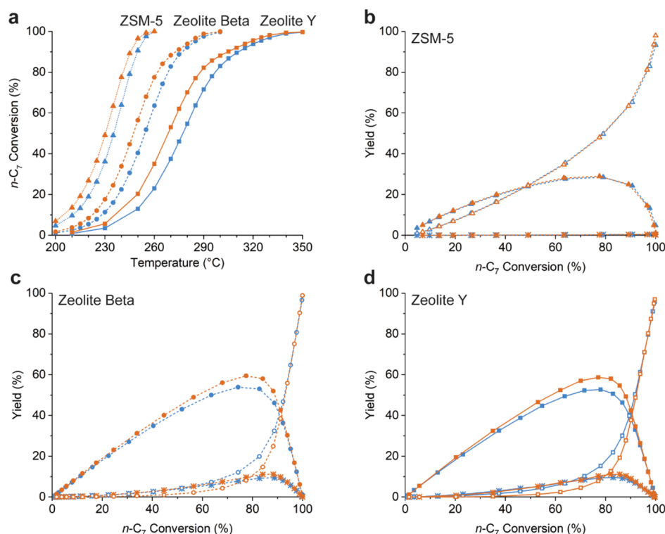
Figure 3. Catalytic activity of the Pt/ \gamma -Al 2 O 3 /zeolite composite catalysts (a), n -heptane conversion as a function of temperature, at a feed rate of 2.6 \text{ g}_{n\text{-C}_7} \cdot \text{g}_{\text{cat}}^{-1} \cdot \text{h}^{-1} , a total pressure of 10 bar, and 9 \text{ mol}_{\text{H}_2} \cdot \text{mol}_{n\text{-C}_7}^{-1} . Weight-based product yields toward monobranched isomers (closed symbols), dibranched isomers (asterisks), and C 3 and C 4 cracking products (open symbols) as a function of conversion for the ZSM-5-based catalyst (b), zeolite Beta-based catalyst (c), and zeolite Y-based catalyst (d). Catalysts with Pt nanoparticles located in the zeolite are indicated in blue, while catalysts with Pt nanoparticles located on the \gamma -Al 2 O 3 binder are indicated in orange. The differences in temperature of samples based on the same zeolite are within a margin of 5–10 °C, while differences between catalysts based on ZSM-5 and zeolite Y are \sim 50 °C.
