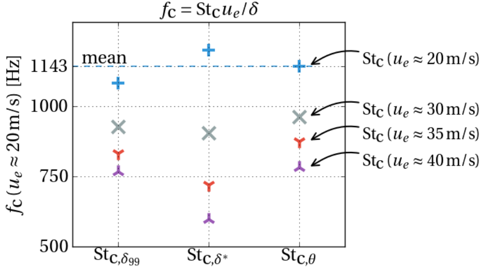
Figure 18: Predicted value of f_c based on the pressure side measurements of St_c based on U_\infty = 30 m/s ( \times ), U_\infty = 35 m/s ( \gamma ), U_\infty = 40 m/s ( \wedge ), and the linear extrapolation to U_\infty = 20 m/s ( + ).
