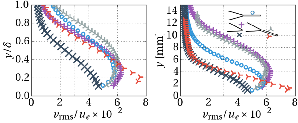
Figure 16: Wall-normal fluctuations, v_{rms} .
