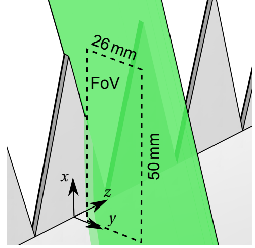
Figure 8: Location of the field of view for the stereoscopic PIV measurements in the z/\lambda = 0.25 measurement plane.
