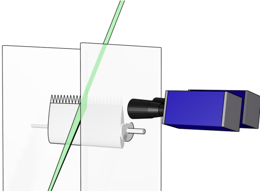
Figure 5: Planar PIV measurement setup.
