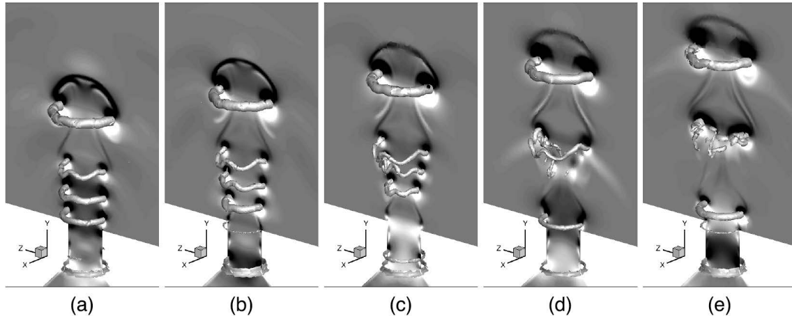
Figure 10. Vertical density gradient (vertical plan) and Q iso-criteria surfaces (3D) for (a) t = 60 \mu s ; (b) t = 65 \mu s ; (c) t = 70 \mu s ; (d) t = 75 \mu s ; (e) t = 80 \mu s [63].
