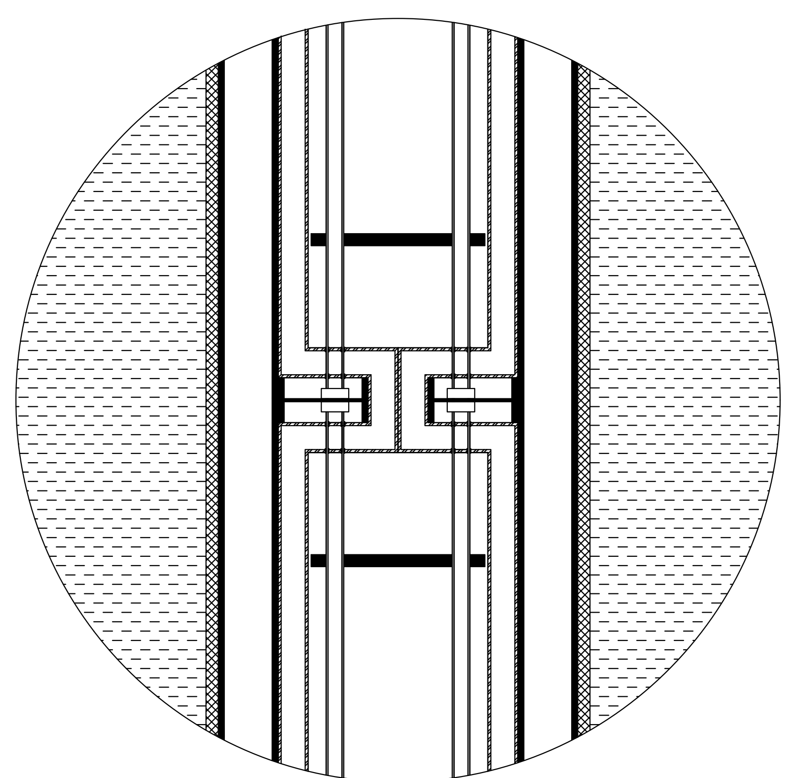
CONNECTION DETAIL 1-5
