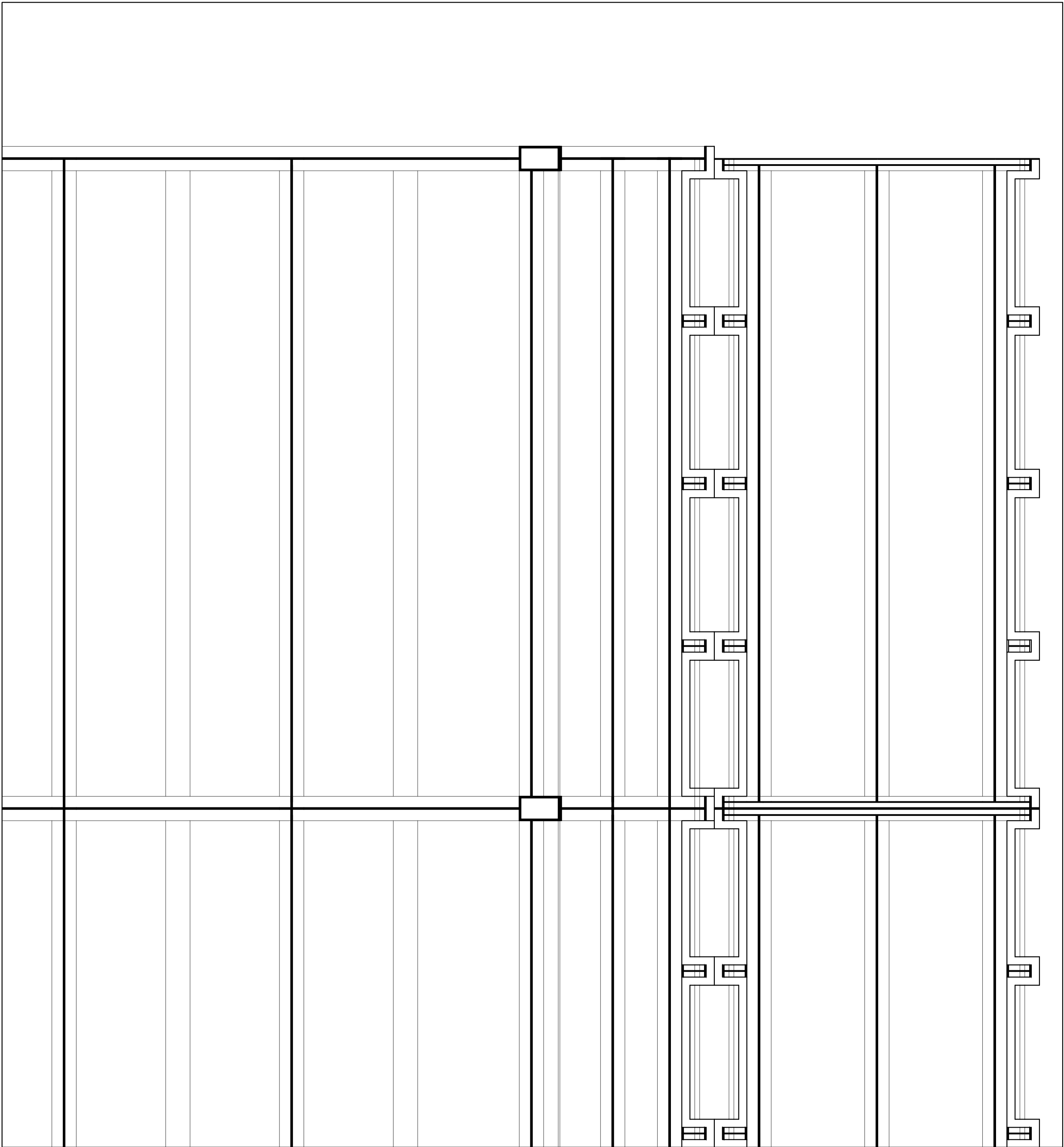
HORIZONTAL SECTION 1-20
