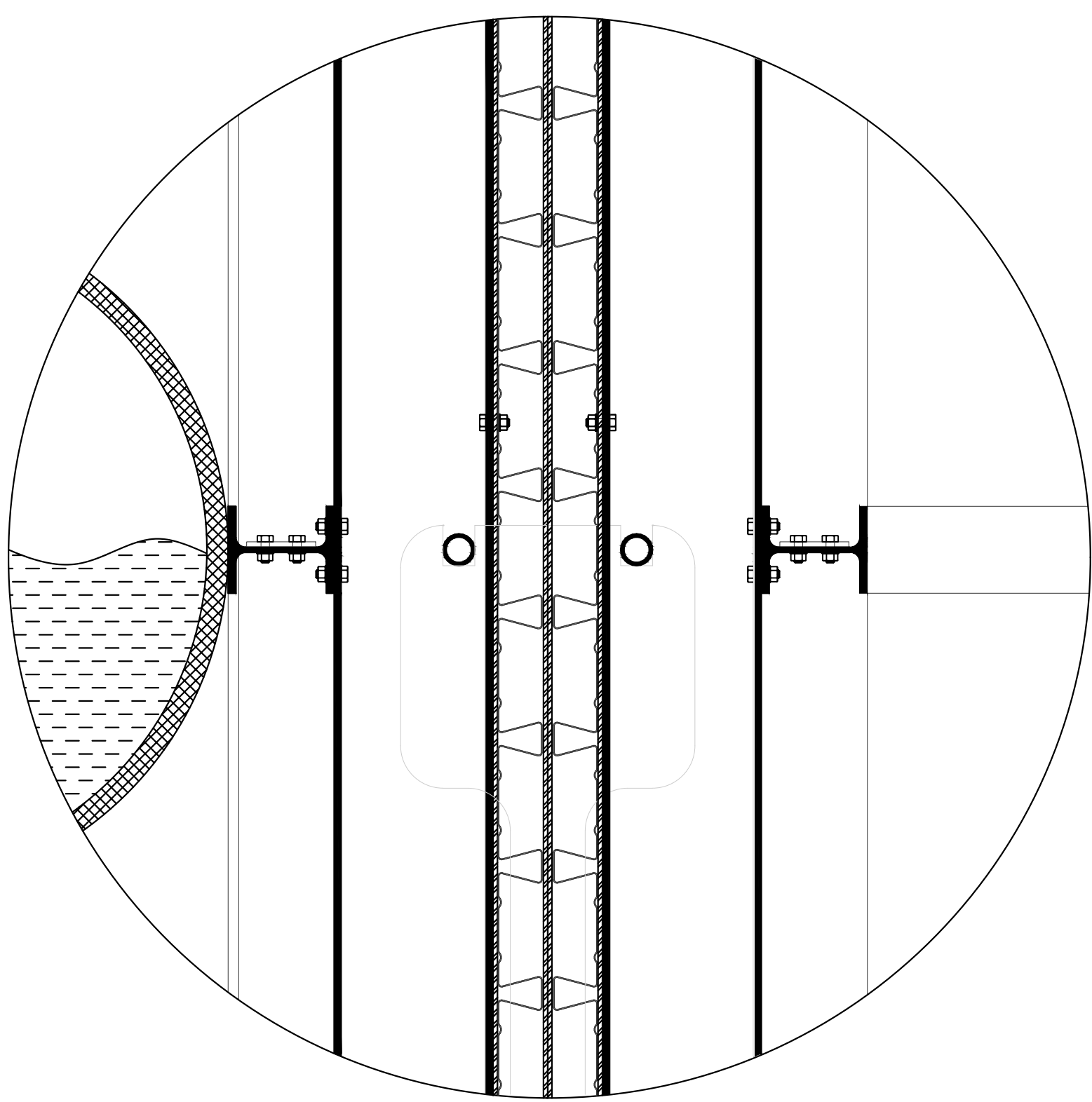
CONNECTION DETAIL 1-5
