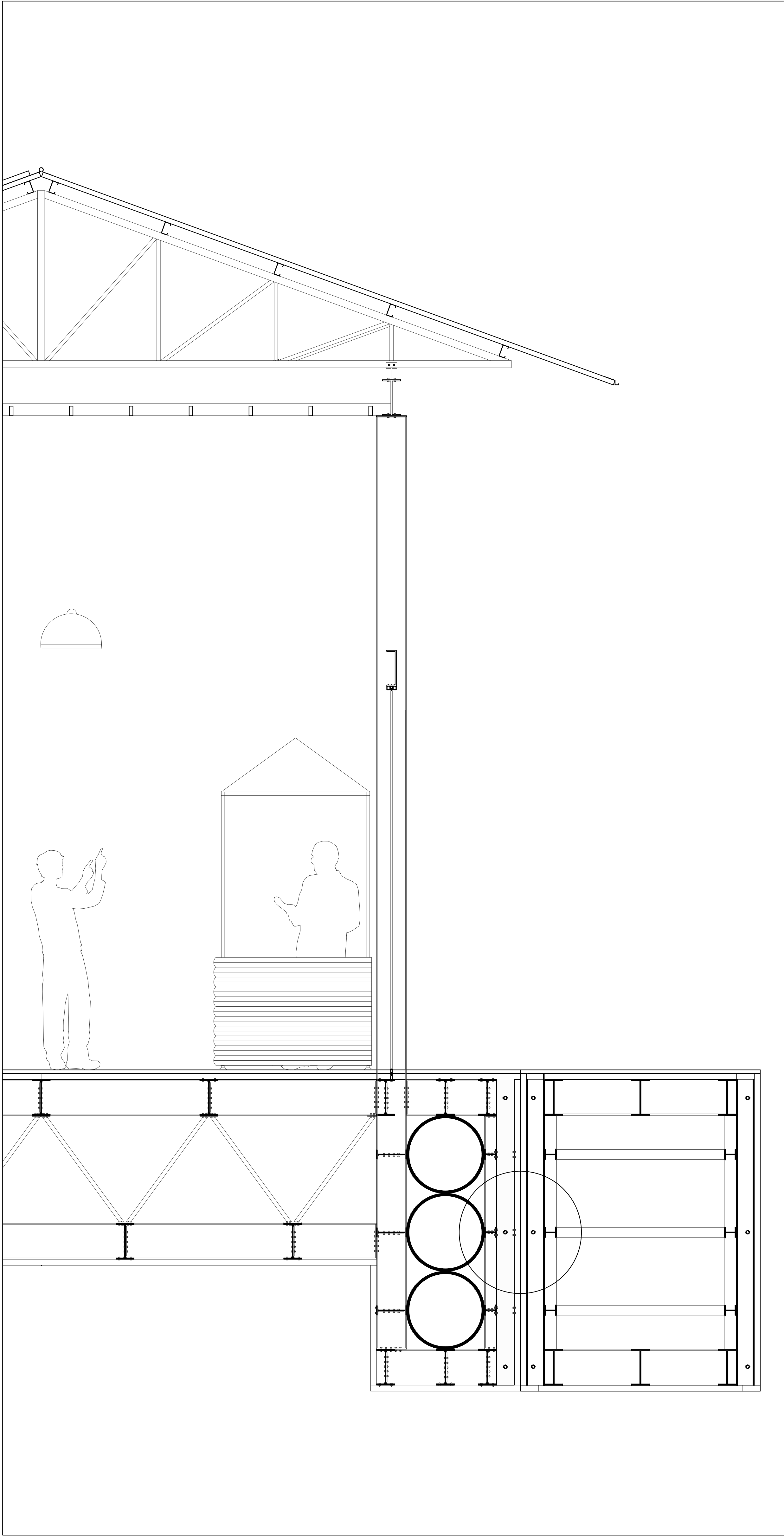
VERTICAL SECTION 1-20
