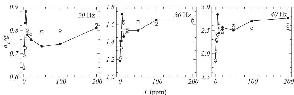
Figure 7. Comparison of computed and measured onset acceleration as a function of surfactant concentration. The computed a_c values were inferred from a measurement of the pattern wavelength, combined with the linear Floquet theory. Filled circles are the direct measurements, and empty circles are computations. The error bars of the computed a_c are derived from the uncertainty in the measured wavelength.
