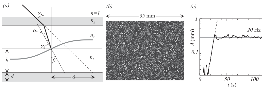
Figure 3. Estimating the amplitude of interfacial waves. (a) The apparent displacement \delta of a dot pattern reflects the gradient \nabla h = \beta of the interface. The relation between \delta and \beta follows the derivation by Moisy et al., 31 but now we also have to account for refraction between the upper fluid layer and air. The refraction at the glass top cover is not shown, but the relation between the gradient \nabla h and the apparent displacement \delta in eq 9 does allow for these covers. (b) Image of a dot pattern that is deformed by the interfacial waves. (c) Wave amplitude A at driving frequency \Omega/2\pi = 20 Hz as a function of time after the start of the excitation. After an exponential rise, the wave amplitude is saturated when A = 0.3 mm. It will be used to estimate flow velocities in eq 9.
