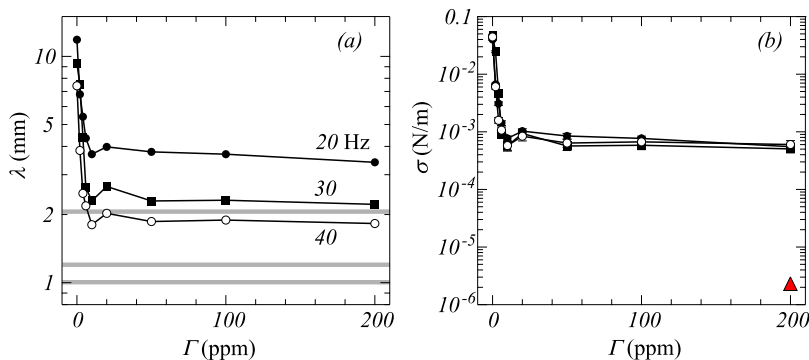
Figure 5. (a) Measured wavelengths of Faraday waves driven at \Omega/2\pi = 20, 30, and 40 Hz, for filled circles, filled squares, and empty circles, respectively, as a function of surfactant concentration \Gamma . The three horizontal lines indicate the minimum wavelength \lambda_{th} of waves in the limit of vanishing interfacial tension \sigma . This limiting wavelength decreases monotonically with an increase in frequency. (b) Interfacial tension computed from the wavelengths in panel a. The red triangle indicates a reference measurement of the interfacial tension using a spinning drop tensiometer. The error bars, obscured by the symbols, were computed from the uncertainty in the measured wavelength.
