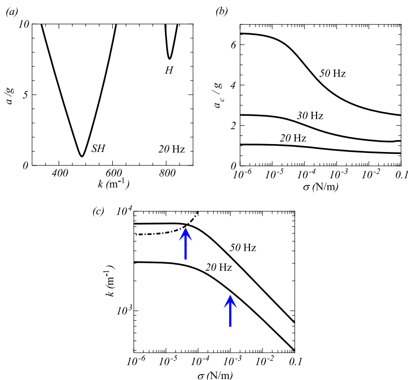
Figure 1. Faraday waves on the interface between water (1) and dodecane (2). The mass densities and viscosities are as follows: \rho_1 = 1000 \text{ kg m}^{-3} , \rho_2 = 749.5 \text{ kg m}^{-3} , \eta_1 = 1.0 \times 10^{-3} \text{ kg m}^{-1} \text{ s}^{-1} , and \eta_2 = 1.34 \times 10^{-3} \text{ kg m}^{-1} \text{ s}^{-1} . (a) Neutral stability curve for the subharmonic (SH) and harmonic (H) response of an interfacial layer at driving frequency \Omega = 20 Hz and interfacial tension \sigma = 5.287 \times 10^{-2} N/m (corresponding to the clean interface). The onset wavenumber k_c and driving amplitude a_c/g where waves first appear on the surface correspond to the minimum of the neutral stability curve. (b) Critical acceleration amplitude a_c/g for \Omega values of 20, 30, and 50 Hz. (c) Dependence of the wavenumber k_c of the fastest-growing mode on the interfacial tension \sigma for driving frequencies \Omega of 20 and 50 Hz. For large values of \sigma , the curves follow the dependence k \sim \sigma^{-1/3} from eq 1. The dashed–dotted line indicates the wavenumber k_d above which waves are critically damped using \gamma_{k_d} = \omega_{0k_d} (eqs 1 and 2). The arrows indicate the wavenumber k_B where gravity and surface tension forces balance, i.e., where the Bond number, \text{Bo} = g(\rho_1 - \rho_2)/(\sigma k_B^2) , equals 1. At 50 Hz, this occurs when the dependence of k on \sigma has already flattened due to viscous damping. The results of this figure were computed using the linear Floquet theory of Kumar and Tuckerman. 7
