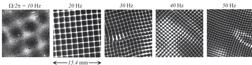
Figure 4. Images of waves at increasing driving frequencies and surfactant concentration \Gamma = 6 ppm. For frequencies \Omega/2\pi > 20 Hz, the square interface pattern can be recognized clearly.
