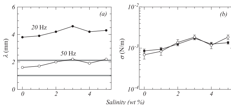
Figure 6. (a) Measured wavelength of Faraday waves driven at \Omega/2\pi = 20 and 50 Hz at a surfactant concentration \Gamma = 200 ppm and varying salt concentrations. The two horizontal lines indicate the theoretical minimum wavelength \lambda_{th} of waves in the limit of vanishing interfacial tension \sigma at driving frequencies of 50 Hz (bottom line) and 20 Hz (top line). (b) Interfacial tension computed from the wavelengths in panel a. The error bars are computed from an uncertainty of 0.2 mm in the measurement of the wavelengths.
