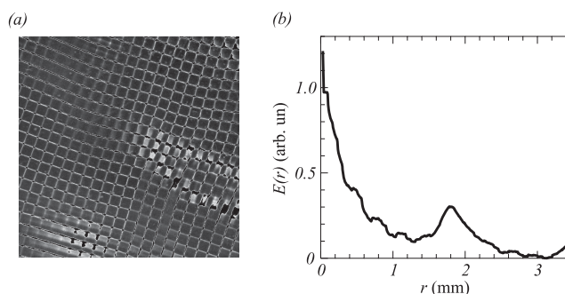
Figure 2. (a) Image of waves at driving frequency \Omega/2\pi = 50 Hz and acceleration amplitude a/g = 4.3 . (b) Azimuthally averaged energy spectrum, indicating a pattern wavelength \lambda = 1.8 mm.
